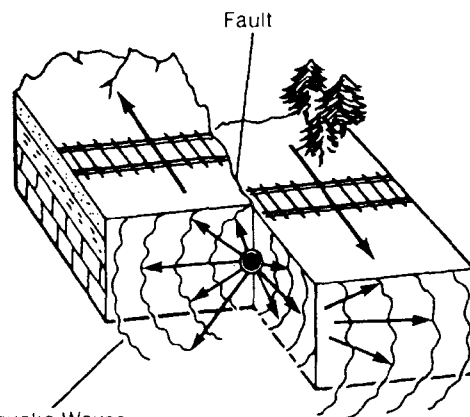
Earthquake Waves
