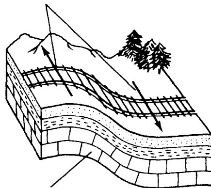
Deformed Rocks
