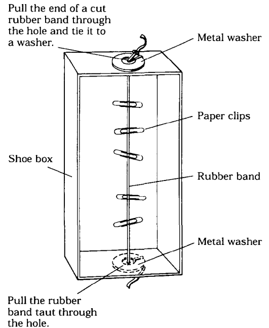
Master 35. The S-Wave Machine
