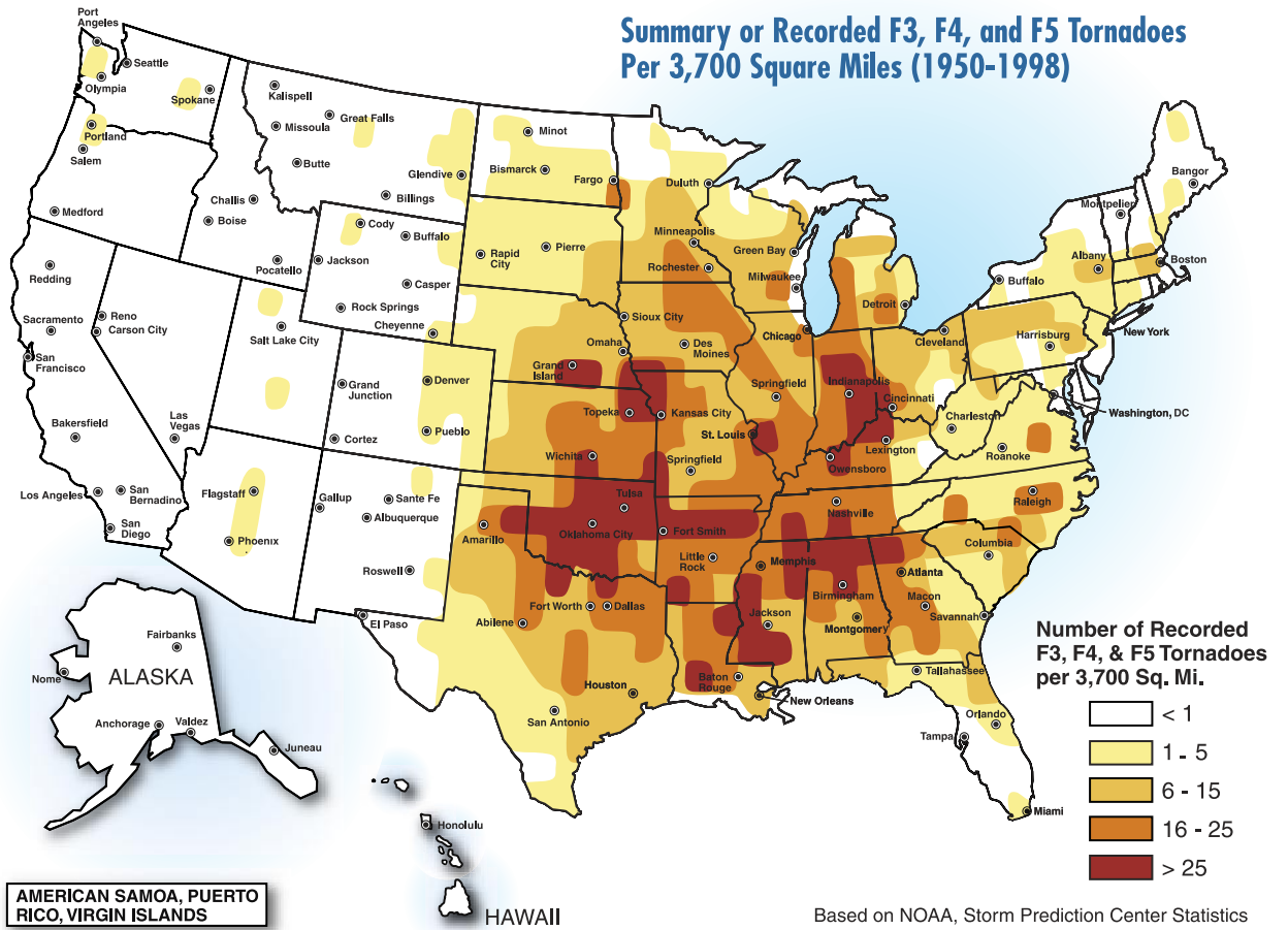
Figure 6-2 Tornado occurrence in the United States based on historical data
