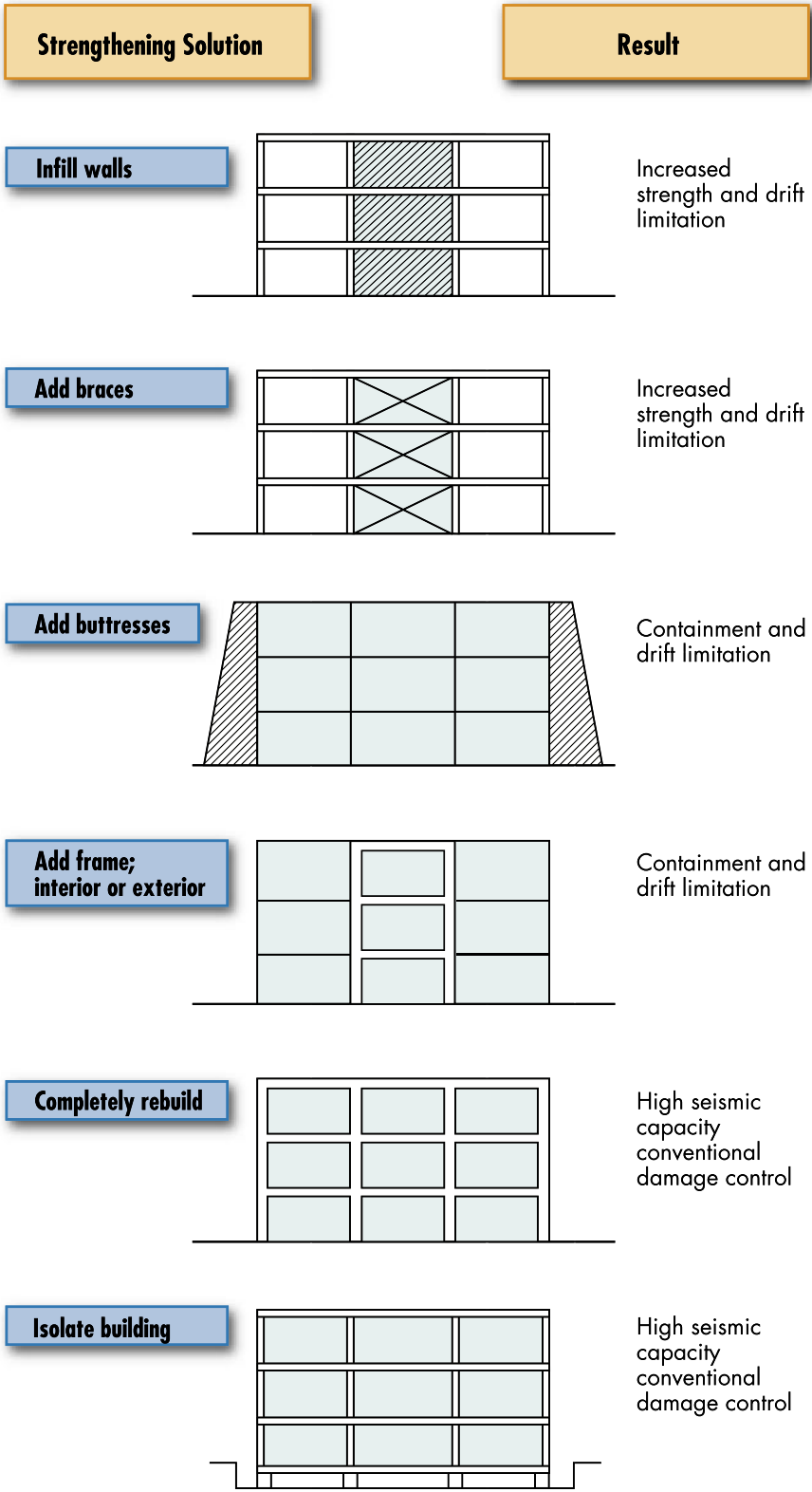
Figure 4-36 Design strategies for seismic retrofit of existing buildings
