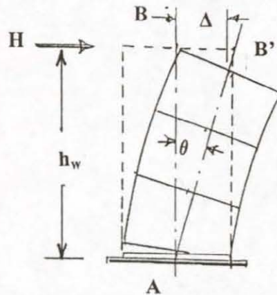
Fig. C9.6.2.2.1 Definition of drift ratio \theta .
