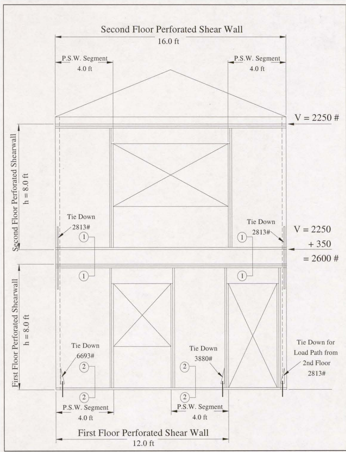
Figure C12.3-6 Elevation for perforated shear wall Example 2.
