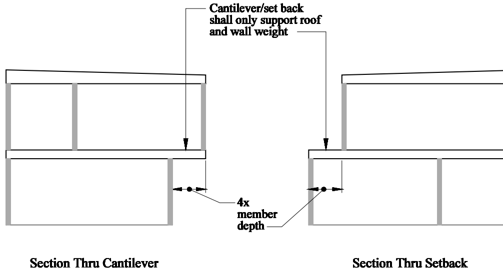
Figure 12.4-3 Permitted Cantilevers and Setbacks.
