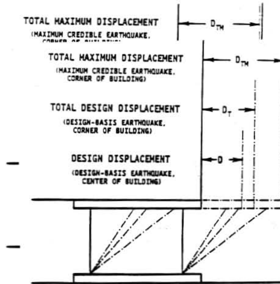
Figure C13.3-1 Displacement terminology.
