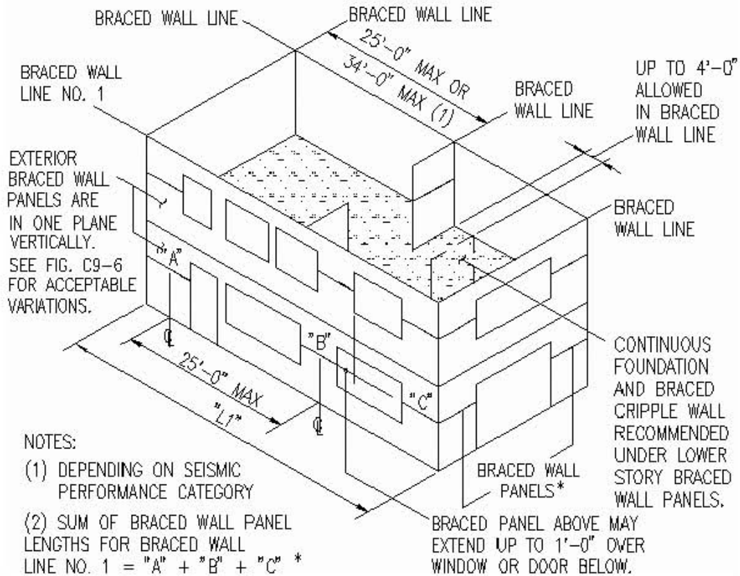
Figure C12.4-2 Acceptable two-story bracing example.
