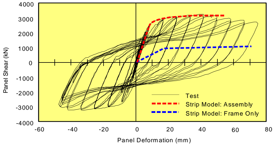
DRIVER ET. AL.'S TEST RESULTS FOR LOWER PANEL OF MULTI-STOREY SSPW FRAME
