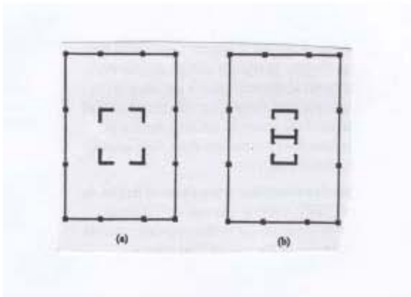
Figure C4.3-1 Arrangement of shear walls and braced frames – not recommended. Note that the heavy lines indicate shear walls and/or braced frames.
