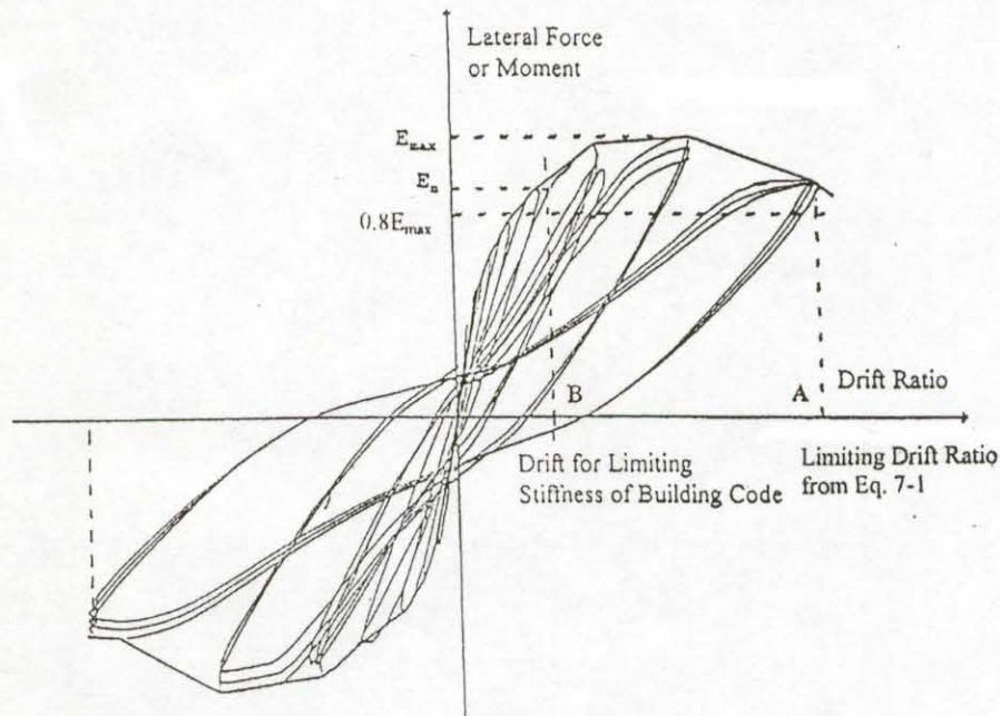
Fig. C9.6.9.1 Quantities used in evaluating acceptance criteria.
