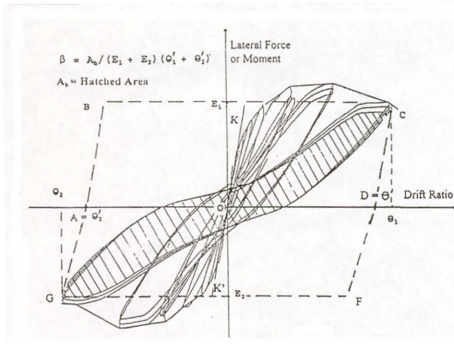
Fig. C9.6.2.5 Relative energy dissipation ratio.
