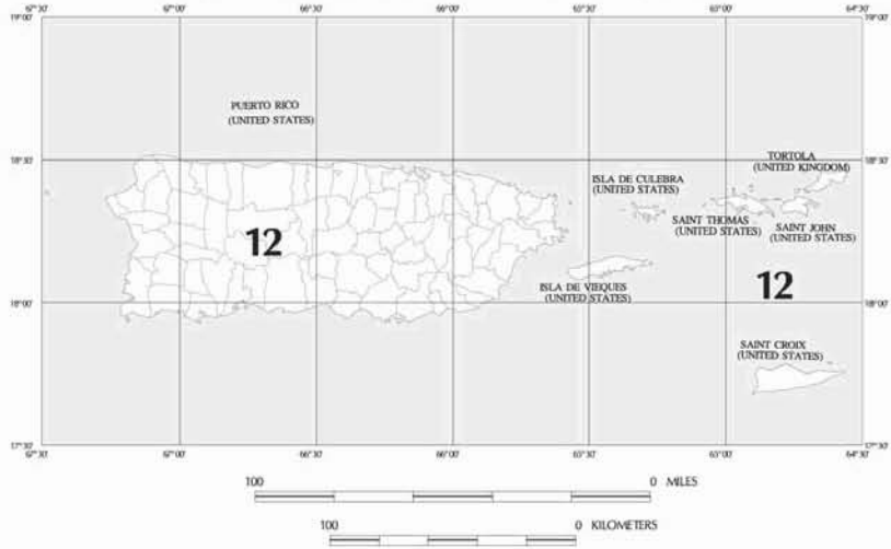
FIGURE 3.3-20 LONG-PERIOD TRANSITION PERIOD, T_i (sec), FOR PUERTO RICO, CULEBRA, VIEQUES, ST. THOMAS, ST. JOHN, AND ST. CROIX
