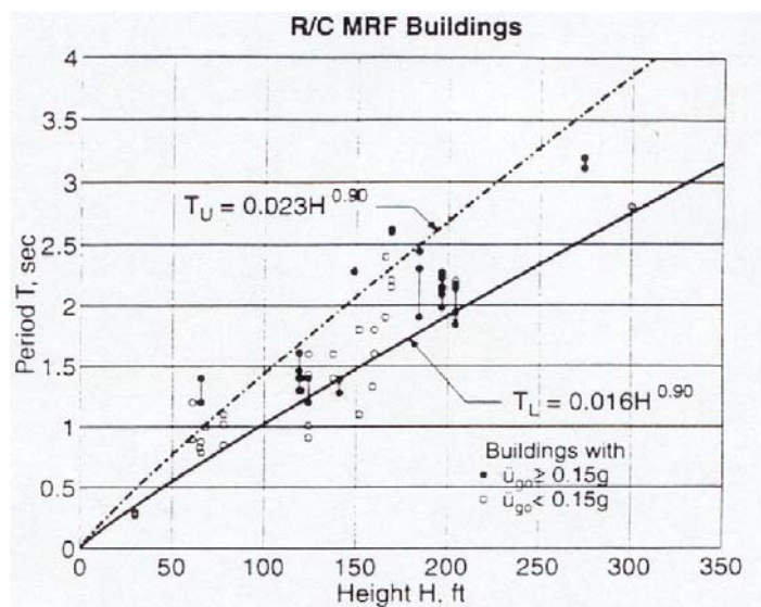
Figure C5.2-1 Measured building period for reinforced concrete frame structures.
