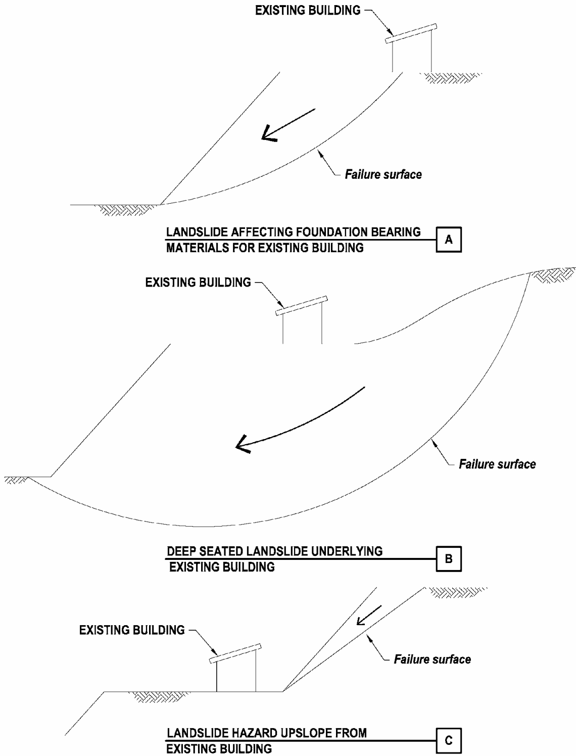
Figure 23.10.4-1: Landslide Hazards
