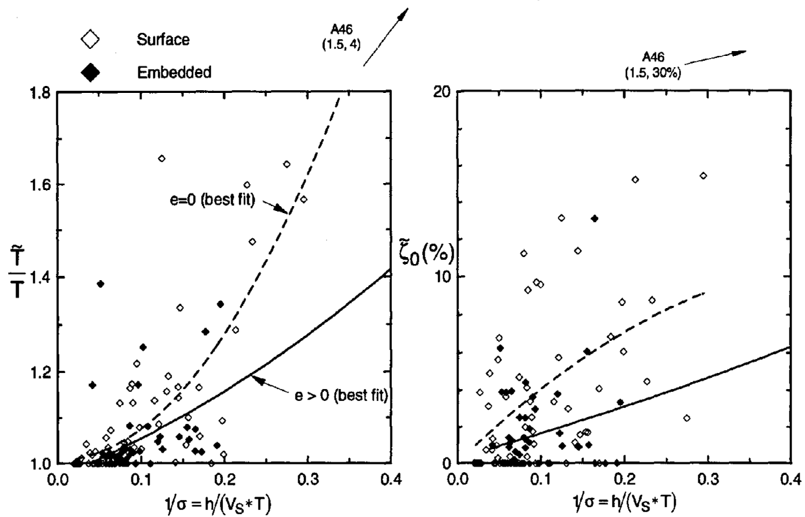
Fig. 5.10: Effect of embedment on period lengthening ratio and foundation damping factor
