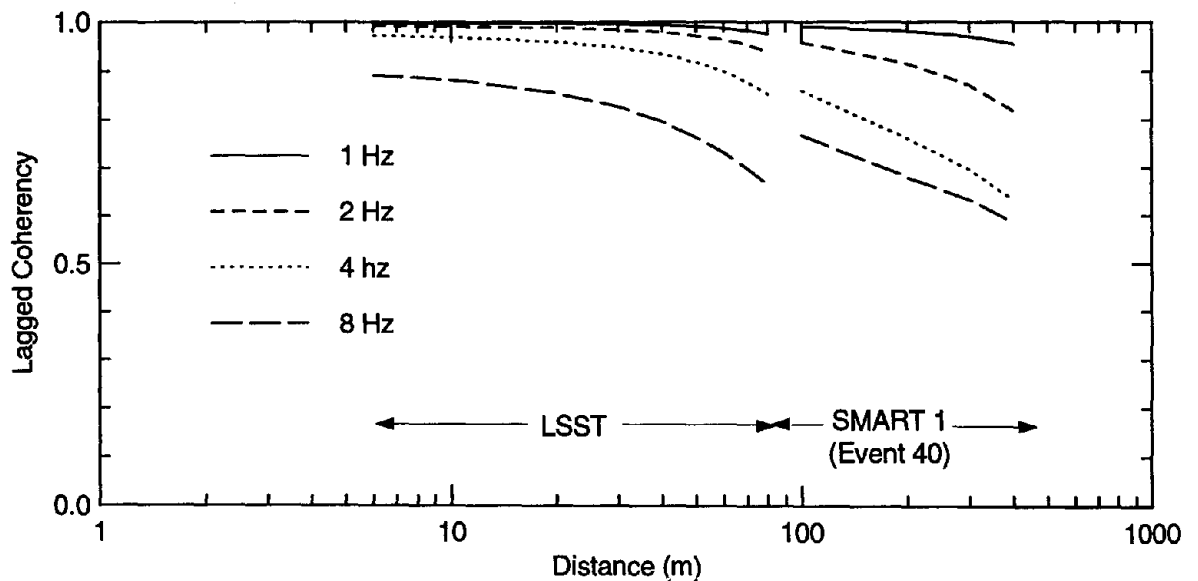
Fig. 4.6: Comparison of coherencies computed from regression equations in Abrahamson et al., 1991 for LSST array (all events) and Abrahamson, 1988 for SMART1 array (Event 40)
