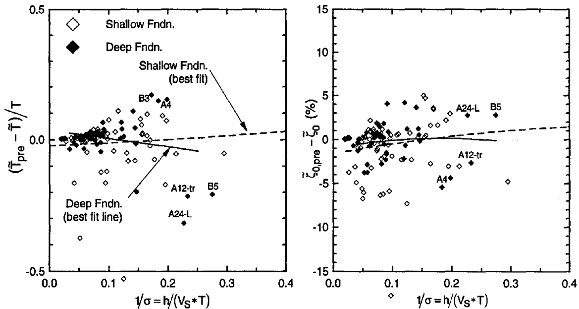
Fig. 5.18: Errors in predicted period lengthening ratios and foundation damping factors for sites sorted according to foundation type
