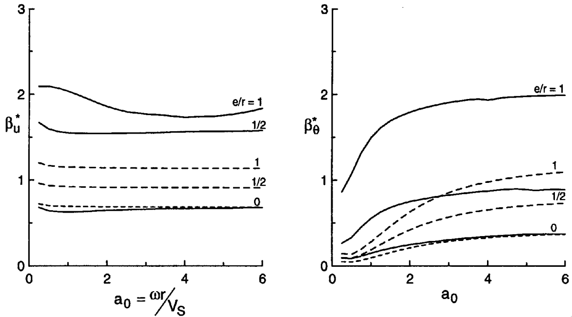
Fig. 2.5: Foundation stiffness and damping factors for rigid cylindrical foundations embedded in a halfspace; approximation vs. solution by Apsel and Luco (1987)
