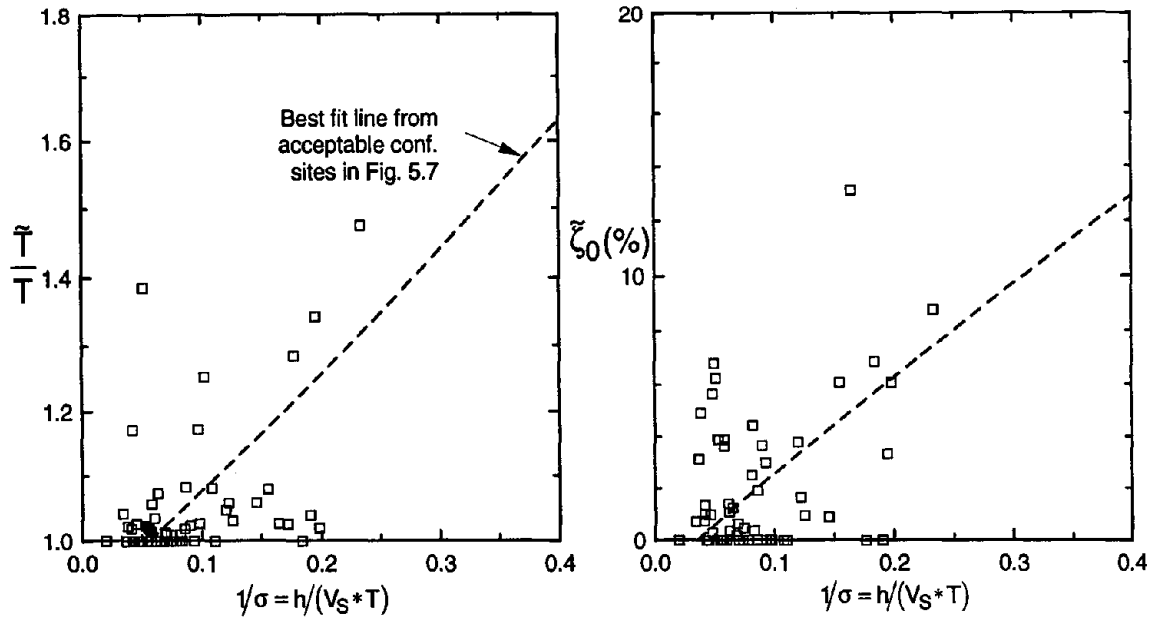
Fig. 5.12: Period lengthening ratios and foundation damping factors for moment frame and dual wall/frame buildings
