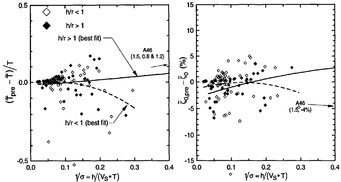
Fig. 5.17: Errors in predicted period lengthening ratios and foundation damping factors for sites sorted according to aspect ratio
