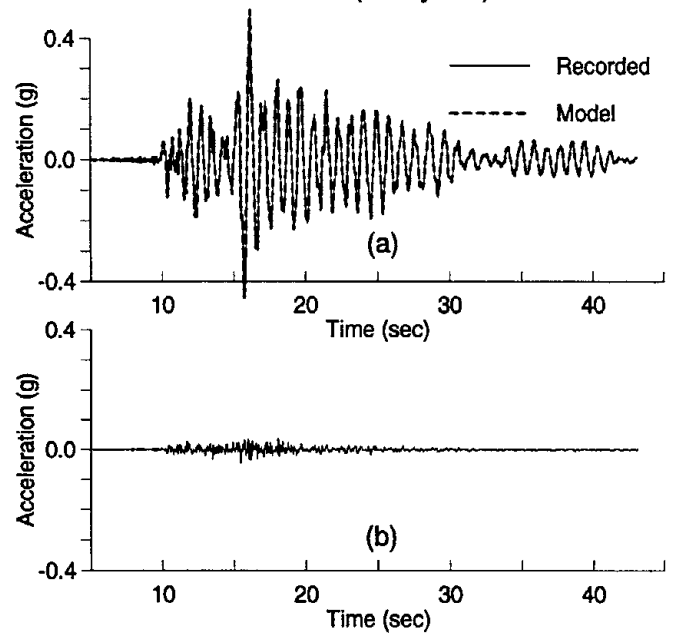
Fig. 3.7: (a) Comparison of model and recorded output, and (b) residual of identification for roof motions
