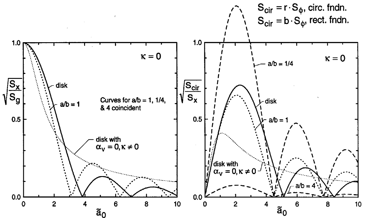
Fig. 2.14: Magnitudes of transfer functions between free-field ground motion and FIM for obliquely incident coherent waves. Curves for disk and vertically incident incoherent waves also shown for comparison (Veletsos et al., 1997 and Veletsos and Prasad, 1989)
