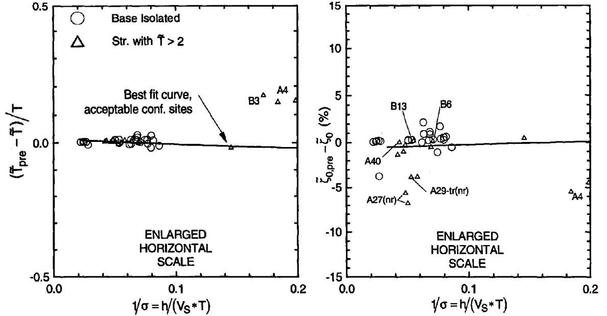
Fig. 5.19: Errors in predicted period lengthening ratios and foundation damping factors for sites with base isolated and long period structures
