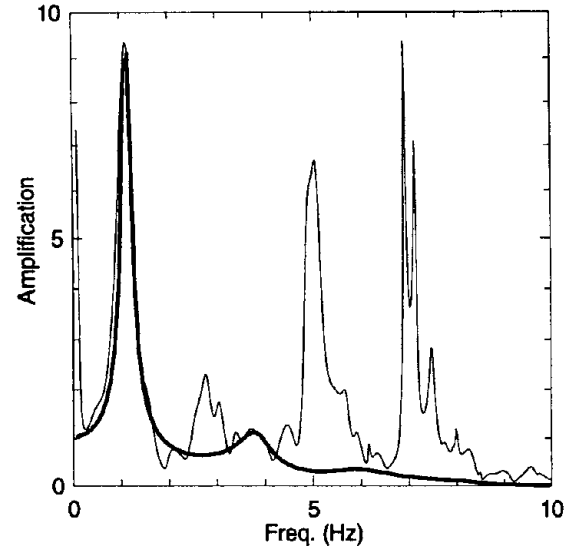
Fig. 3.5: Comparison of transmissibility functions from nonparametric analysis (light line) and parametric model (heavy line)
