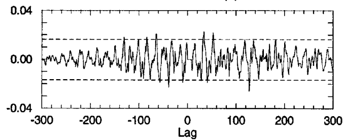
Fig. 3.8: Cross-correlation function between input and residual and 99% confidence limits of independence
