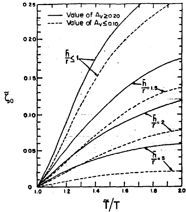
Fig. 5.22: Relationship between foundation damping factor ( \zeta_0 ) and period lengthening ratio for rigid disk foundation on homogeneous halfspace (BSSC, 1995; ATC, 1978)
