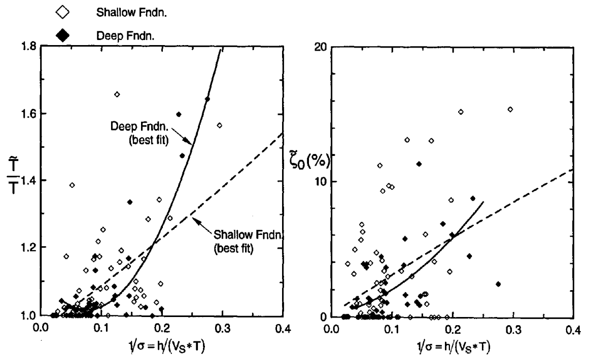
Fig. 5.9: Effect of foundation type on period lengthening ratio and foundation damping factor
