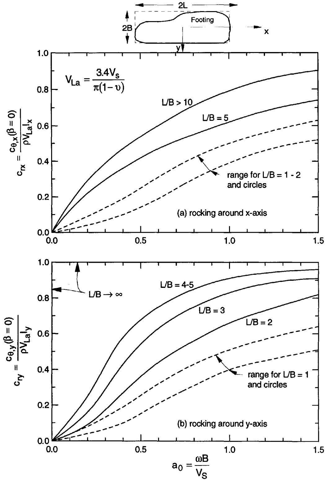
Fig. 2.6: Dashpot coefficients for rocking radiation damping vs. frequency for different foundation shapes (Dobry and Gazetas, 1986)
