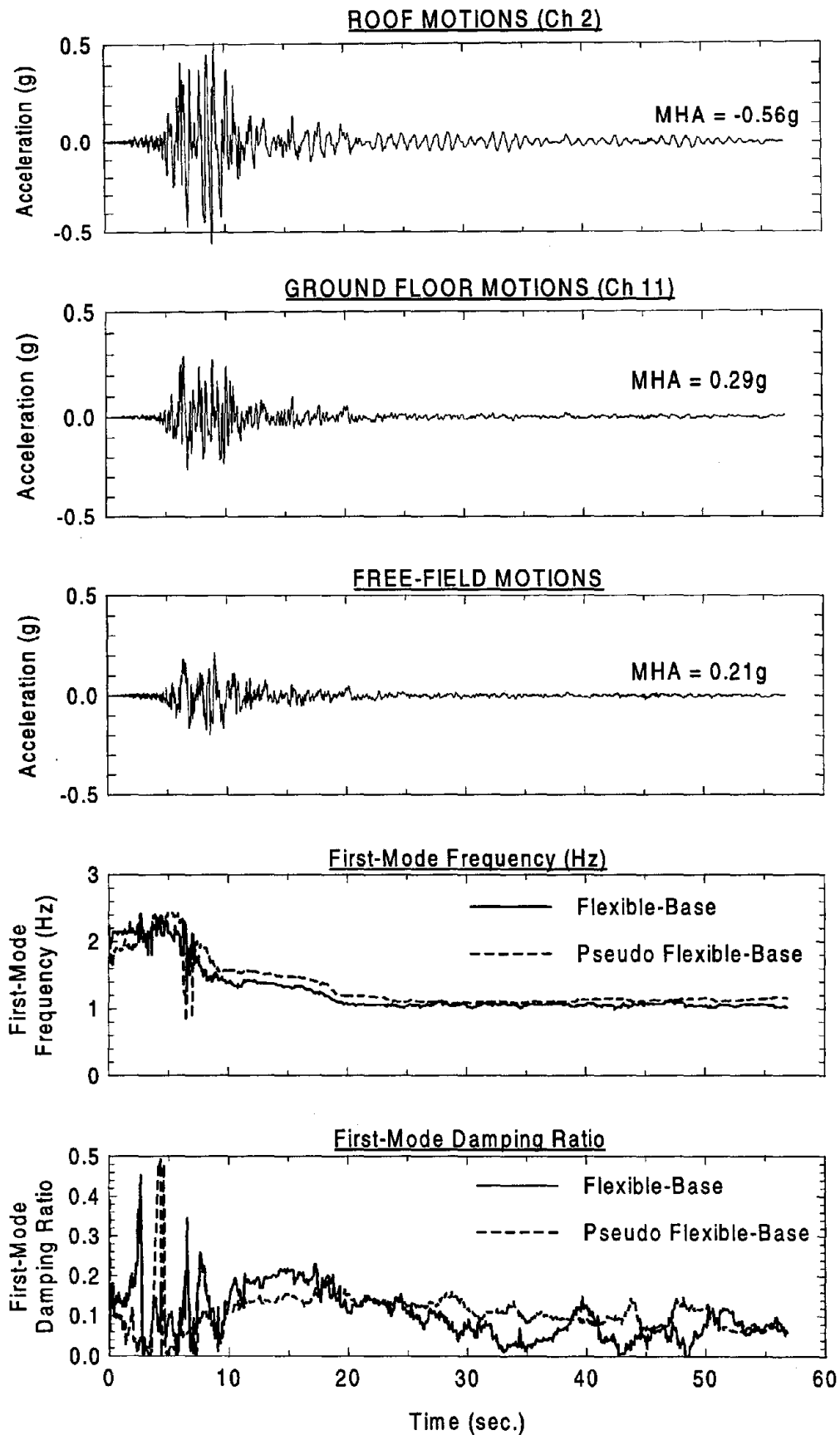
Fig. 5.6: Transverse acceleration time histories and time variation of first-mode parameters, Imperial County Services Building, 1979 Imperial Valley Earthquake
