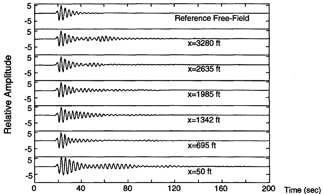
Fig. 4.3: Synthetic seismograms for ground sites and reference free-field; f(\text{bldg})=0.5 Hz, f(\text{site})=0.3 Hz, f(\text{input})=0.25 Hz (Wirgin and Bard, 1996)
