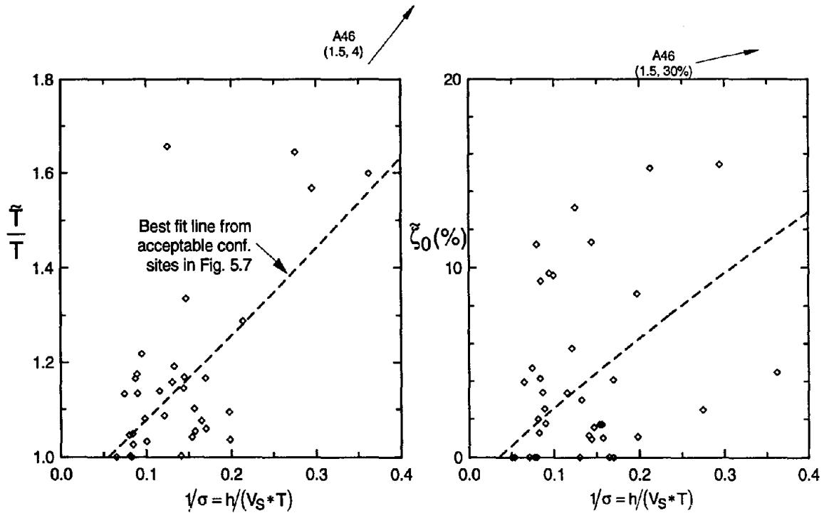
Fig. 5.13: Period lengthening ratios and foundation damping factors for shear wall buildings
