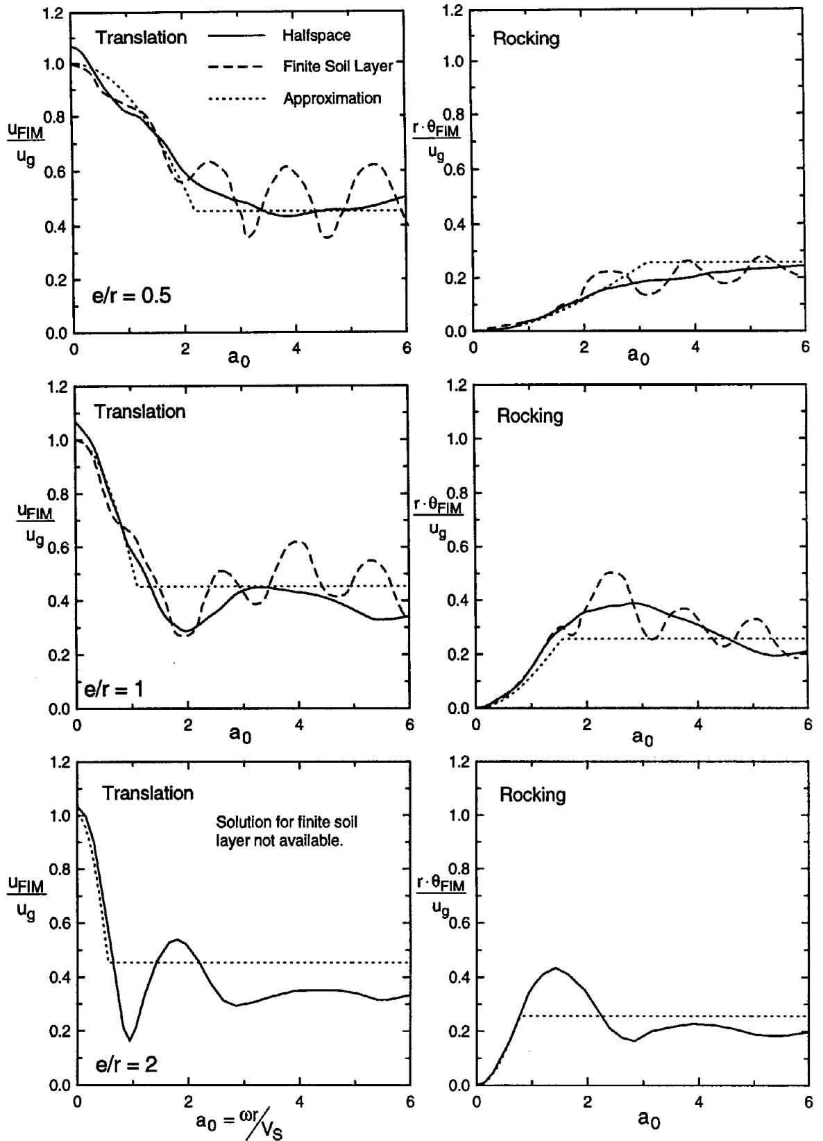
Fig. 2.17: Comparison of transfer function amplitudes for cylinders embedded in a halfspace and finite soil layer and approximation by Elsabee and Morray (Day, 1977 and Elsabee and Morray, 1977)
