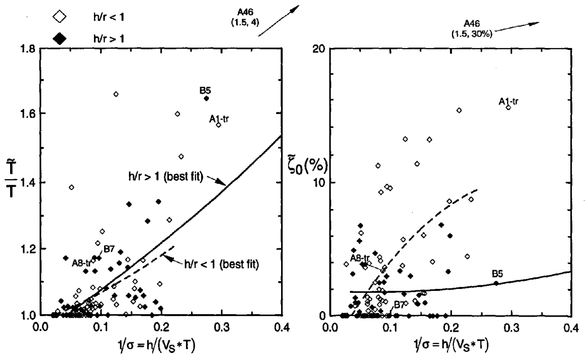
Fig. 5.8: Effect of aspect ratio on period lengthening ratio and foundation damping factor
