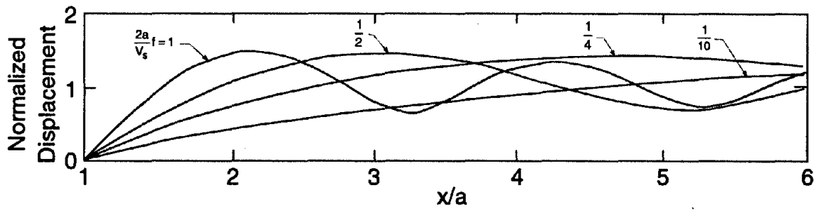
Fig. 4.2: Fourier amplitude of ground surface displacement adjacent to shear wall for vertically incident SH waves (Trifunac, 1972)
