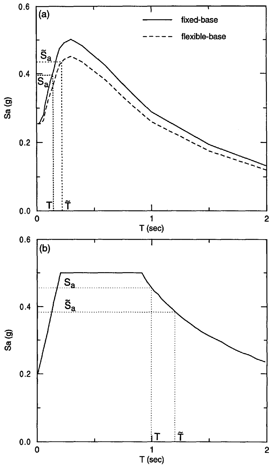
Fig. 6.1: (a) Example of increased spectral acceleration resulting from consideration of inertial interaction effects with smoothed site-specific spectra, and (b) example of reduced spectral acceleration resulting from consideration of inertial interaction effects with code-based spectra with no damping correction
