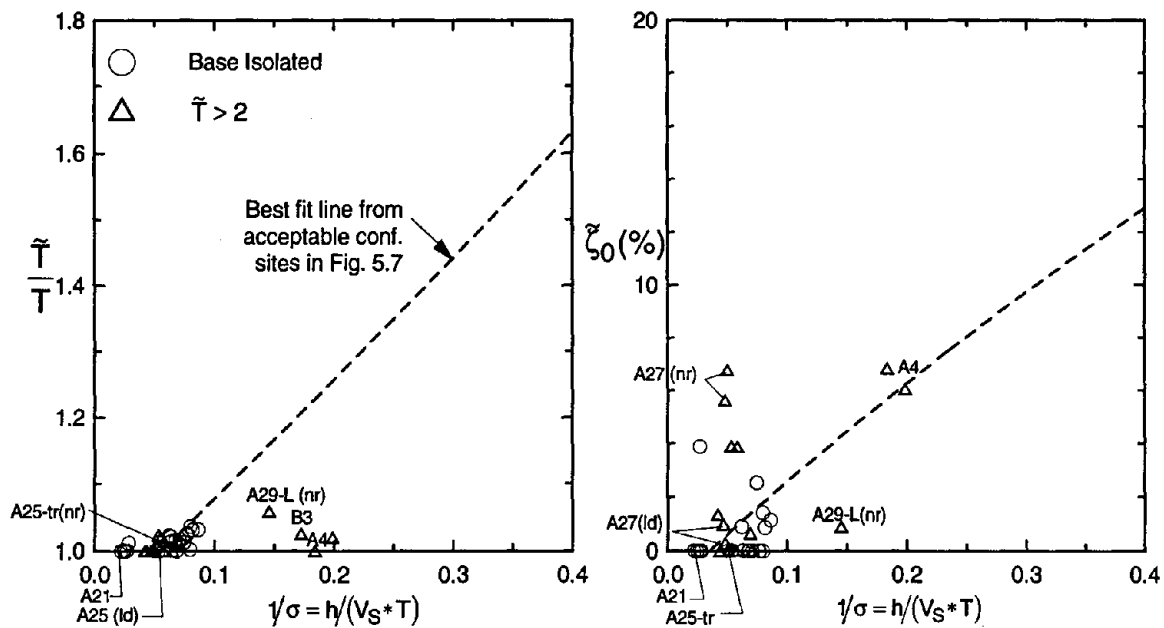
Fig. 5.11: Period lengthening ratios and foundation damping factors for base isolated and long-period structures compared to the best fit line from acceptable confidence sites
