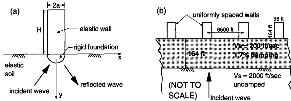
Fig. 4.1: Systems considered by (a) Trifunac (1972) and (b) Wirgin and Bard (1996)
