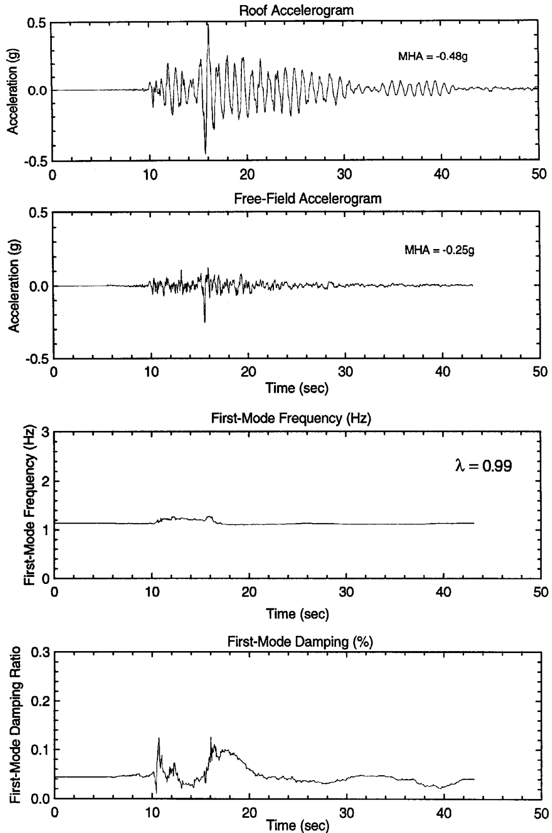
Fig. 3.2: Time variation of first-mode, flexible-base parameters for Site A23, transverse direction, 1994 Northridge Earthquake
