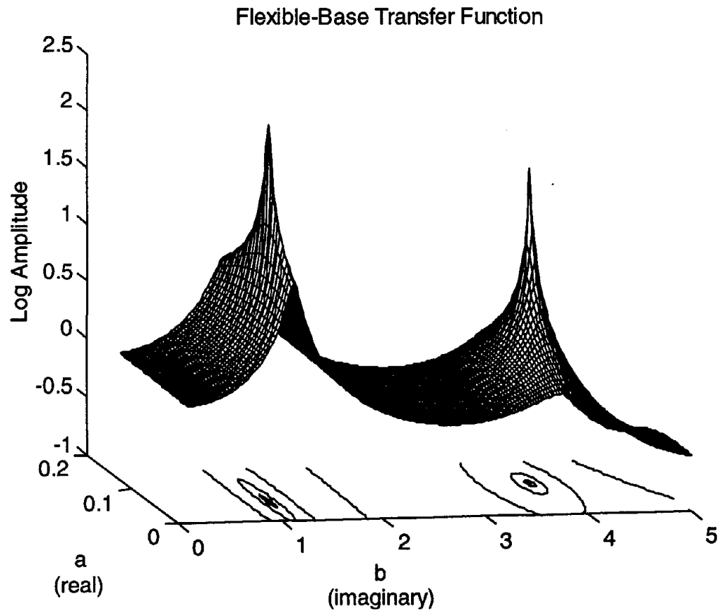
Fig. 3.9: Flexible-base transfer function surface identified by parametric system identification, Site A23, 1994 Northridge earthquake
