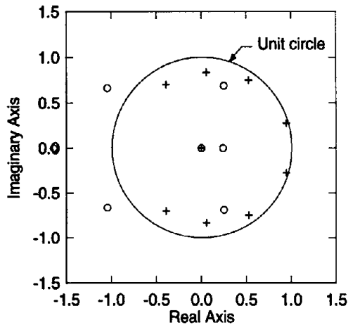
Fig. 3.6: Zeros (o) and poles (+) of the discrete-time transfer function
