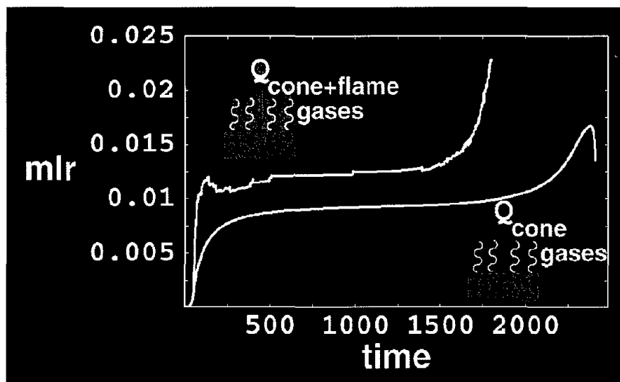
The Cone Calorimeter model is used to calculate the mass loss rate ( \text{kg/m}^2\text{s} ), or \text{mlr} , vs. \text{time(s)} for a burning polypropylene sample (upper plot). Radiative/convective feedback from the flame causes more rapid mass loss rate than for the pyrolyzing sample (lower plot) heated solely by incident radiation of 40 \text{ kW/m}^2 from the Cone heater.
