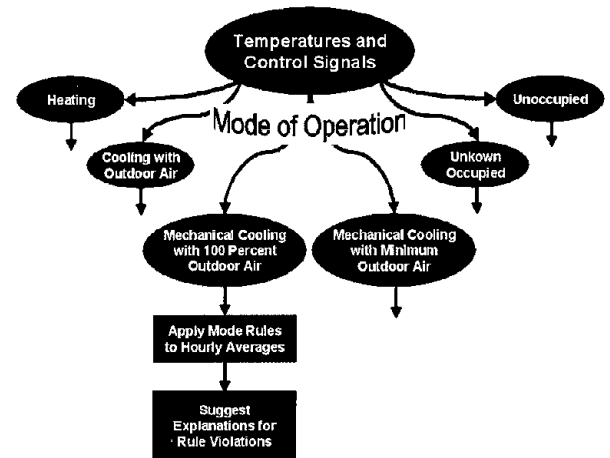
Flow diagram highlighting the main steps in the rule-based fault detection and diagnostic method for air-handling units.
