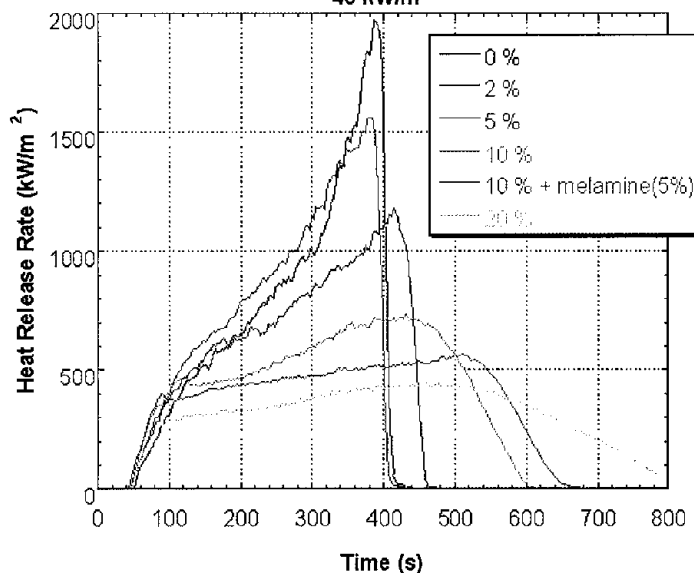
Effects of Silica gel Content on Heat Release Rate of PP 40 kW/m 2
