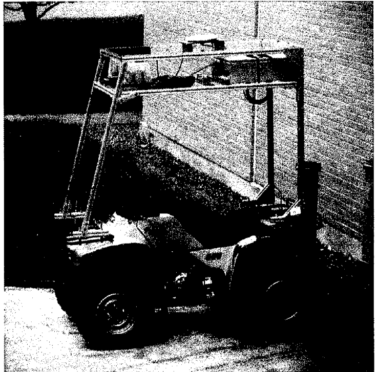
Prototype of the "strap down" construction machinery status system. The position and orientation of the vehicle are relayed to the project database in real-time.
