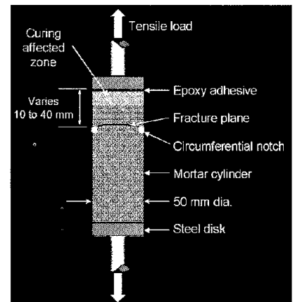
Testing technique to measure the tensile strength as a function of distance from the drying surface.
