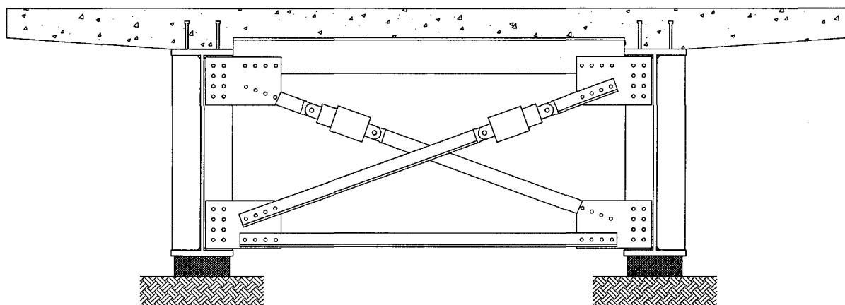
Figure 3.4 Configuration with dampers inserted into existing cross-braces.
