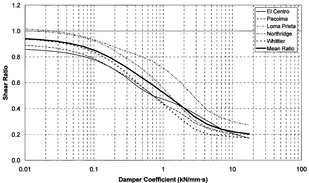
Figure 4.6 Shear connector stress ratio with viscous fluid dampers in chevron braces.
