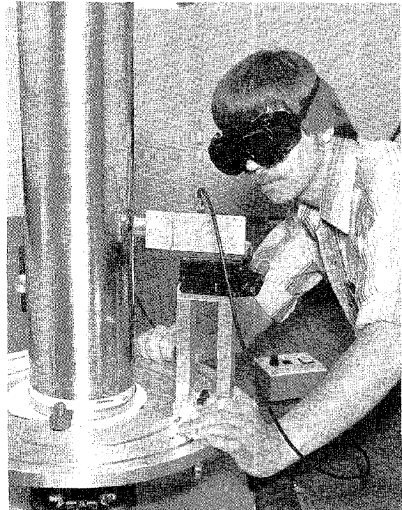
To measure the internal temperature in a steel billet, laboratory assistant Christian Turner combines a piezoelectric detector with a rapidly scanned laser.
