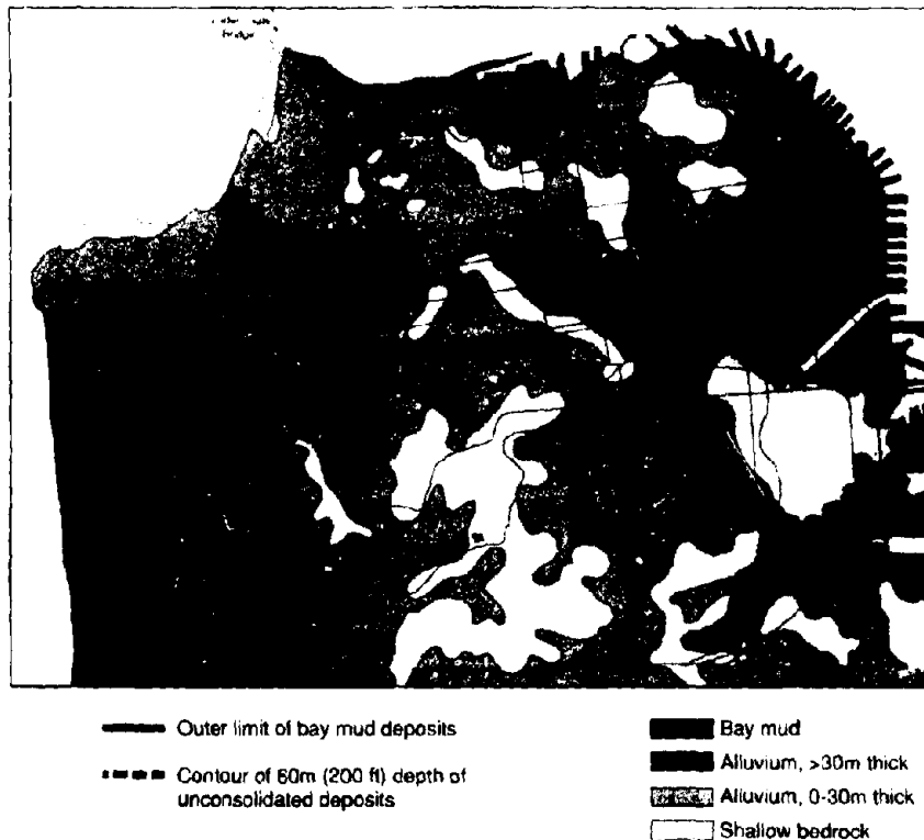
Unstable soil played a major role in the damage of buildings and "lifelines"—bridges, highways, and water and gas pipelines—during the October 1989 Loma Prieta earthquake in the San Francisco Bay area. These figures, from the NIST report, show the surface geology of the area (below) and the correlating damage (right).
