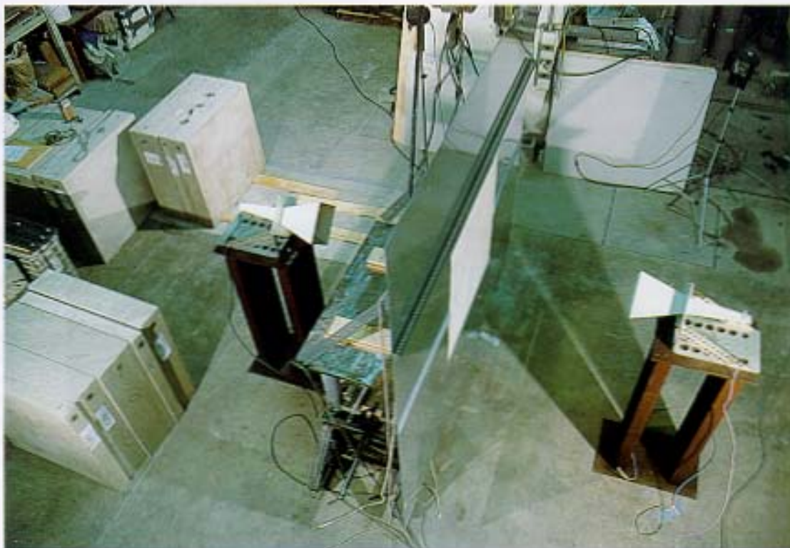
Prototype Non-Line-of-Sight surveying system
