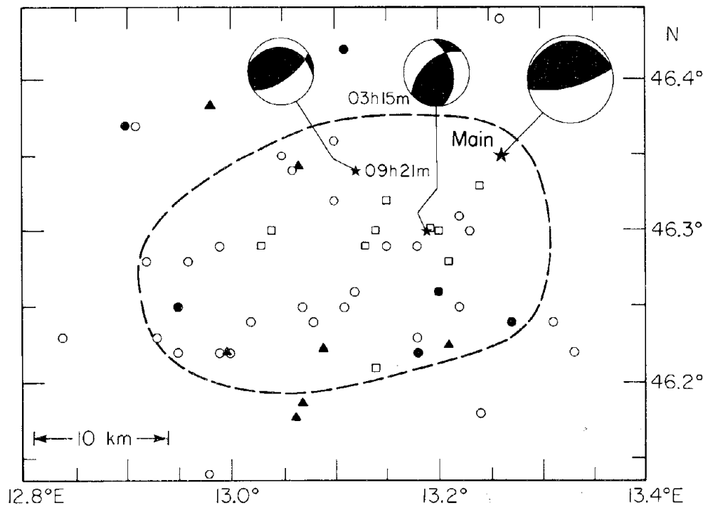
FIG. 2. Epicenters of the main shock and larger aftershocks of the Friuli earthquake sequence as reported by the ISC. Large star indicates the main shock. Closed circles represent aftershocks which occurred within the first 24 hr, and open circles are later aftershocks up to September 11. Smaller stars are epicenters of the two largest earthquakes on September 15. Open squares are aftershocks of these events. Focal mechanisms are determined in this paper with compressional quadrants shaded. Heavy dashed line denotes the approximate limit of aftershock concentration. Triangles are accelerograph stations.
