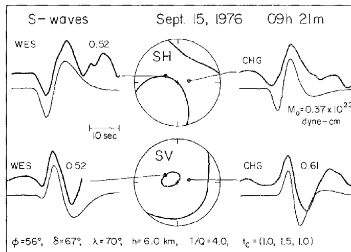
FIG. 11. S waves for the aftershock of 09h 21m showing observed and synthetic records and SH and SV radiation patterns.
