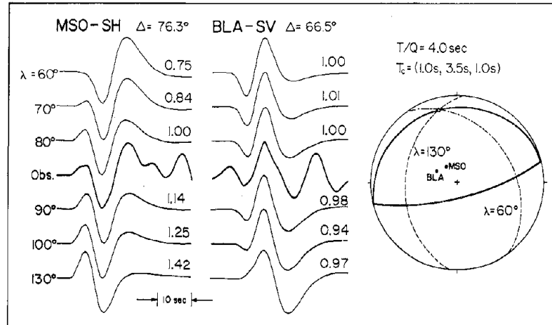
FIG. 6. Determination of shallowly dipping nodal plane using S -wave data. Note variation of SH -wave synthetics at MSO and SV -wave synthetics at BLA with change in rake angle. Best estimate is that the rake angle lies between 80^\circ and 90^\circ , corresponding to almost pure dip-slip fault mechanism.
