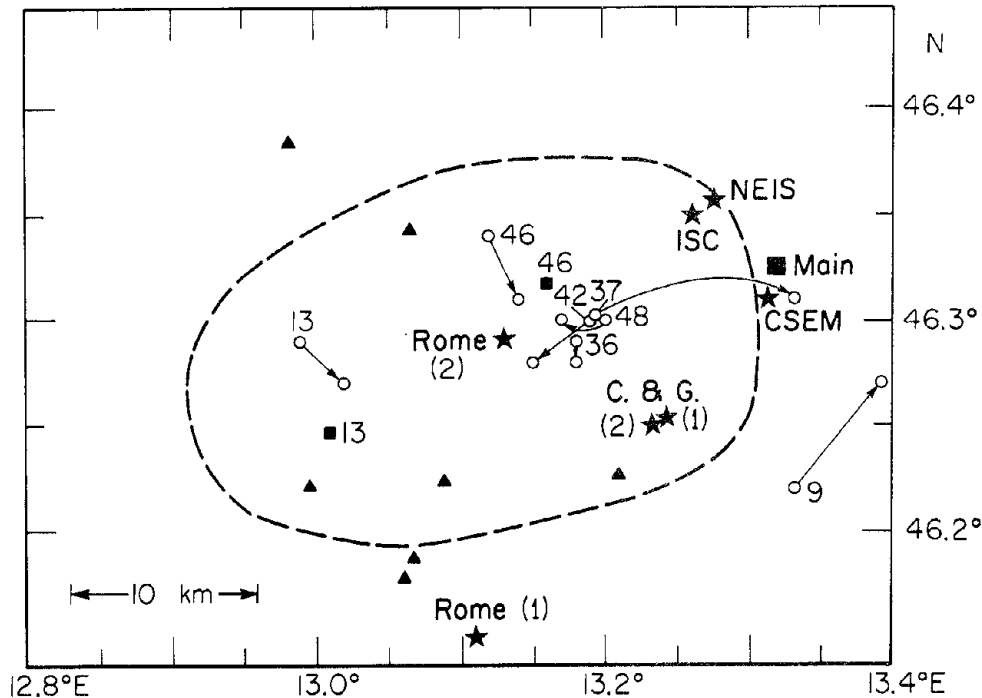
FIG. 3. Locations of the main shock and largest aftershocks. Main shock epicenters determined by various agencies are indicated by stars (Table 2). Aftershock epicenters (numbers correspond to Table 1) calculated by ISC and Rome are indicated by open circles; arrows point from ISC location to Rome location. Filled squares indicate locations of main shock and aftershocks 13 and 46 relative to aftershock 36 determined in this paper.
