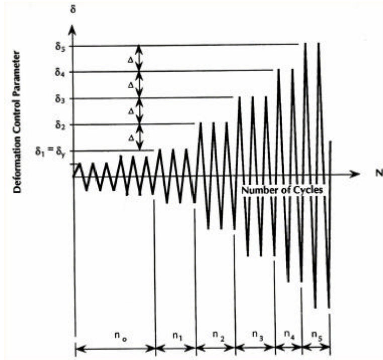
FIGURE 4-1 ATC-24 Displacement History for Cyclic Testing
