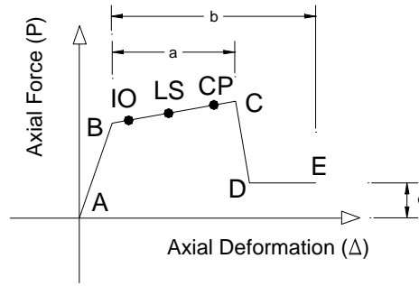
FIGURE 2-3 Axial Force-Axial Deformation Relation and Acceptance Criteria for Braces in Nonlinear Static Procedure, FEMA 356 (2000)
