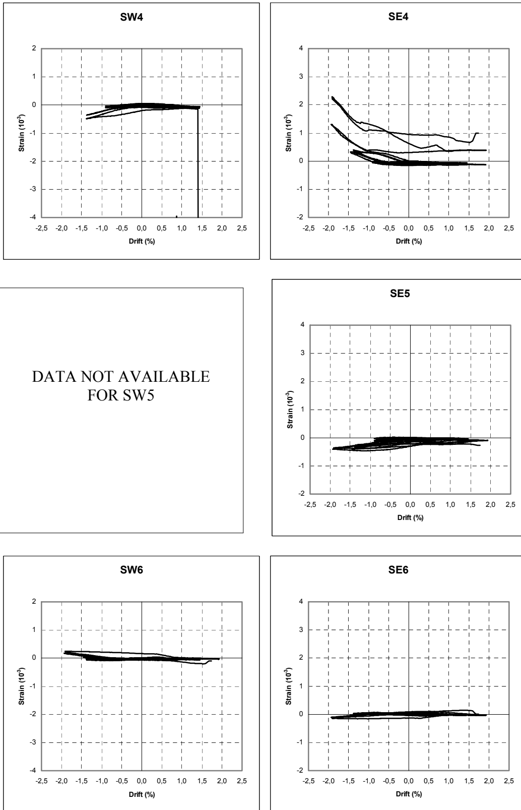
FIGURE C-2 Outer Flange Strain versus Drift Hysteresses for CFSS Members (continued)
