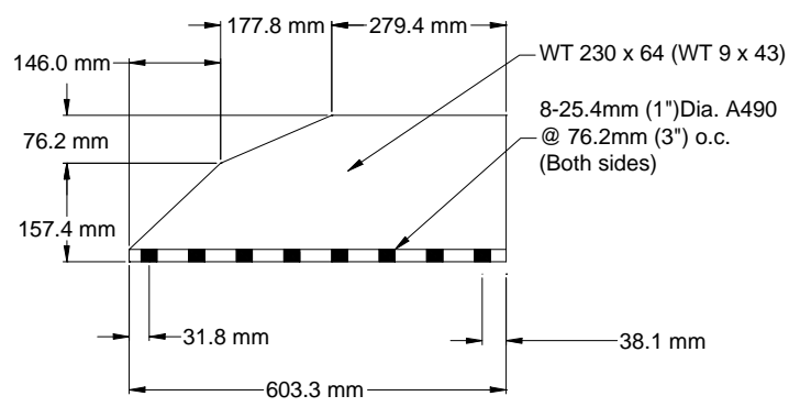
Gusset 2 (For F3 and F4) Quantity: 8
