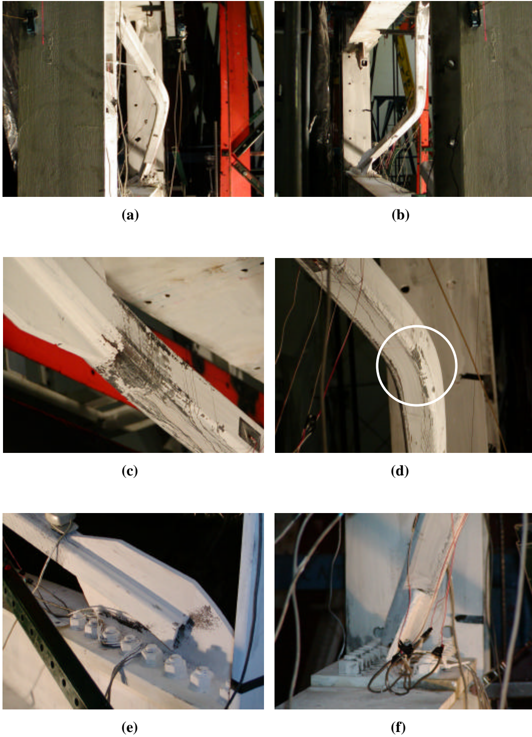
FIGURE 4-13 Damage Level in Specimen F2 at \pm 4d_y : (a,b) General Views (Cycle 16, -4d_y ); (c) Yielding at North Upper Brace-to-Gusset Connection (West View) (Cycle 16, -4d_y ); (d) Development of Out-of-Plane Displacement; (e,f) Severe Out-of-Plane Bending of South Lower Gusset (Cycle 16, -4d_y )
