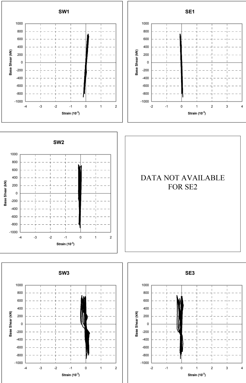
FIGURE E-1 Base Shear versus Outer Flange Strain Hystereses for CFSS Members
