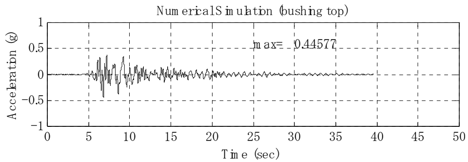
Figure 5-27 Comparison of Test Results and Numerical Simulation: RB/Kobe/x375
