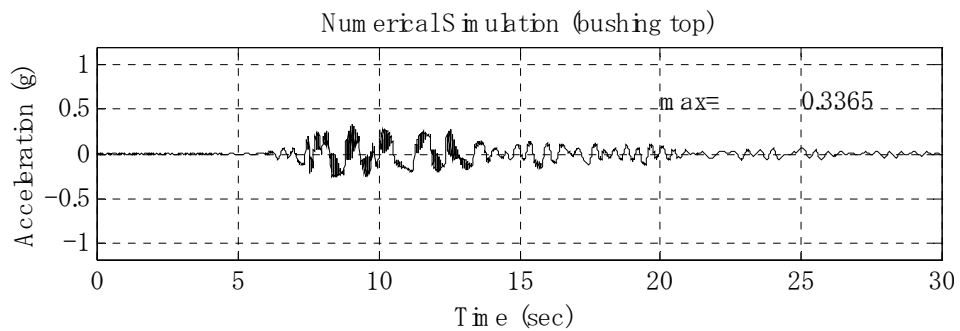
Figure 5-6 Comparison of Test Results and Numerical Simulation: 161kV/B/Kobe/x375, Base-Isolated System
