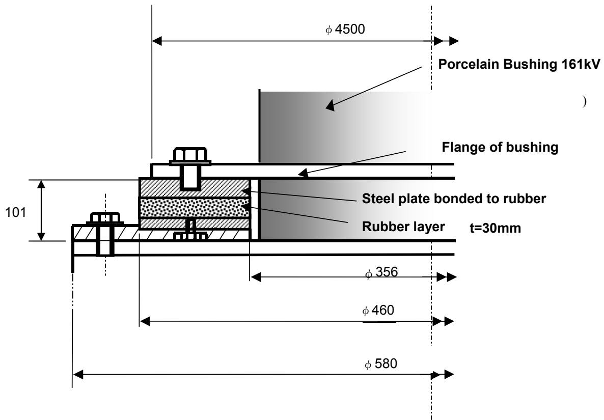
Figure 4-3 Flexible Rubber Ring
