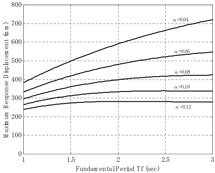
Figure 2-15 Relationship of Fundamental Period and Response Displacement
