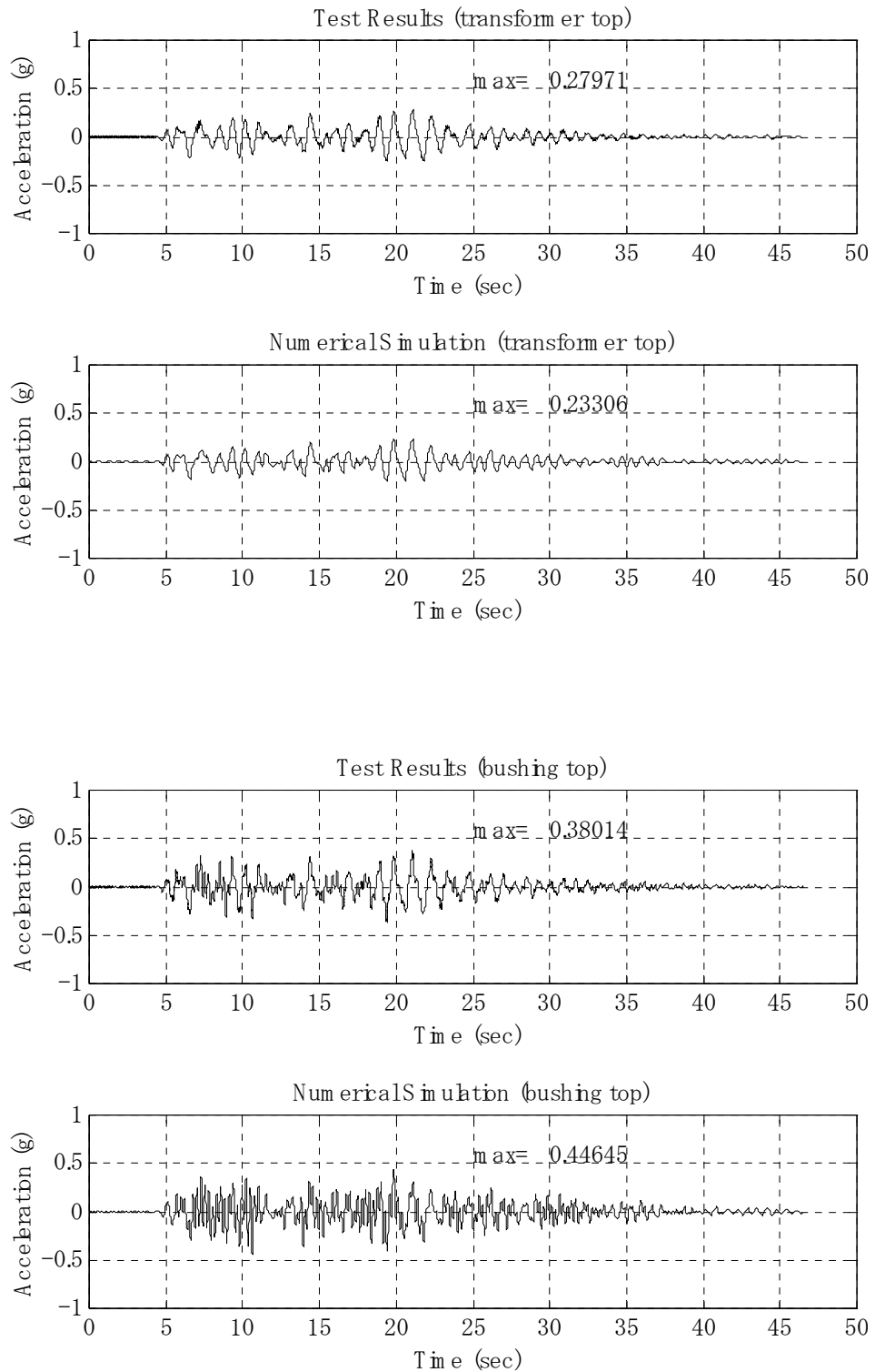
Figure 5-30 Comparison of Test Results and Numerical Simulation in RB/Art-693/xy375, x-dir.
