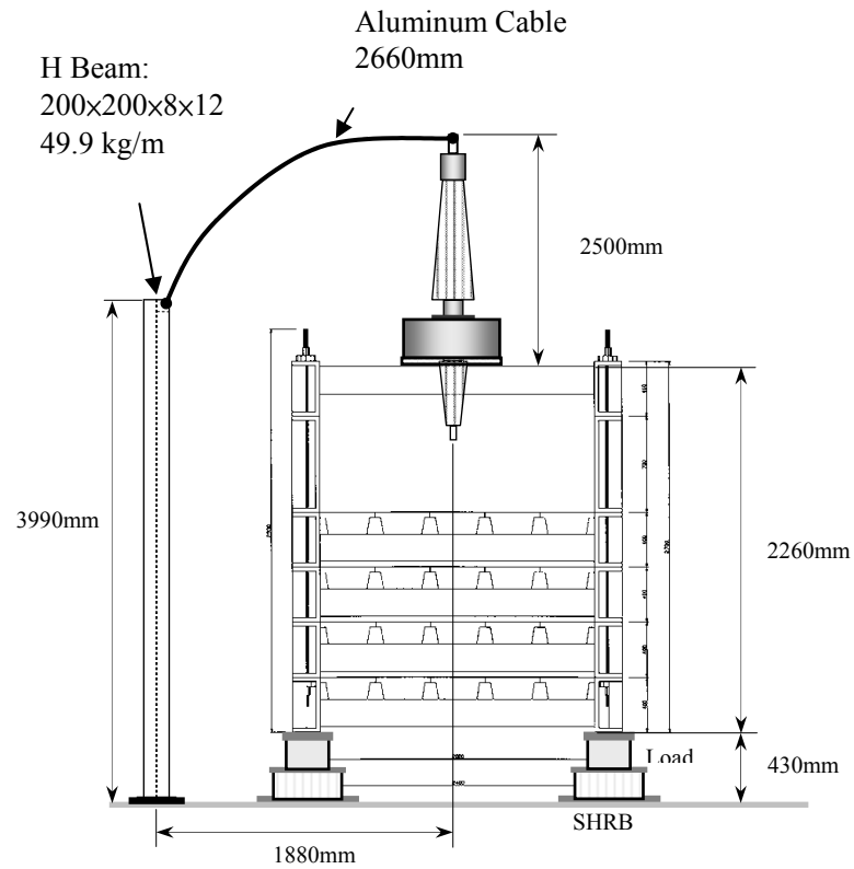
Figure A-2 Geometry of the Test Setup
