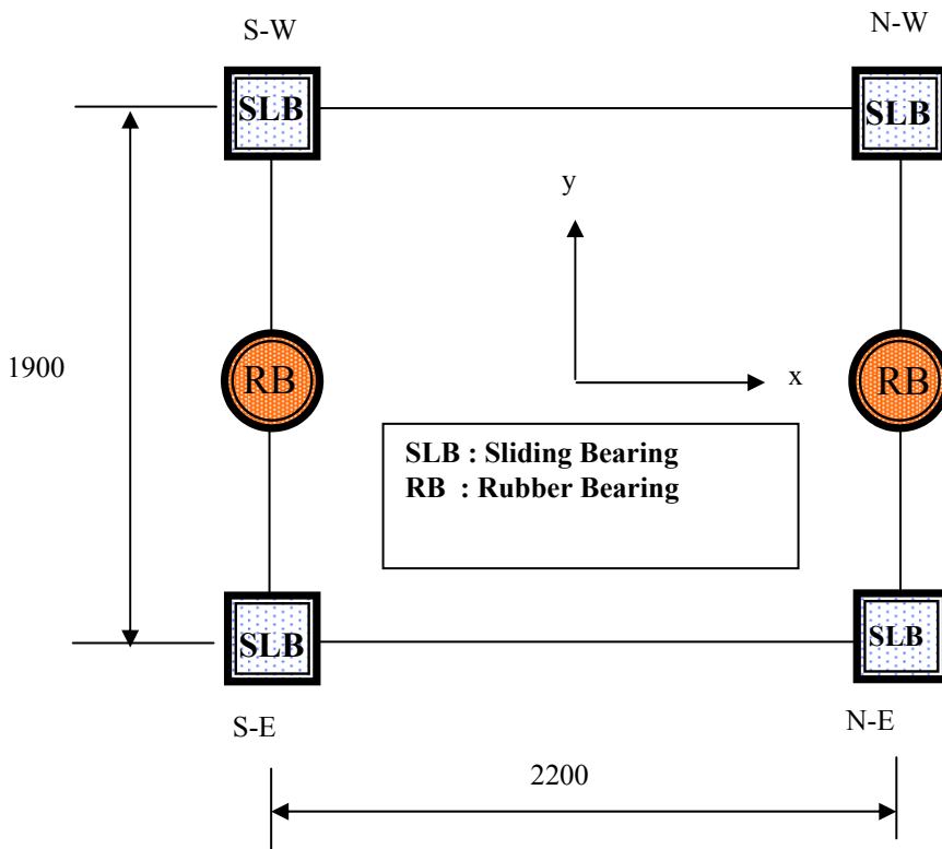
Figure 3-3 Layouts of Sliding Bearings and Rubber Bearings
