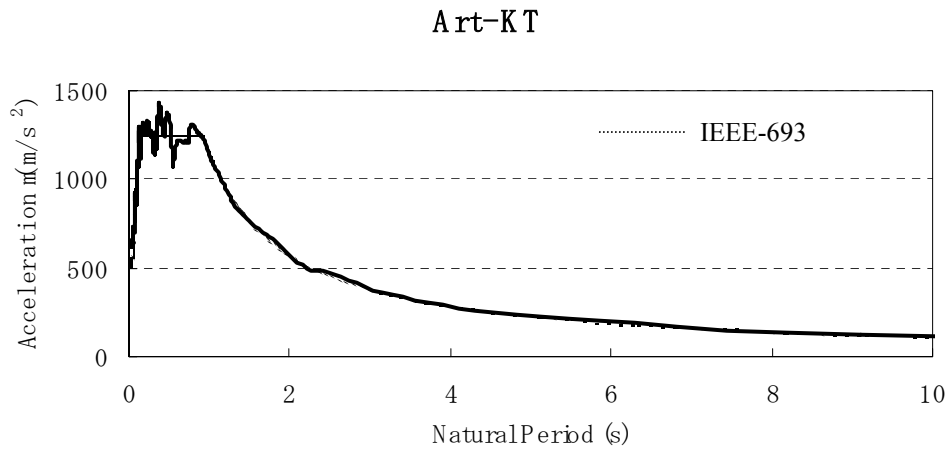
Figure 2-16 Response Spectrum of Artificial Wave: Art-R1, Art-KT, and Art-NY
