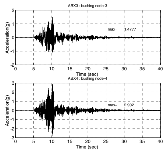
Figure 3-11 Time History of Bushing Response Acceleration:
