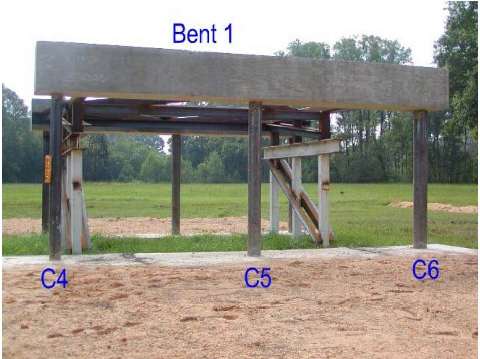
Figure 4-18 Test Setup from Bent 1 Front
