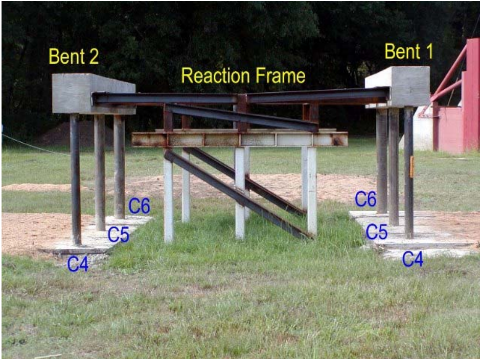
Figure 4-17 Test Setup from Side View
