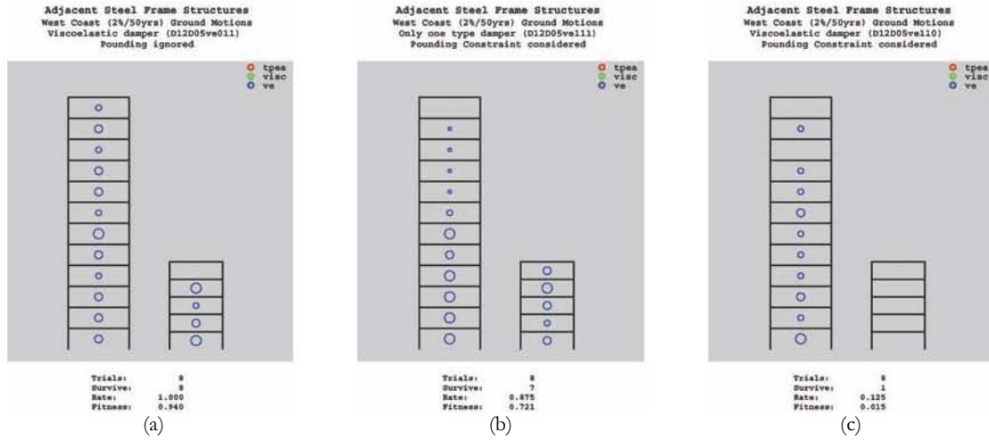
Figure 3. Twelve-story and five-story steel frames with viscoelastic dampers - robust designs with pounding (a) ignored (b) considered (c) considered but only Building A retrofitted
