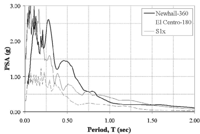
Figure 2. Target Pseudo-Spectral Acceleration Spectra for 3 Seismic Inputs
