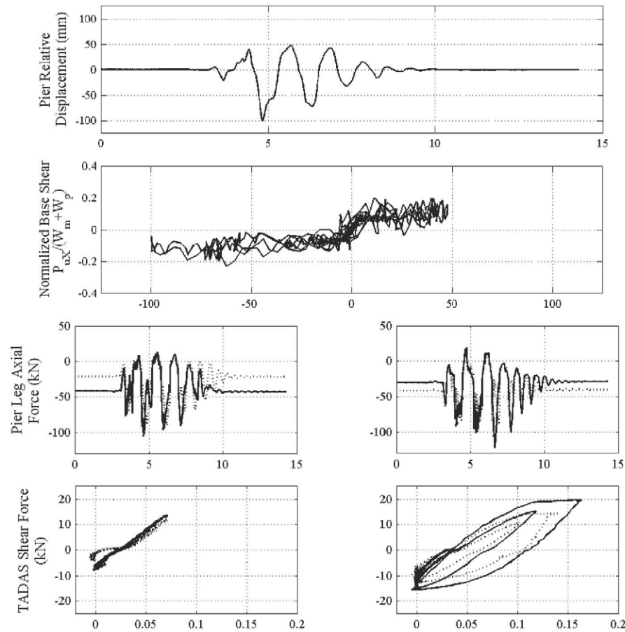
Figure 3. Experimental Testing Results ( \theta=0\text{deg.} , \eta_L=0.67 , Syn-150%)
