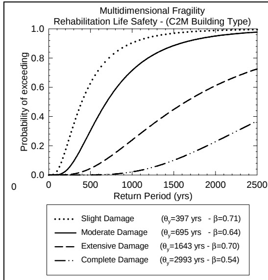
Figure 3. Multidimensional fragility curves for C2M type structure -Rehabilitation to Life Safety
