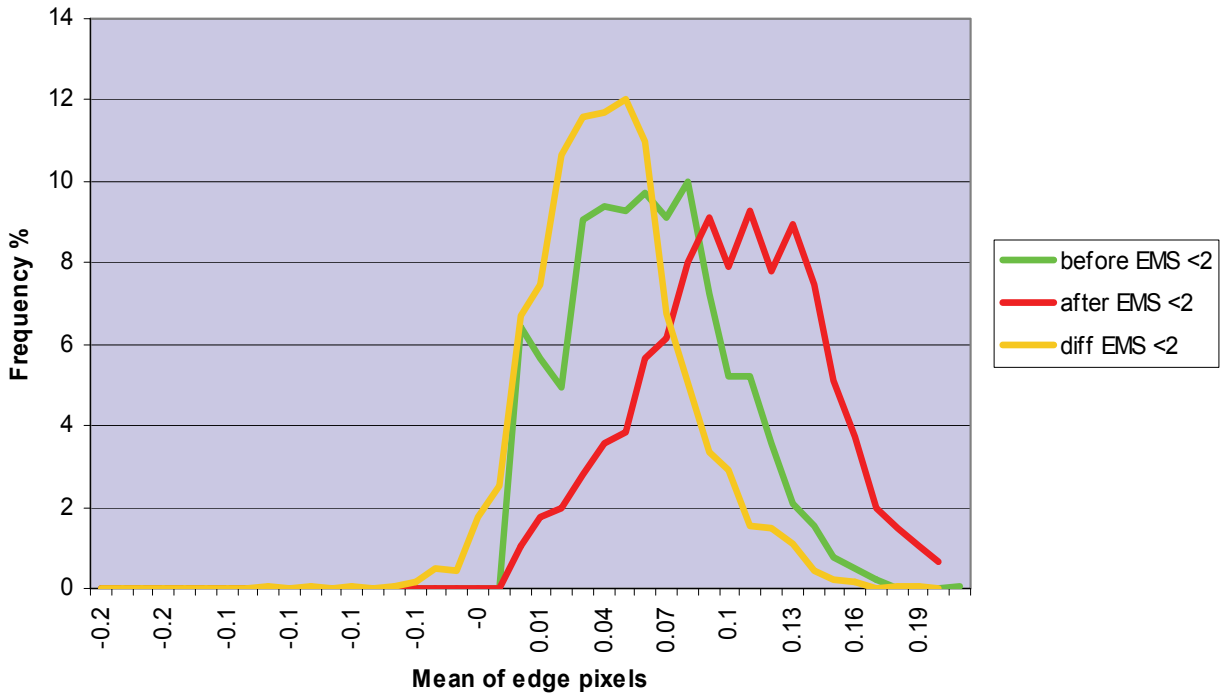
Figure 5-5 Variation in the Frequency of Edge Pixels Occurring within Buildings Classified as EMS98 Level 5 (Destruction) and Level 2 (Moderate Damage) for Non-Damaged (Before) and Damaged (After) Scenarios. The Difference Between the Before and After Results is also Shown.
