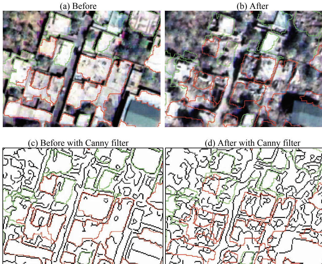
Figure 5-2 (a) Before Event Image; (b) After Event Image; c) 17x17 Canny Filtered Before Image; and d) 17x17 Canny Filtered After Image. Building Outlines are Superimposed, with Non-Collapsed in Green and Collapsed in Red.
