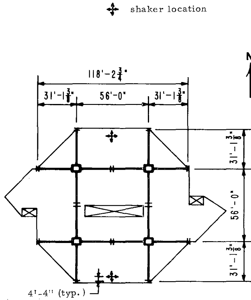
Figure 5.8 Typical tower floor plan with the location of the shakers indicated for the roof.
