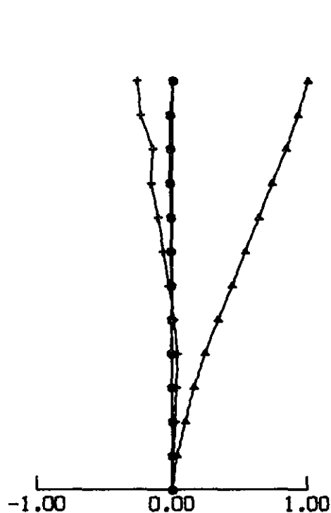
MODE 3 0.410 HZ.
