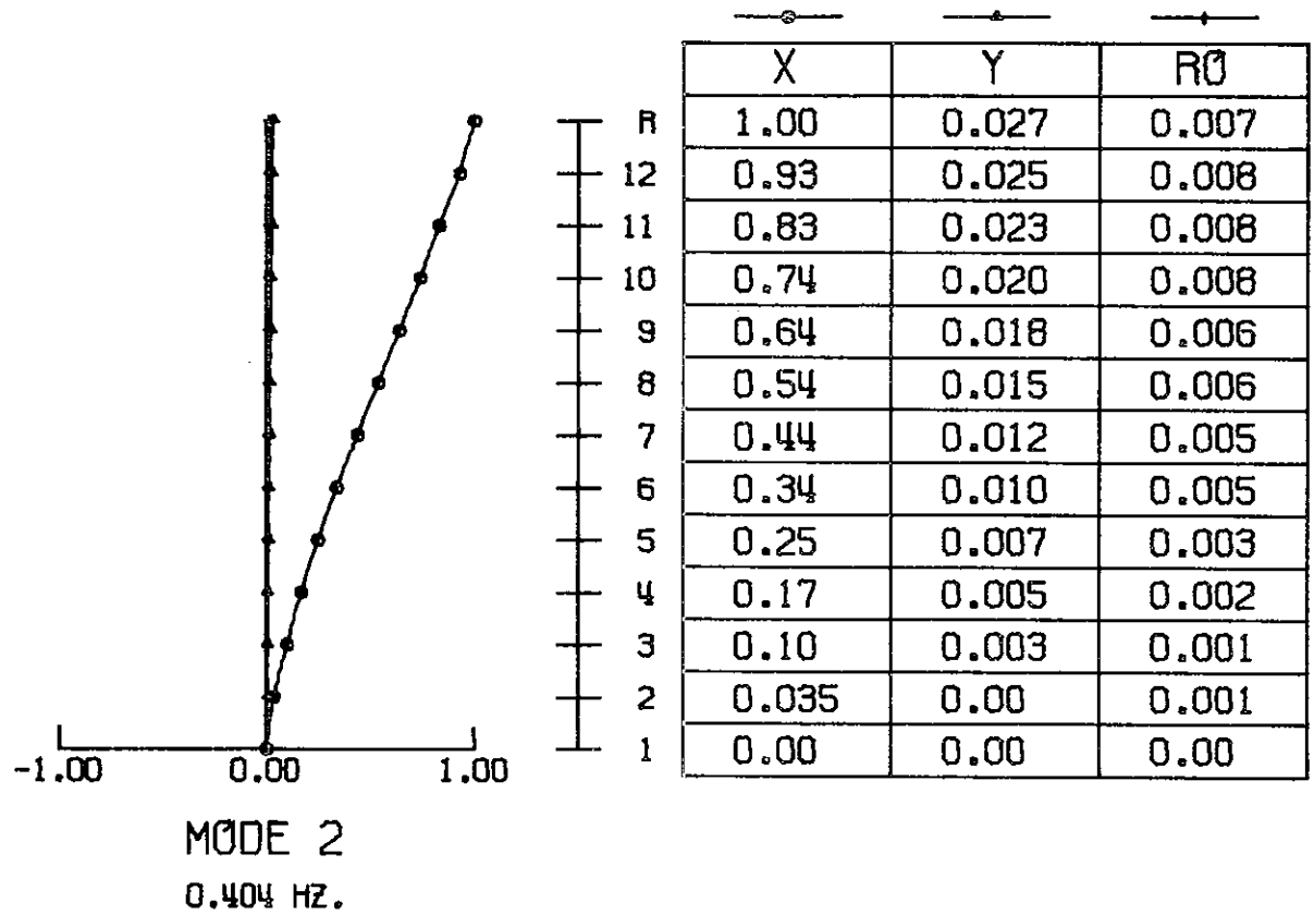
Figure 6.3 Computed mode shapes and frequencies of the Parsons building.
