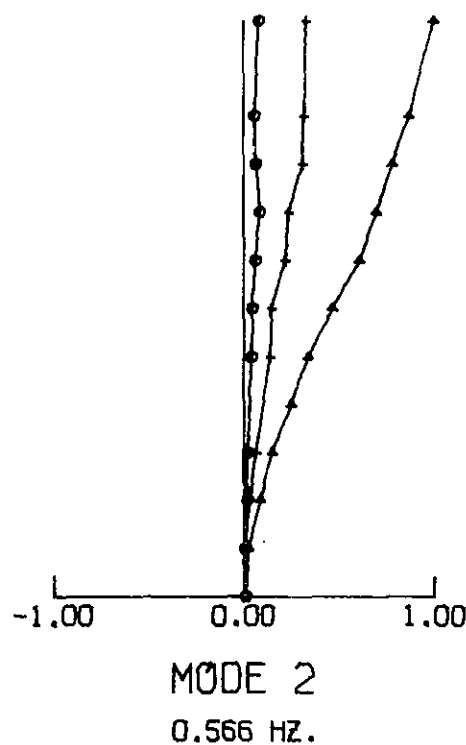
Figure 5.13 Natural frequencies and mode shapes of the Parsons building.
