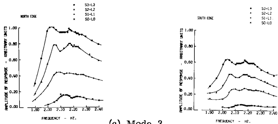
(c) Mode 3
