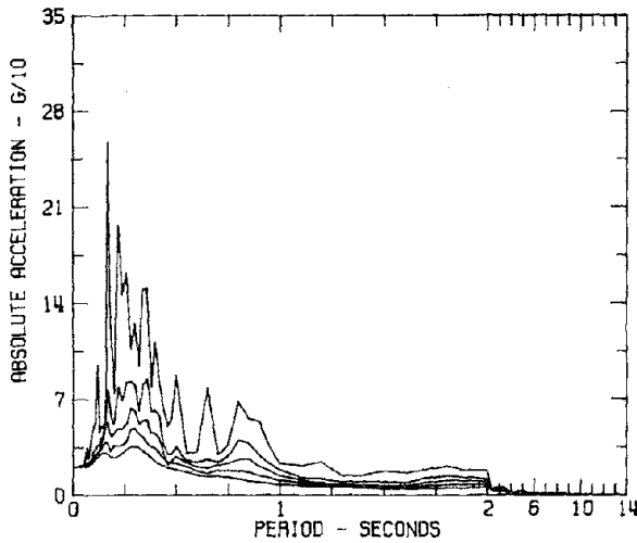
RESPONSE SPECTRA IIIG108 COMP N00E SAN FERNANDO EARTHQUAKE FEB 9, 1971 - 0600 PST CALTECH MILLIKAN LIBRARY, BASEMENT, PASADENA, CAL. DAMPING VALUES ARE 0, 2, 5, 10 AND 20 PERCENT OF CRITICAL
