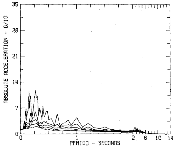
RESPONSE SPECTRA IIC054 COMP S38W SAN FERNANDO EARTHQUAKE FEB 9, 1971 - 0600 PST 445 FIGUEROA STREET, SUB-BASEMENT, LOS ANGELES, CAL. DAMPING VALUES ARE 0, 2, 5, 10 AND 20 PERCENT OF CRITICAL
