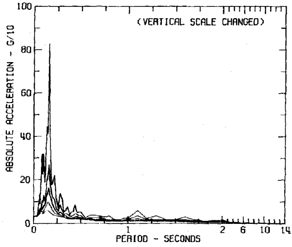
RESPONSE SPECTRA IIIZ001 COMP DOWN MANAGUA EARTHQUAKE DEC 23, 1972 - 0629 GMT MANAGUA, NICARAGUA DAMPING VALUES ARE 0, 2, 5, 10 AND 20 PERCENT OF CRITICAL
