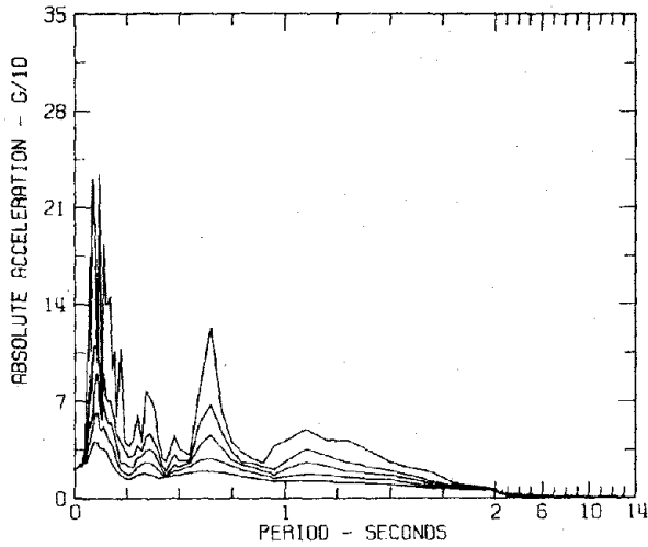
RESPONSE SPECTRA IIIB033 COMP DOWN PARKFIELD, CALIFORNIA EARTHQUAKE JUNE 27, 1966 - 2026 PST CHOLAME, SHANDON, CALIFORNIA ARRAY NO. 2 DAMPING VALUES ARE 0, 2, 5, 10 AND 20 PERCENT OF CRITICAL
