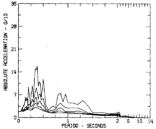
RESPONSE SPECTRA IIIG108 COMP N90E SAN FERNANDO EARTHQUAKE FEB 9, 1971 - 0600 PST CALTECH MILLIKAN LIBRARY, BASEMENT, PASADENA, CAL. DAMPING VALUES ARE 0, 2, 5, 10 AND 20 PERCENT OF CRITICAL
