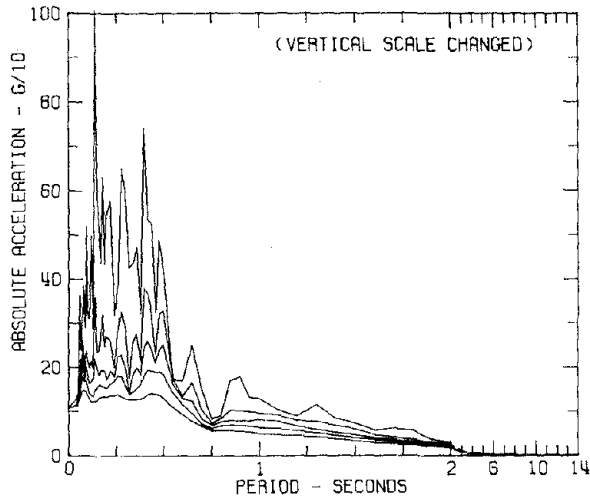
RESPONSE SPECTRA I11C041 COMP S74W SAN FERNANDO EARTHQUAKE FEB 9, 1971 - 0600 PST PACIFICA DAM, CAL. DAMPING VALUES ARE 0, 2, 5, 10 AND 20 PERCENT OF CRITICAL
