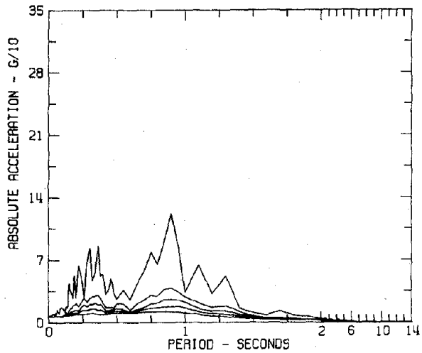
RESPONSE SPECTRA IIIB028 COMP S02W WESTERN WASHINGTON EARTHQUAKE APR 13, 1949 - 1156 PST SEATTLE, WASH. DIST ENGAS OFFC AT ARMY BASE DAMPING VALUES ARE 0, 2, 5, 10 AND 20 PERCENT OF CRITICAL
