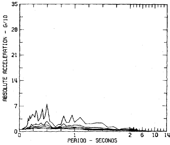
RESPONSE SPECTRA IIIA006 COMP 500W KERN COUNTY, CALIFORNIA EARTHQUAKE JULY 21, 1952 - 0453 PDT HOLLYWOOD STORAGE BASEMENT DAMPING VALUES ARE 0, 2, 5, 10 AND 20 PERCENT OF CRITICAL
