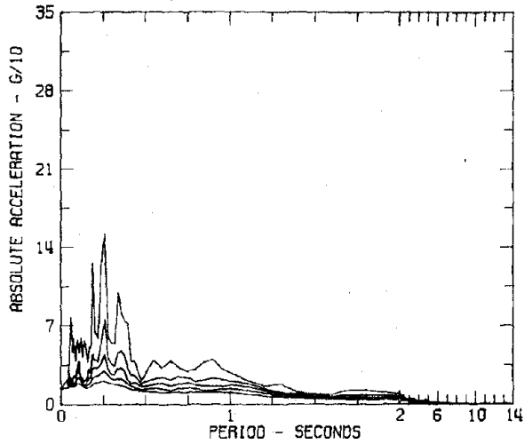
RESPONSE SPECTRA IIIG110 COMP S08W SAN FERNANDO EARTHQUAKE FEB 9, 1971 - 0600 PST JET PROPULSION LAB., BASEMENT, PASADENA, CAL. DAMPING VALUES ARE 0, 2, 5, 10 AND 20 PERCENT OF CRITICAL
