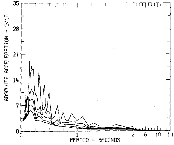
RESPONSE SPECTRA IIB035 COMP N40W PARKFIELD, CALIFORNIA EARTHQUAKE JUNE 27, 1966 - 2026 PST CHOLAME, SHANDON, CALIFORNIA ARRAY NO. 8 DAMPING VALUES ARE 0, 2, 5, 10 AND 20 PERCENT OF CRITICAL
