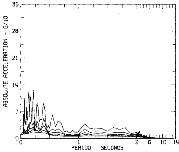
RESPONSE SPECTRA IIIH115 COMP DOWN SAN FERNANDO EARTHQUAKE FEB 9, 1971 - 0600 PST 15250 VENTURA BLVD., BASEMENT, LOS ANGELES, CAL. DAMPING VALUES ARE 0, 2, 5, 10 AND 20 PERCENT OF CRITICAL
