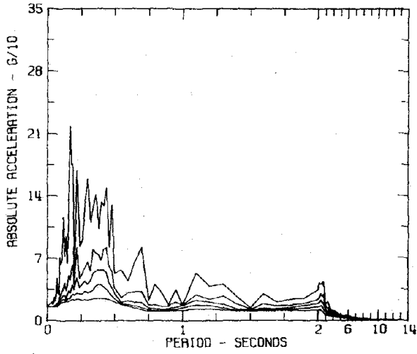
RESPONSE SPECTRA IIIH115 COMP N79W SAN FERNANDO EARTHQUAKE FEB 9, 1971 - 0600 PST 15250 VENTURA BLVD., BASEMENT, LOS ANGELES, CAL. DAMPING VALUES ARE 0, 2, 5, 10 AND 20 PERCENT OF CRITICAL
