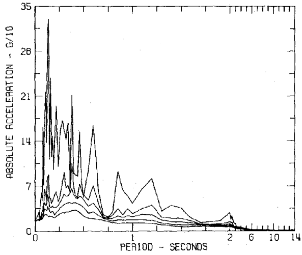
RESPONSE SPECTRA IIIB029 COMP N04W WESTERN WASHINGTON EARTHQUAKE APR 13, 1949 - 1156 PST OLYMPIA, WASHINGTON HWY TEST LAB DAMPING VALUES ARE 0, 2, 5, 10 AND 20 PERCENT OF CRITICAL
