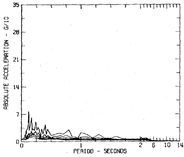
RESPONSE SPECTRA IIIC054 COMP DOWN SAN FERNANDO EARTHQUAKE FEB 9, 1971 - 0600 PST 445 FIGUEROA STREET, SUB-BASEMENT, LOS ANGELES, CAL. DAMPING VALUES ARE 0, 2, 5, 10 AND 20 PERCENT OF CRITICAL
