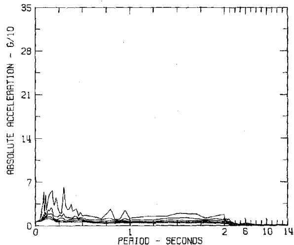
RESPONSE SPECTRA IIIB036 COMP N40W PARKFIELD, CALIFORNIA EARTHQUAKE JUNE 27, 1966 - 2026 PST CHOLAME, SHANDON, CALIFORNIA ARRAY NO. 12 DAMPING VALUES ARE 0, 2, 5, 10 AND 20 PERCENT OF CRITICAL
