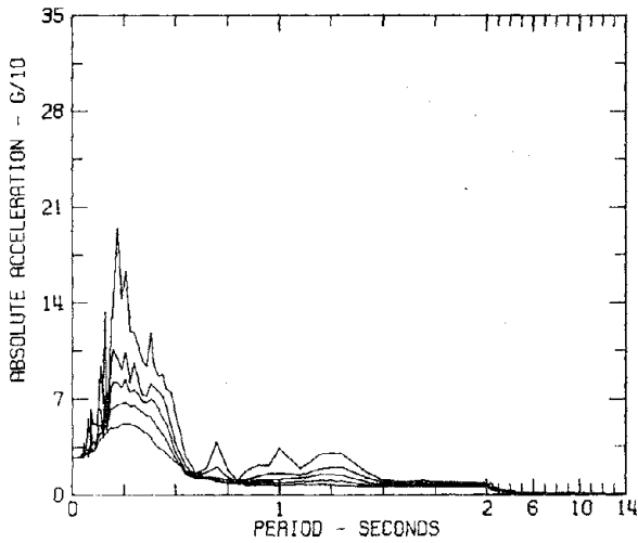
RESPONSE SPECTRA IIIB037 COMP N65W PARKFIELD, CALIFORNIA EARTHQUAKE JUNE 27, 1966 - 2026 PST TEMBLOR, CALIFORNIA NO. 2 DAMPING VALUES ARE 0, 2, 5, 10 AND 20 PERCENT OF CRITICAL
