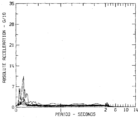
RESPONSE SPECTRA IIIB036 COMP DOWN PARKFIELD, CALIFORNIA EARTHQUAKE JUNE 27, 1966 - 2026 PST CHOLAME, SHANDON, CALIFORNIA ARRAY NO. 12 DAMPING VALUES ARE 0, 2, 5, 10 AND 20 PERCENT OF CRITICAL
