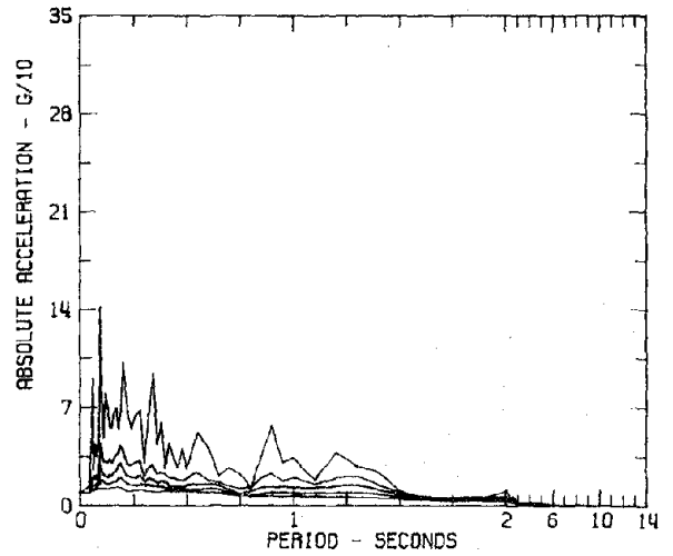
RESPONSE SPECTRA IIIG114 COMP DOWN SAN FERNANDO EARTHQUAKE FEB 9, 1971 - 0600 PST PALMDALE FIRE STATION, STORAGE ROOM, PALMDALE, CAL. DAMPING VALUES ARE 0, 2, 5, 10 AND 20 PERCENT OF CRITICAL
