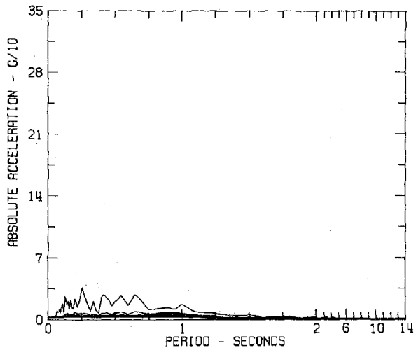
RESPONSE SPECTRA IIIB028 COMP VERT WESTERN WASHINGTON EARTHQUAKE APR 13, 1949 - 1156 PST SEATTLE, WASH. DIST ENGAS OFFC AT ARMY BASE DAMPING VALUES ARE 0, 2, 5, 10 AND 20 PERCENT OF CRITICAL
