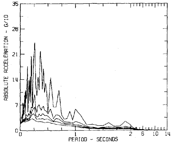
RESPONSE SPECTRA IIIB024 COMP S90W LOWER CALIFORNIA EARTHQUAKE DEC 30, 1934 - 0552 PST EL CENTRO IMPERIAL VALLEY DAMPING VALUES ARE 0, 2, 5, 10 AND 20 PERCENT OF CRITICAL
