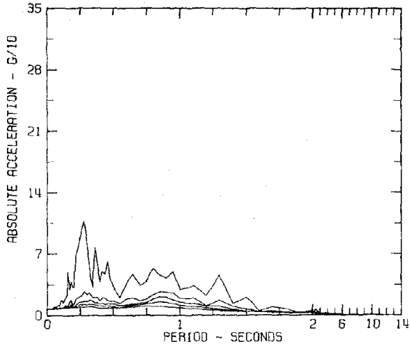
RESPONSE SPECTRA IIIB028 COMP N88W WESTERN WASHINGTON EARTHQUAKE APR 13, 1949 - 1156 PST SEATTLE, WASH. DIST ENGRS OFFC AT ARMY BASE DAMPING VALUES ARE 0, 2, 5, 10 AND 20 PERCENT OF CRITICAL
