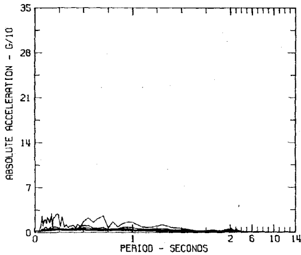
RESPONSE SPECTRA IIIA007 COMP VERT KERN COUNTY, CALIFORNIA EARTHQUAKE JULY 21, 1952 - 0453 PDT HOLLYWOOD STORAGE P.E. LOT DAMPING VALUES ARE 0, 2, 5, 10 AND 20 PERCENT OF CRITICAL
