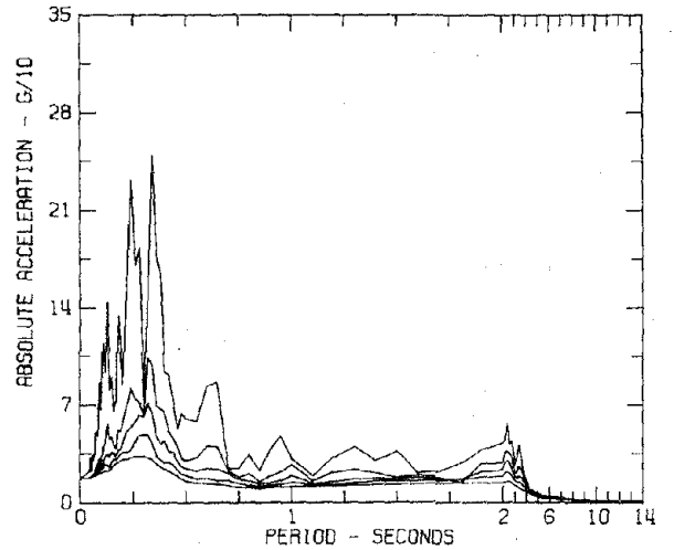
RESPONSE SPECTRA I11C048 COMP DOWN SAN FERNANDO EARTHQUAKE FEB 9, 1971 - 0600 PST 8244 ORION BLVD. 1ST FLOOR, LOS ANGELES, CAL. DAMPING VALUES ARE 0, 2, 5, 10 AND 20 PERCENT OF CRITICAL
