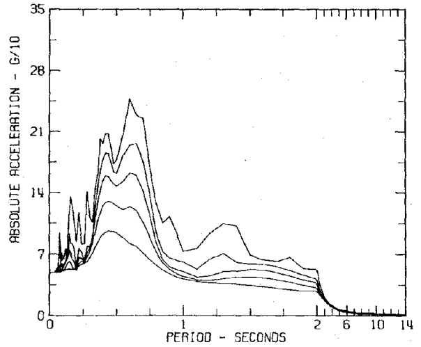
RESPONSE SPECTRA IIIB033 COMP N65E PARKFIELD, CALIFORNIA EARTHQUAKE JUNE 27, 1966 - 2026 PST CHOLAME, SHANDON, CALIFORNIA ARRAY NO. 2 DAMPING VALUES ARE 0, 2, 5, 10 AND 20 PERCENT OF CRITICAL
