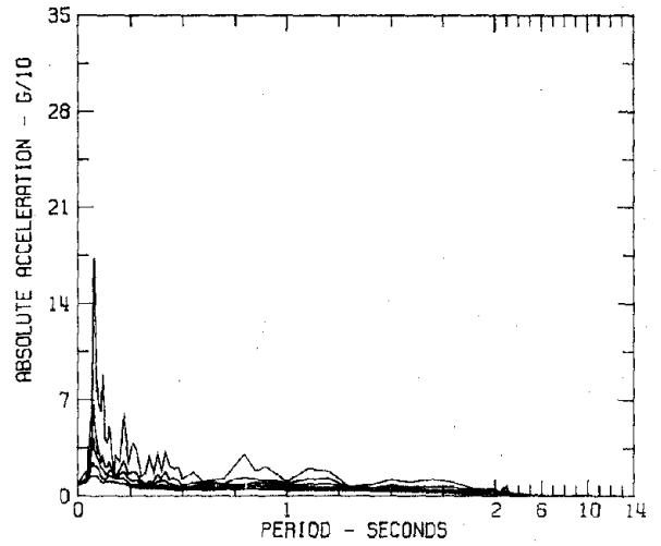
RESPONSE SPECTRA IIB035 PARKFIELD, CALIFORNIA EARTHQUAKE JUNE 27, 1966 - 2026 PST CHOLAME, SHANDON, CALIFORNIA ARRAY NO. 8 DAMPING VALUES ARE 0, 2, 5, 10 AND 20 PERCENT OF CRITICAL
