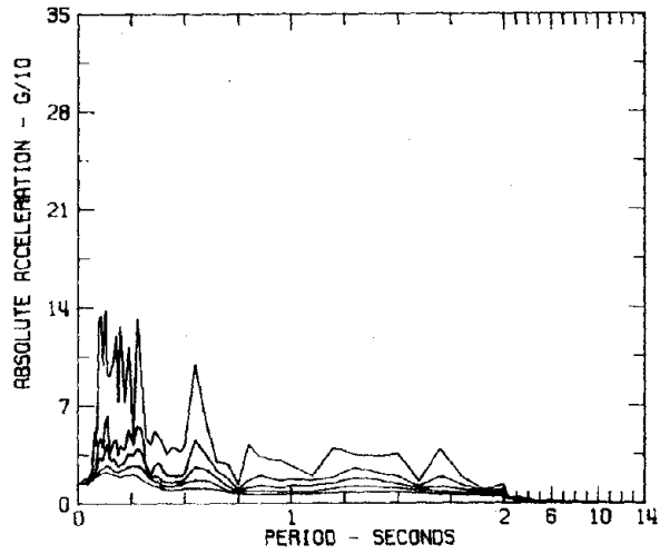
RESPONSE SPECTRA IIIG114 COMP S30W SAN FERNANDO EARTHQUAKE FEB 9, 1971 - 0600 PST PALMDALE FIRE STATION, STORAGE ROOM, PALMDALE, CAL. DAMPING VALUES ARE 0, 2, 5, 10 AND 20 PERCENT OF CRITICAL
