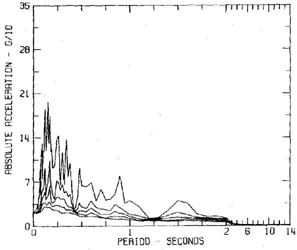
RESPONSE SPECTRA IIIB032 COMP S86W PUGET SOUND, WASHINGTON EARTHQUAKE APR 29, 1965 - 0728 PST OLYMPIA, WASHINGTON HWY TEST LAB DAMPING VALUES ARE 0, 2, 5, 10 AND 20 PERCENT OF CRITICAL
