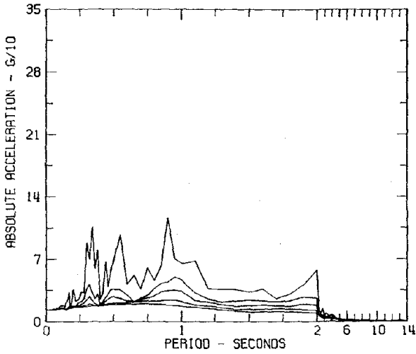
RESPONSE SPECTRA IIIA005 COMP S48E KERN COUNTY, CALIFORNIA EARTHQUAKE JULY 21, 1952 - 0453 PDT SANTA BARBARA COURTHOUSE DAMPING VALUES ARE 0, 2, 5, 10 AND 20 PERCENT OF CRITICAL
