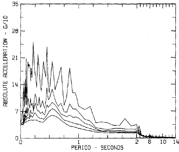
RESPONSE SPECTRA IIIA001 COMP S00E IMPERIAL VALLEY EARTHQUAKE MAY 18, 1940 - 2037 PST EL CENTRO SITE IMPERIAL VALLEY IRRIGATION DISTRICT DAMPING VALUES ARE 0, 2, 5, 10 AND 20 PERCENT OF CRITICAL
