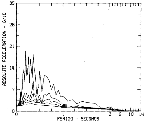
RESPONSE SPECTRA IIIA004 COMP N21E KERN COUNTY, CALIFORNIA EARTHQUAKE JULY 21, 1952 - 0453 PDT TAFT LINCOLN SCHOOL TUNNEL DAMPING VALUES ARE 0, 2, 5, 10 AND 20 PERCENT OF CRITICAL
