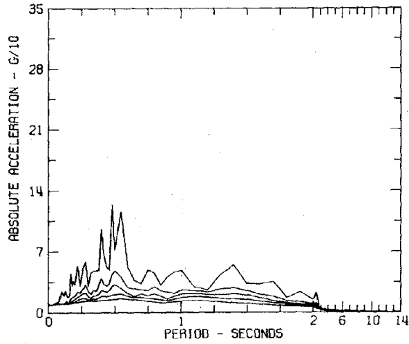
RESPONSE SPECTRA IIIA005 COMP N42E KERN COUNTY, CALIFORNIA EARTHQUAKE JULY 21, 1952 - 0453 PDT SANTA BARBARA COURATHOUSE DAMPING VALUES ARE 0, 2, 5, 10 AND 20 PERCENT OF CRITICAL
