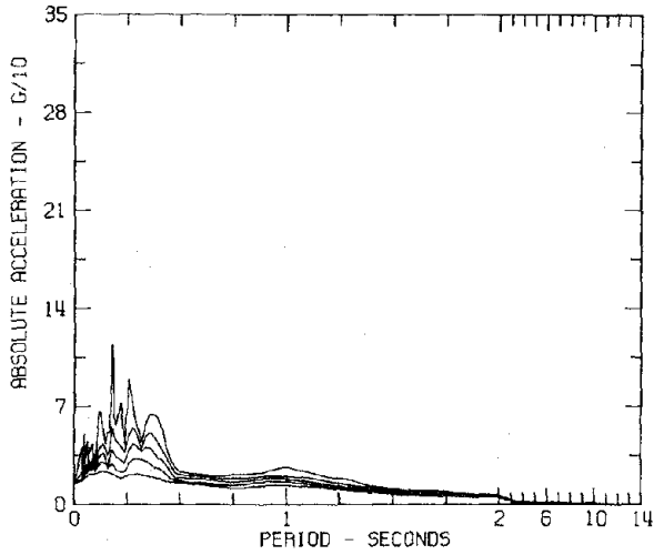
RESPONSE SPECTRA IIIB025 COMP S90W HELENA, MONTANA EARTHQUAKE OCT 31, 1935 - 1138 MST HELENA, MONTANA CARROLL COLLEGE DAMPING VALUES ARE 0, 2, 5, 10 AND 20 PERCENT OF CRITICAL
