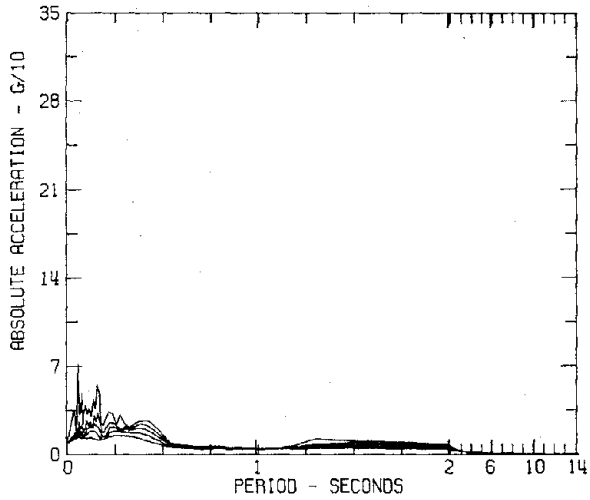
RESPONSE SPECTRA IIIB025 COMP DOWN HELENA, MONTANA EARTHQUAKE OCT 31, 1935 - 1138 MST HELENA, MONTANA CARROLL COLLEGE DAMPING VALUES ARE 0, 2, 5, 10 AND 20 PERCENT OF CRITICAL
