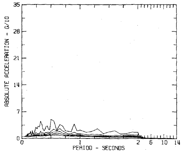
RESPONSE SPECTRA IIIA003 COMP 500E KERN COUNTY, CALIFORNIA EARTHQUAKE JULY 21, 1952 - 0453 PDT PASADENA - CALTECH ATHENAEUM DAMPING VALUES ARE 0, 2, 5, 10 AND 20 PERCENT OF CRITICAL
