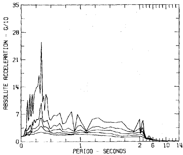
RESPONSE SPECTRA IIIC048 COMP S90W SAN FERNANDO EARTHQUAKE FEB 9, 1971 - 0600 PST 8244 ORION BLVD. 1ST FLOOR, LOS ANGELES, CAL. DAMPING VALUES ARE 0, 2, 5, 10 AND 20 PERCENT OF CRITICAL
