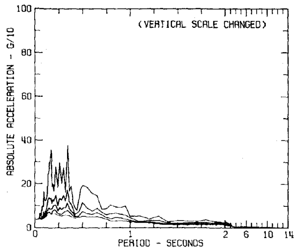
RESPONSE SPECTRA IIIZ001 COMP EAST MANAGUA EARTHQUAKE DEC 23, 1972 - 0629 GMT MANAGUA, NICARAGUA DAMPING VALUES ARE 0, 2, 5, 10 AND 20 PERCENT OF CRITICAL
