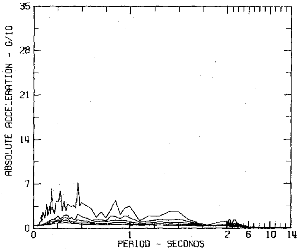
RESPONSE SPECTRA IIIA007 COMP N90E KERN COUNTY, CALIFORNIA EARTHQUAKE JULY 21, 1952 - 0453 PDT HOLLYWOOD STORAGE P.E. LOT DAMPING VALUES ARE 0, 2, 5, 10 AND 20 PERCENT OF CRITICAL
