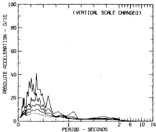
RESPONSE SPECTRA IIIZ001 COMP SOUTH MANAGUA EARTHQUAKE DEC 23, 1972 - 0629 GMT MANAGUA, NICARAGUA DAMPING VALUES ARE 0, 2, 5, 10 AND 20 PERCENT OF CRITICAL
