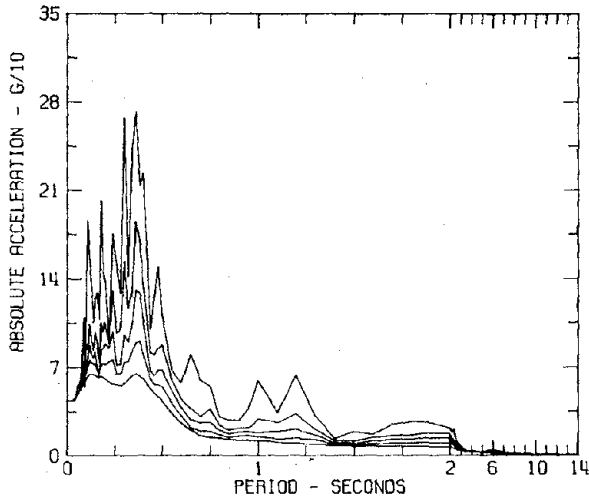
RESPONSE SPECTRA IIB034 COMP N85E PARKFIELD, CALIFORNIA EARTHQUAKE JUNE 27, 1966 - 2026 PST CHOLAME, SHANDON, CALIFORNIA ARRAY NO. 5 DAMPING VALUES ARE 0, 2, 5, 10 AND 20 PERCENT OF CRITICAL
