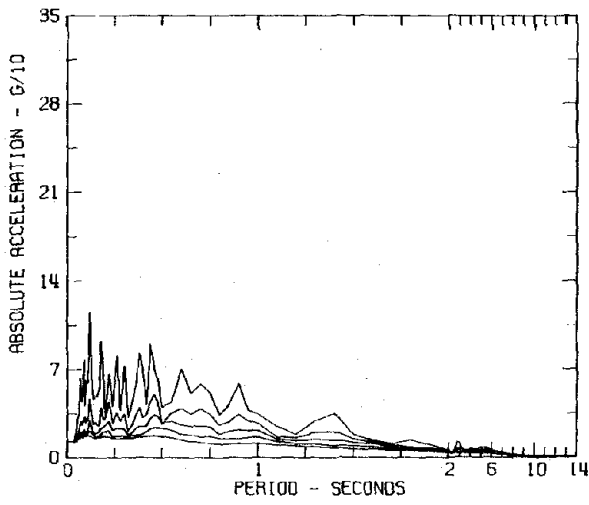
RESPONSE SPECTRA IIIC051 COMP N54W SAN FERNANDO EARTHQUAKE FEB 9, 1971 - 0600 PST 250 E FIRST STREET BASEMENT, LOS ANGELES, CAL. DAMPING VALUES ARE 0, 2, 5, 10 AND 20 PERCENT OF CRITICAL
