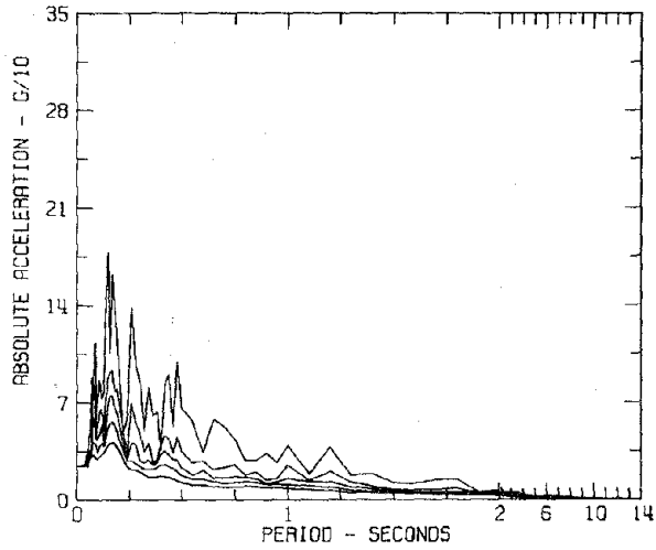
RESPONSE SPECTRA IIB035 COMP N50E PARKFIELD, CALIFORNIA EARTHQUAKE JUNE 27, 1966 - 2026 PST CHOLAME, SHANDON, CALIFORNIA ARRAY NO. 8 DAMPING VALUES ARE 0, 2, 5, 10 AND 20 PERCENT OF CRITICAL
