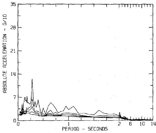
RESPONSE SPECTRA III8021 COMP N82W LONG BEACH EARTHQUAKE MAR 10, 1933 - 1754 PST VERNON CMO BLDG DAMPING VALUES ARE 0, 2, 5, 10 AND 20 PERCENT OF CRITICAL
