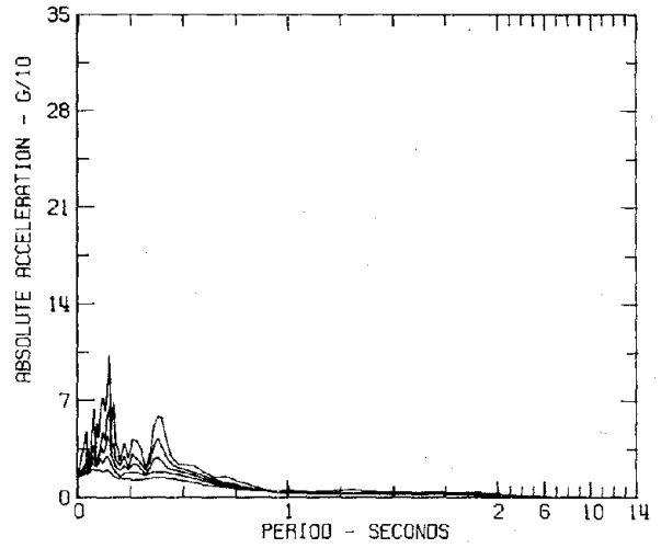
RESPONSE SPECTRA IIIB025 COMP S00W HELENA, MONTANA EARTHQUAKE OCT 31, 1935 - 1138 MST HELENA, MONTANA CARROLL COLLEGE DAMPING VALUES ARE 0, 2, 5, 10 AND 20 PERCENT OF CRITICAL
