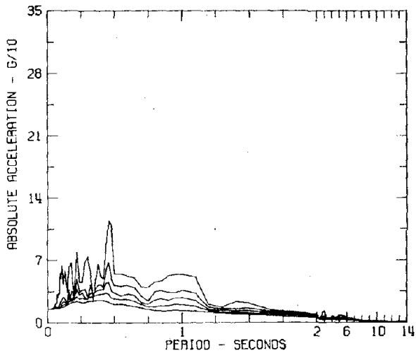
RESPONSE SPECTRA IIC054 COMP N52W SAN FERNANDO EARTHQUAKE FEB 9, 1971 - 0600 PST 445 FIGUEROA STREET, SUB-BASEMENT, LOS ANGELES, CAL. DAMPING VALUES ARE 0, 2, 5, 10 AND 20 PERCENT OF CRITICAL
