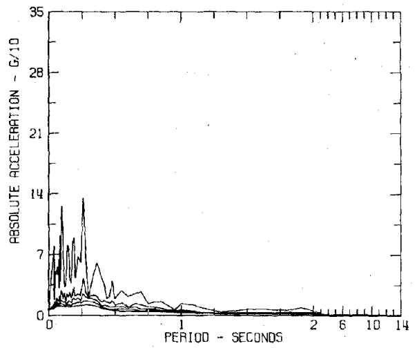
RESPONSE SPECTRA III8024 COMP VERT LOWER CALIFORNIA EARTHQUAKE DEC 30, 1934 - 0552 PST EL CENTRQ IMPERIAL VALLEY DAMPING VALUES ARE 0, 2, 5, 10 AND 20 PERCENT OF CRITICAL
