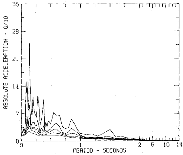
RESPONSE SPECTRA IIIB032 COMP S04E PUGET SOUND, WASHINGTON EARTHQUAKE APR 29, 1965 - 0728 PST OLYMPIA, WASHINGTON HWY TEST LAB DAMPING VALUES ARE 0, 2, 5, 10 AND 20 PERCENT OF CRITICAL
