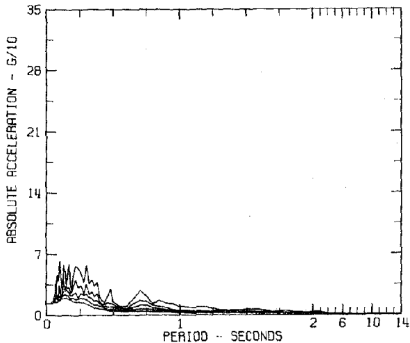
RESPONSE SPECTRA IIIB037 COMP DOWN PARKFIELD, CALIFORNIA EARTHQUAKE JUNE 27, 1966 - 2026 PST TEMBLOR, CALIFORNIA NO. 2 DAMPING VALUES ARE 0, 2, 5, 10 AND 20 PERCENT OF CRITICAL
