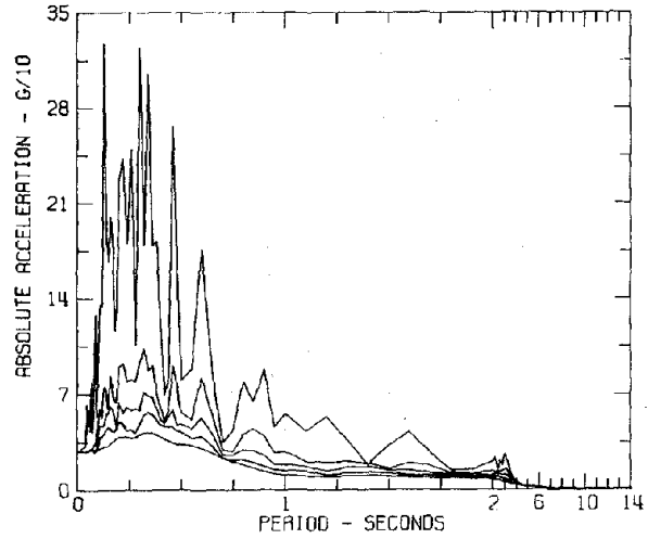
RESPONSE SPECTRA IIIB029 COMP N86E WESTERN WASHINGTON EARTHQUAKE APR 13, 1949 - 1156 PST OLYMPIA, WASHINGTON HWY TEST LAB DAMPING VALUES ARE 0, 2, 5, 10 AND 20 PERCENT OF CRITICAL
