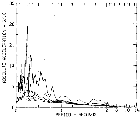
RESPONSE SPECTRA IIIB024 COMP 500W LOWER CALIFORNIA EARTHQUAKE DEC 30, 1934 - 0552 PST EL CENTRO IMPERIAL VALLEY DAMPING VALUES ARE 0, 2, 5, 10 AND 20 PERCENT OF CRITICAL
