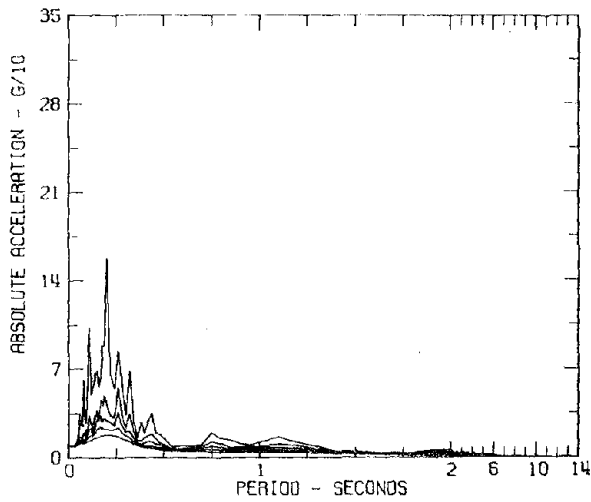
RESPONSE SPECTRA IIIG106 COMP S00W SAN FERNANDO EARTHQUAKE FEB 9, 1971 - 0600 PST CALTECH SEISMOLOGICAL LAB., PASADENA, CAL. DAMPING VALUES ARE 0, 2, 5, 10 AND 20 PERCENT OF CRITICAL
