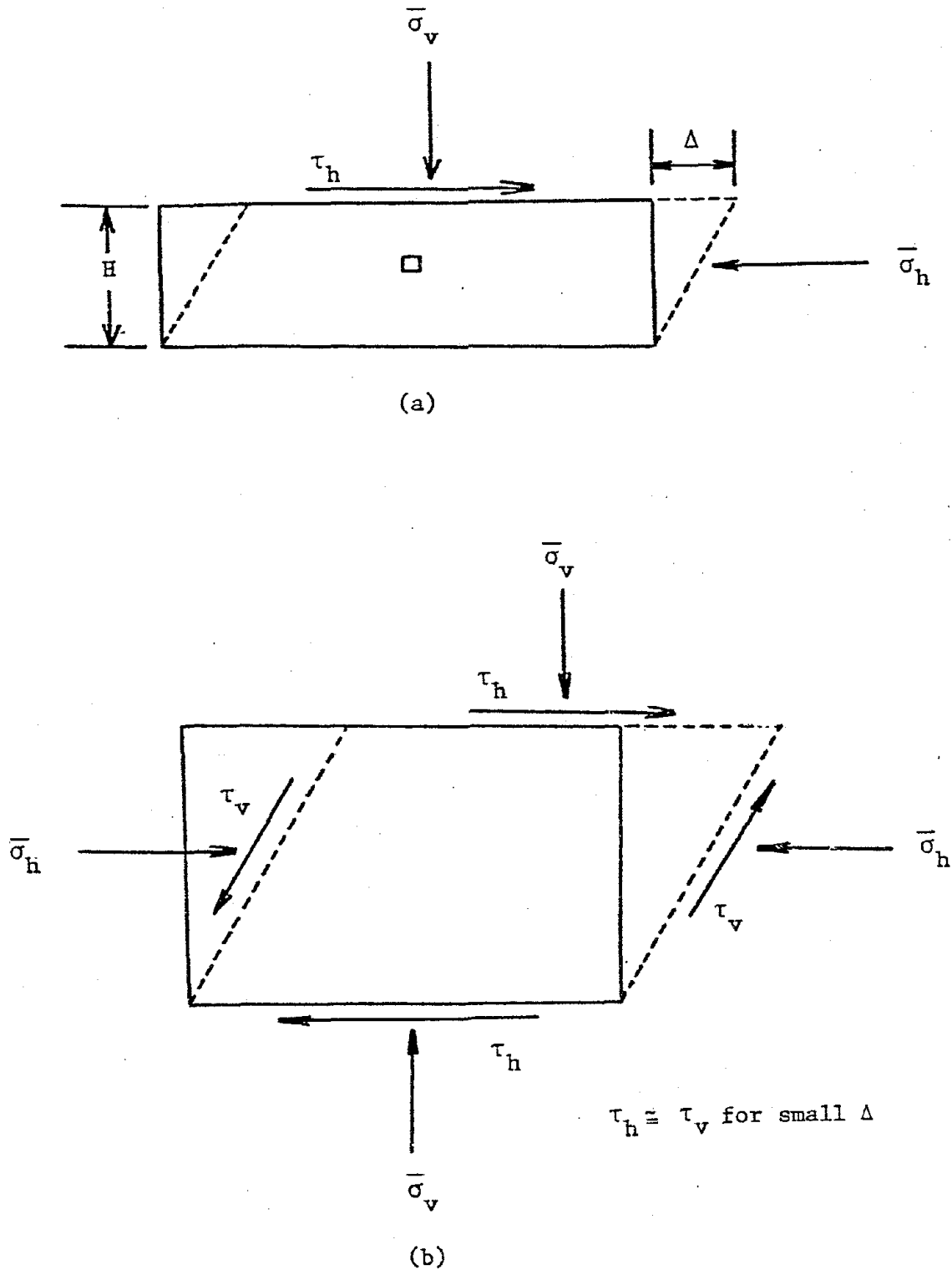
FIGURE 2. (a) MEASURED BOUNDARY STRESSES ACTING ON THE NGI DIRECT SIMPLE SHEAR SAMPLE (b) ASSUMED STRESS CONDITIONS ACTING ON AN ELEMENT FROM THE CENTER OF THE SAMPLE
