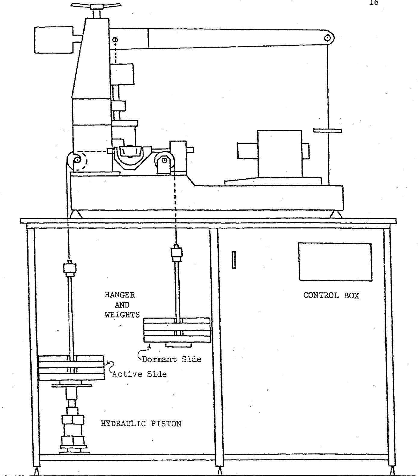
FIGURE 6. NGI DIRECT SIMPLE SHEAR DEVICE WITH MODIFICATIONS FOR CYCLIC LOADING CAPABILITIES
