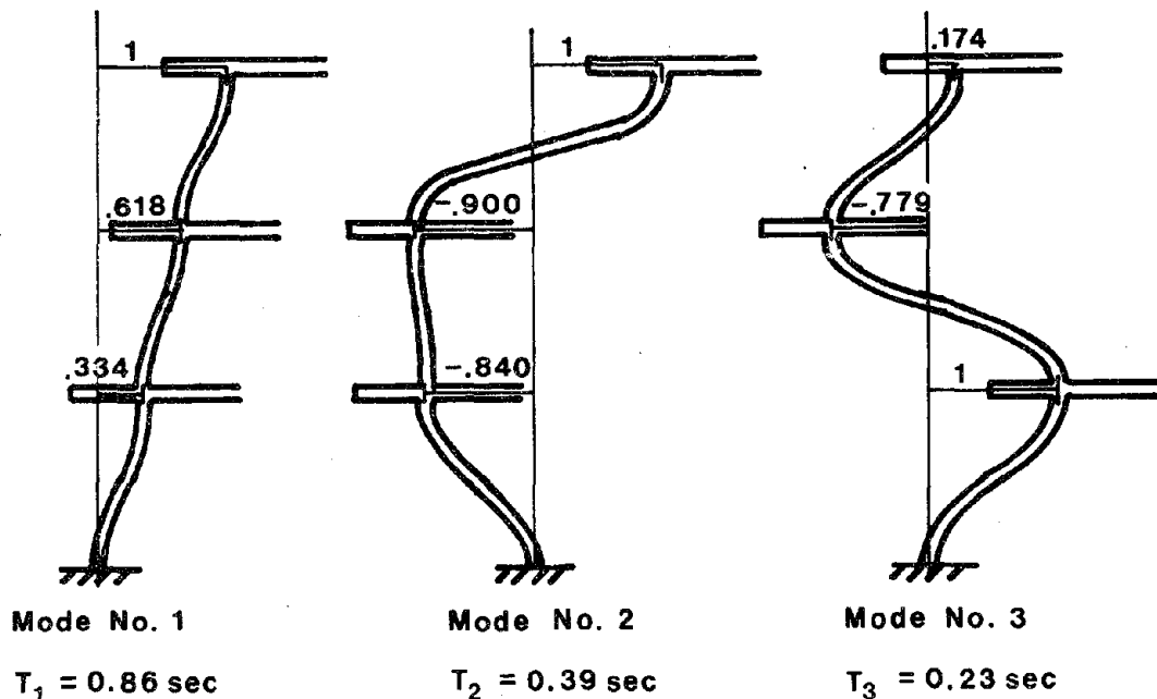
Figure 28 Computing center, mode shapes and periods.
