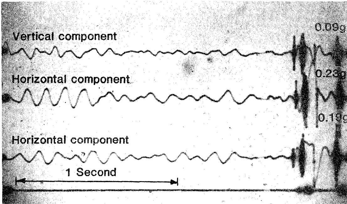
Figure 5 MO-2 strong-motion accelerogram recorded at Vrincioaia. Film drive malfunctioned.
