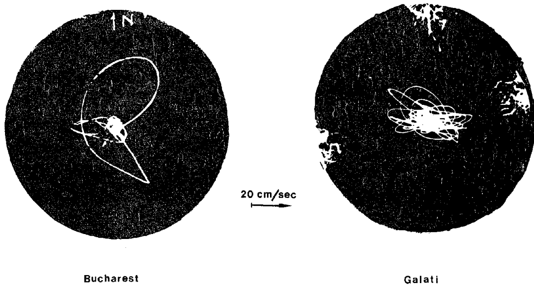
Figure 4 Seismoscope records obtained in Bucharest and Galati.
