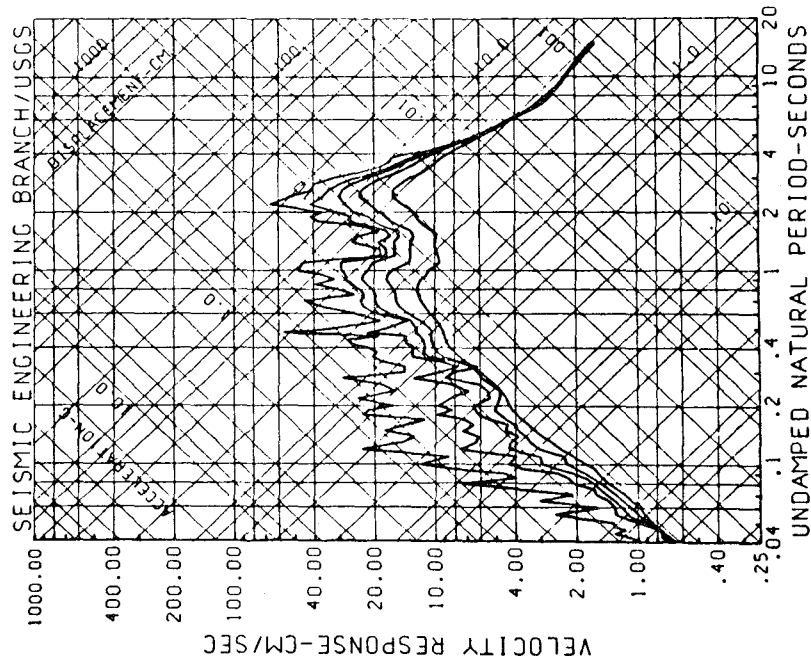
Figure 8 Response spectra, Bucharest (INCERC), March 4, 1977, down-up 0, 2, 5, 10, 20 percent critical damping (Ref 6).
