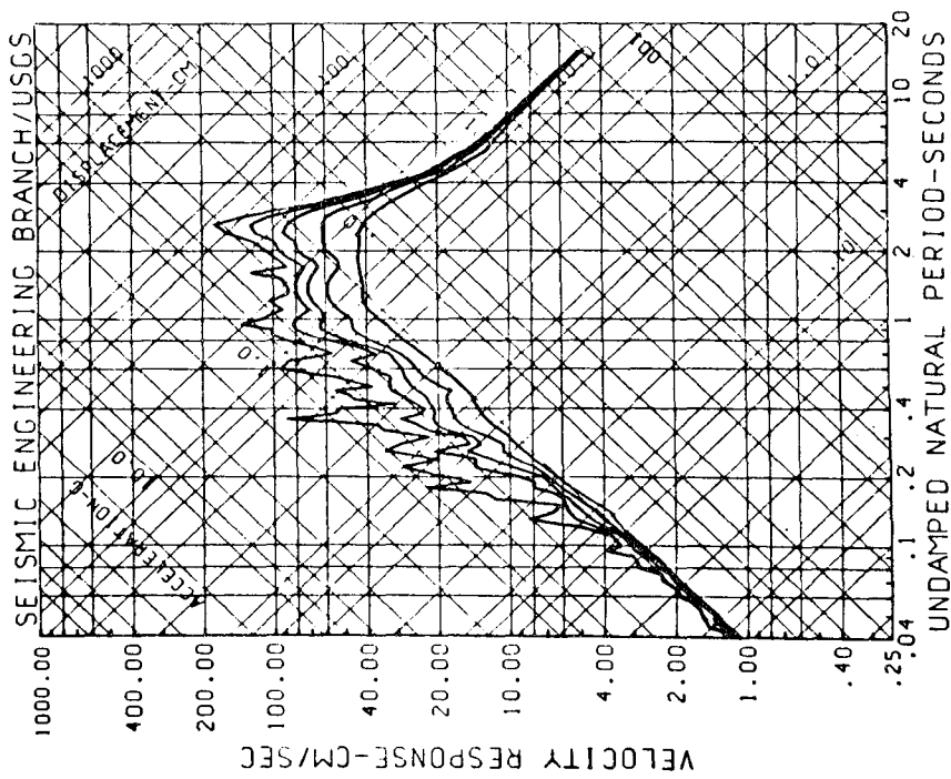
Figure 9 Response spectra, Bucharest (INCERC), March 4, 1977, E-W 0, 2, 5, 10, 20 percent critical damping (Ref 6).
