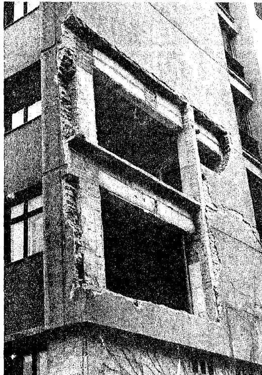
Figure 22 End wall of Emergency Hospital.
