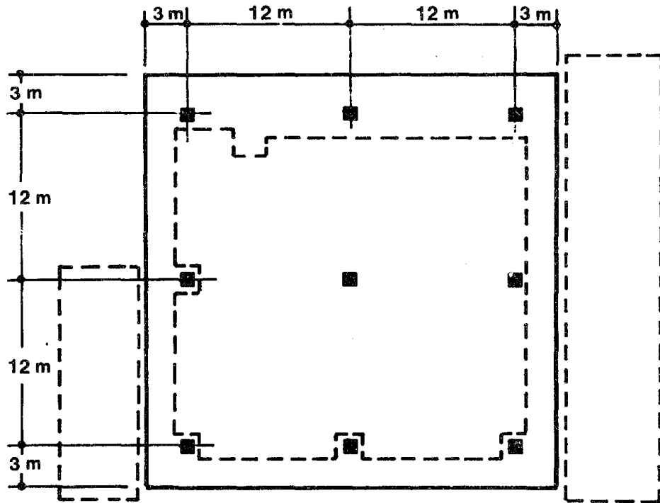
Figure 25 Computing center, ground-floor layout.
