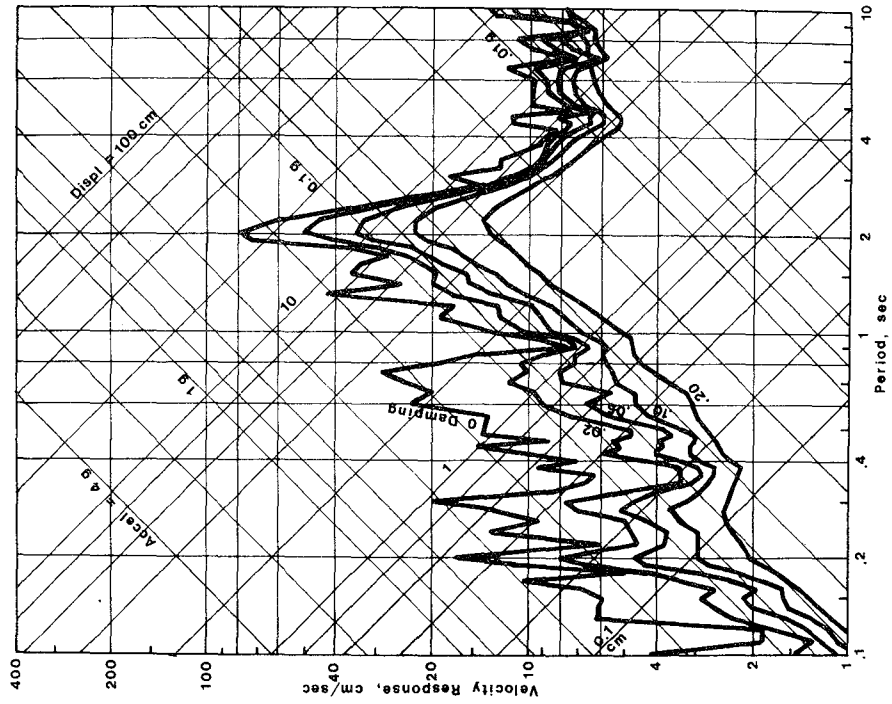
Figure 14 Response spectra, Nis, Yugoslavia, accelerogram of March 4, 1977, E-W component (epicentral distance = 1,200 km).
