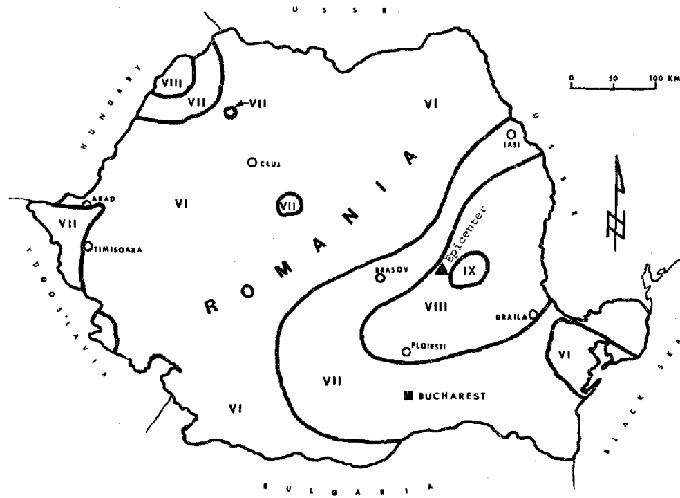
Figure 29 Seismic-zone map of Romania, 1970 code.
