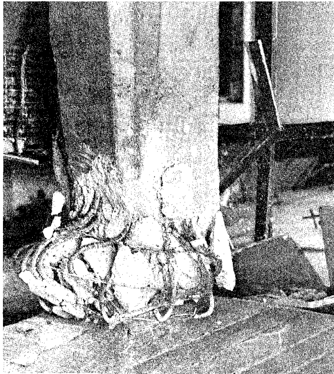
Figure 27 Computing center, column failure in ground story.
