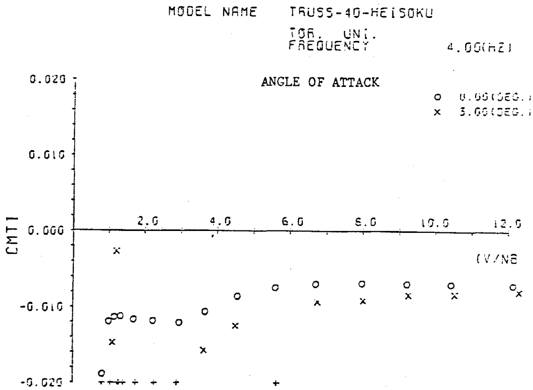
Fig.4-4 C_{MT}^I - V/NB (Model No.10)
