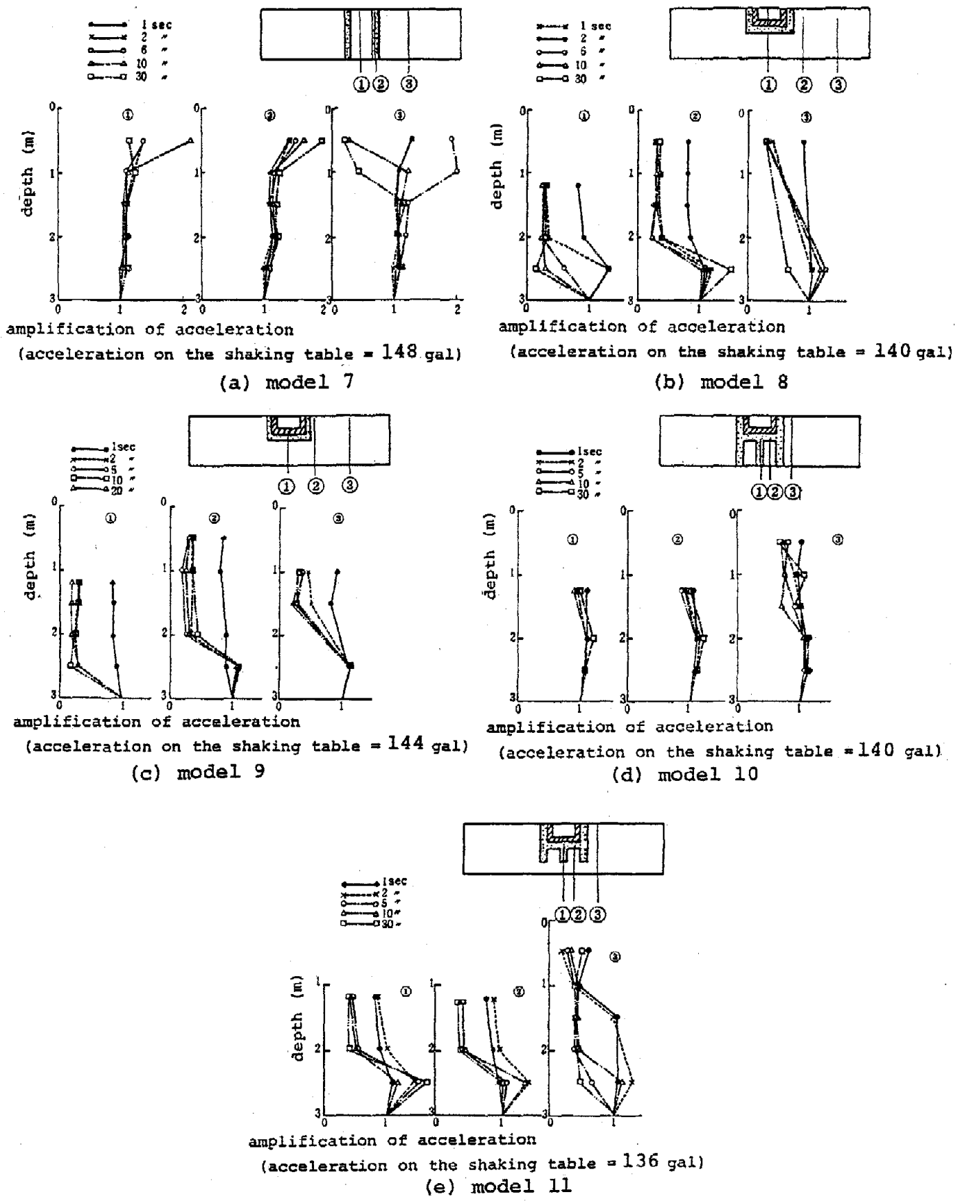
Figure 4 Amplification of acceleration along vertical direction
