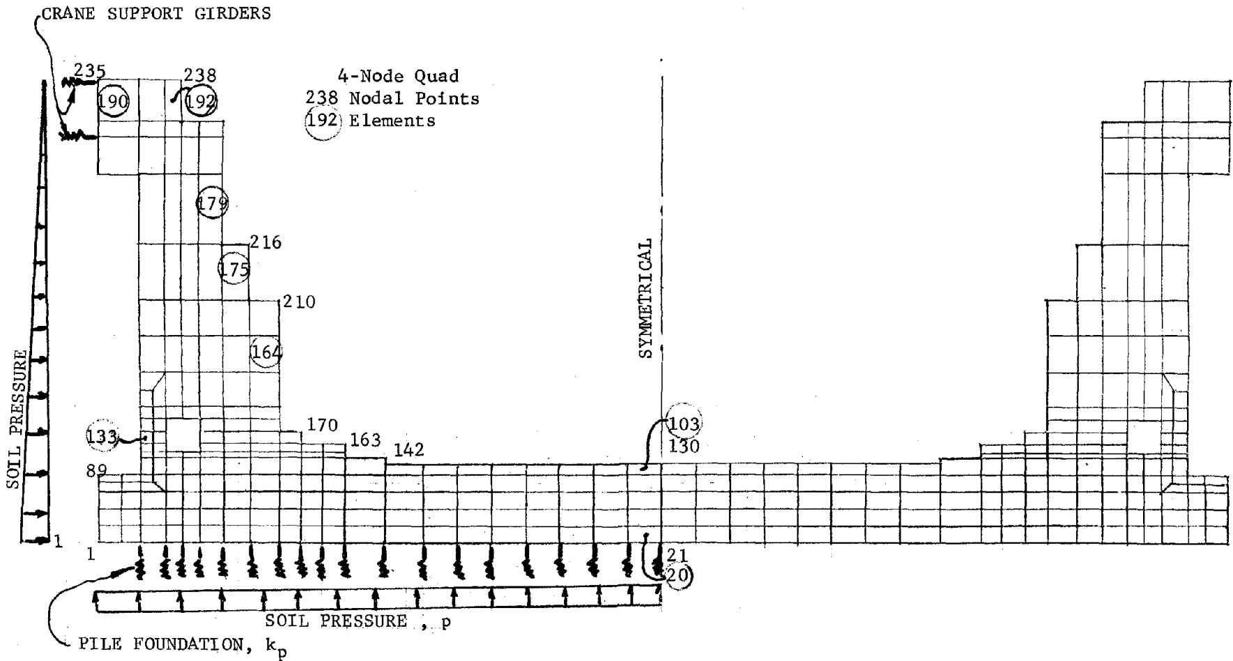
Figure 11. Computer model of one-half of a graving drydock
