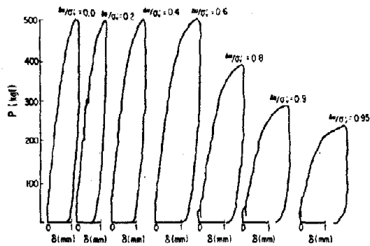
Fig. 19 An Example of Static Loading Test Results
