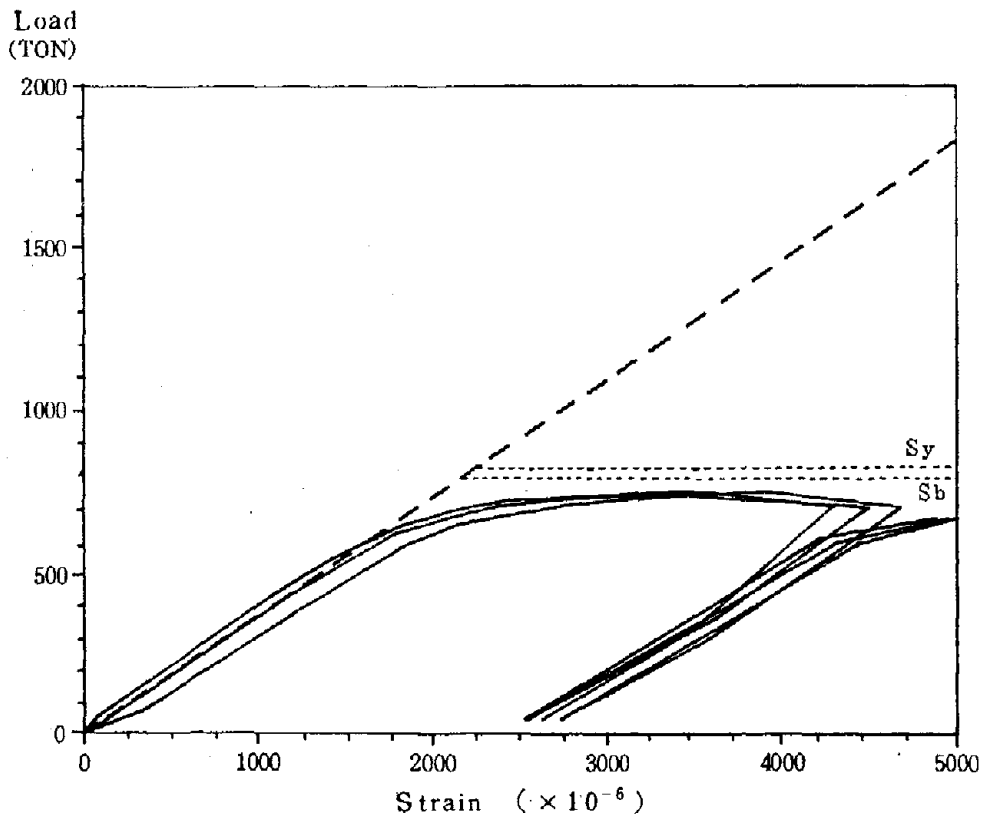
Fig. 19 Load - Strain Curve (A - 2)
