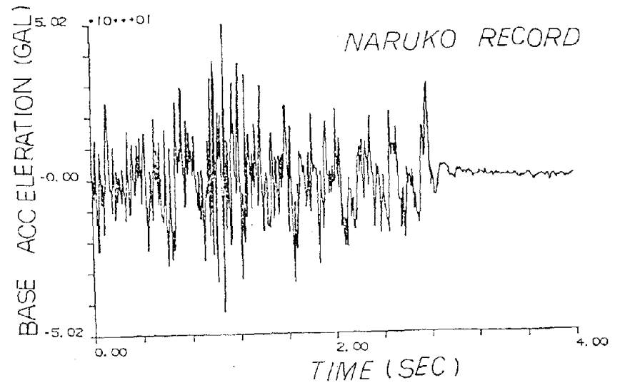
Figure 11. Time history of model no. 6
