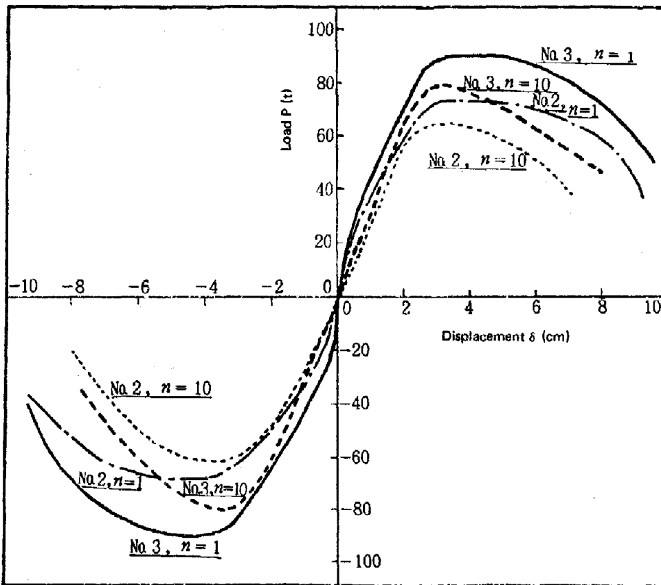
Fig. 37 Effect of the Hunch (Comparison of No. 2 and No. 3 Models)
