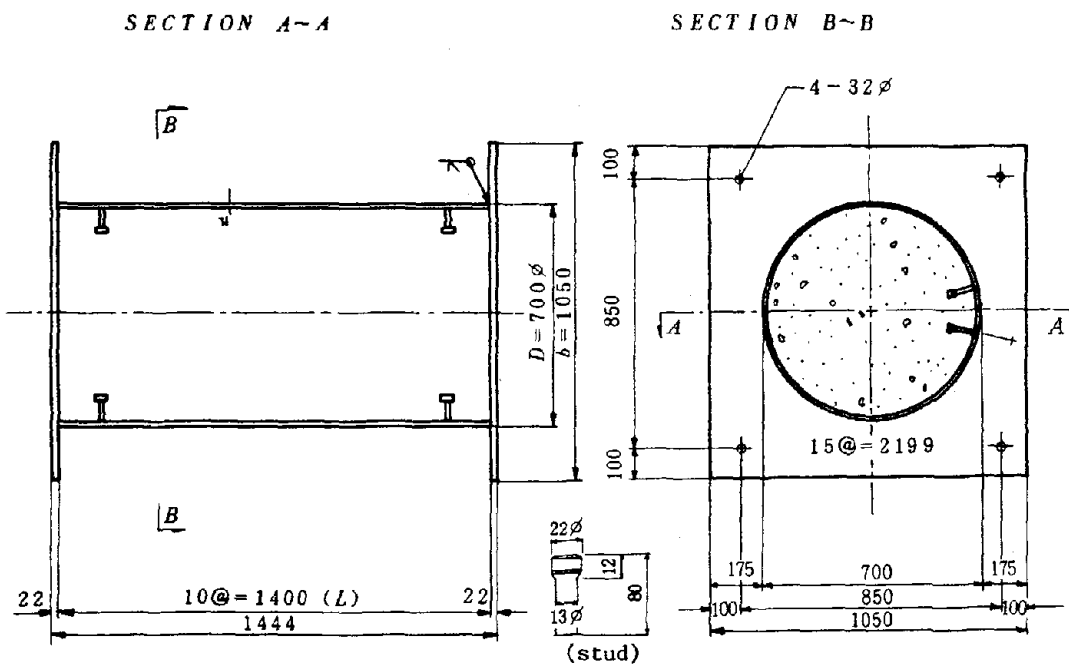
Fig. 4 Configuration of Test Specimen
