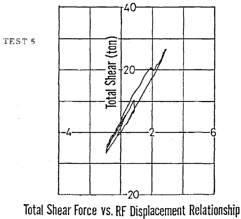
Fig. 6 Hysteresis Loops
