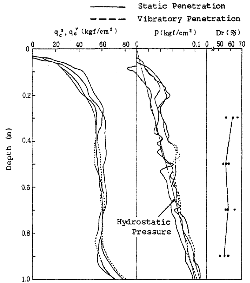
Fig. 5 Example of Penetration Test Result (Dense Condition)
