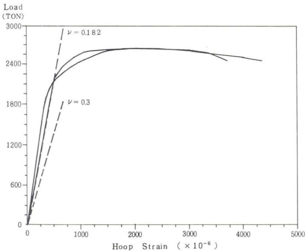
Fig. 38 Load - Hoop Strain Curve (B - 6)
