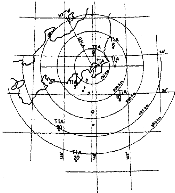
Fig. 6 Locations of Epicenter
