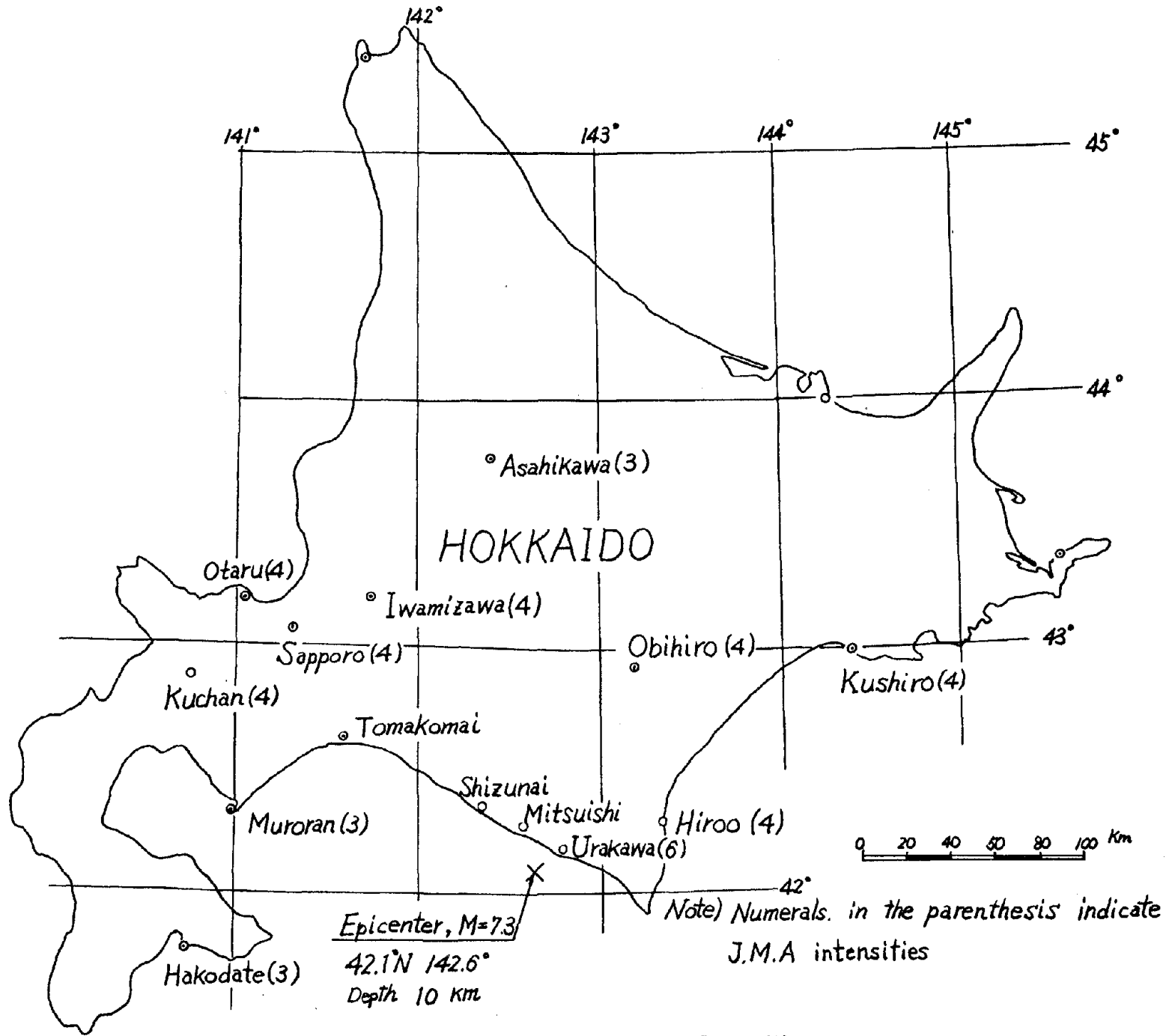
Figure 1. Epicenter and J.M.A. Intensities, (Urakawa-oki Earthquake of March 21, 1982)
