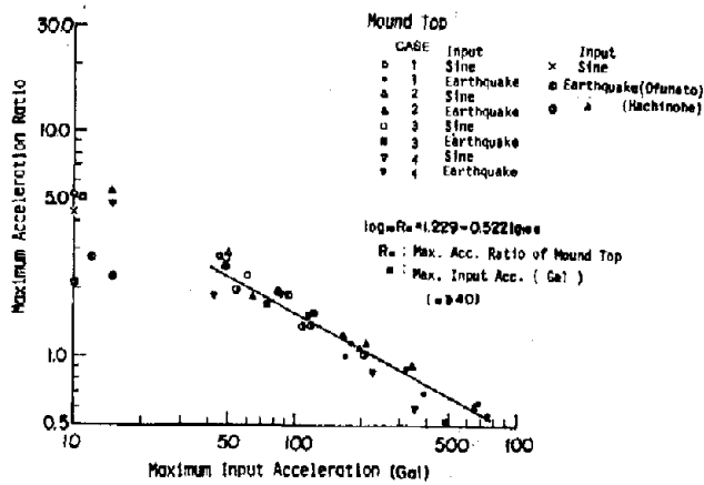
Fig. 9 Maximum Acceleration Ratio of Mound Top versus Maximum Input Acceleration
