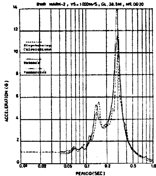
Fig.14 Floor Response Spectra (Damping Ratio 1%); V_s=1000\text{m/sec} , Magnitude 7.0 and Epicentral Distance 20km
