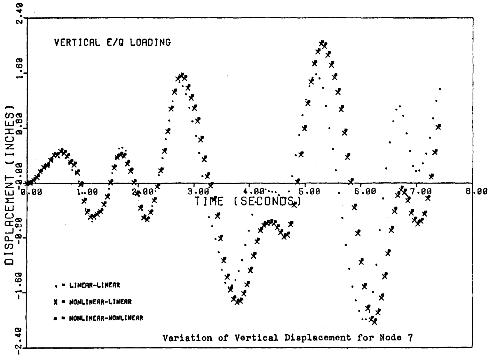
Figure 11. Variation of vertical displacement for Node 7
