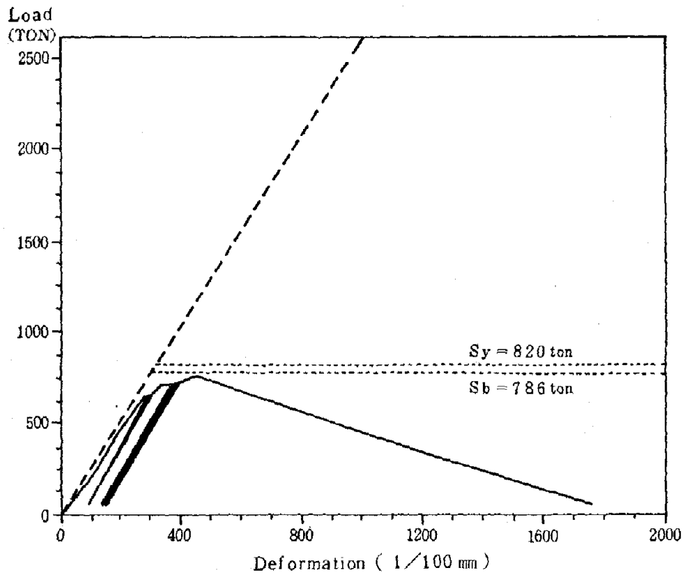
Fig. 10 Load - Deformation Curve (A - 3)
