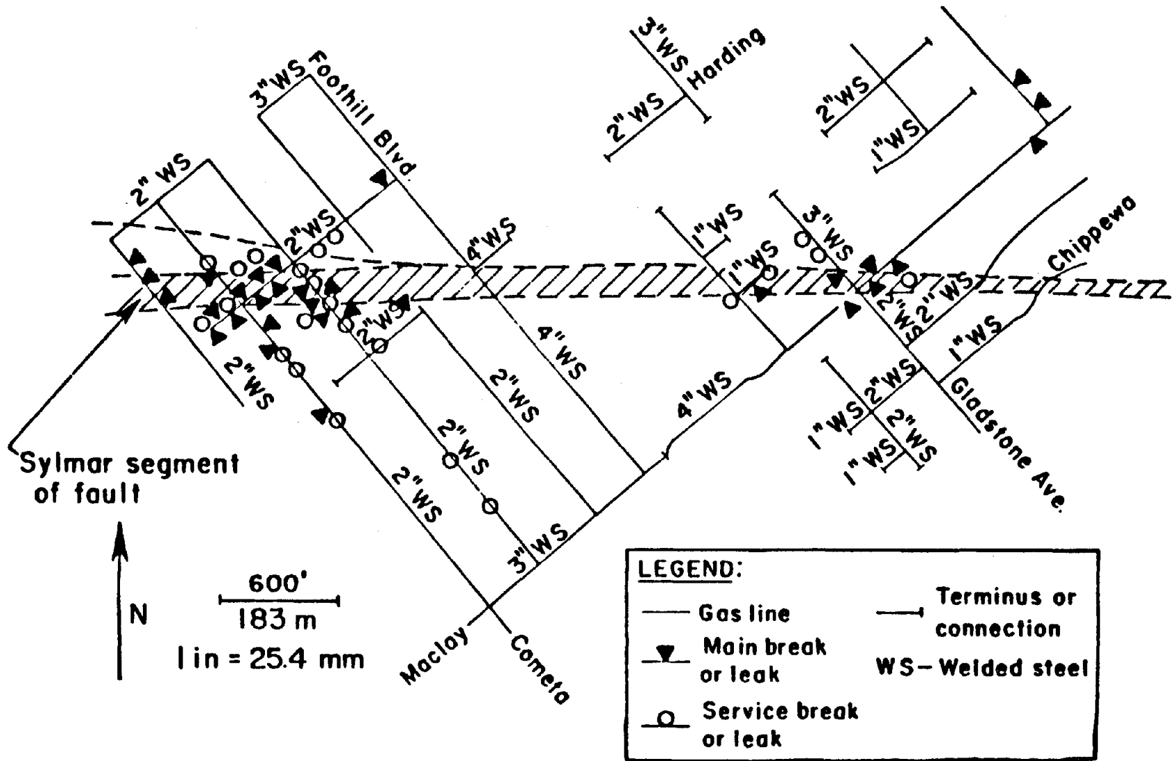
Figure 1b: Gas main damage along the Sylmar segment of San Fernando fault zone [1].
