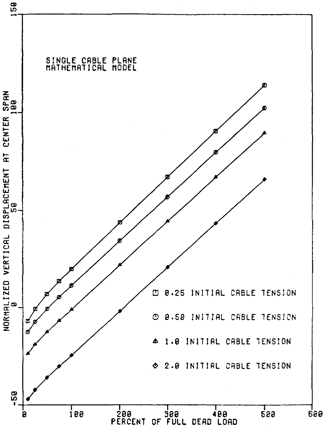
Figure 7. Effect of cable non-linearity
