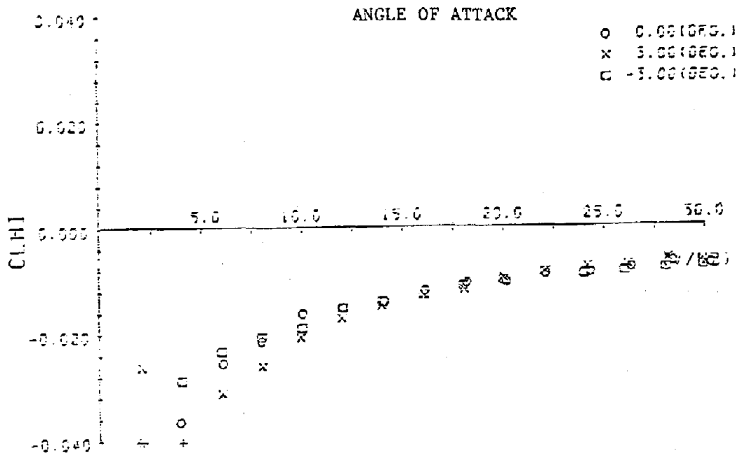
Fig. 4-1 C_{LH}^I - V/NB (Model No. 7)
