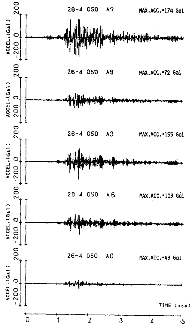
Fig. 6 Response Acceleration
