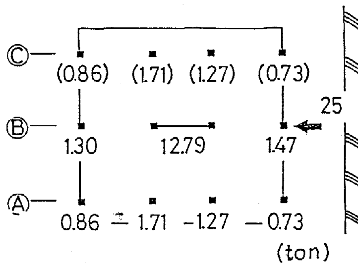
Fig.5 Measured Shear Force Distribution (5th Story)
