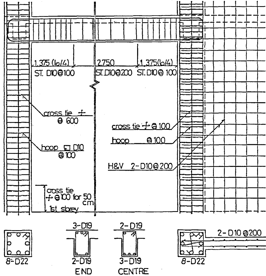
Fig. 3 Details of Reinforcing First Floor
