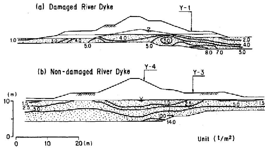
Fig. 26 Distribution of Excessive Pore Water Pressure Comparing Liquefied River Dyke with Non-Liquefied River Dyke
