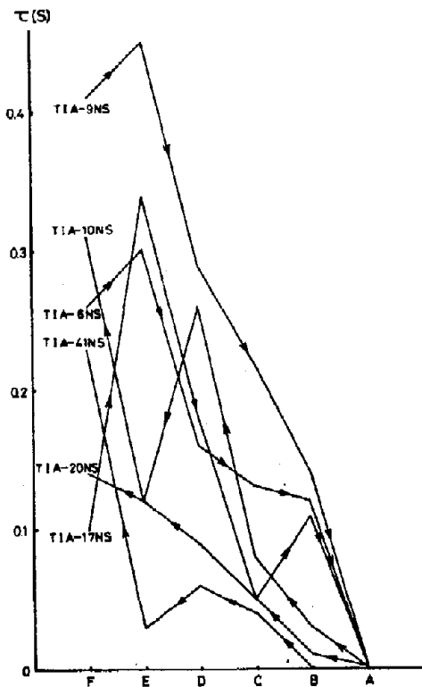
Fig. 11 Phase Delays
