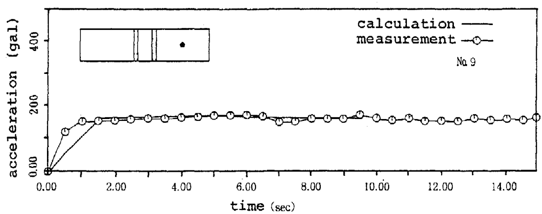
Figure 10 Comparison of acceleration of calculation and measurement
