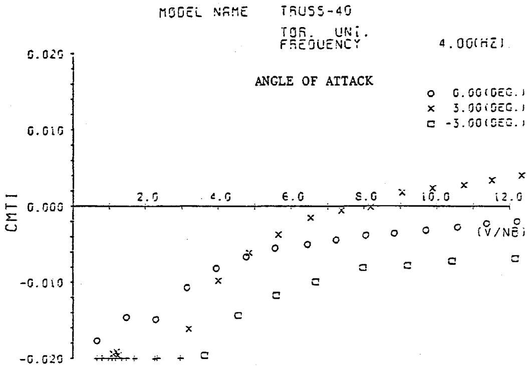
Fig.4-3 C_{MT}^I - V/NB (Model No.7)
