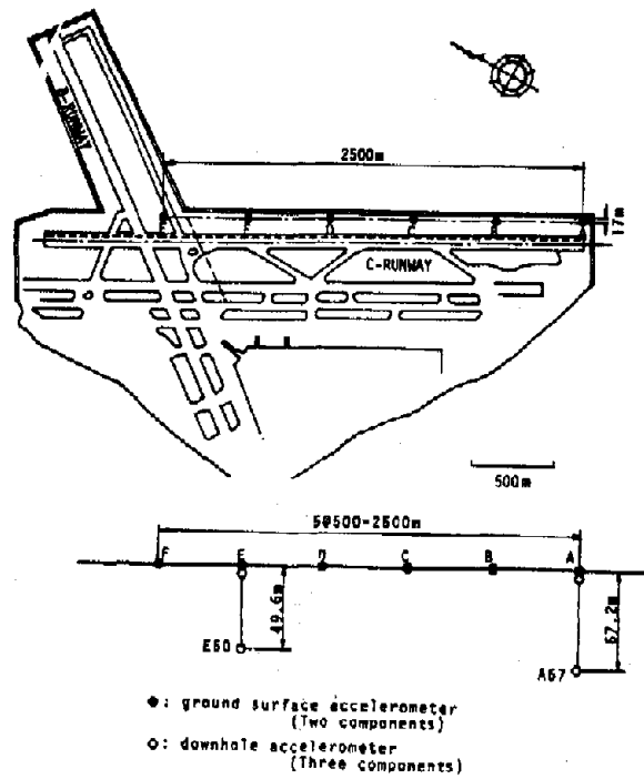
Fig. 1 Deployment of Accelerometers
