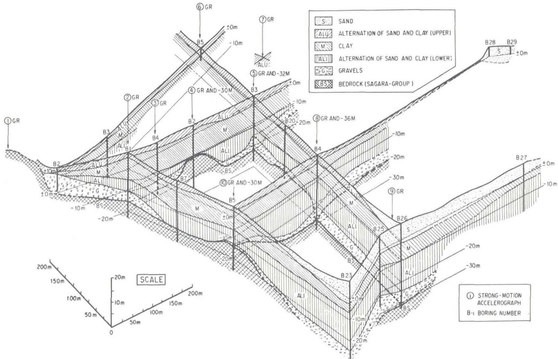
Fig. 4 Ground Conditions at Array Region of Sagara Area
