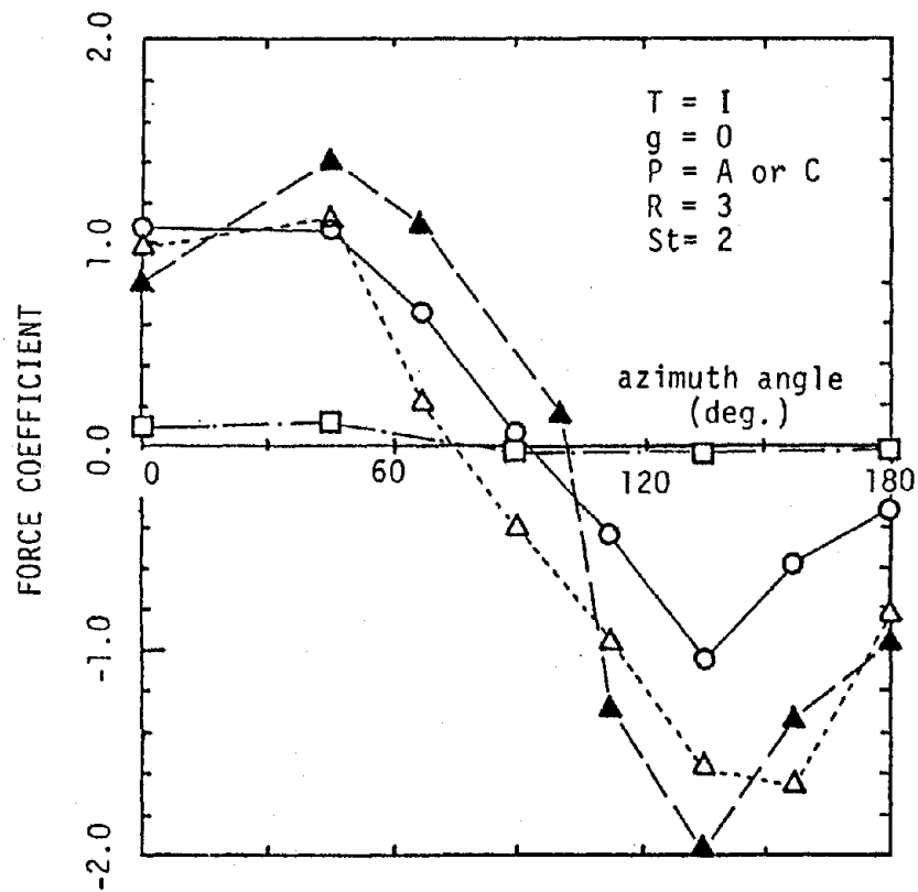
Fig. 13 Variation of force coefficient with azimuth angle □--- mounting pattern (b), \Delta --- (c), \circ — (d), \blacktriangle — (e)
