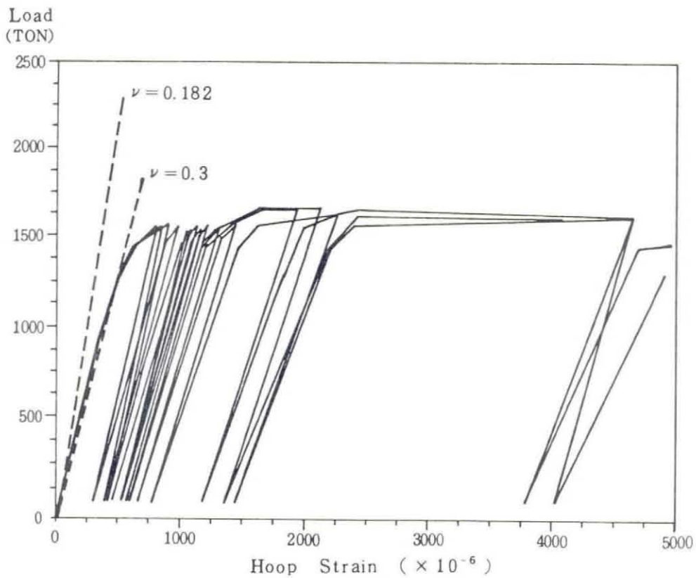
Fig. 37 Load - Hoop Strain Curve (B - 5)
