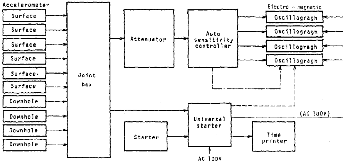
Fig. 5 Observation System
