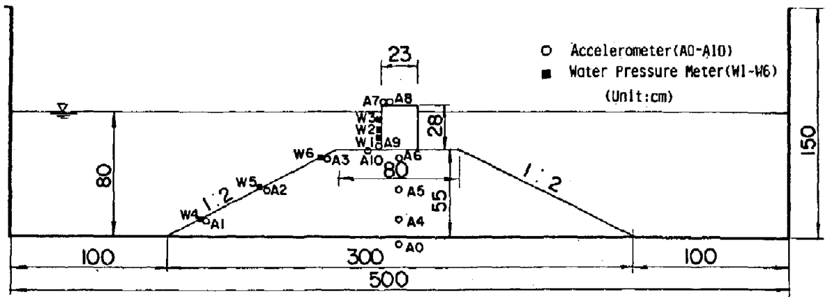
Fig. 2 Section of Breakwater Model
