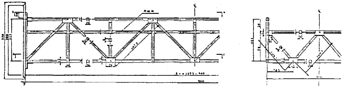
Stiffening truss
