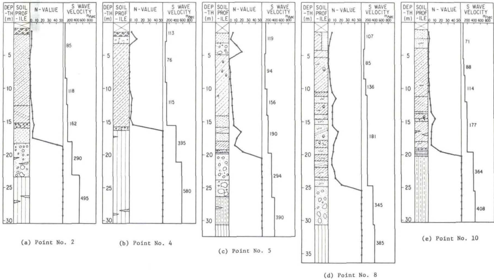
Fig. 3 Typical Soil Profile at Sagara Area
