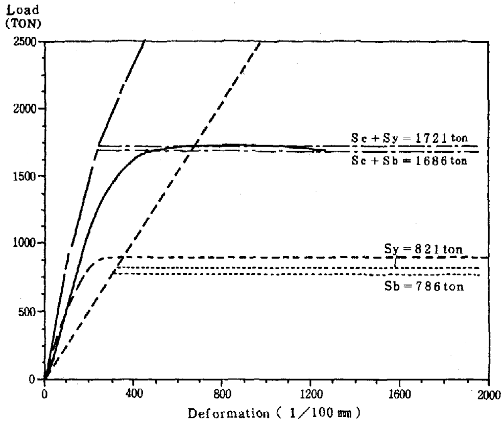
Fig. 13 Load - Deformation Curve (B - 2)
