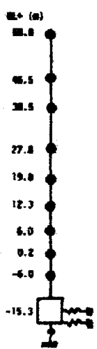
Fig.9 Lumped Mass Model
