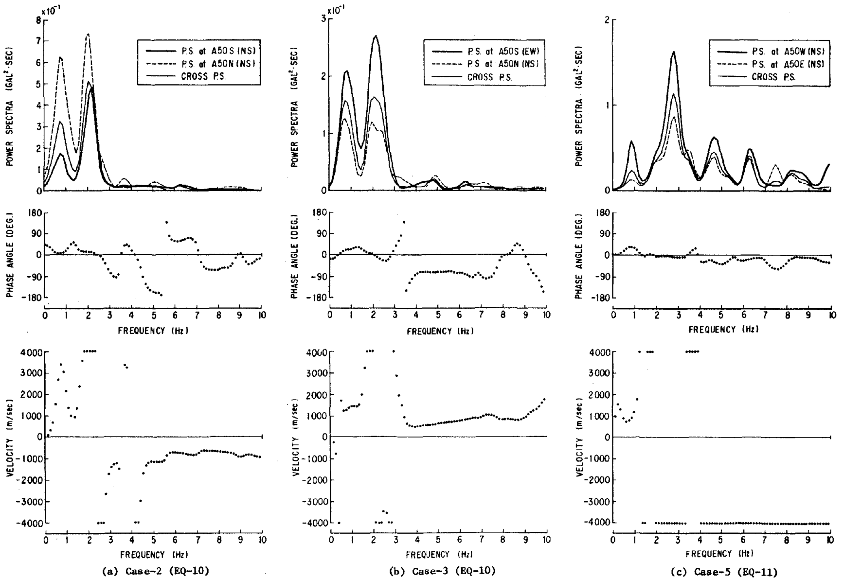
Fig. 19 (1) Power Spectra S_{mm} , S_{nn} and S_{mn} , Phase Angle \theta_{mn} , and Apparent Velocity V_{mn} in Horizontal Direction between A50S and A50N (Cases 2 and 3), and, between A50W and A50E (Case 5) at A-Field of Local Laboratory Array at PWRI Campus
