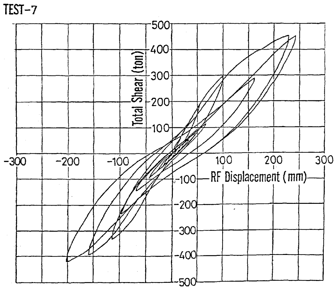
Total Shear Force vs. RF Displacement Relationship
