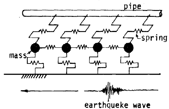
Fig. 14 Calculation Model
