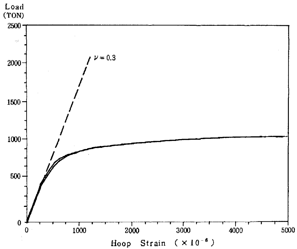
Fig. 32 Load-Hoop Strain Curve (A - 4)
