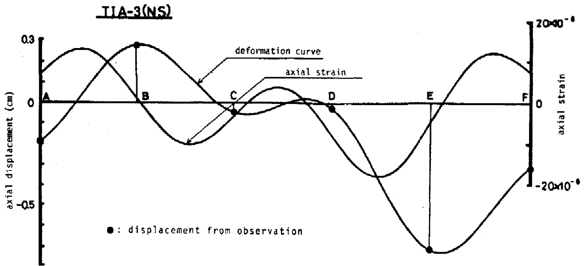
Fig. 8 Deformation Curve and Axial Strain
