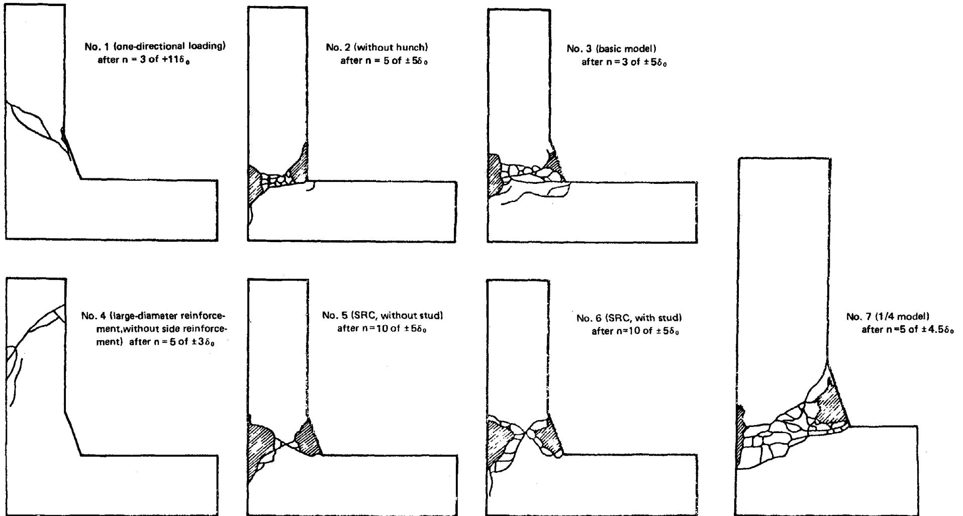
Fig. 34 Final Destruction Modes of Specimens
