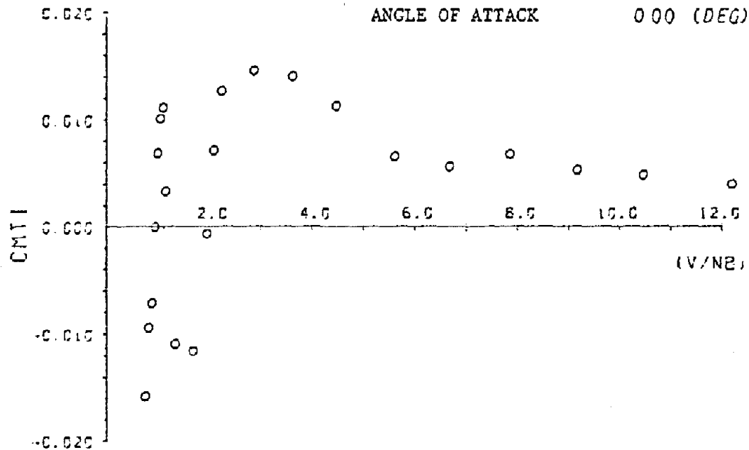
Fig.4-13 C_{MT}^I - V/NB (Model No.16)
