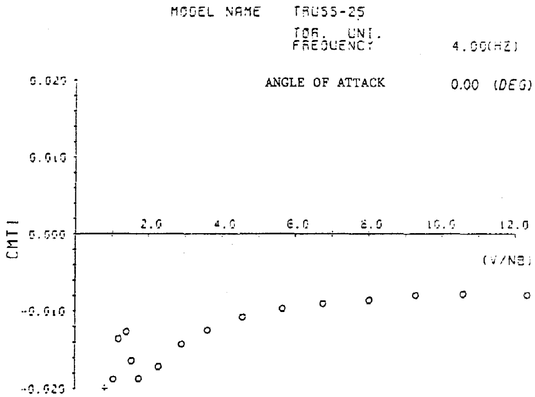
Fig.4-8 C_{MT}^I - V/NB (Model No.1)
