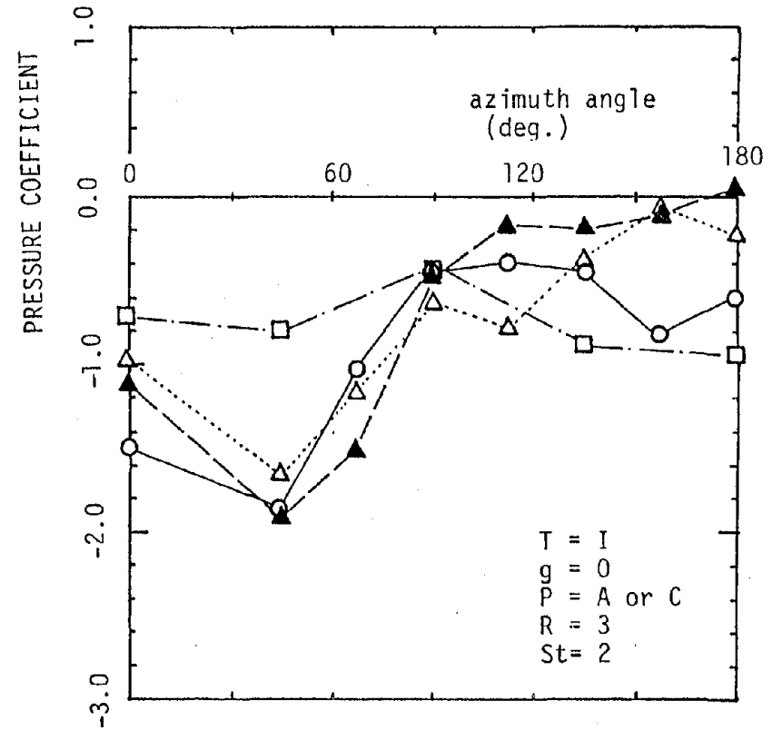
Fig. 12 Variation of lower wind pressure coefficient with azimuth angle □---mounting pattern (b), △----(c), ○—(d), ▲--(e)
