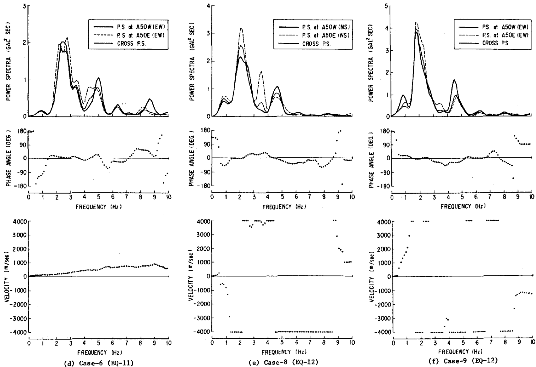
Fig. 19 (2) Power Spectra S_{mm} , S_{nn} and S_{mn} , Phase Angle \theta_{mn} , and Apparent Velocity V_{mn} in Horizontal Direction between A50W and A50E at A-Field of Local Laboratory Array at PWRI Campus
