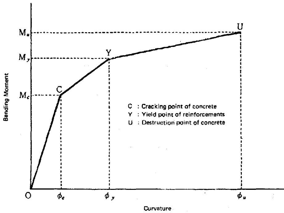
Fig. 41 Assumption of the M-\phi Relationship
