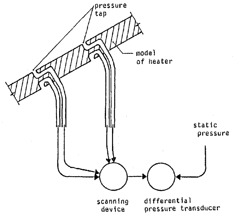
Fig. 3 Wind pressure measurement system
