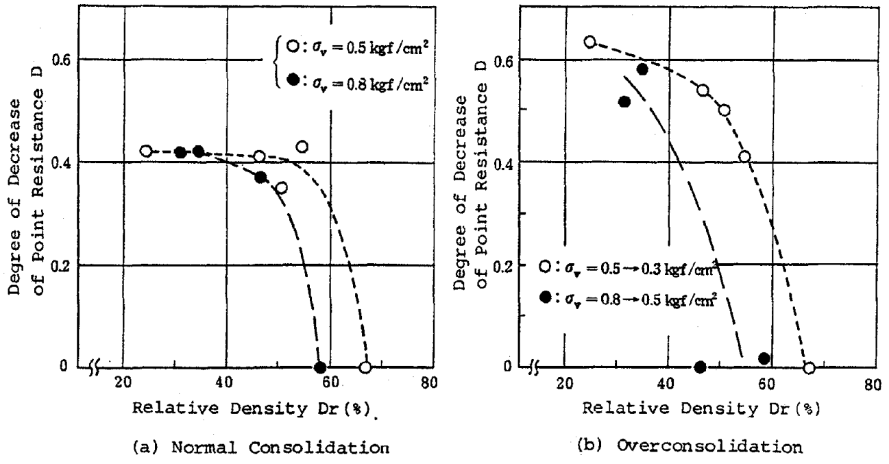
Fig. 7 Effect of Relative Density or Degree of Decrease of Point Resistance
