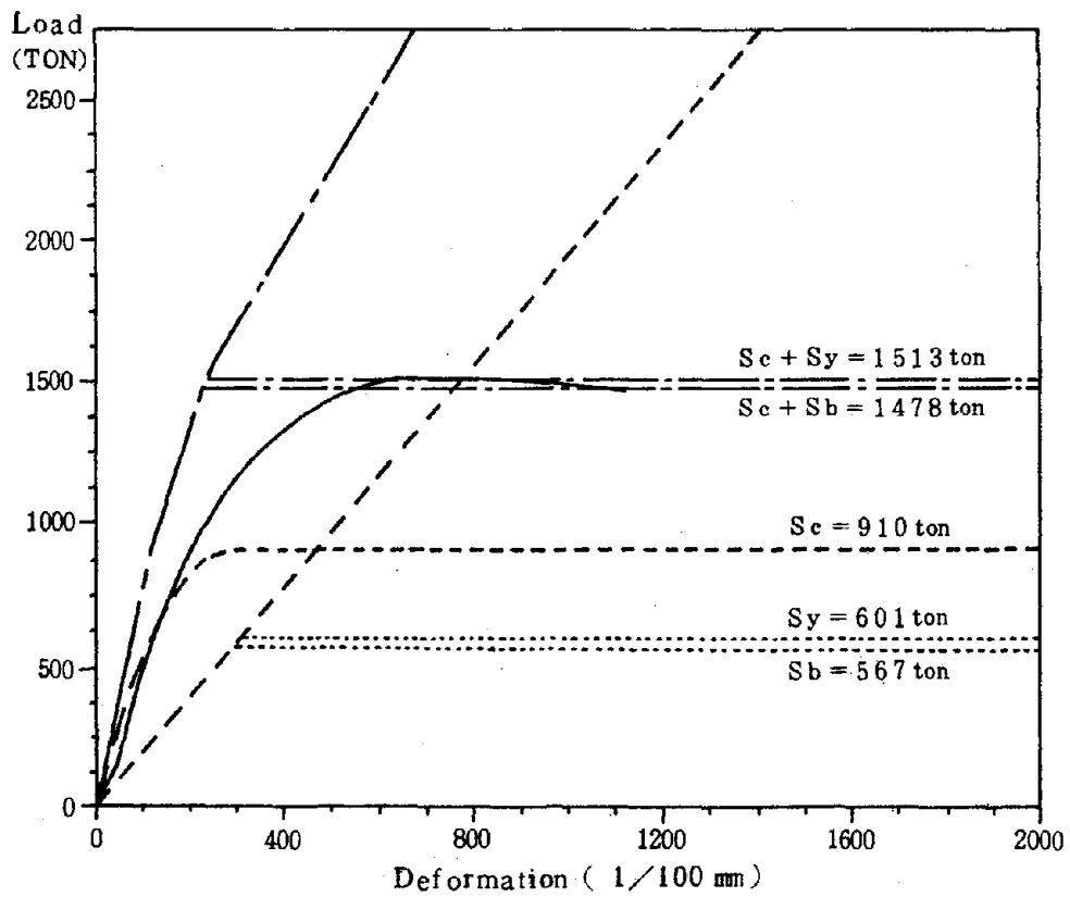
Fig. 12 Load - Deformation Curve (B - 1)
