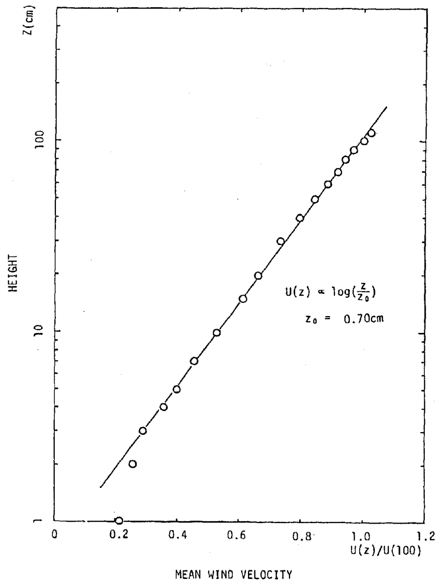
Fig. 6 Mean wind velocity profile
