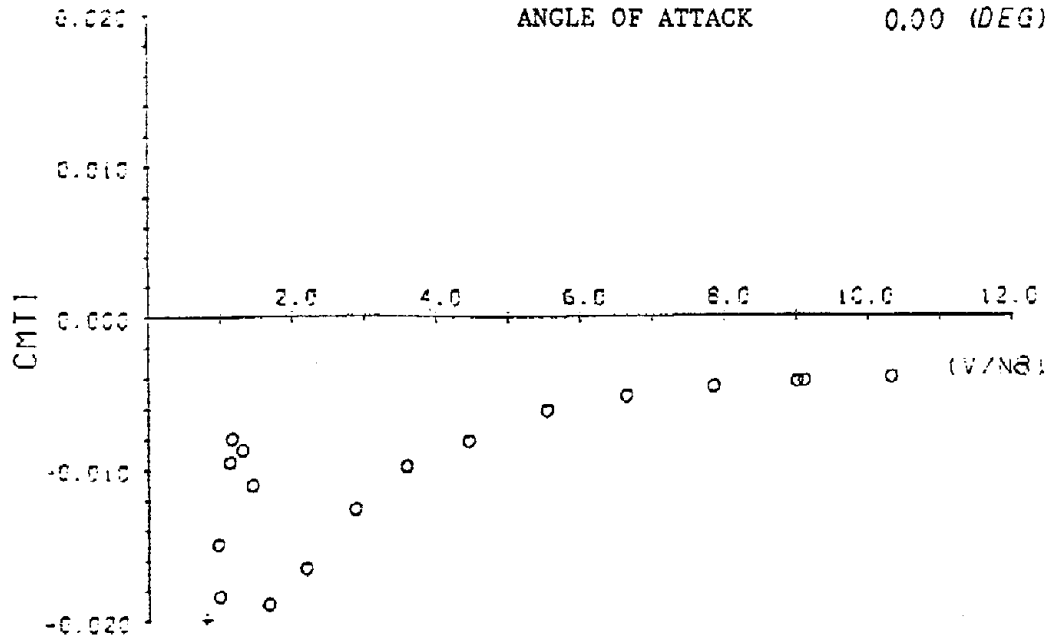
Fig.4-10 C_{MT}^I - V/NB (Model No.5)
