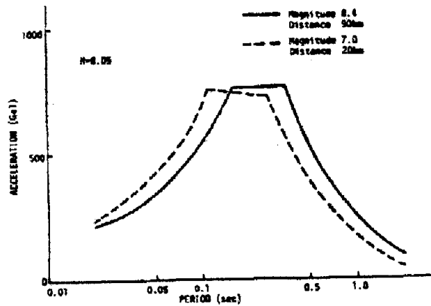
Fig.11 Design Response Spectra
