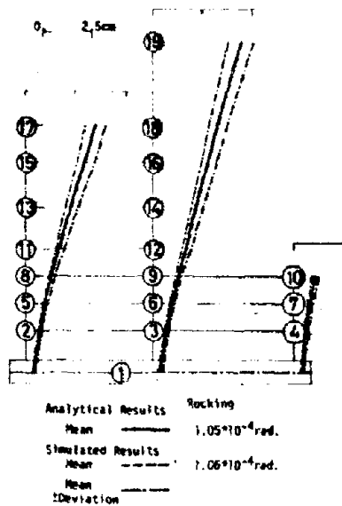
Fig. 5 Maximum Responses of Relative Displacements
