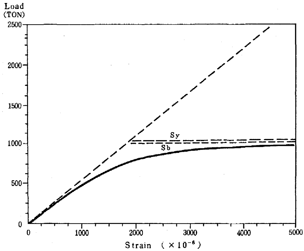
Fig. 21 Load - Strain Curve (A - 4)
