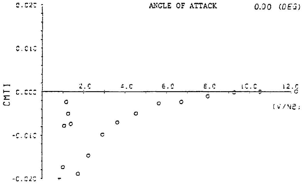
Fig.4-11 C_{MT}^I - V/NB (Model No.12)
