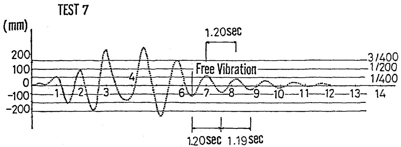
Fig. 9 Response Time Hystory
