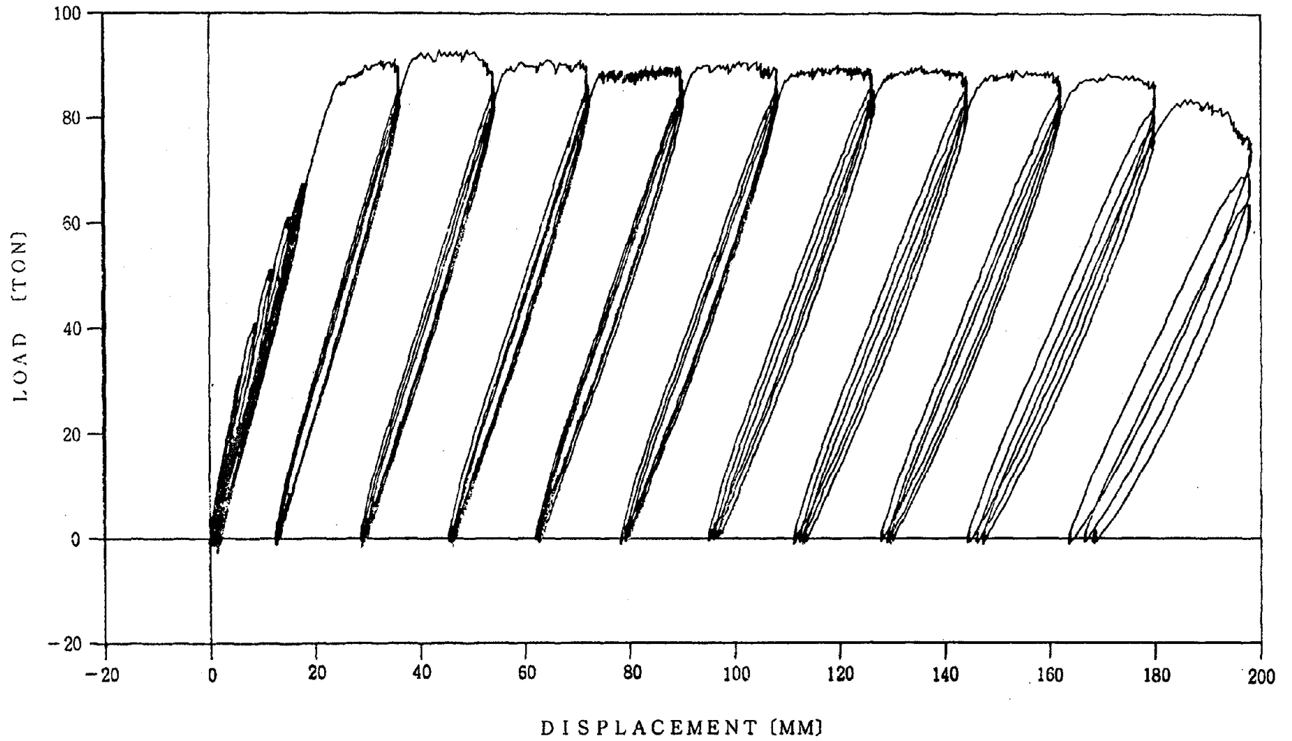
Fig. 32 Load-displacement Curve of No. 1 (One-directional Loading) Model
