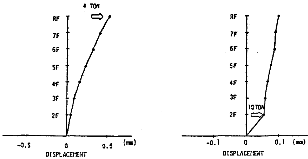
Fig.4 Distribution of Story Displacement Under Static Load
