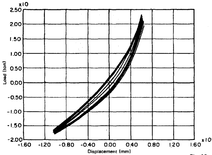
Fig. 18 Hysteretic Curve
