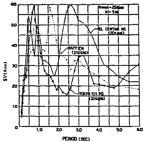
Fig. 1 Velocity response spectra ( V_{max} = 25 \text{ kine} , h = 5\% )
