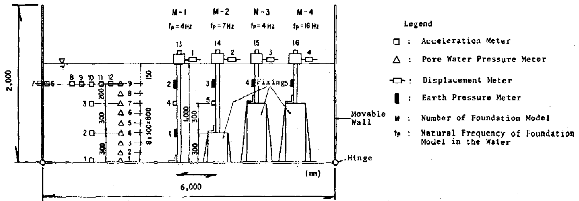
Fig. 8 Outline of Test Models and Measurement
