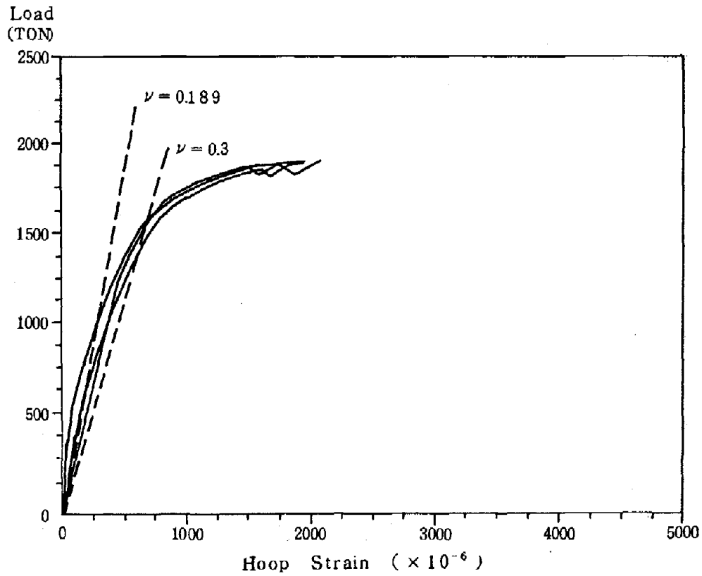
Fig. 36 Load -Hoop Strain Curve (B - 4)
