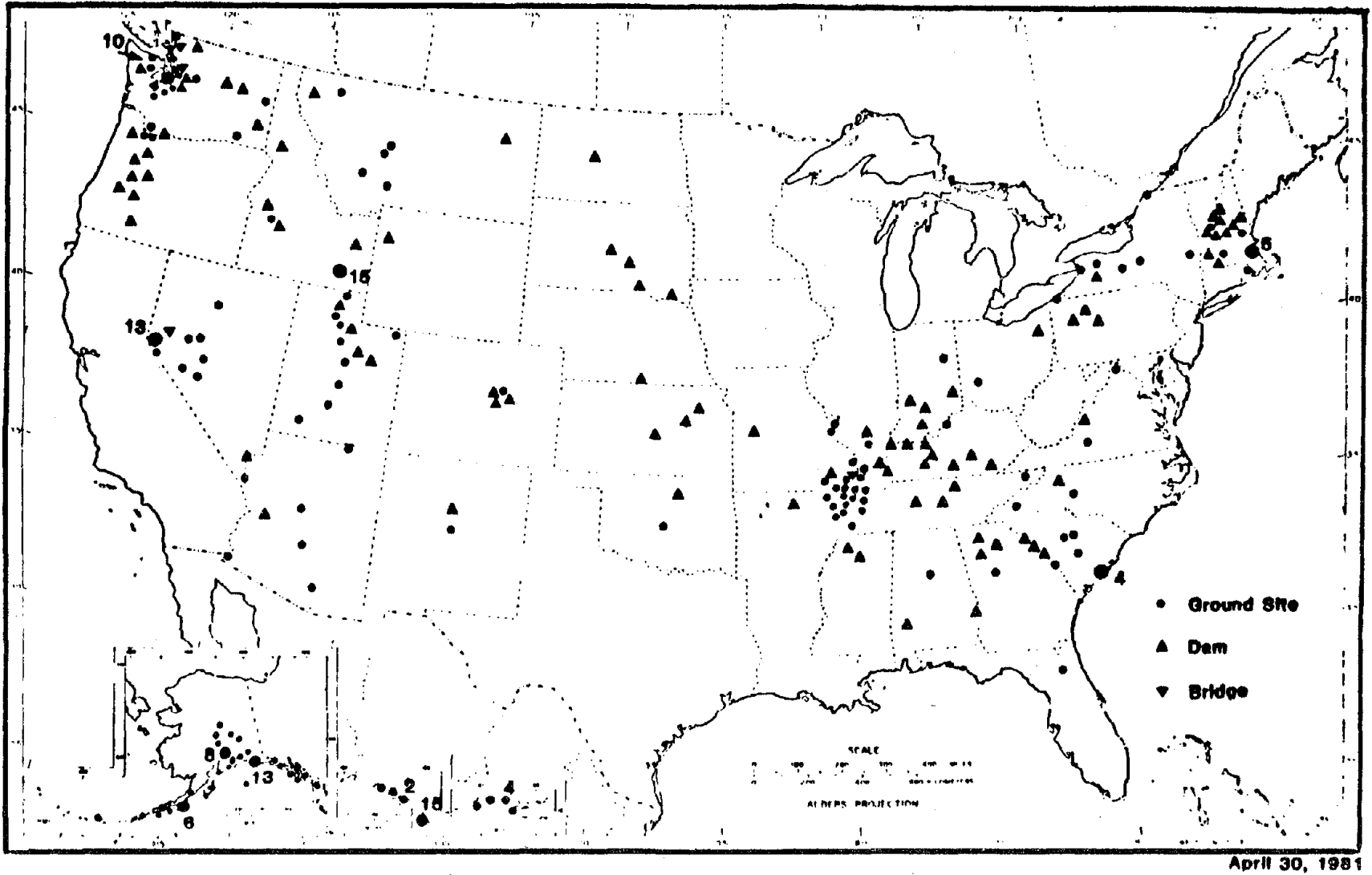
Figure 1.- Known accelerographs in the United States outside of California. Excludes commercial nuclear-powered electrical generating plants. April 30, 1981.
