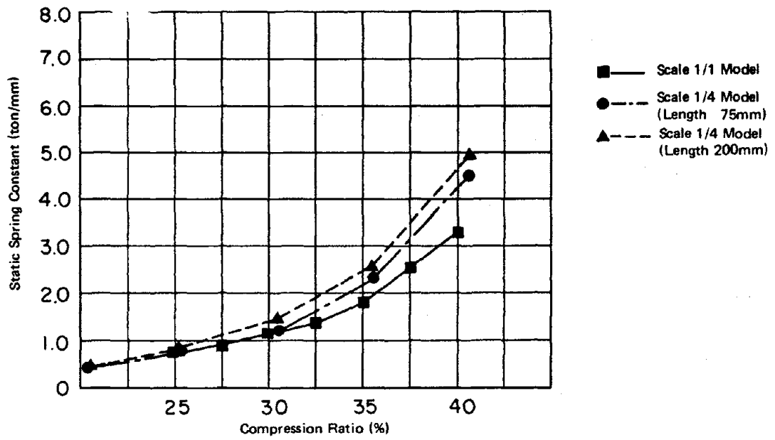
Fig. 17 Static Spring Constant
