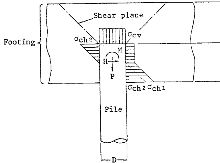
Fig. 2 Connection by Method A
