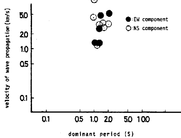
Fig. 12 Velocity of Wave Propagation
