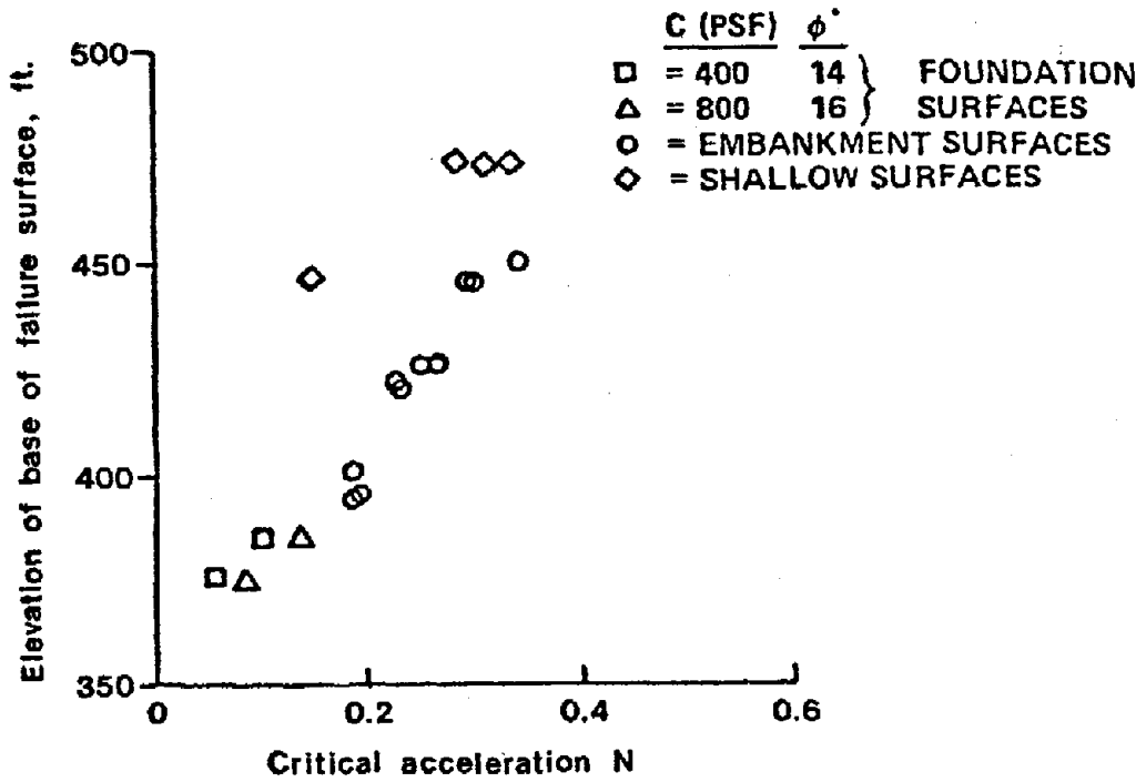
b. Critical acceleration vs. elevation
