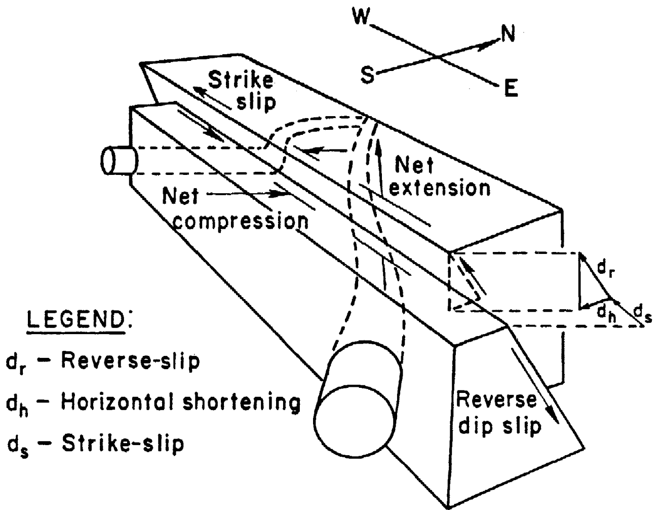
Figure 2: Block diagram of San Fernando fault motion [1].
