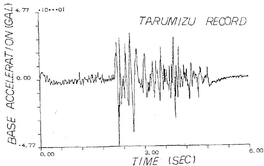
Figure 8. Time history of model no. 3
