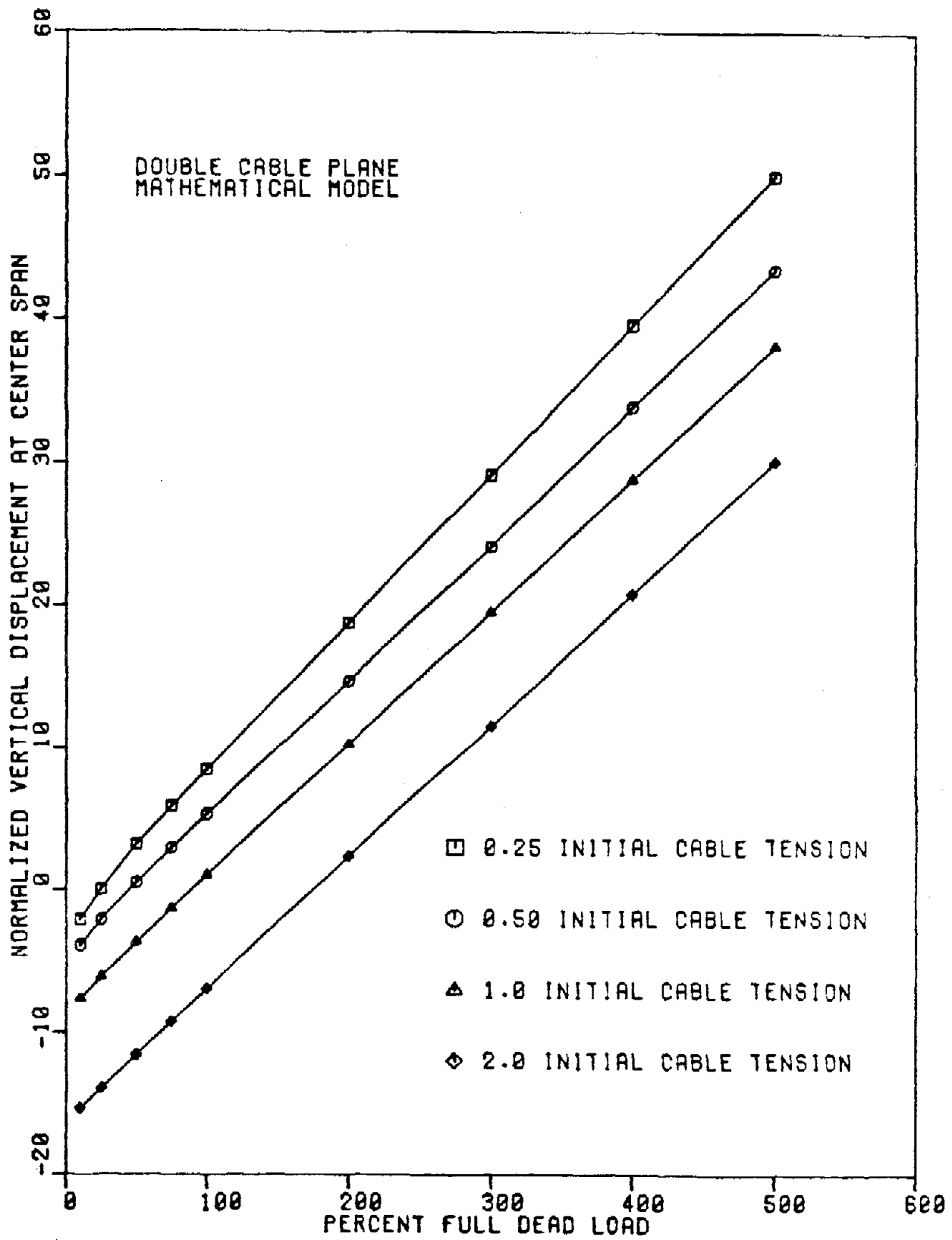
Figure 6. Effect of cable non-linearity
