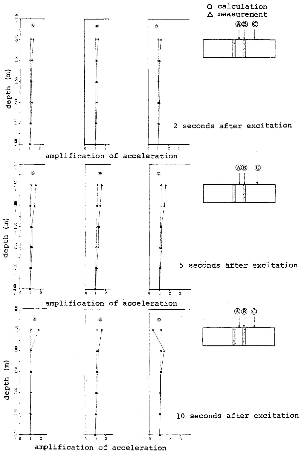
Figure 11 Amplification of acceleration
