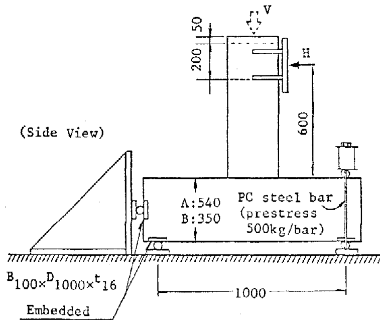
Fig. 6 Loading Method
