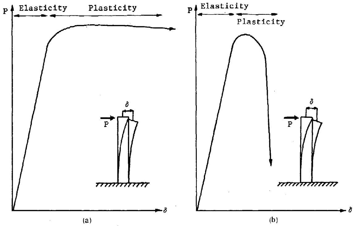
Fig. 1 Ductile and Brittle Structures
