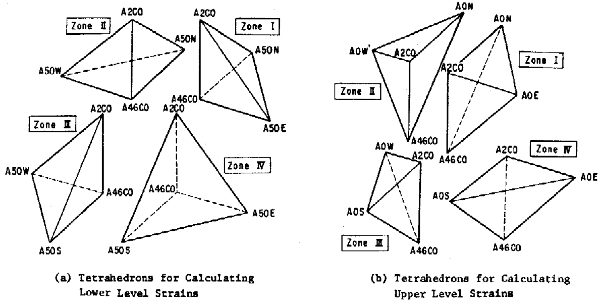
Fig. 9 Tetrahedrons Formulated to Calculate Ground Strains
