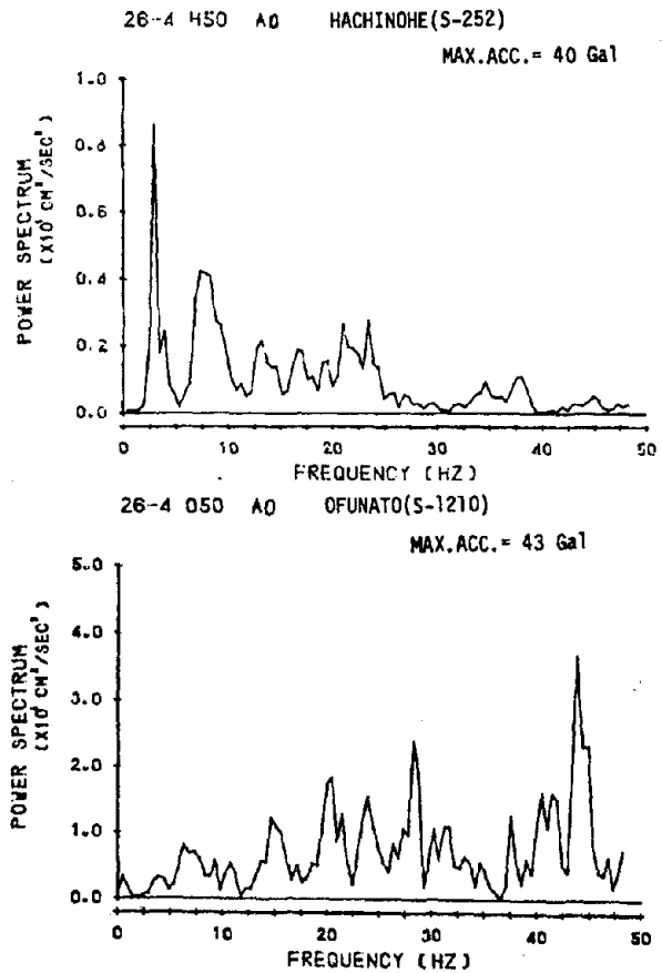
Fig. 5 Power Spectra of Earthquake Acceleration Input
