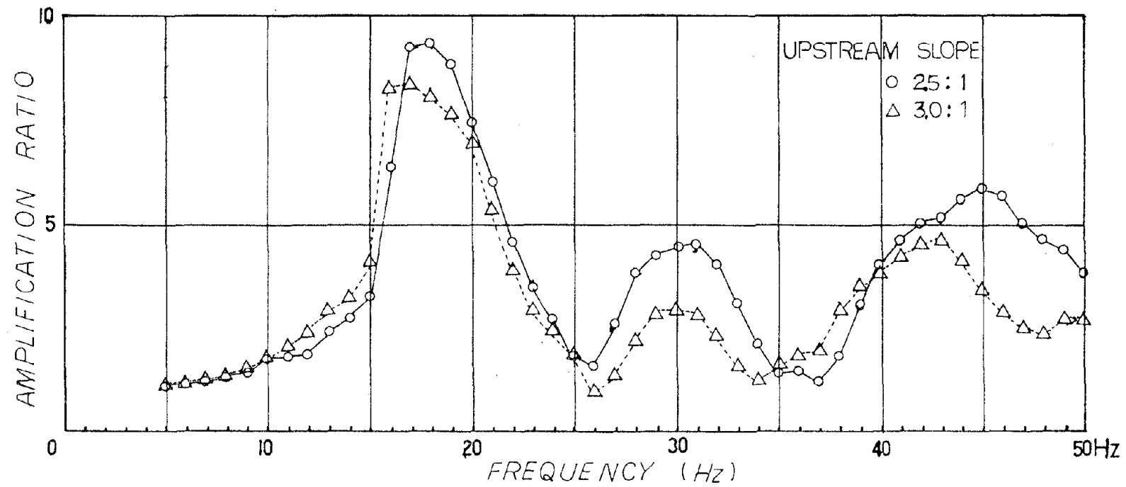
Figure 7. Effects of upstream sloping
