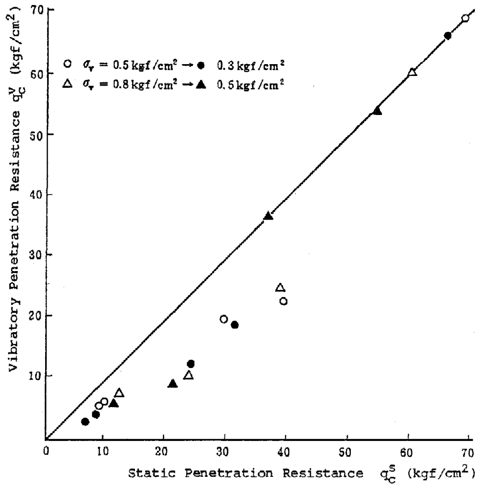
Fig. 6 Relationship of Static and Vibratory Penetration Resistance
