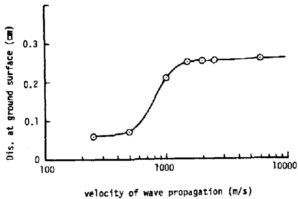
Fig. 15 Displacement at Ground Surface
