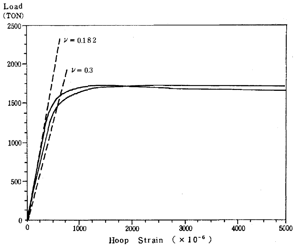
Fig. 34 Load - Hoop Strain Curve (B - 2)
