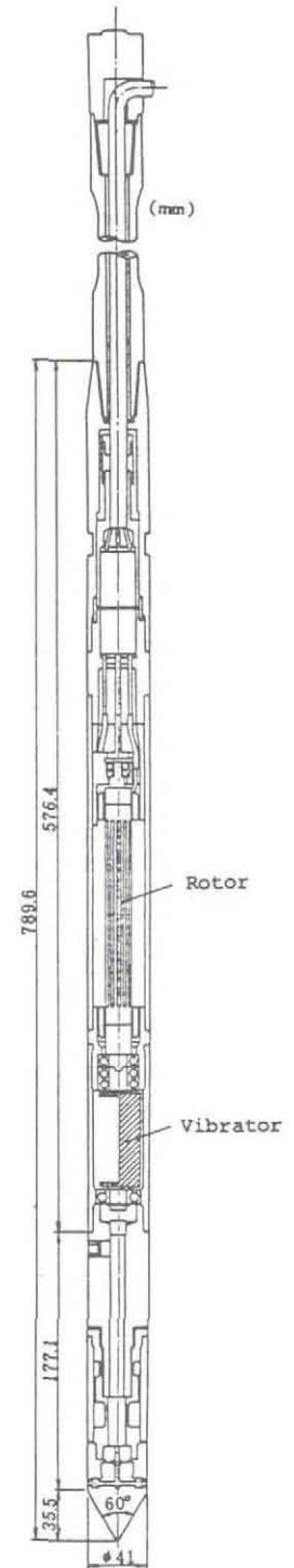
Fig. 1 Diagram of Vibratory Cone
