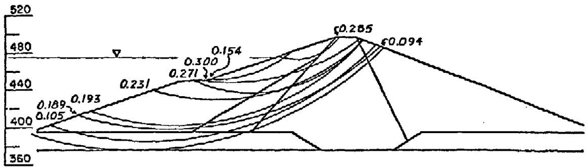
a. Critical slip surfaces
