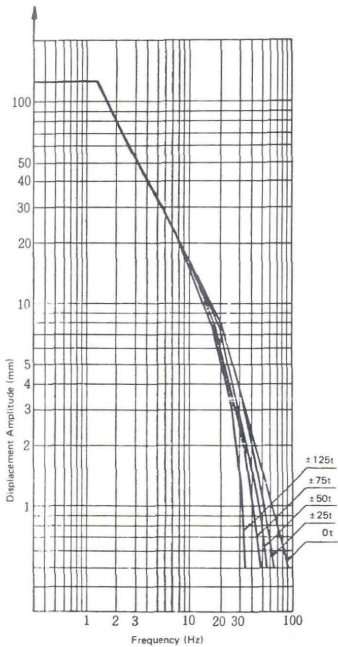
Fig. 1 Performance Curve of the Actuator
