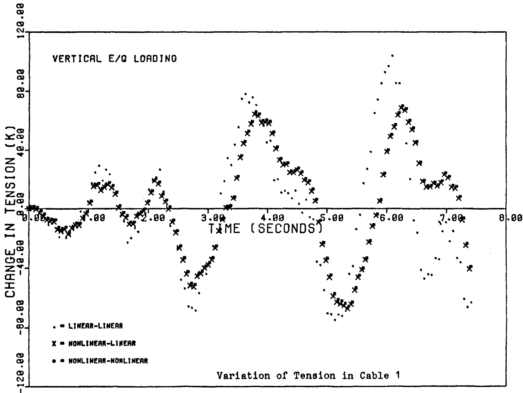
Figure 12. Variation of tension in cable
