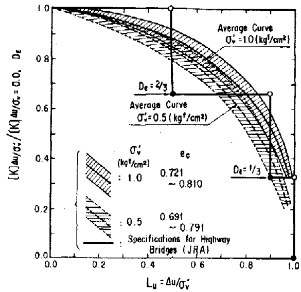
Fig. 21 Relationships between K/K_0 , D_E and L_u (= \Delta u/\sigma_v)
