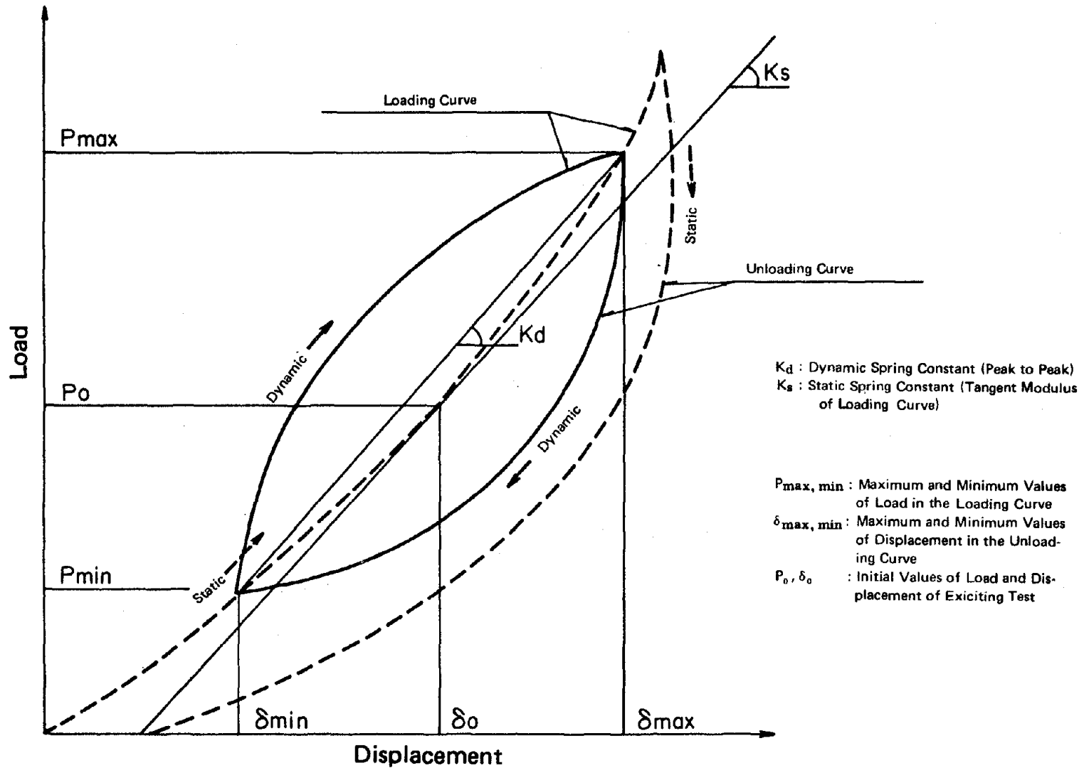
Fig. 15 Dynamic Spring Constant and Static Spring Constant
