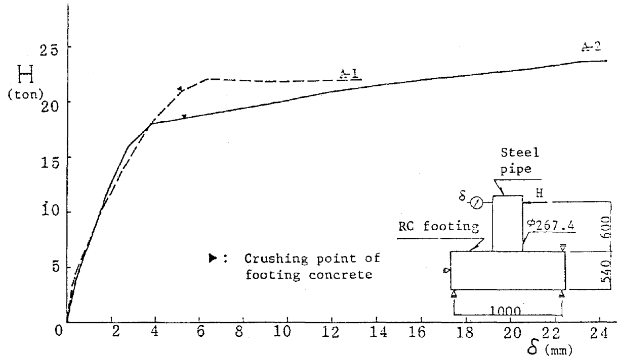
Fig. 7 Load-Deflection at Loading Point
