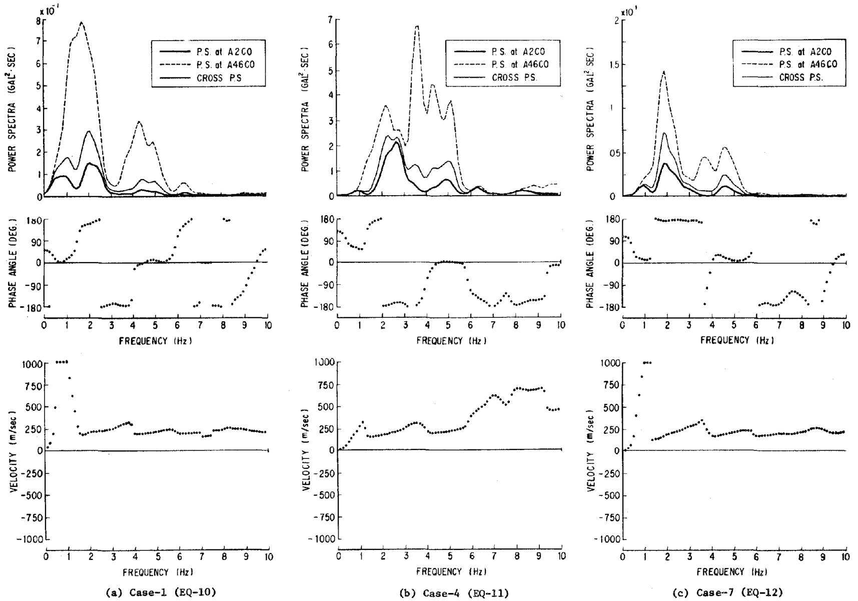
Fig. 15 Power Spectra S_{mm} , S_{nn} and S_{mn} , Phase Angle \theta_{mn} and Apparent Velocity V_{mn} in Vertical Direction between A20C0 and A46C0 at A-Field of Local Laboratory Array of PWRI Compus
