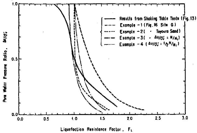
Fig. 17 Relationships between \Delta u/\sigma'_v and F_L
