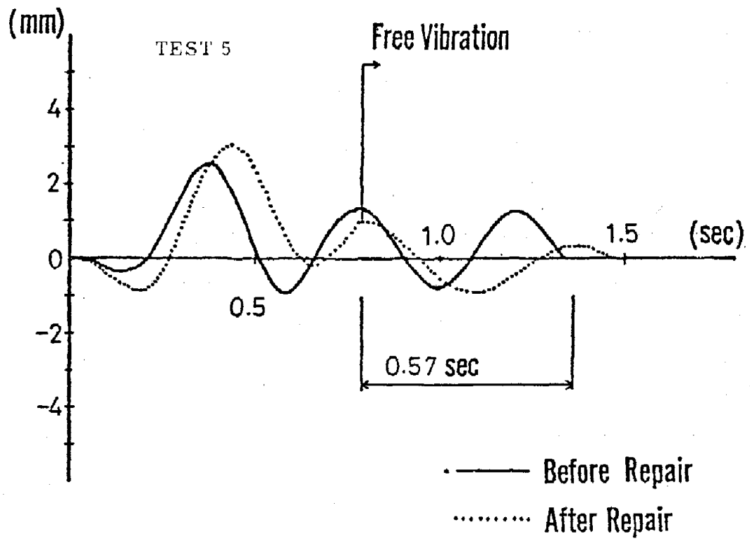
Fig. 5 Response Time History
