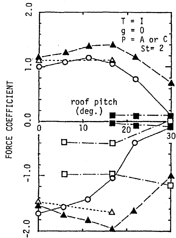
Fig. 14 Variation of maximum and minimum force coefficient with roof pitch □--- mounting pattern (a), \blacksquare --- (b) \Delta --- (c), \circ — (d), \blacktriangle — (e)
