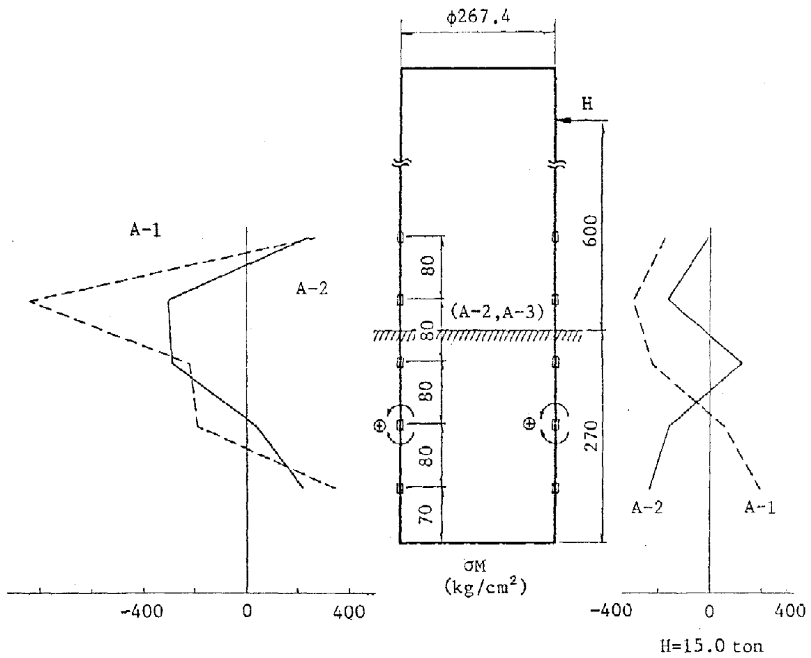
Fig. 11 Distribution of Bending Stress on Steel Pipe
