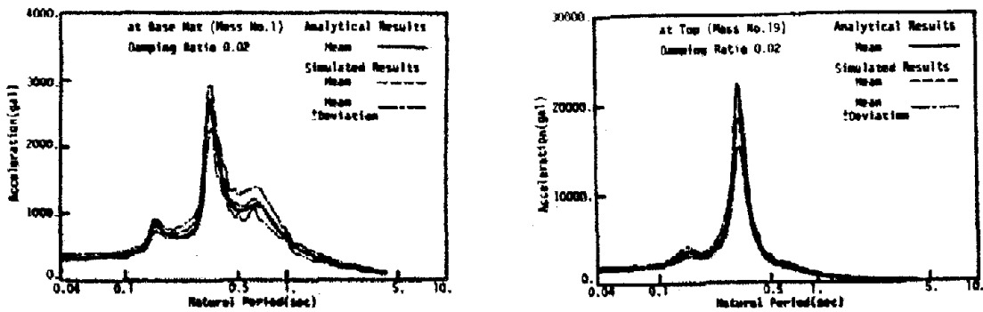
Fig.7 Floor Response Spectra
