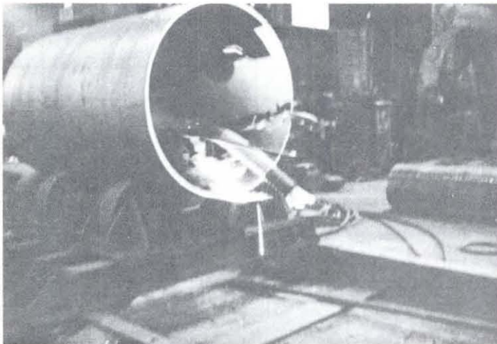
Photo-2. Welding (Inside)
