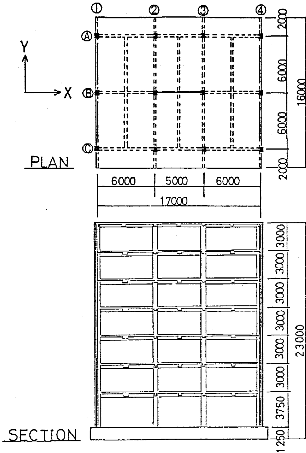
Fig. 1 Plan, Elevation, and Dimension of the Specimen
