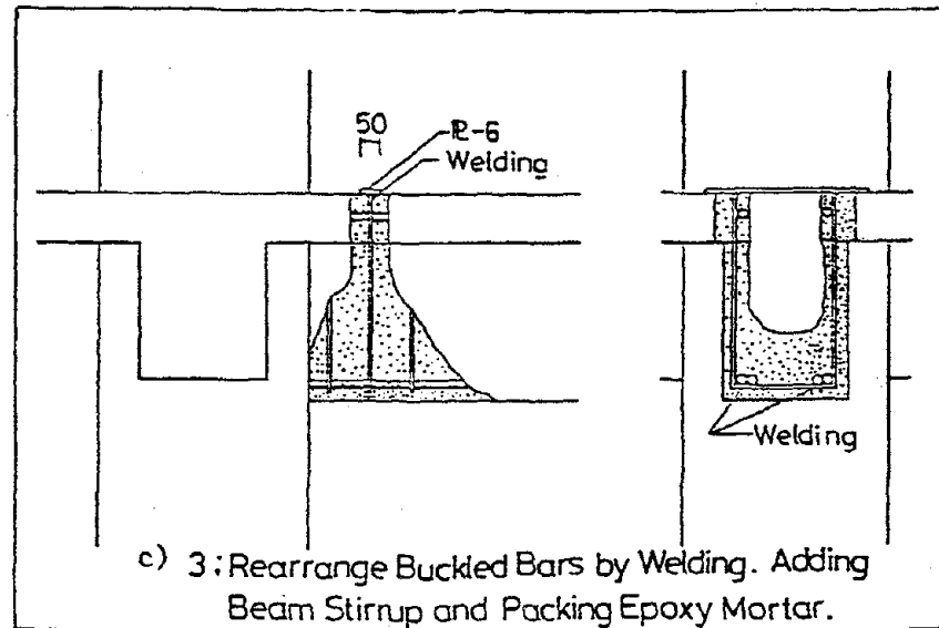
Fig. 2 Details of Repair Works at Beam End
