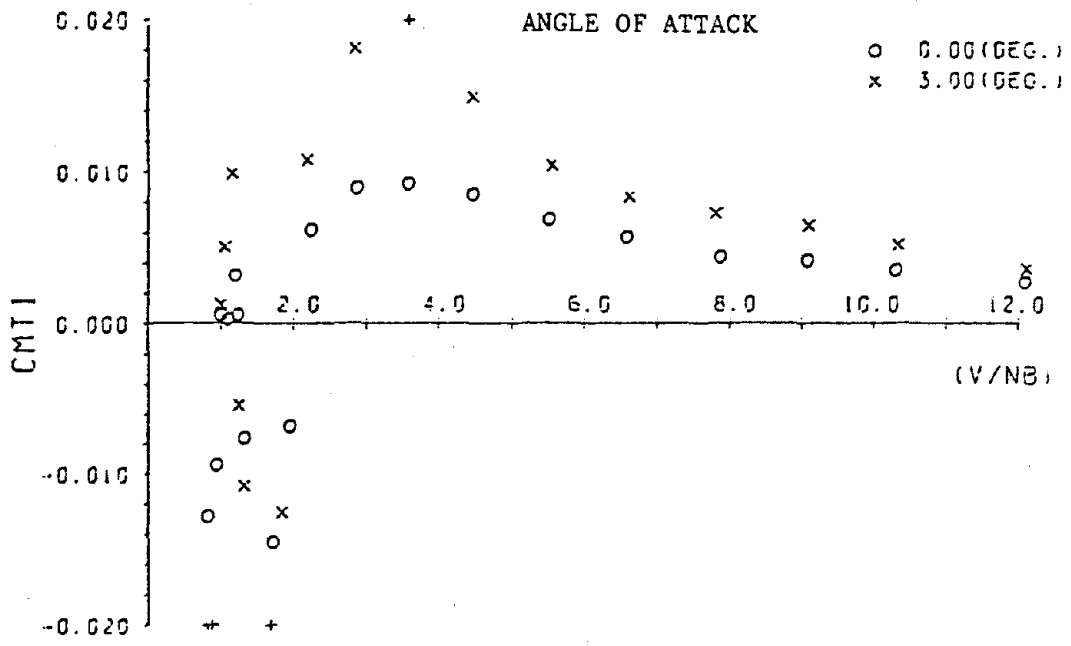
Fig.4-19 C_{MT}^I - V/NB (Model No.17)
