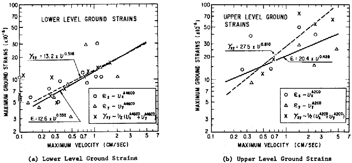
Fig. 10 Relation between Ground Strain and Particle Velocity
