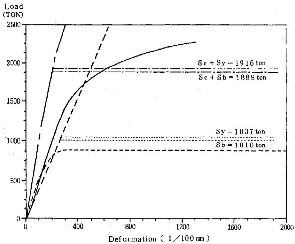
Fig. 15 Load - Deformation Curve (B - 4)
