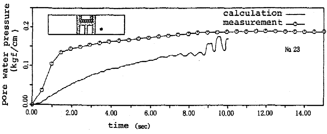
Figur 14 Comparison of pore water pressure (model 10)
