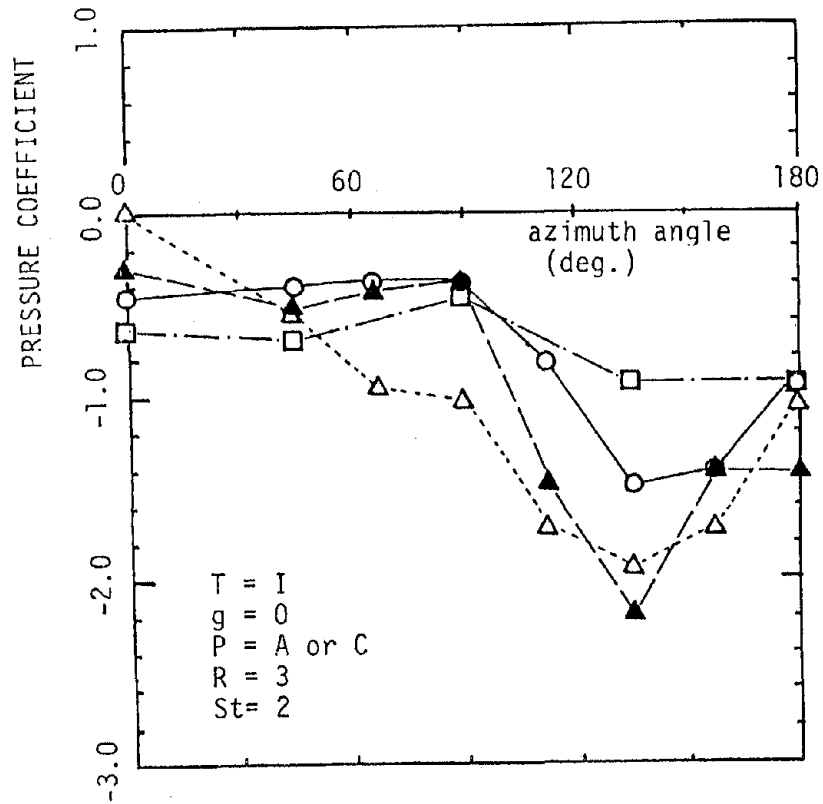
Fig. 11 Variation of upper wind pressure coefficient with azimuth angle □---mounting pattern (b), △----(c), ○—(d), ▲--(e)
