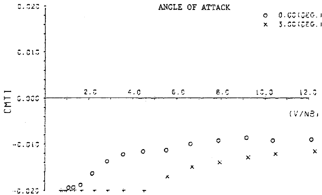
Fig.4-14 C_{MT}^I - V/NB (Model No.2)
