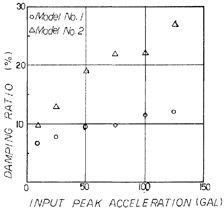
Figure 6. Average damping ratio
