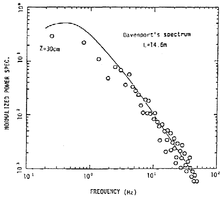
Fig. 8 Power spectrum of turbulence at z=30cm
