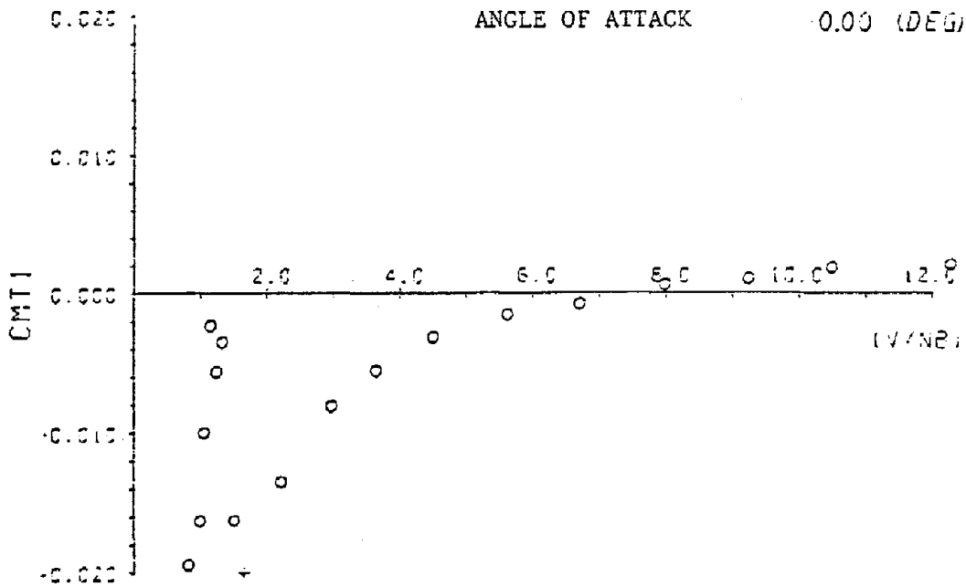
Fig.4-12 C_{MT}^I - V/NB (Model No.14)
