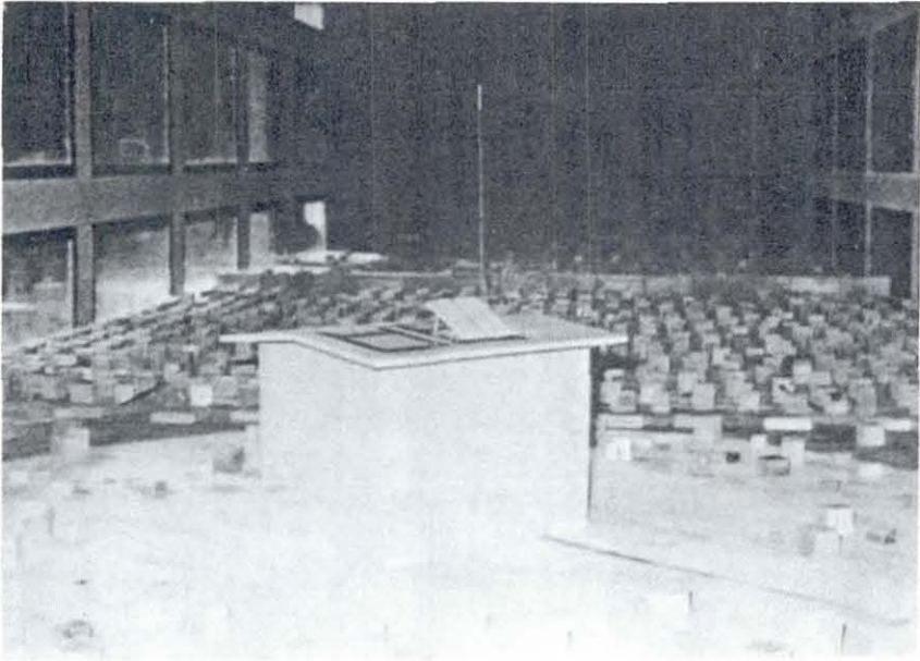
Photo 1 View of a wind tunnel model
