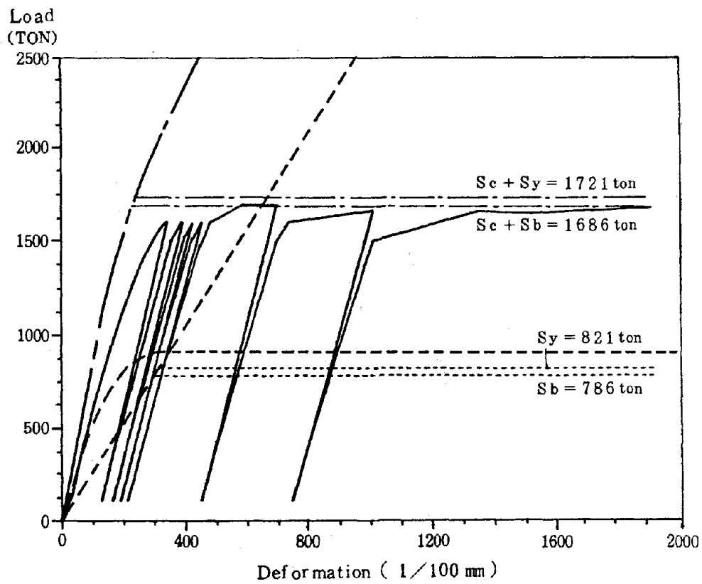
Fig. 16 Load - Deformation Curve (B - 5)
