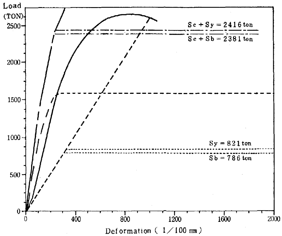
Fig. 17 Load - Deformation Curve (B - 6)
