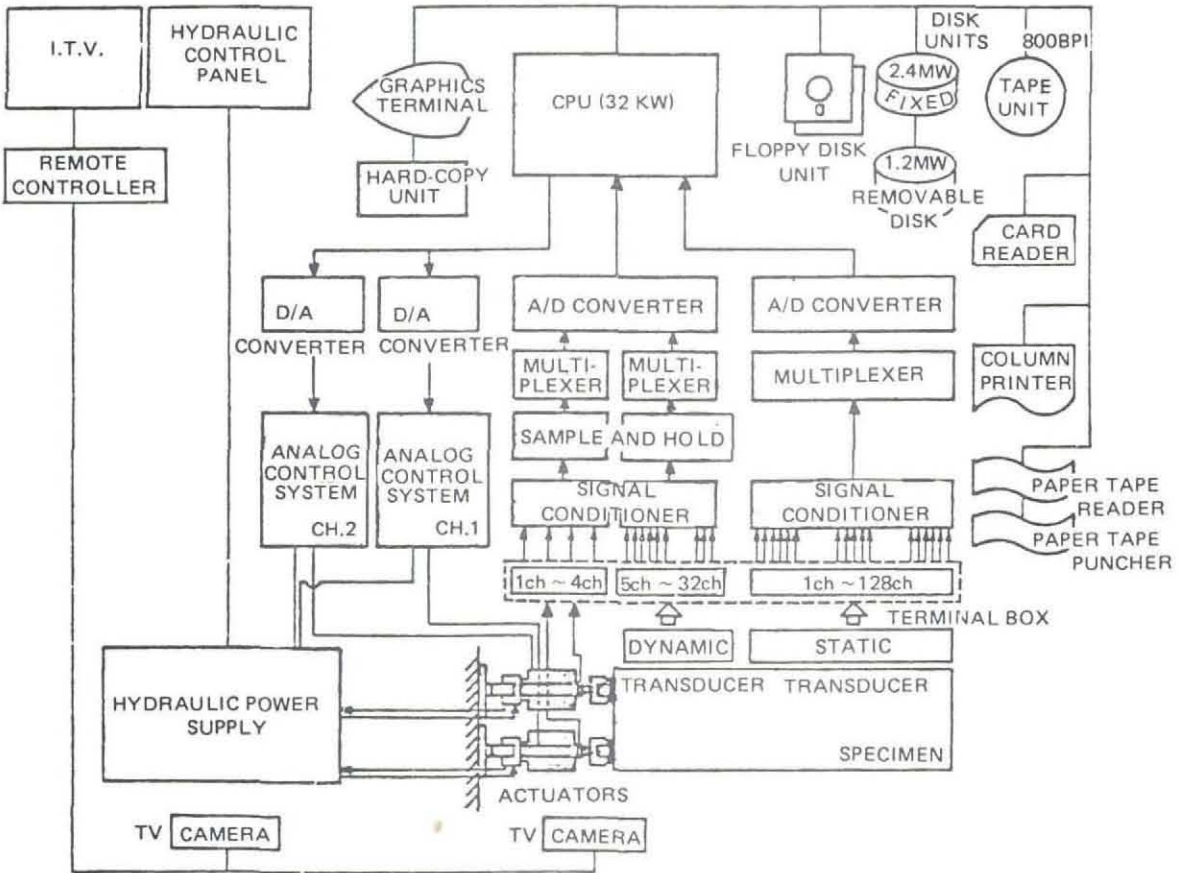
Fig. 9 Control System Diagram
