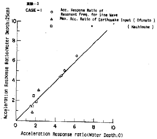
Fig. 12 Effects of Water on Acceleration Response Curve
