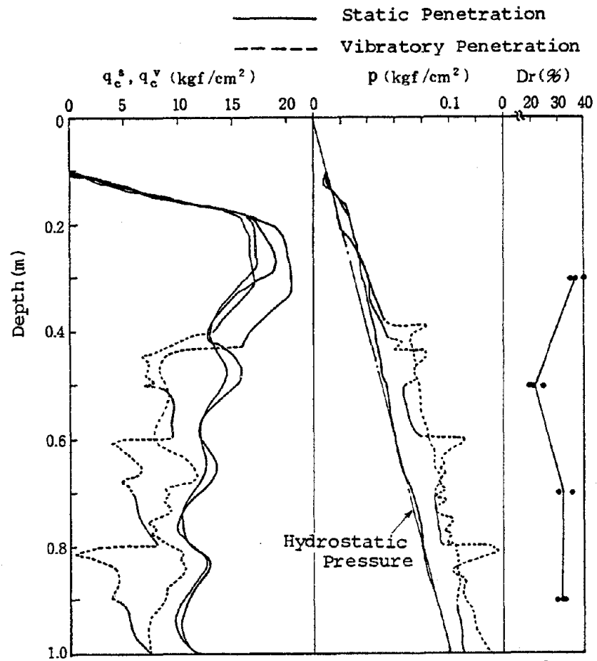
Fig. 4 Example of Penetration Test Result (Loose Condition)
