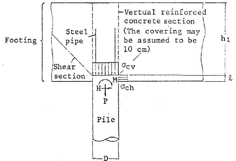
Fig. 3 Connection by Method B
