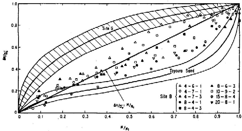
Fig. 16 Relationships between \Delta u / \sigma'_v and N / N_L
