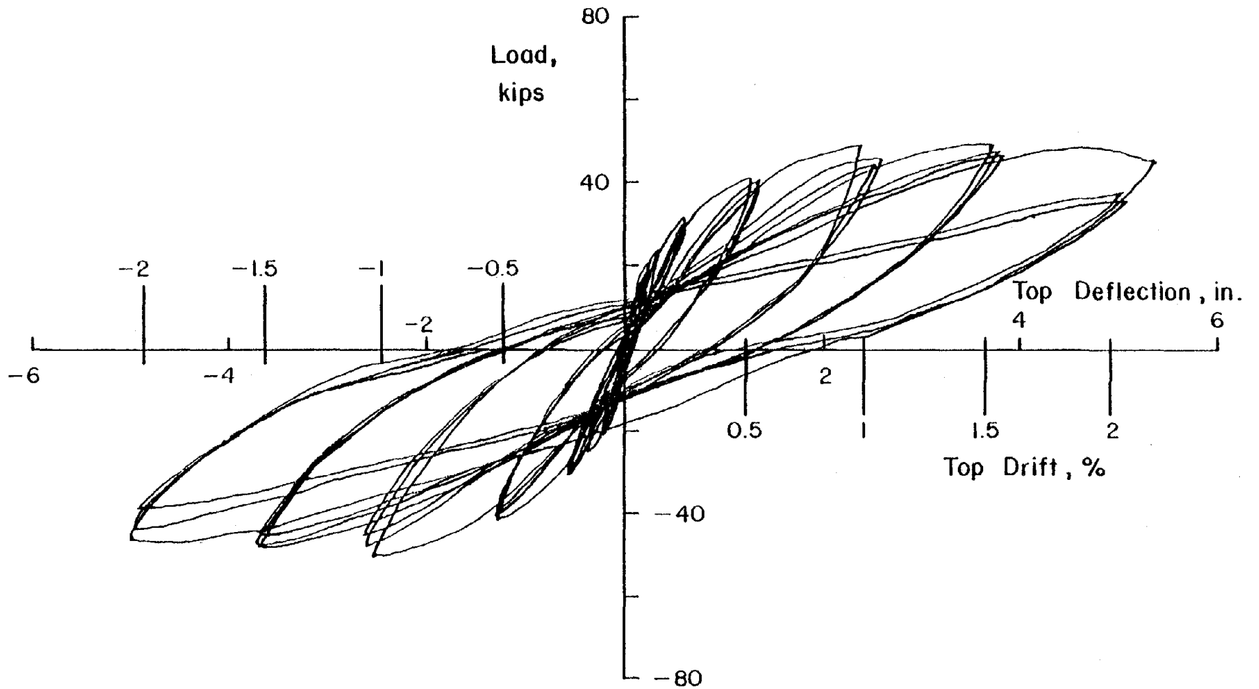
Fig. 4 Load versus Top Deflection, Wall-Frame Specimen
