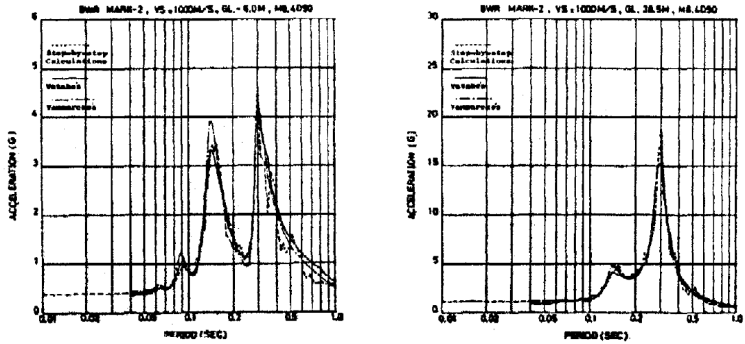
Fig.15 Floor Response Spectra (Damping Ratio 1%); V_s=1000m/sec , Magnitude 8.4 and Epicentral Distance 90km
