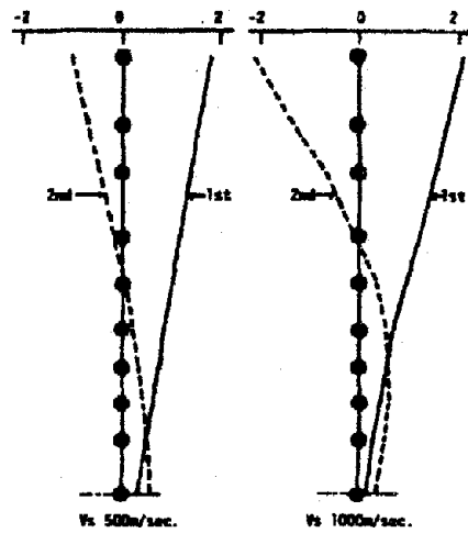
Fig.10 Eigen Vectors multiplied by Participation Factor
