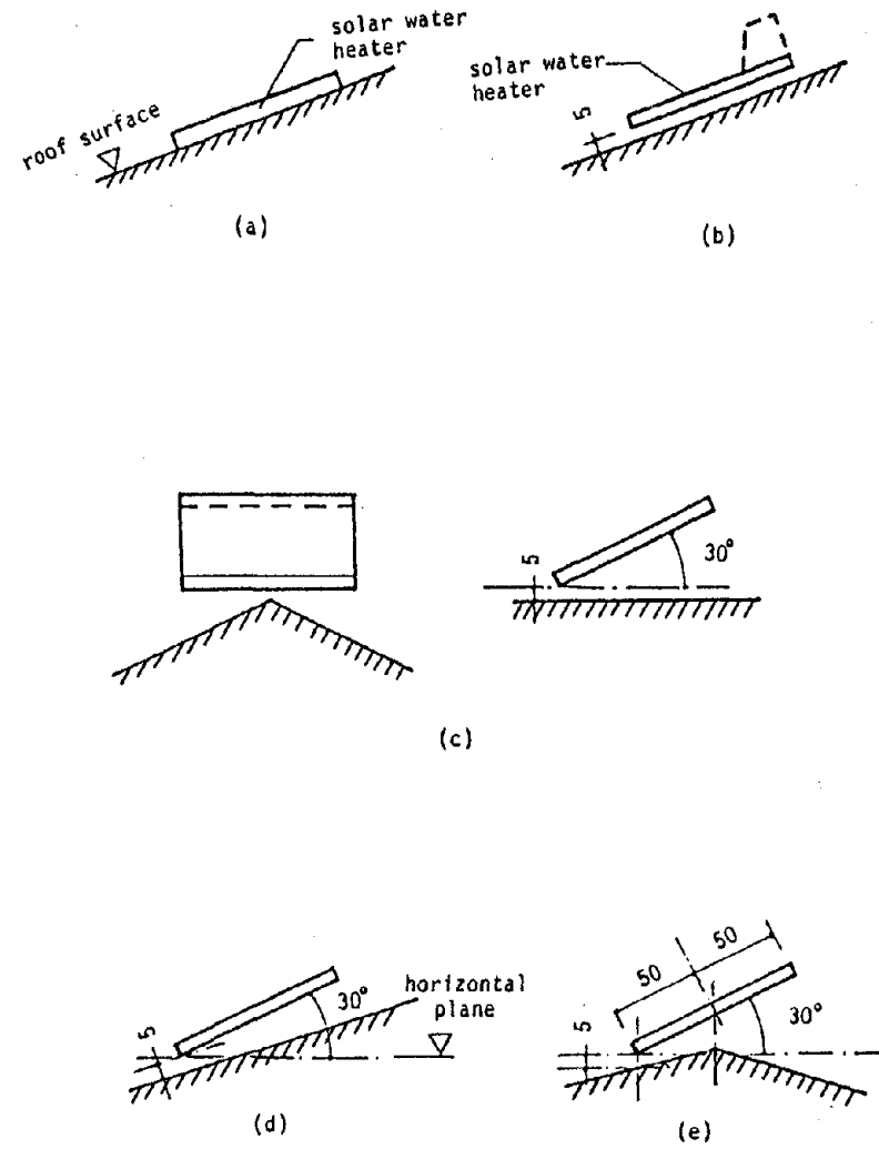
Fig. 5 Mounting pattern
