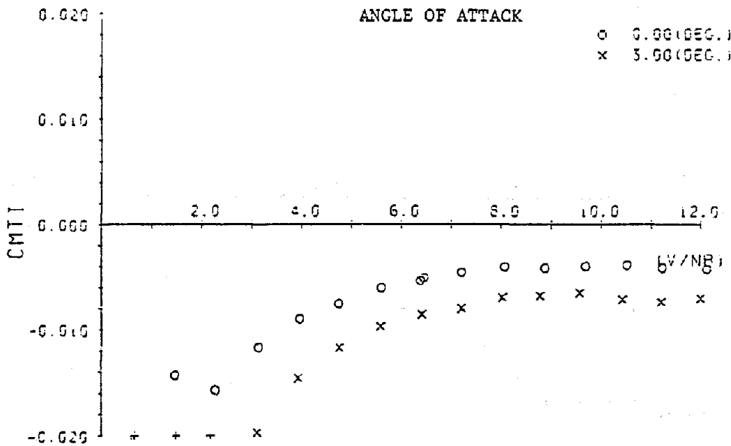
Fig.4-6 C_{MT}^I - V/NB (Model No.8)
