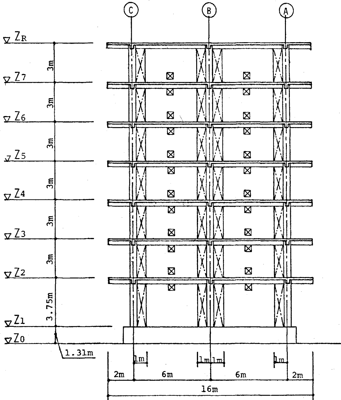
Fig. 3. Elevation, Frame 4
