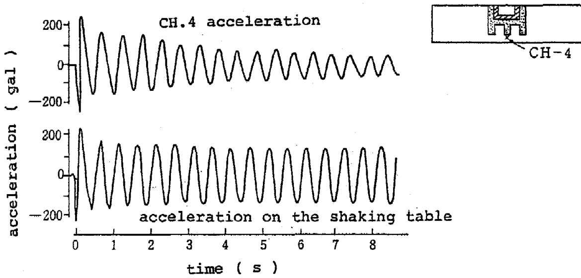
Figure 3 Example of acceleration record (model 11)
