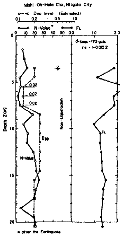
Fig. 2 Relationships between F_L and Depth
