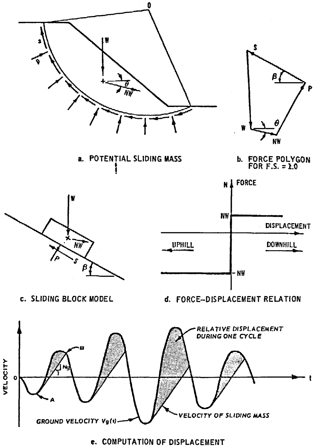
Figure 5. Elements of the Newmark sliding block analysis
