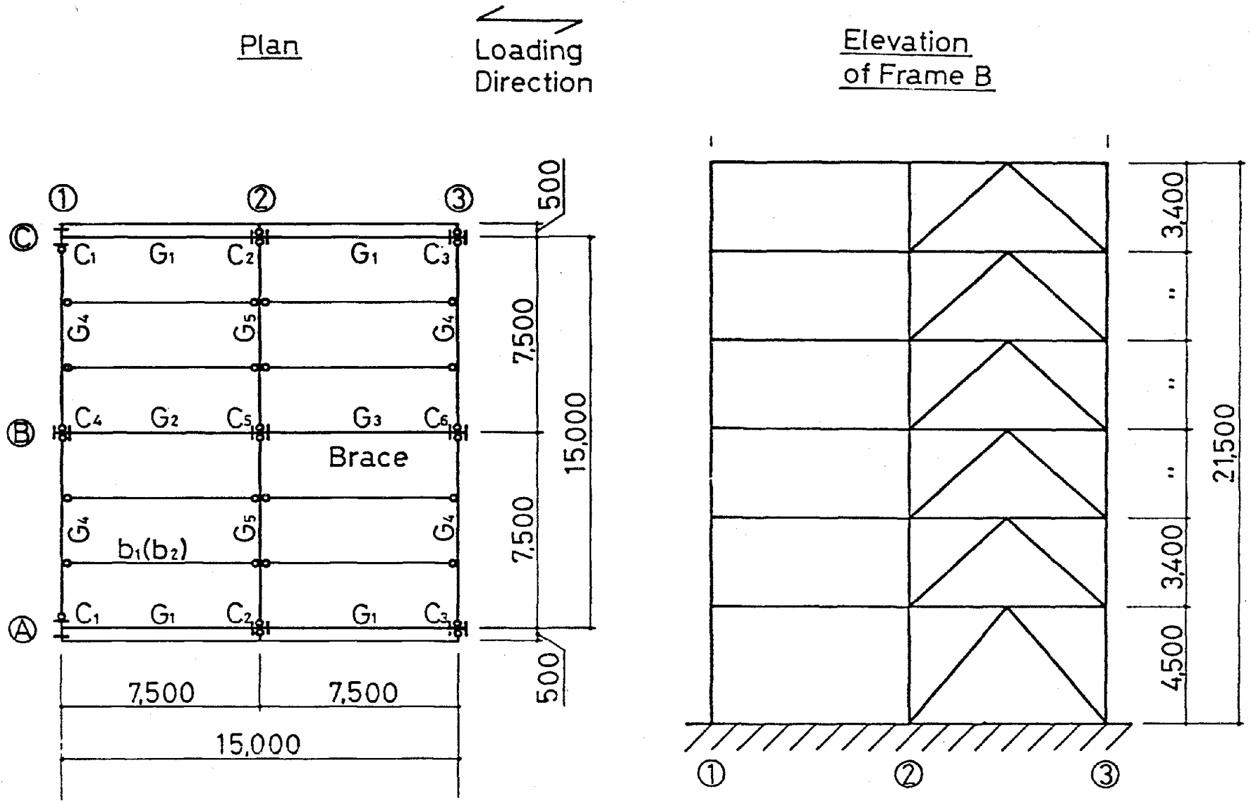
Fig. 3-1 Plan and Elevation of a Full-Scale Six-Story Steel Building
