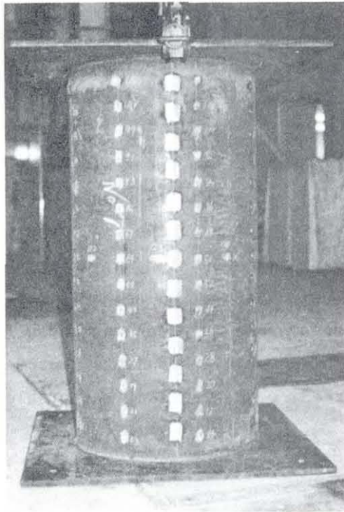
Photo-15. Speimen B - 6 After Loading
