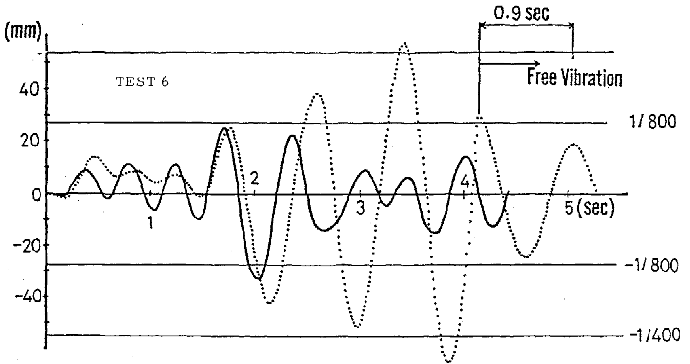
Fig. 7 Response Time Hystory
