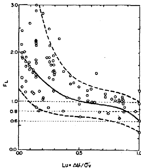
Fig. 11 Relationships between Pore Water Pressure and Acceleration of Non-Liquefied Sand Layers and F_L Values in Shaking Table Tests
