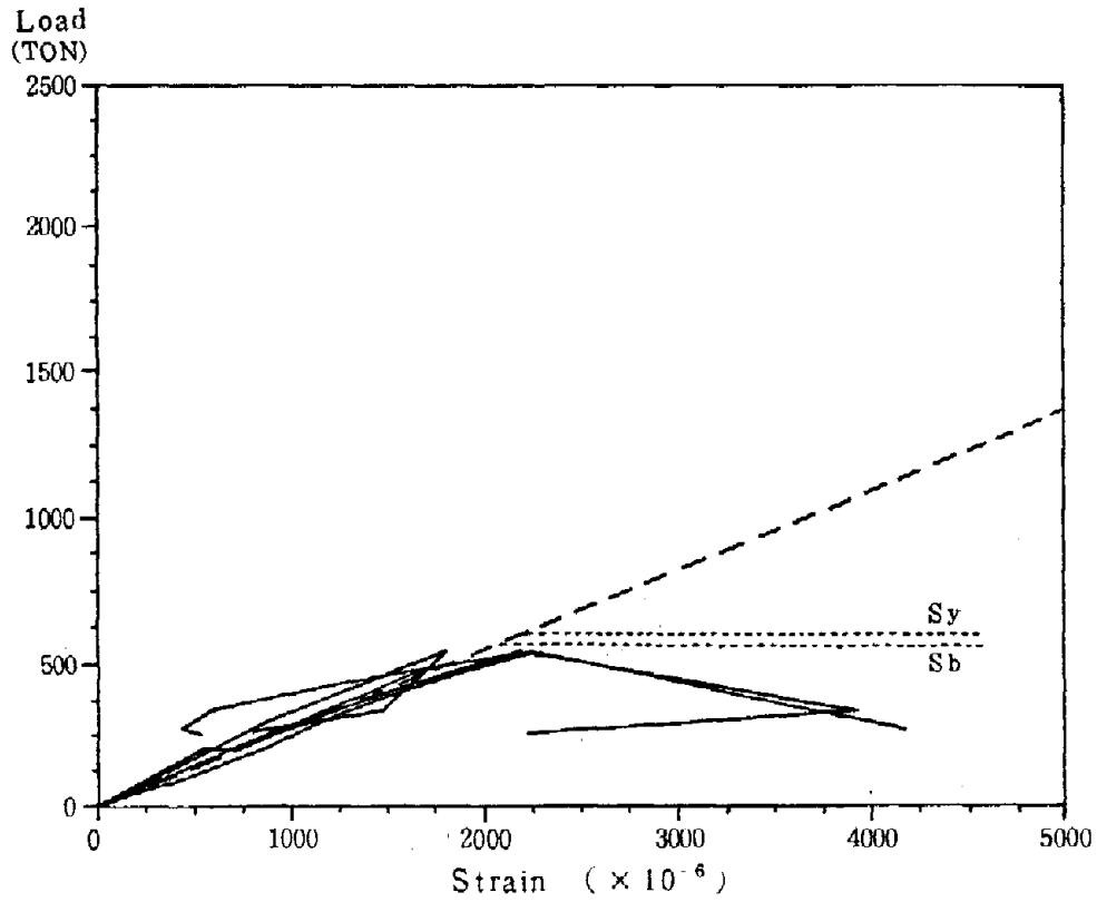
Fig. 18 Load - Strain Curve (A - 1)
