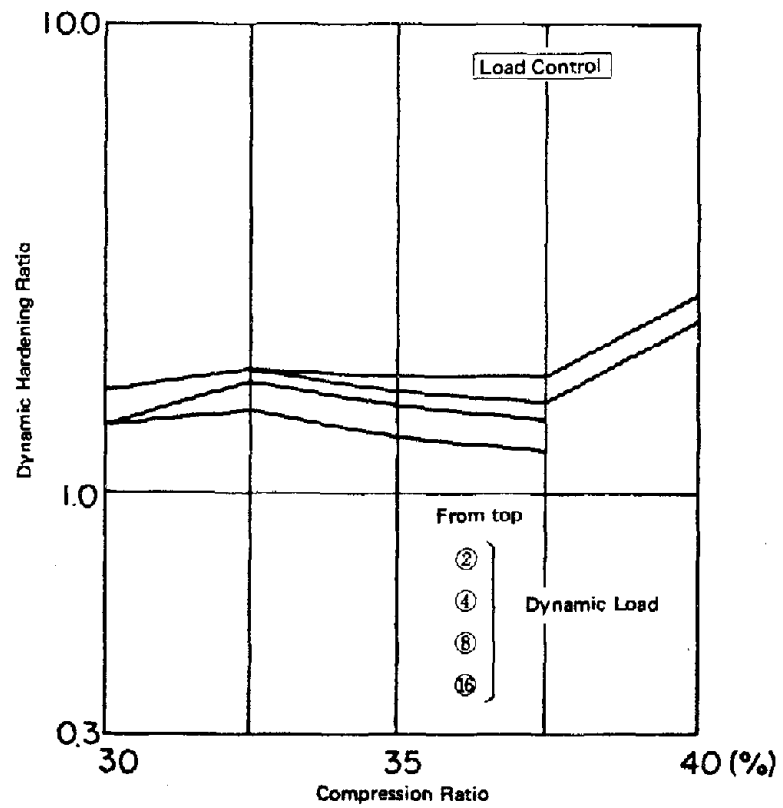
Fig. 20 Dynamic Hardening Ratio
