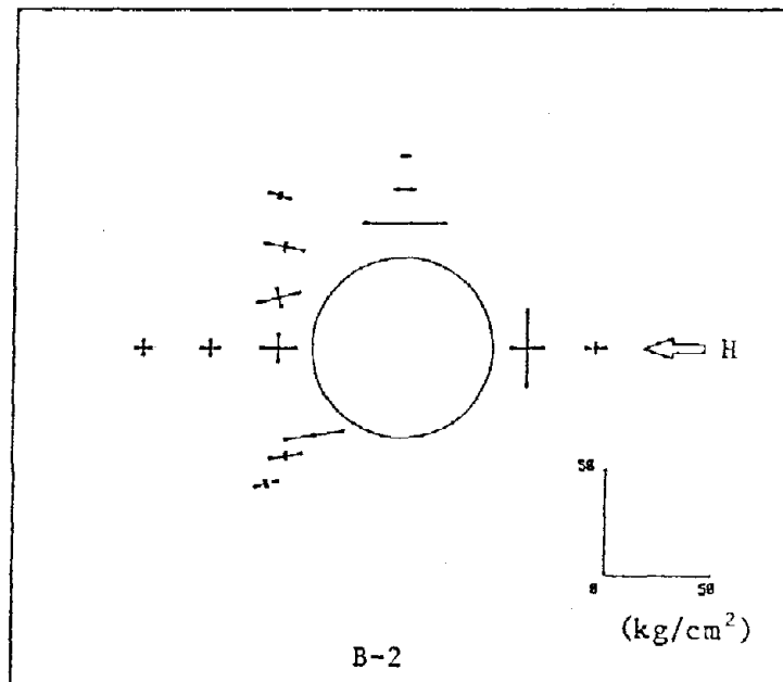
Fig. 10 Distribution of Stress on Footing Surface
