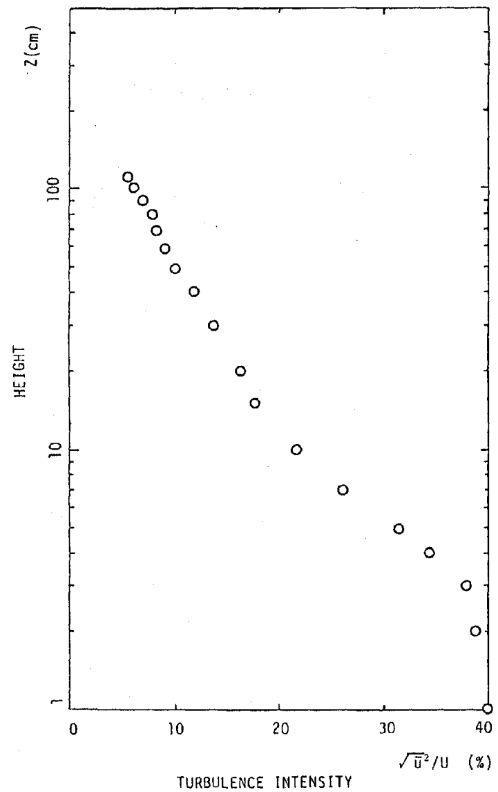
Fig. 7 Turbulence intensity profile
