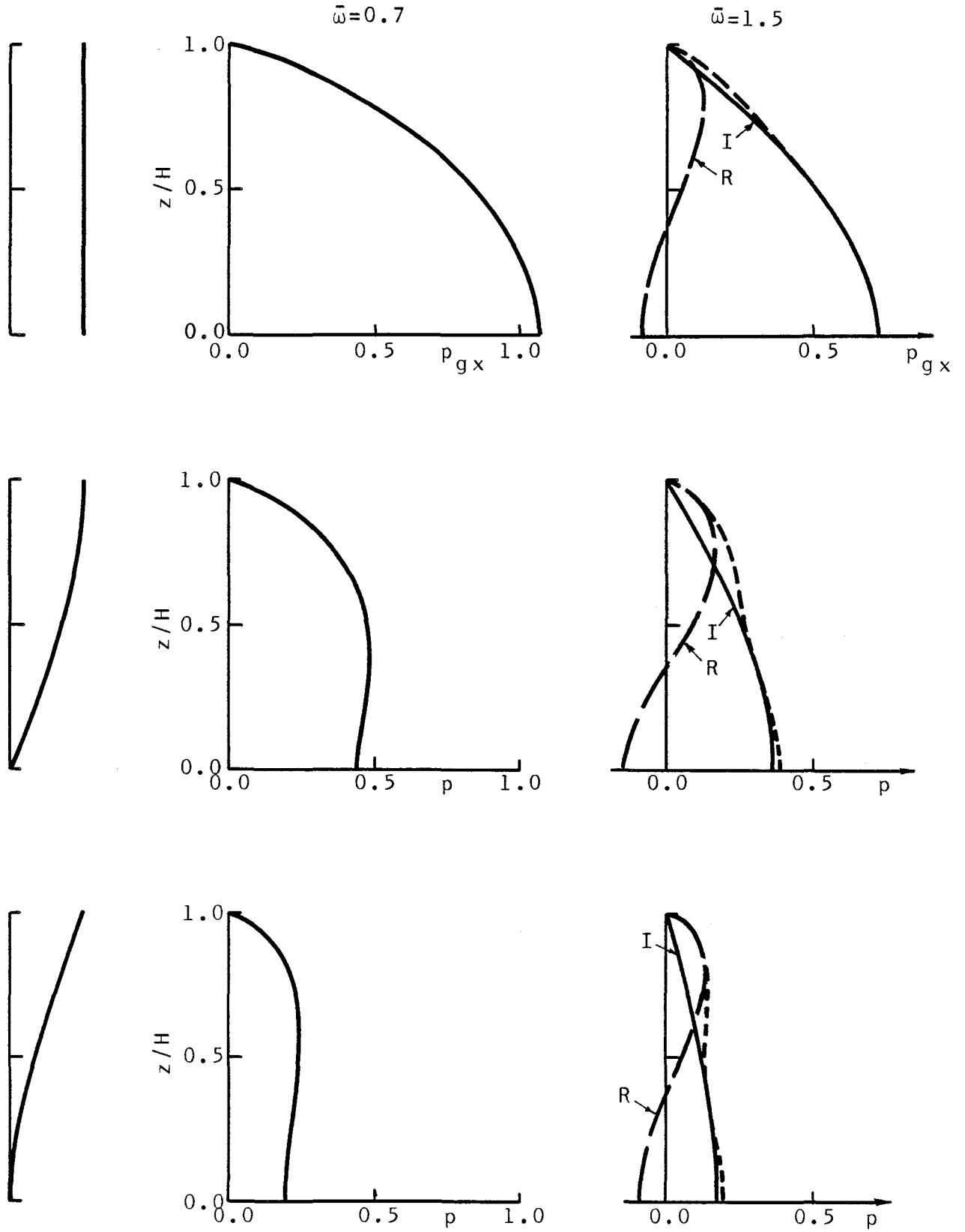
Fig. 2.5 Prescribed Motion and Hydrodynamic Pressure Distribution
