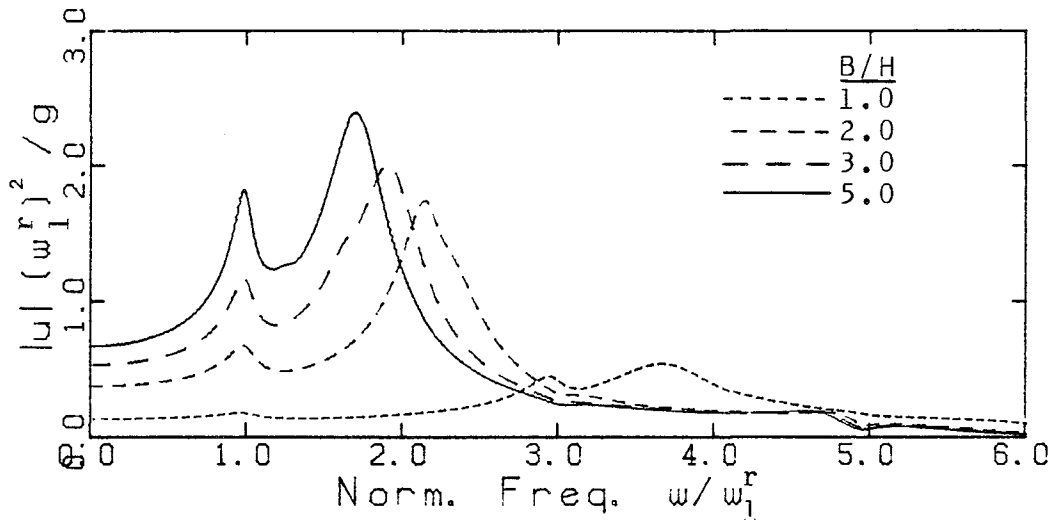
(a) Longitudinal Ground Motion
