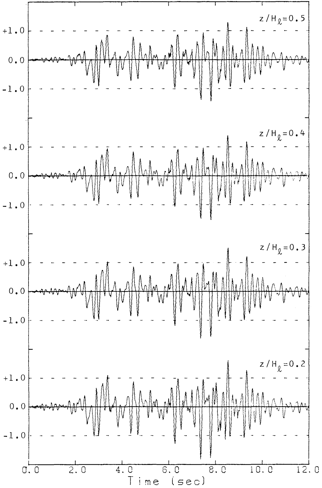
Fig. 5.12 Time Histories of Normalized Hydrodynamic Pressure (continued)
