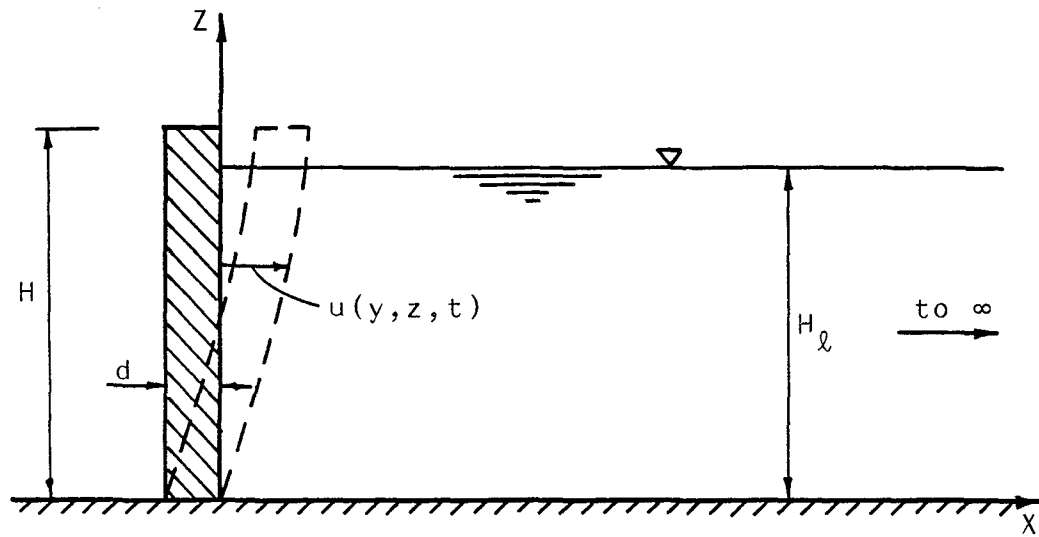
(a) Sectional Elevation
