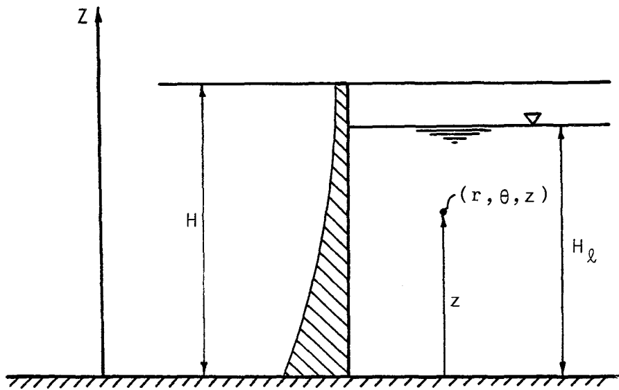
(a) Sectional Elevation
