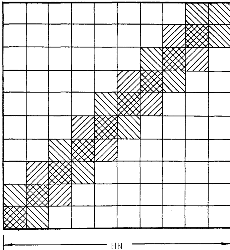
General Form of the "Banded" Mass or Stiffness Matrix
