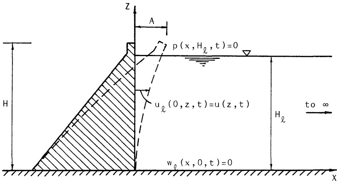
Fig. 2.2 Vibrational Motion
