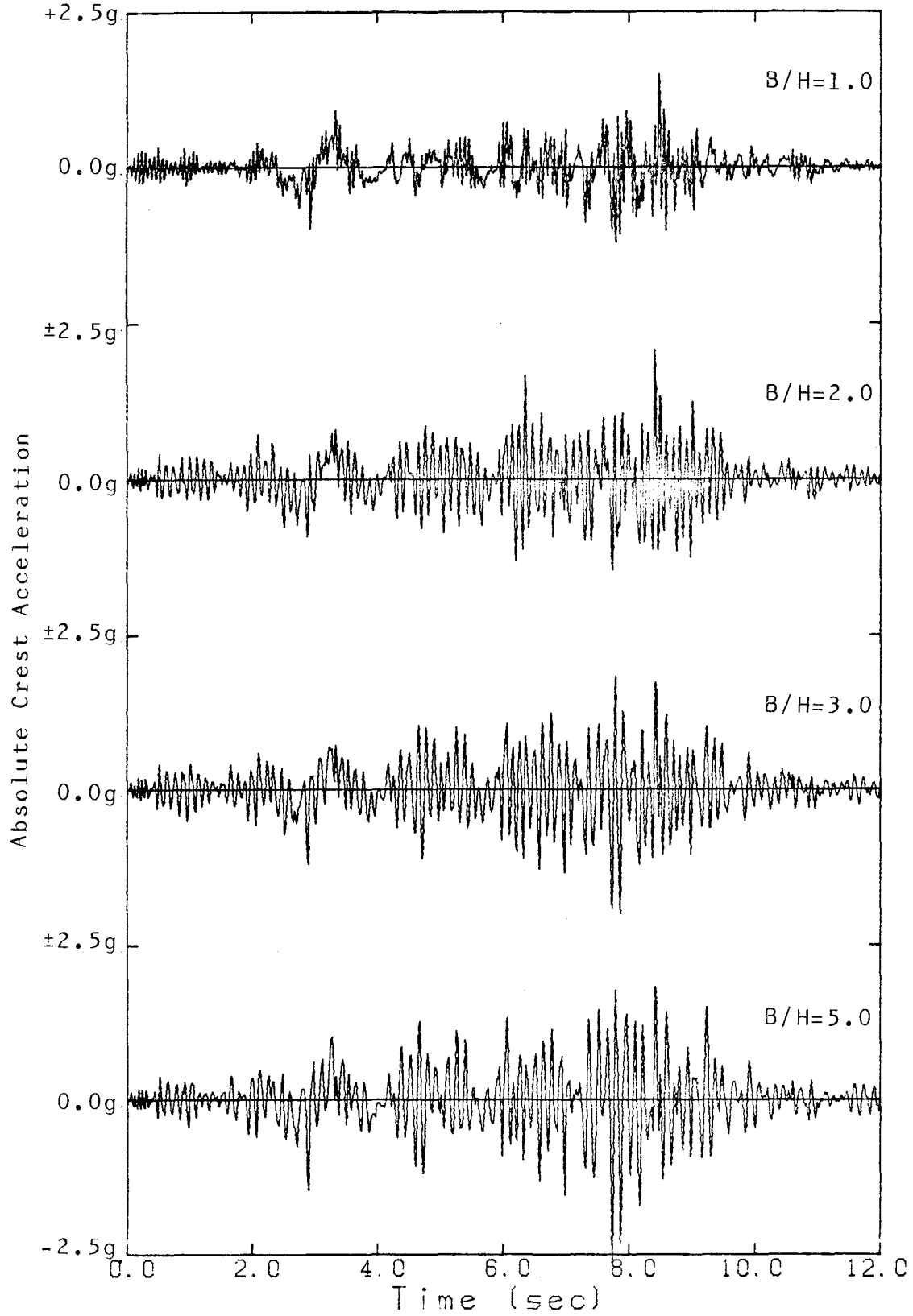
Fig. 5.5 Time Histories of Absolute Crest Acceleration (Longitudinal Ground Motion)
