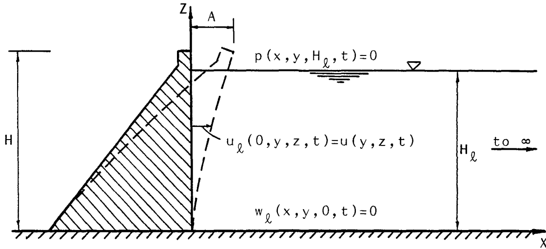
(a) Sectional Elevation
