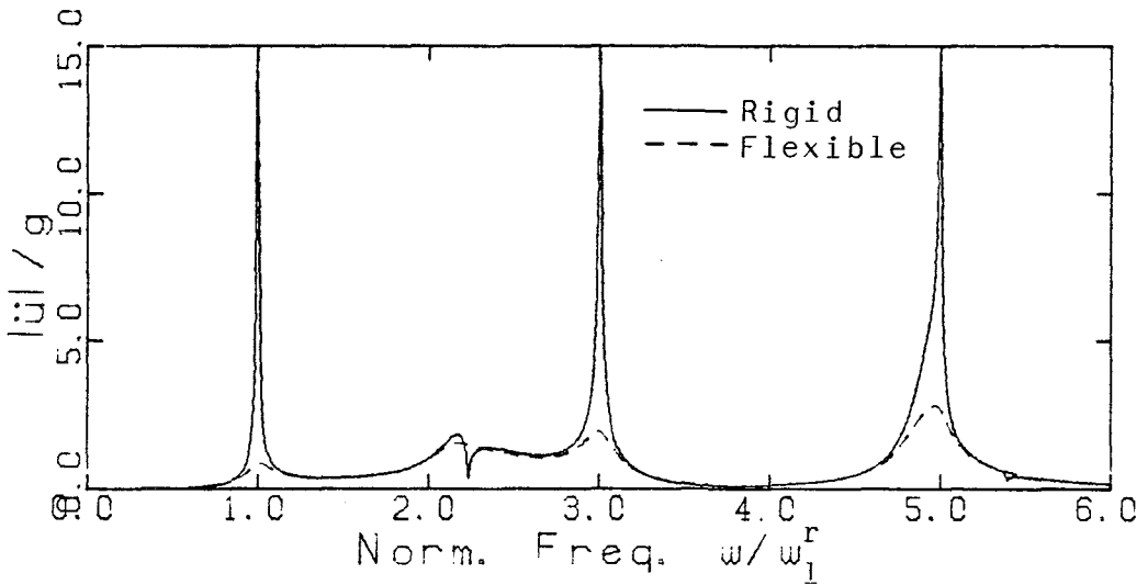
(c) Vertical Ground Motion
