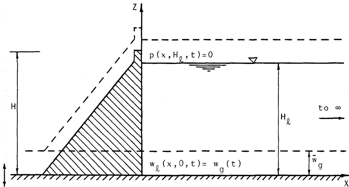
Fig. 2.4 Vertical Ground Motion
