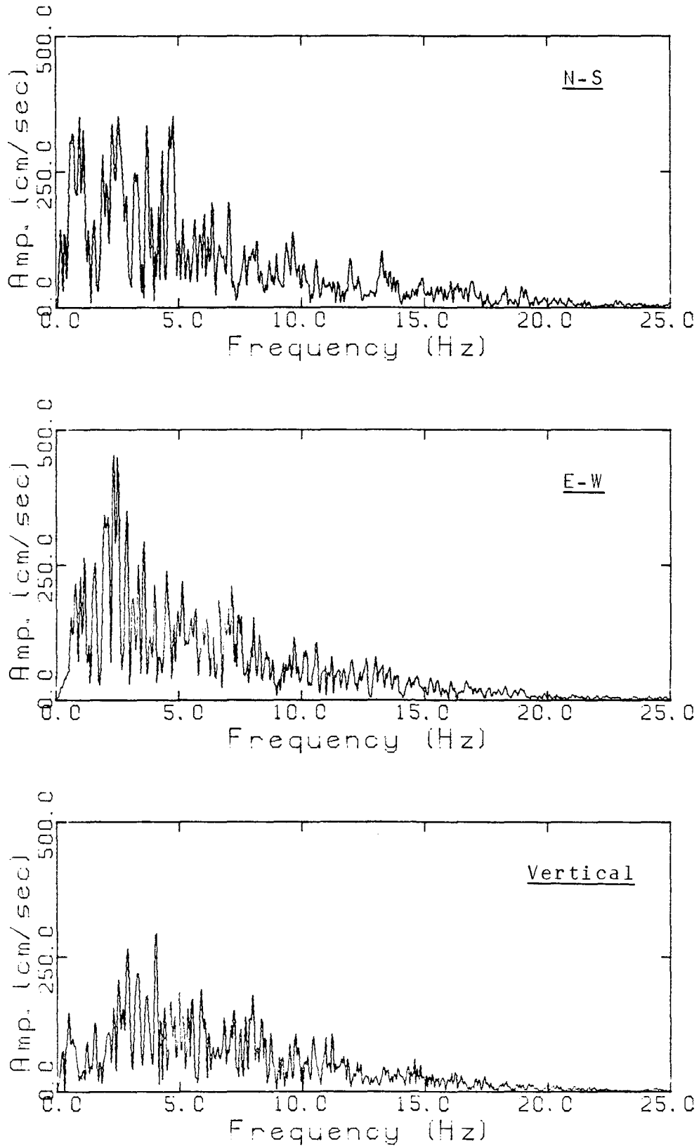
Fig. 5.3 Fourier Amplitude Spectra (Pacoima Dam Record)
