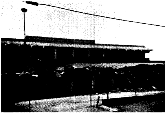
Figure 1-5 (above) Shear failure of columns and joints led to the complete collapse of the roof of the parking garage at the Whittier Quad.
