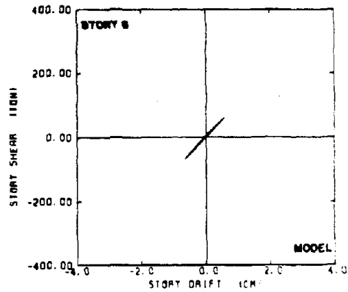
Fig. 6.21 (continued) Comparison of Hysteresis Behavior from the Inelastic Pseudo-Dynamic Test and the Optimal Hysteretic Model
