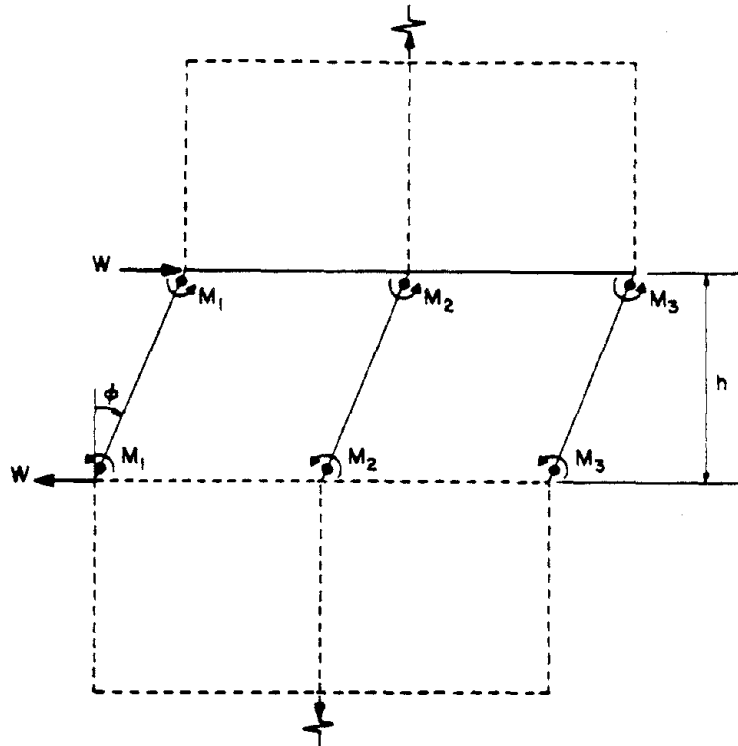
Fig. 6.13 Story Collapse Mechanism for Frame A(C)
