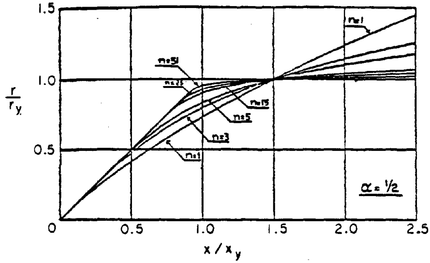
Fig. 5.8 Skeleton Curves Obtained via Ramberg-Osgood Relation [3]
