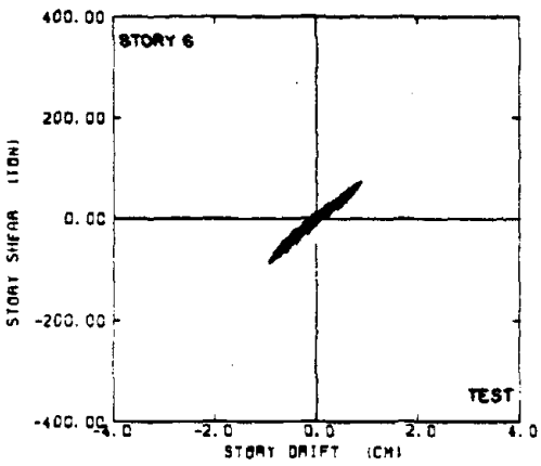
Fig. 6.21 (continued) Comparison of Hysteresis Behavior from the Inelastic Pseudo-Dynamic Test and the Optimal Hysteretic Model
