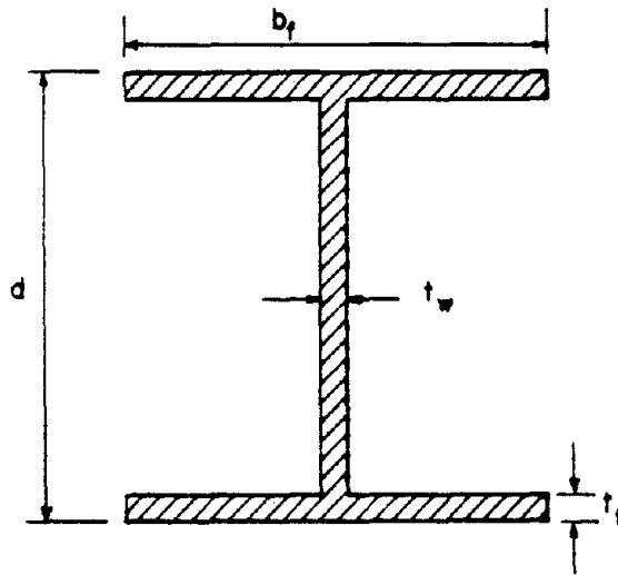
Fig. 6.5 Girder Dimensions
