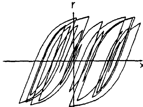
Fig. 5.15 Typical Force-Displacement Curves for Wen's Hysteretic Oscillator Subjected to White Noise Acceleration at Base [29]
