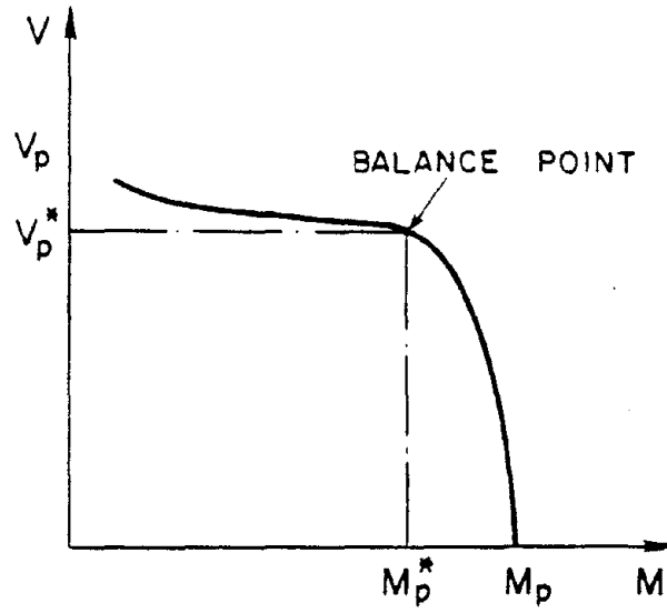
Fig. 6.4 Typical Shear-Moment Interaction Diagram for Wide Flange Sections [3]
