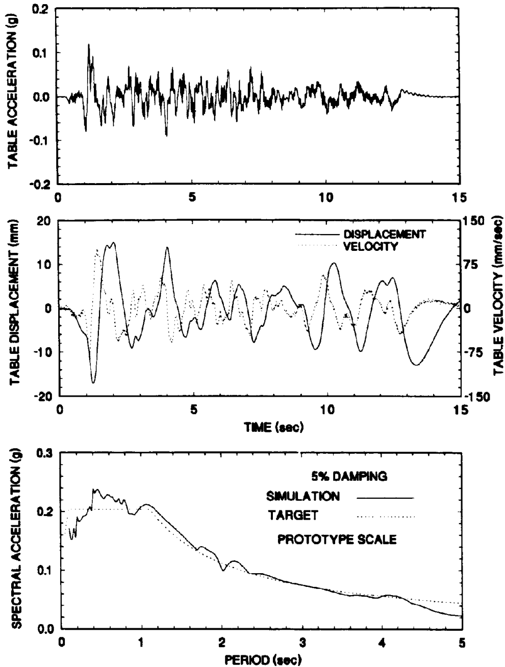
Figure 4-18 Time Histories of Displacement, Velocity and Acceleration and Acceleration Response Spectrum of Shaking Table Motion Excited with JP. Level 1 G.C.1 100% Motion.
