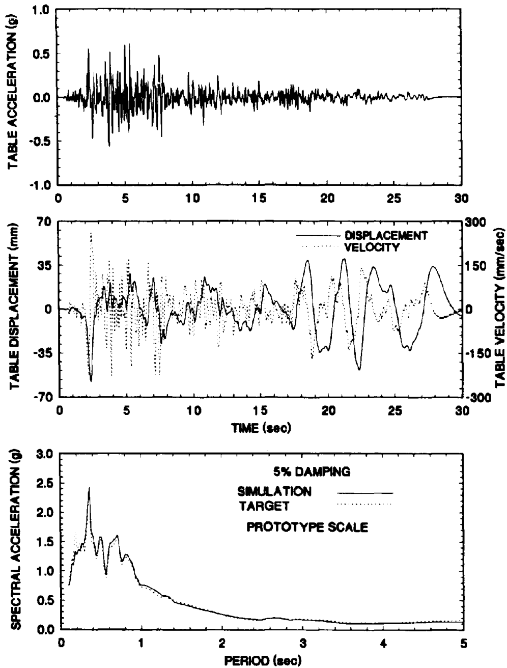
Figure 4-11 Time Histories of Displacement, Velocity and Acceleration and Acceleration Response Spectrum of Shaking Table Motion Excited with Taft N21E 400% Motion.
