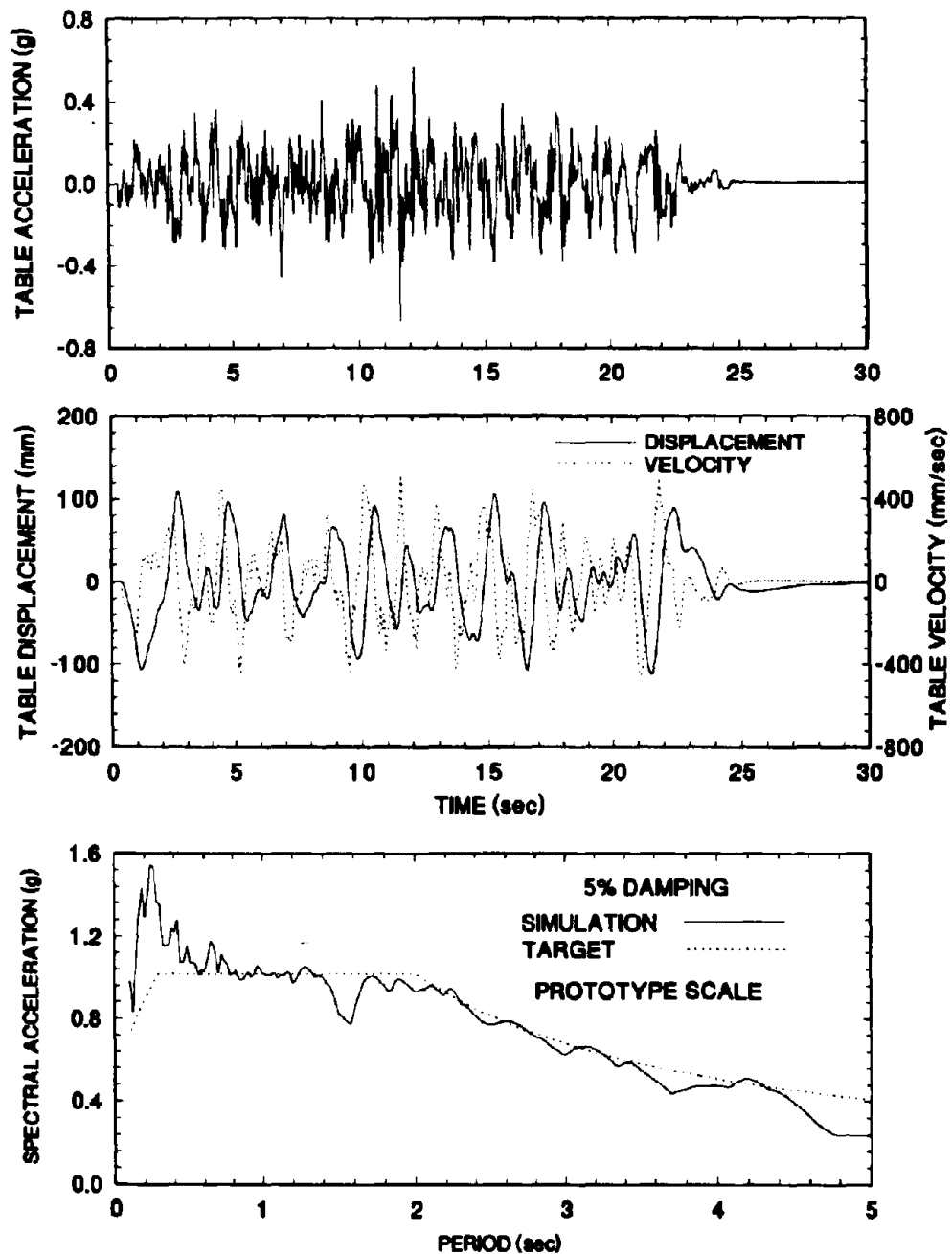
Figure 4-23 Time Histories of Displacement, Velocity and Acceleration and Acceleration Response Spectrum of Shaking Table Motion Excited with JP. Level 2 G.C.3 100% Motion.
