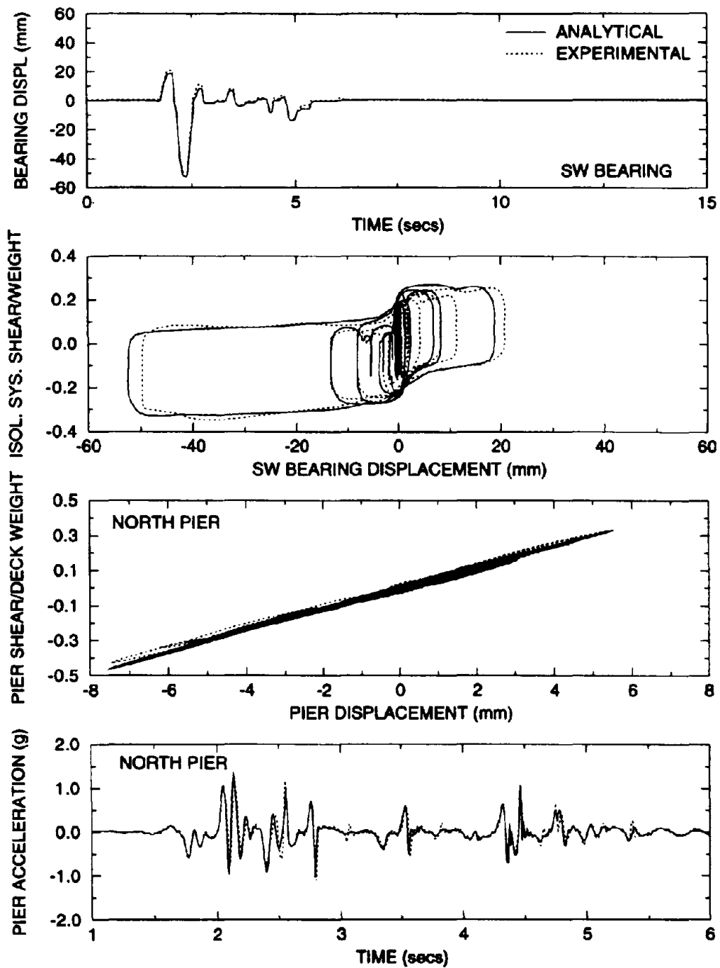
Figure 7-9 Comparison of Experimental and Analytical Results in Test with Pacoima S16E 75% Input (Test No.TDRUN45). Analysis Performed without the Effect of Vertical Pier Acceleration ( \ddot{U}_v=0 ).
