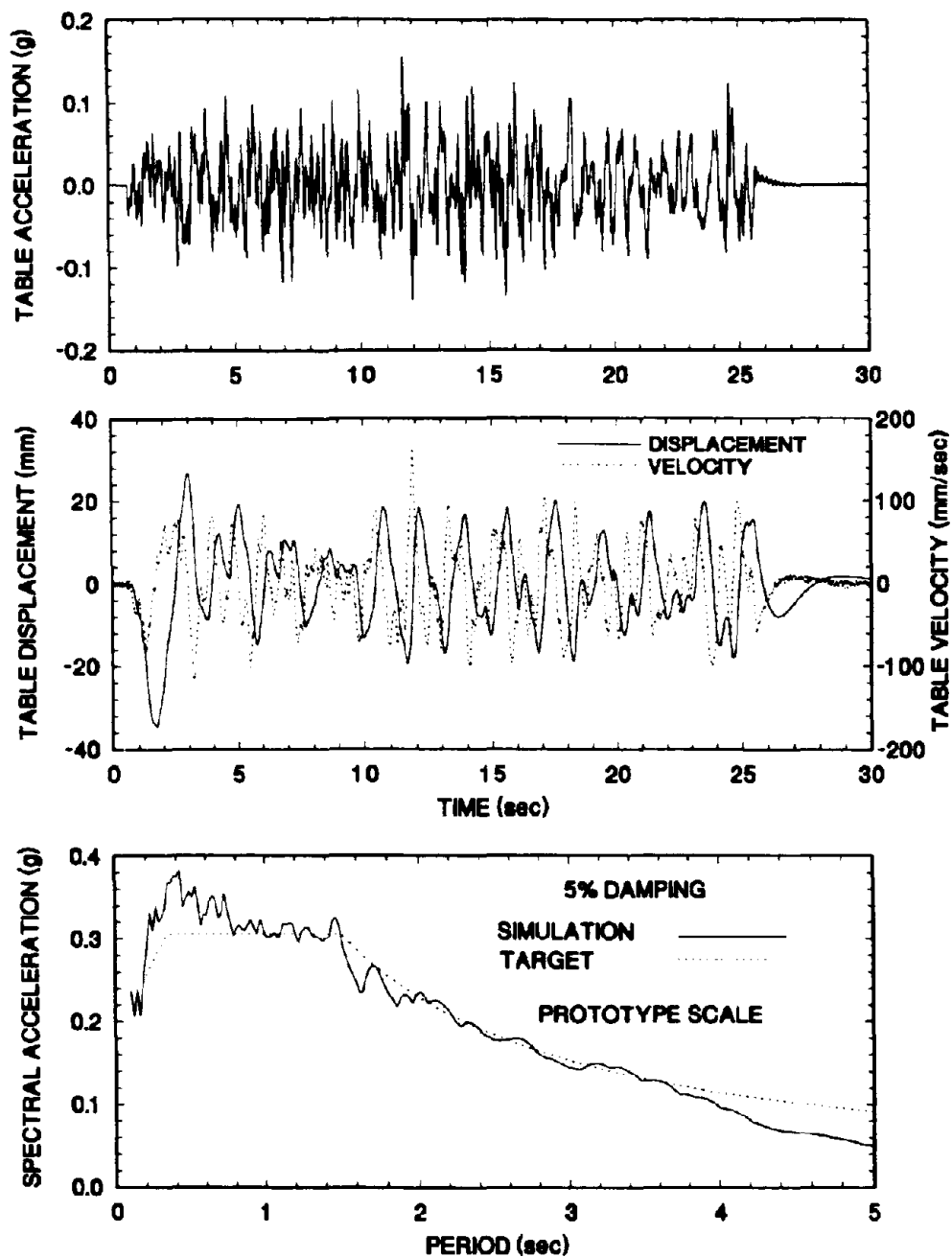
Figure 4-20 Time Histories of Displacement, Velocity and Acceleration and Acceleration Response Spectrum of Shaking Table Motion Excited with JP. Level 1 G.C.3 100% Motion.
