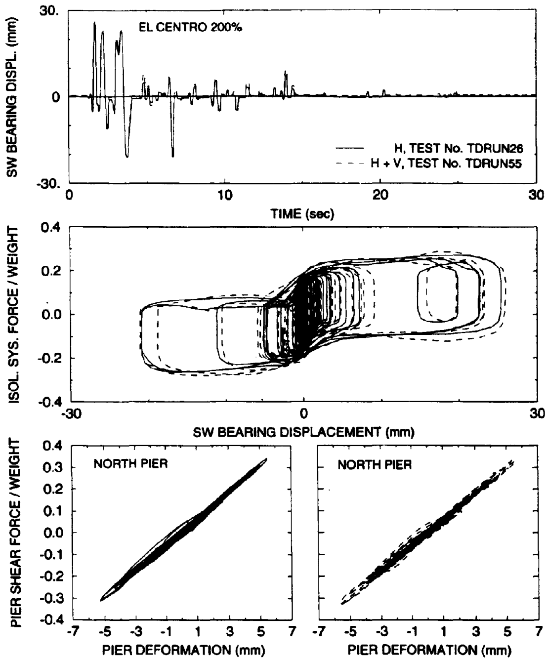
Figure 6-14 Effect of Vertical Ground Motion on Response of System Subjected to El Centro 200% Input.
