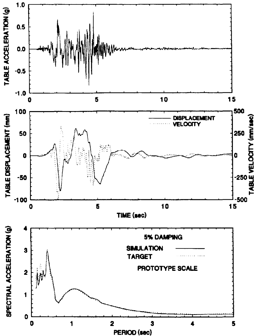
Figure 4-16 Time Histories of Displacement, Velocity and Acceleration and Acceleration Response Spectrum of Shaking Table Motion Excited with Pacoima S16E 100% Motion.
