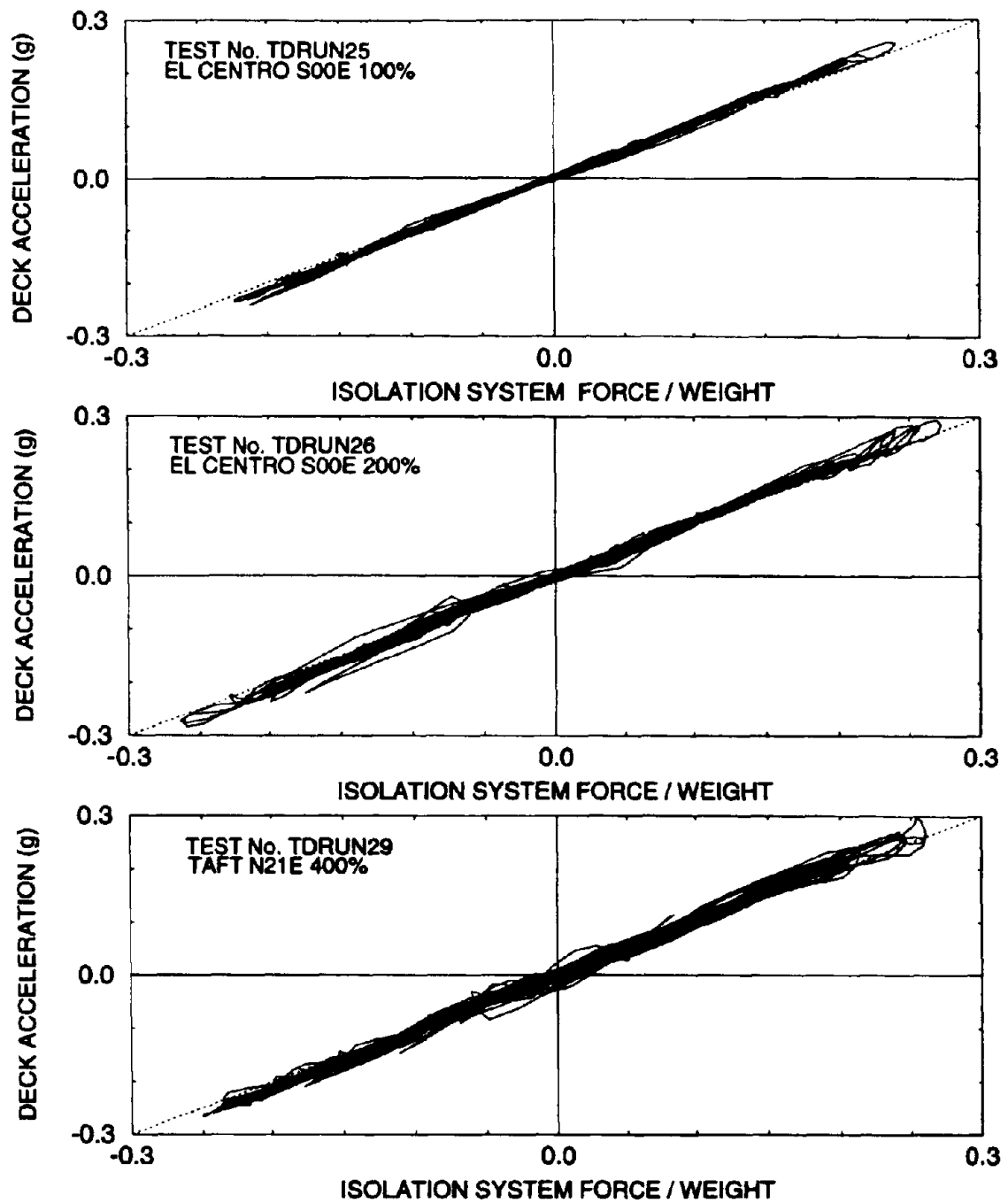
Figure 5-2 Comparison of Deck Acceleration to Isolation System Shear Force in Tests of Model with Flexible Piers.
