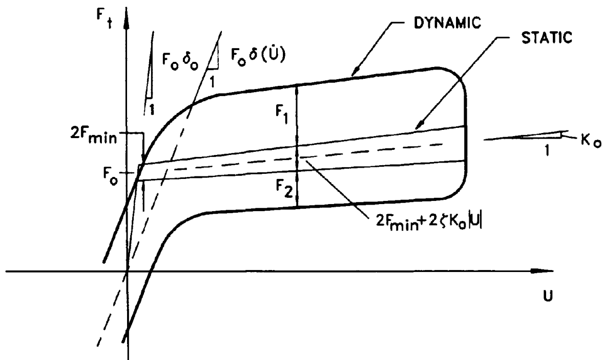
Figure 7-3 Definition of Terms in Model of Fluid Restoring Force/Damping Device.
