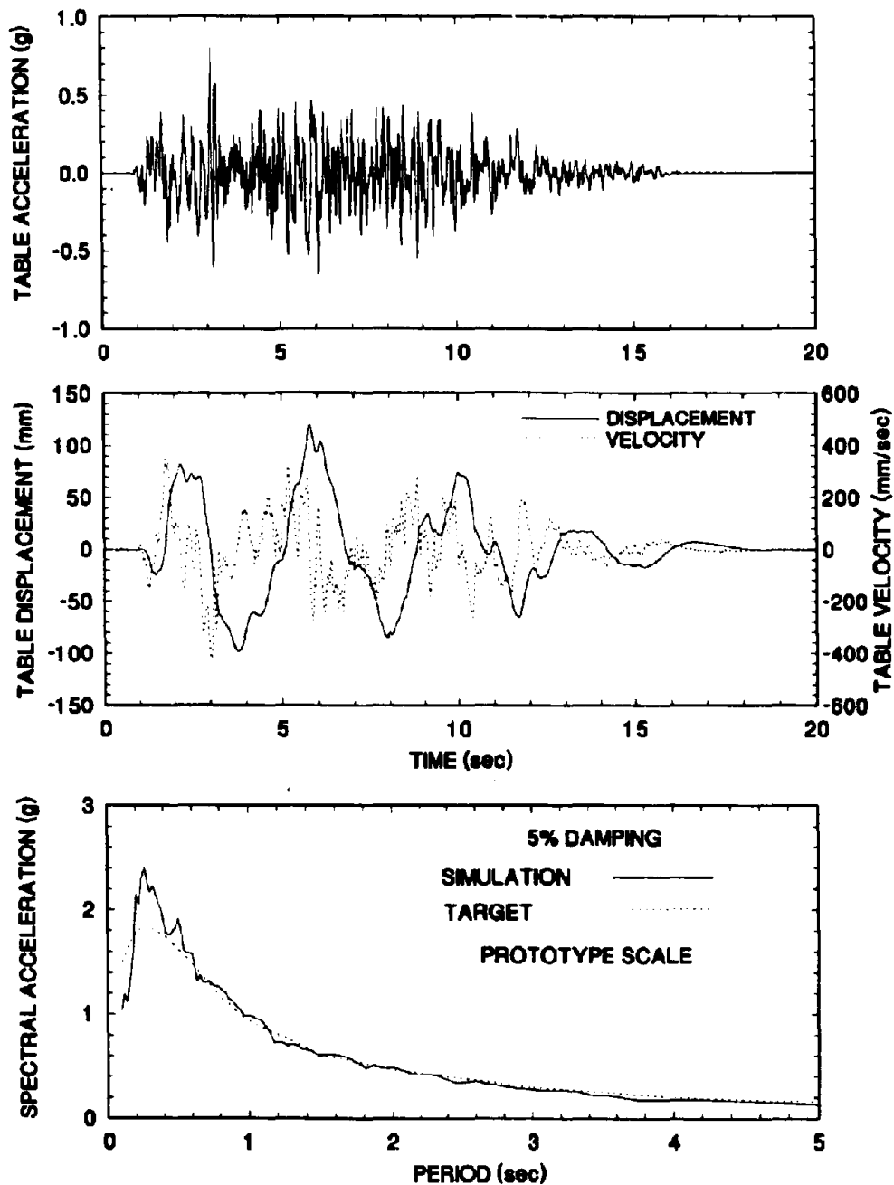
Figure 4-25 Time Histories of Displacement, Velocity and Acceleration and Acceleration Response Spectrum of Shaking Table Motion Excited with CalTrans 10'-80' Alluvium No.3 0.6g 100% Motion.
