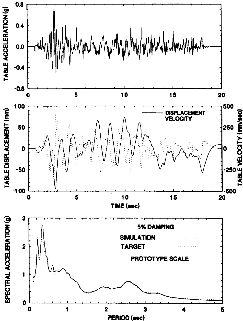
Figure 4-12 Time Histories of Displacement, Velocity and Acceleration and Acceleration Response Spectrum of Shaking Table Motion Excited with Hachinohe N-S 300% Motion.
