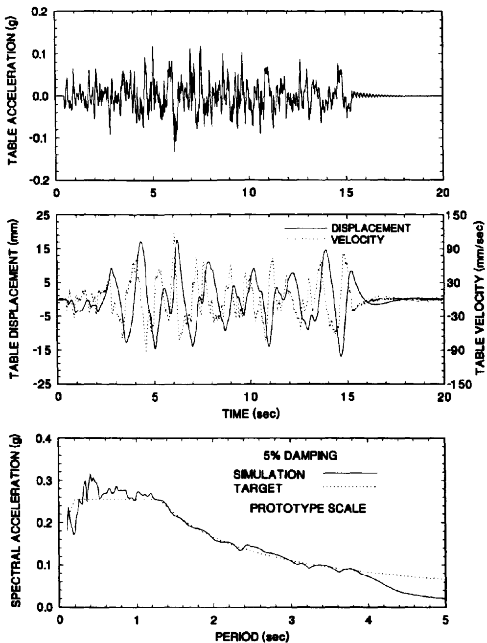
Figure 4-19 Time Histories of Displacement, Velocity and Acceleration and Acceleration Response Spectrum of Shaking Table Motion Excited with JP. Level 1 G.C.2 100% Motion.
