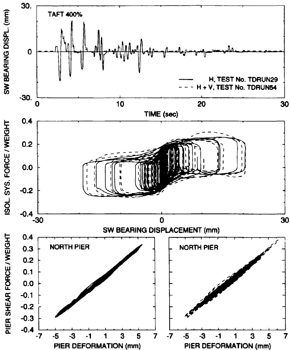
Figure 6-13 Effect of Vertical Ground Motion on Response of System Subjected to Taft 400% Input.
