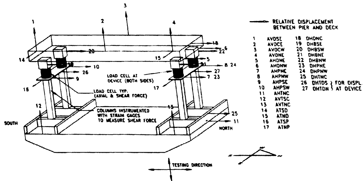
Figure 4-2 Overall Instrumentation Diagram.
