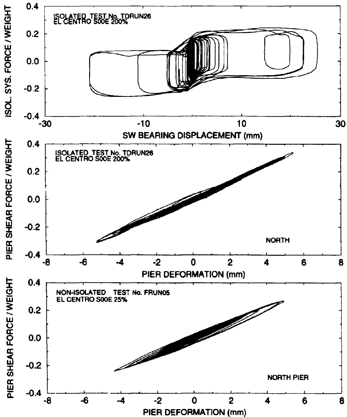
Figure 6-11 Comparison of Non-Isolated and Isolated Bridge Response in the El Centro S00E Motion. Responses are Nearly the Same for Input Being Eight Times Stronger in the Isolated Case.
