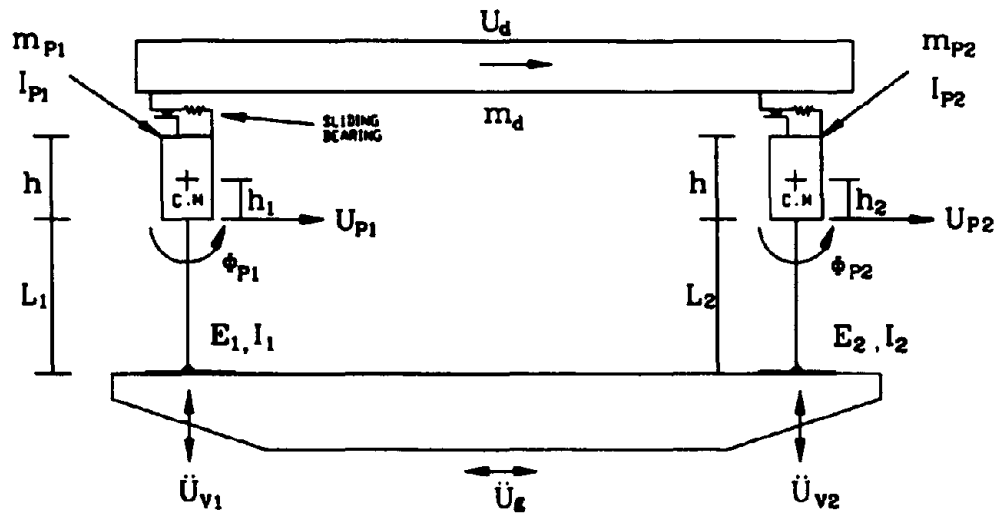
Figure 7-1 Longitudinal Direction Model of Isolated Bridge.
