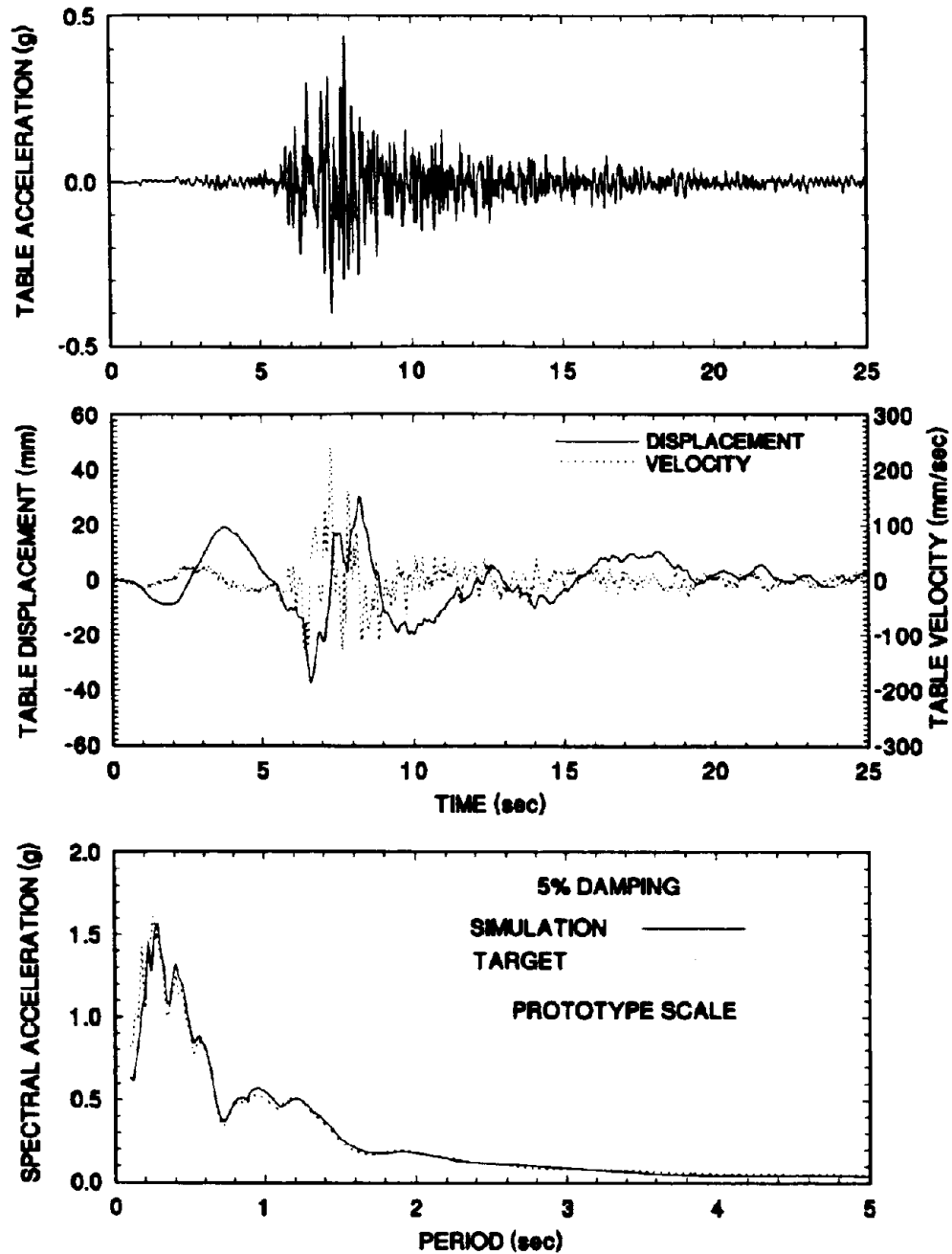
Figure 4-13 Time Histories of Displacement, Velocity and Acceleration and Acceleration Response Spectrum of Shaking Table Motion Excited with Miyagiken Oki E-W 300% Motion.
