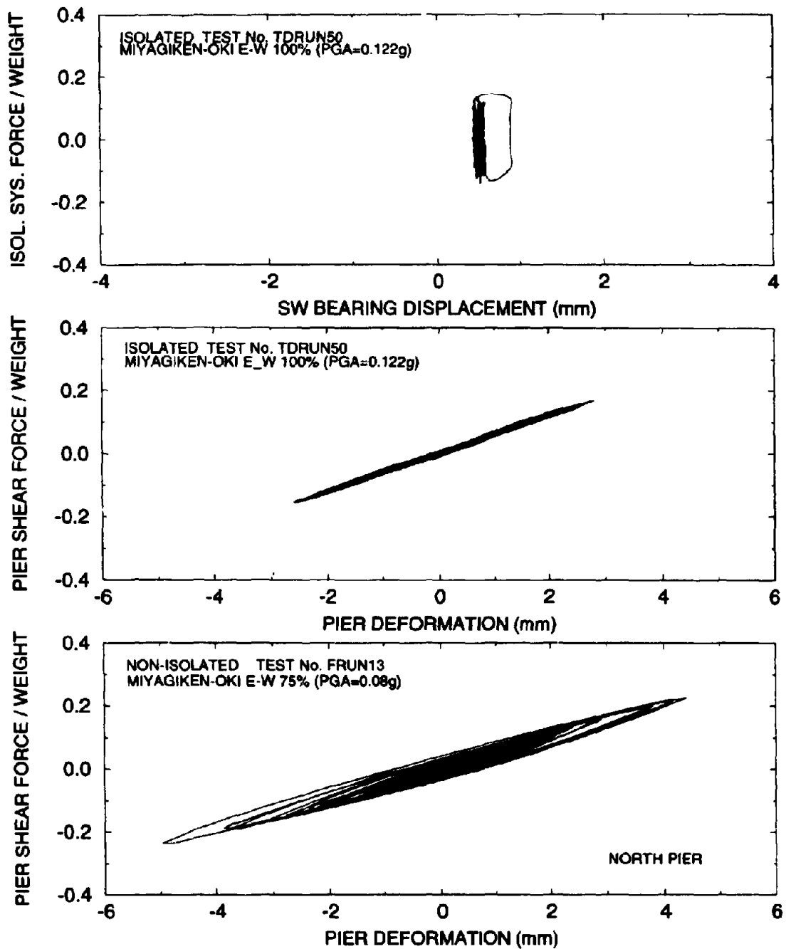
Figure 6-2 Comparison of Response of Isolated and Non-Isolated Bridge in the Weak Miyagiken Oki E-W Motion.
