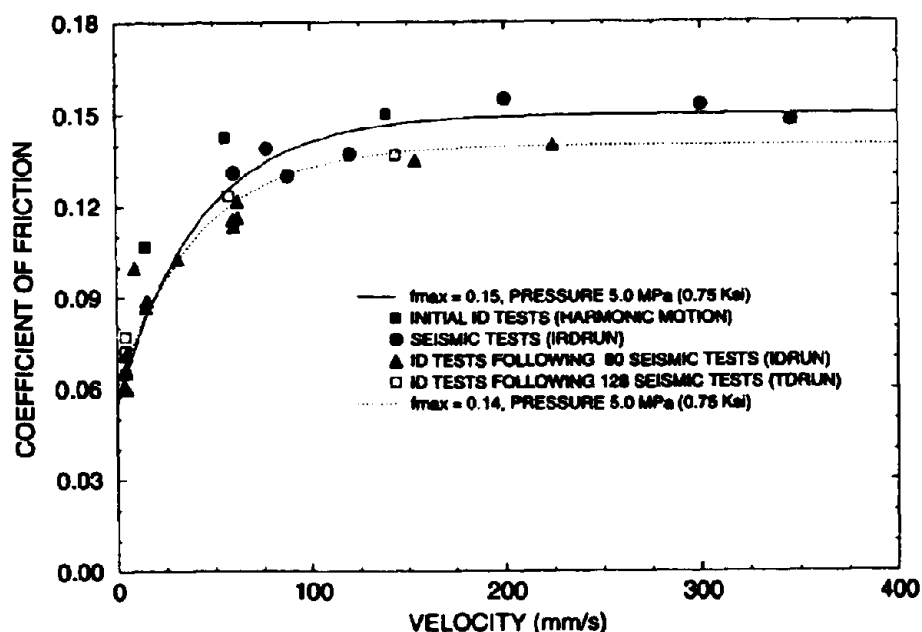
Figure 3-3 Coefficient of Friction as Function of Sliding Velocity of Sliding Disc Bearings.
