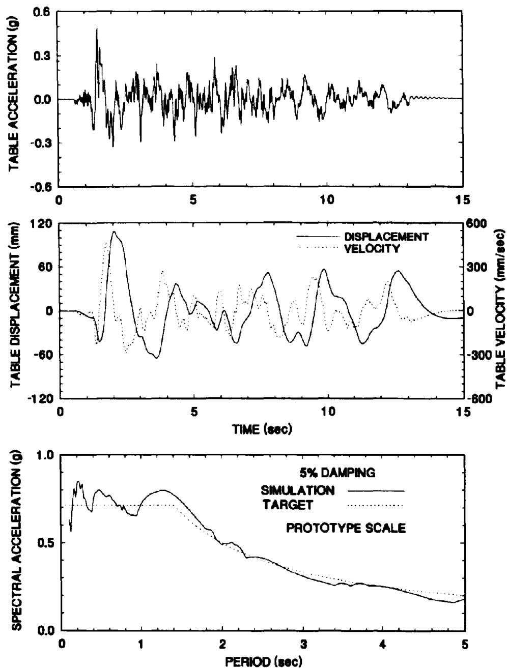
Figure 4-21 Time Histories of Displacement, Velocity and Acceleration and Acceleration Response Spectrum of Shaking Table Motion Excited with JP. Level 2 G.C.1 100% Motion.
