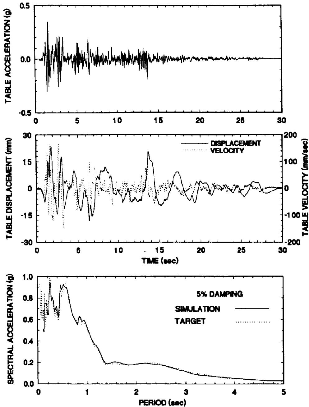
Figure 4-10 Time Histories of Displacement, Velocity and Acceleration and Acceleration Response Spectrum of Shaking Table Motion Excited with El Centro S00E 100% Motion.
