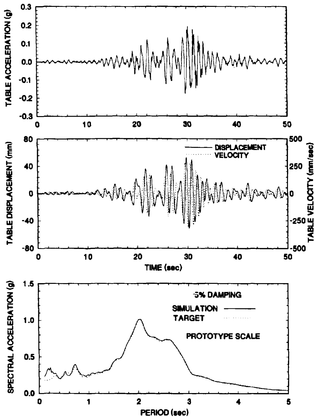
Figure 4-17 Time Histories of Displacement, Velocity and Acceleration and Acceleration Response Spectrum of Shaking Table Motion Excited with Mexico N90W 100% Motion.
