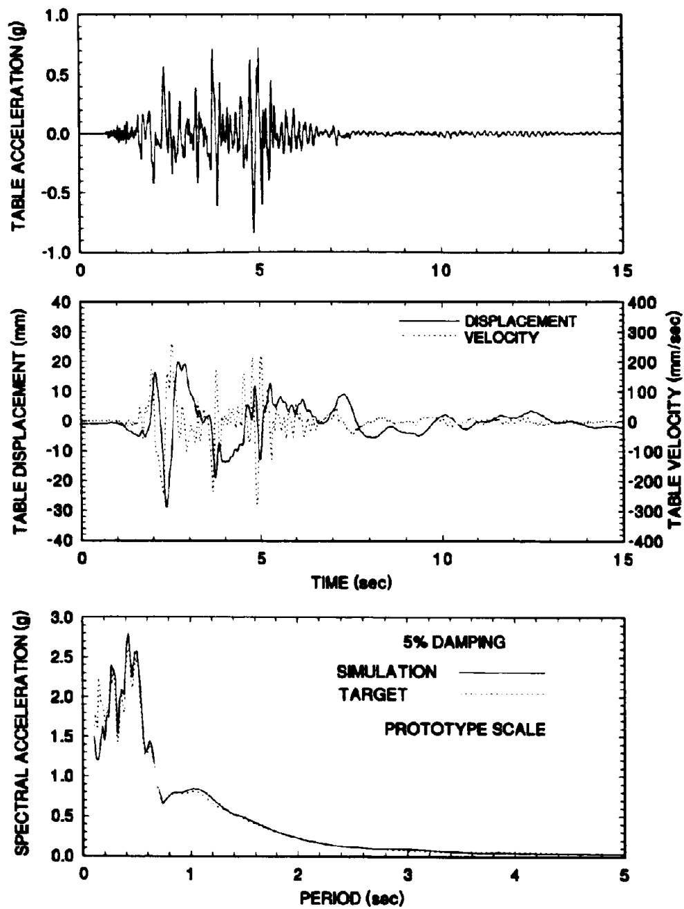
Figure 4-15 Time Histories of Displacement, Velocity and Acceleration and Acceleration Response Spectrum of Shaking Table Motion Excited with Pacoima S74W 100% Motion.
