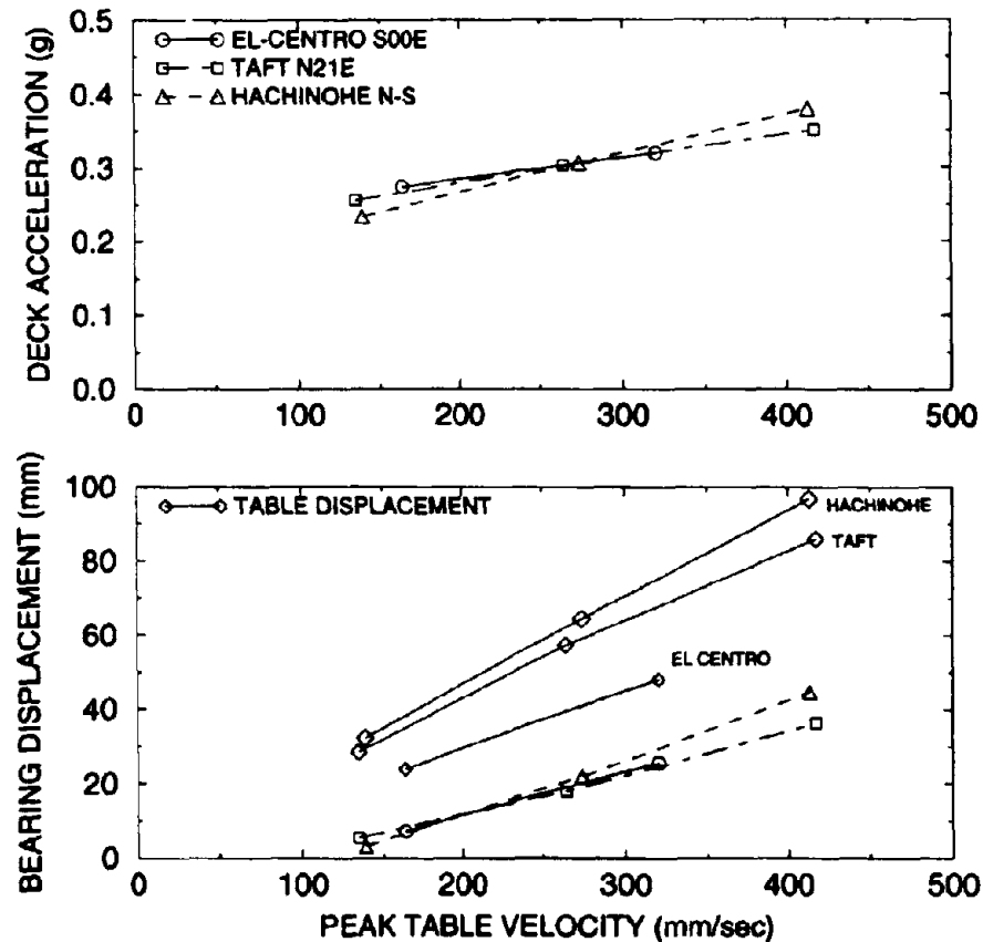
Figure 6-8 Response of Isolated Bridge with Stiff Piers under Increasing Intensity of Input (Represented by Peak Table Velocity).
