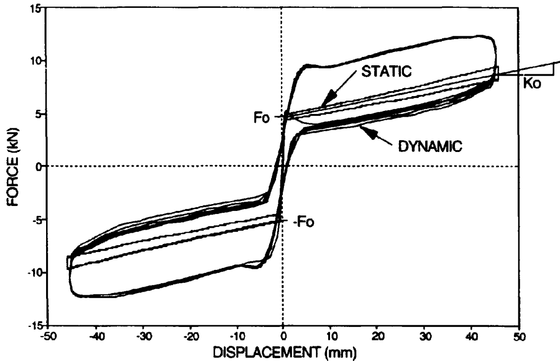
Figure 3-5 Force-Displacement Relationship of Fluid Restoring Force/Damping Device.
