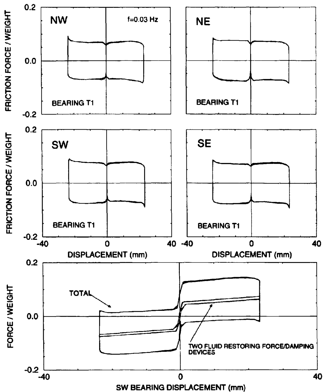
Figure 3-8 Friction Force and Total Force Versus Displacement Loops of Isolation System for Harmonic Excitation at 0.03 Hz.
