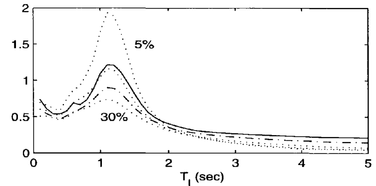
Figure 28: Displacement and base shear spectra of an isolated block subjected to the fault normal component of the Newhall station record (left) and a type-C 2 pulse (right).
