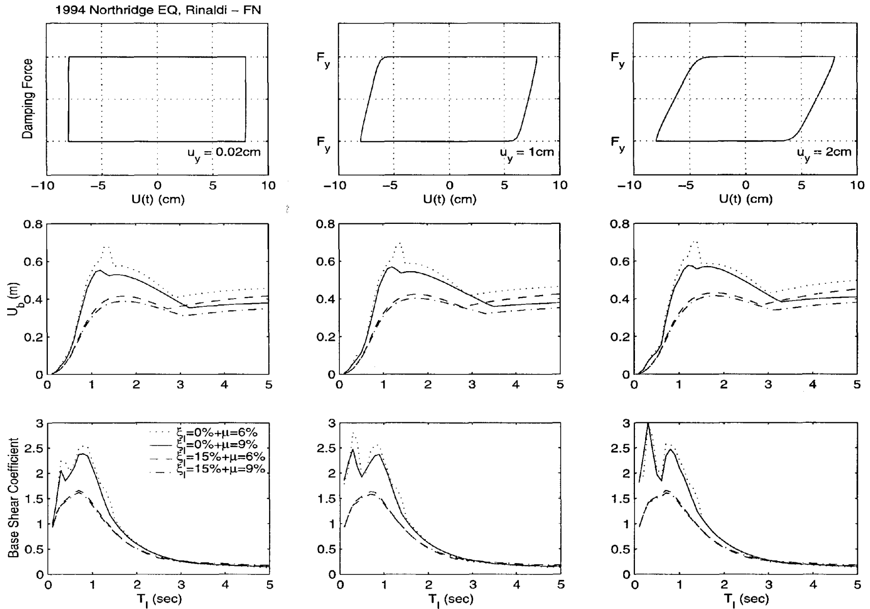
Figure 16: Displacement and base shear spectra of an isolated block subjected to the fault normal component of the Rinaldi station record. Left: u_y = 0.2 mm; center: u_y = 10 mm; right: u_y = 20 mm.
