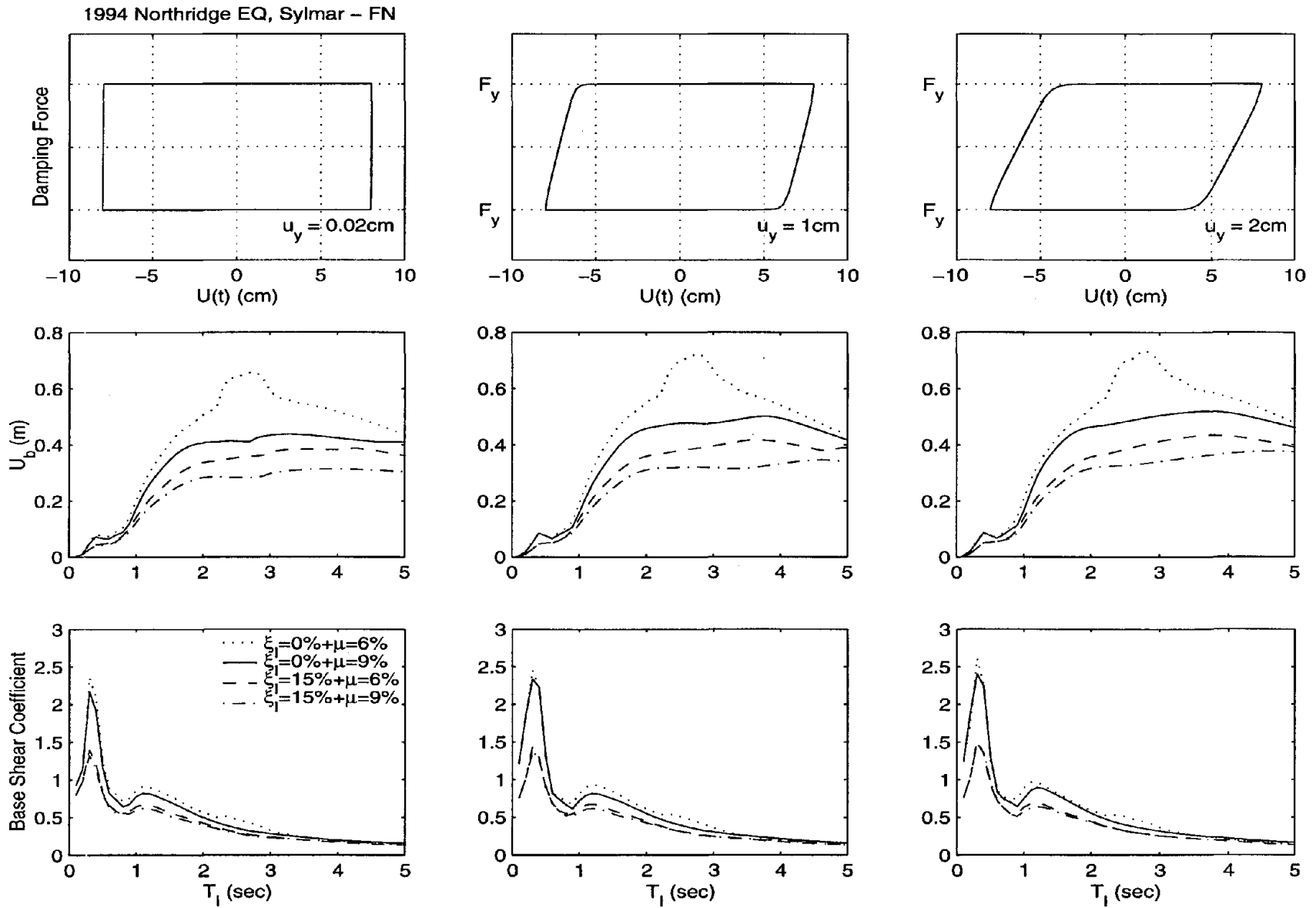
Figure 25: Displacement and base shear spectra of an isolated block subjected to the fault normal component of the Sylmar station record. Left: u_y = 0.2 mm; center: u_y = 10 mm; right: u_y = 20 mm.
