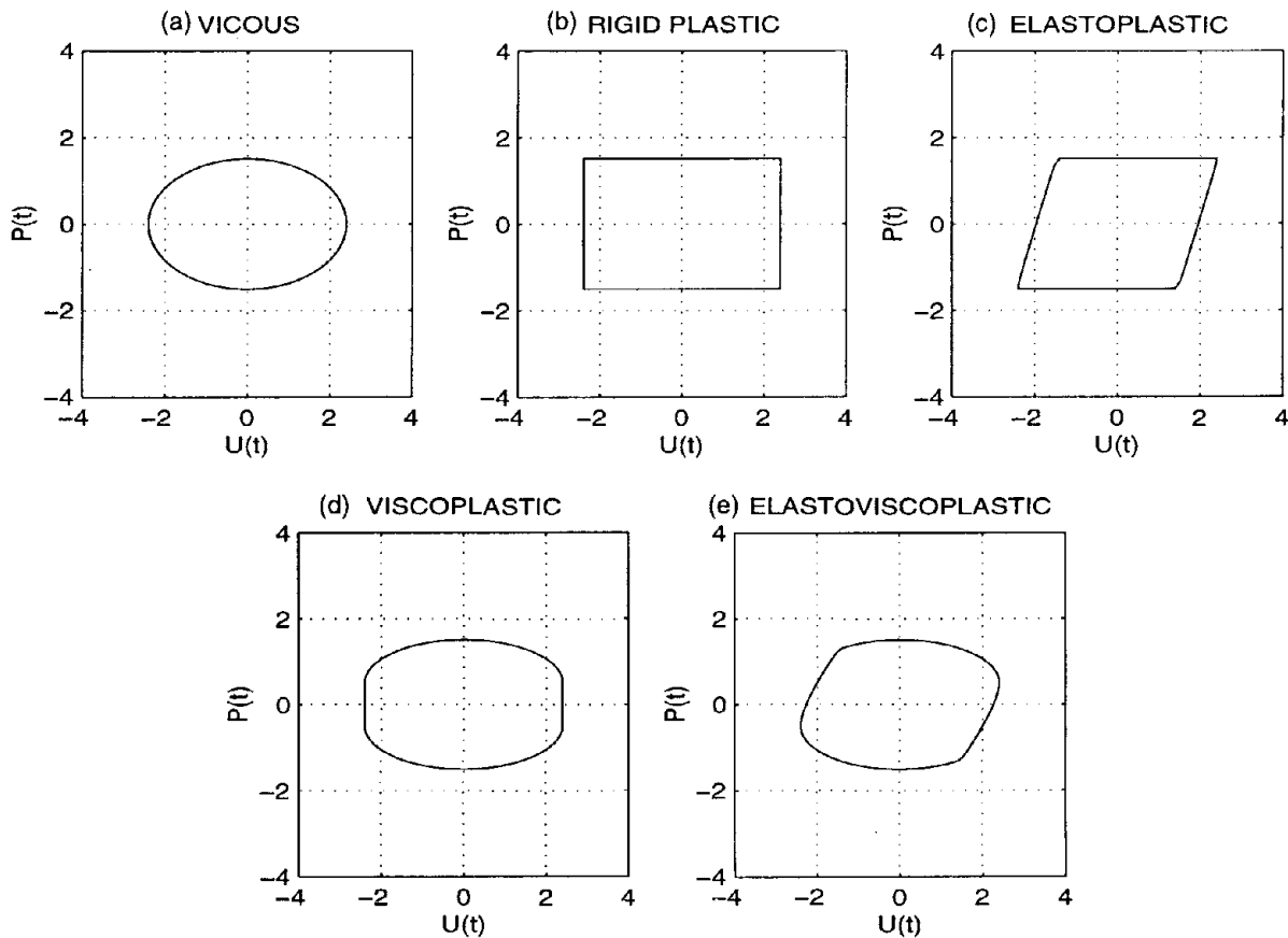
Figure 11: Five idealizations of energy dissipation mechanisms of practical seismic isolation systems.
