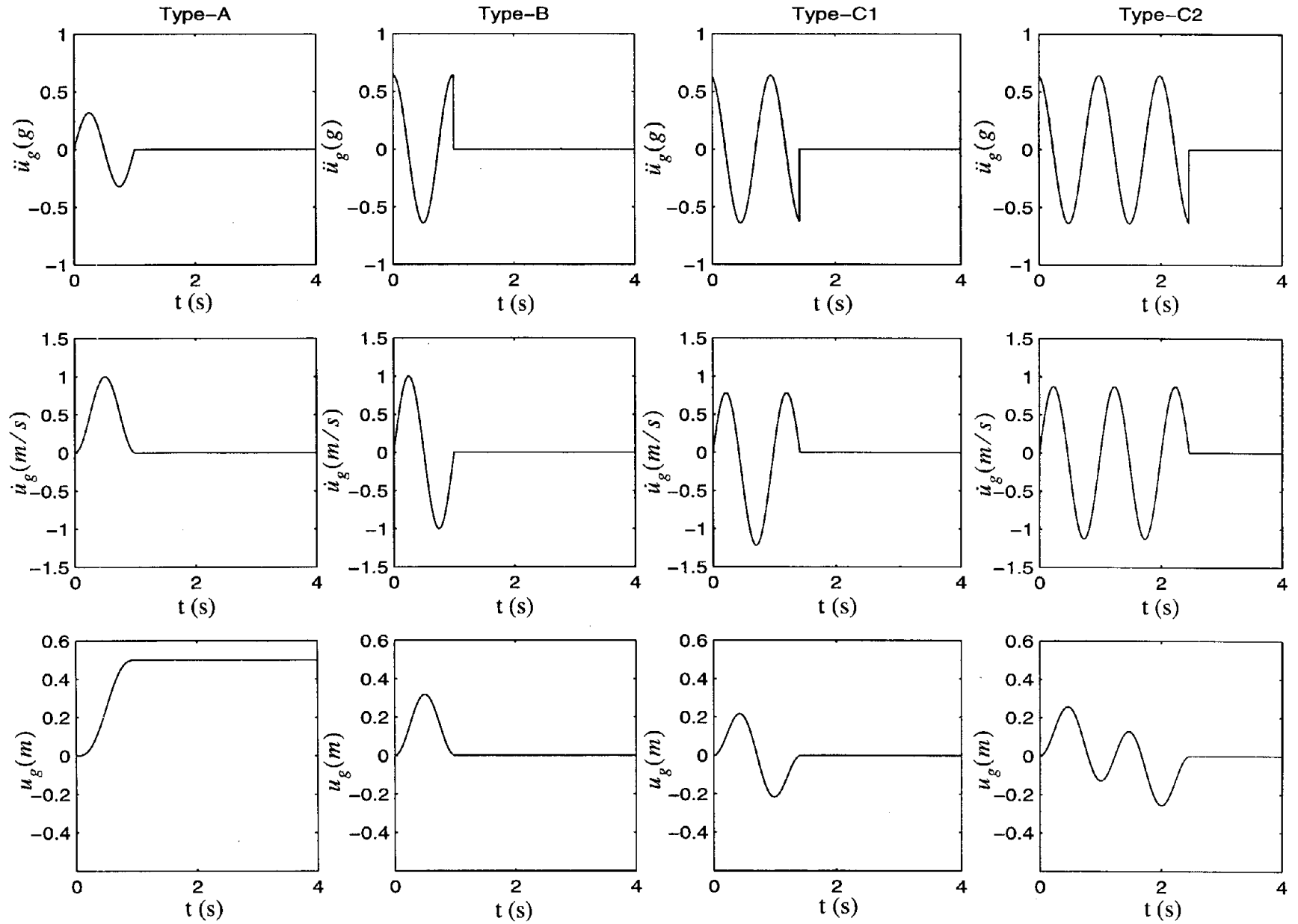
Figure 10: Acceleration, velocity and displacement time histories of cycloidal pulses type-A (first column), type-B (second column), type-C 1 (third column) and type-C 2 (fourth column).
