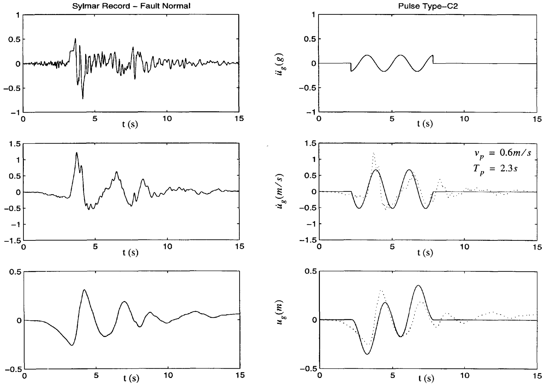
Figure 7: Fault normal components of the acceleration, velocity and displacement time histories recorded at the Sylmar station during the January 17th, 1994 Northridge, California earthquake (left) and a cycloidal type-C 2 pulse (right).
