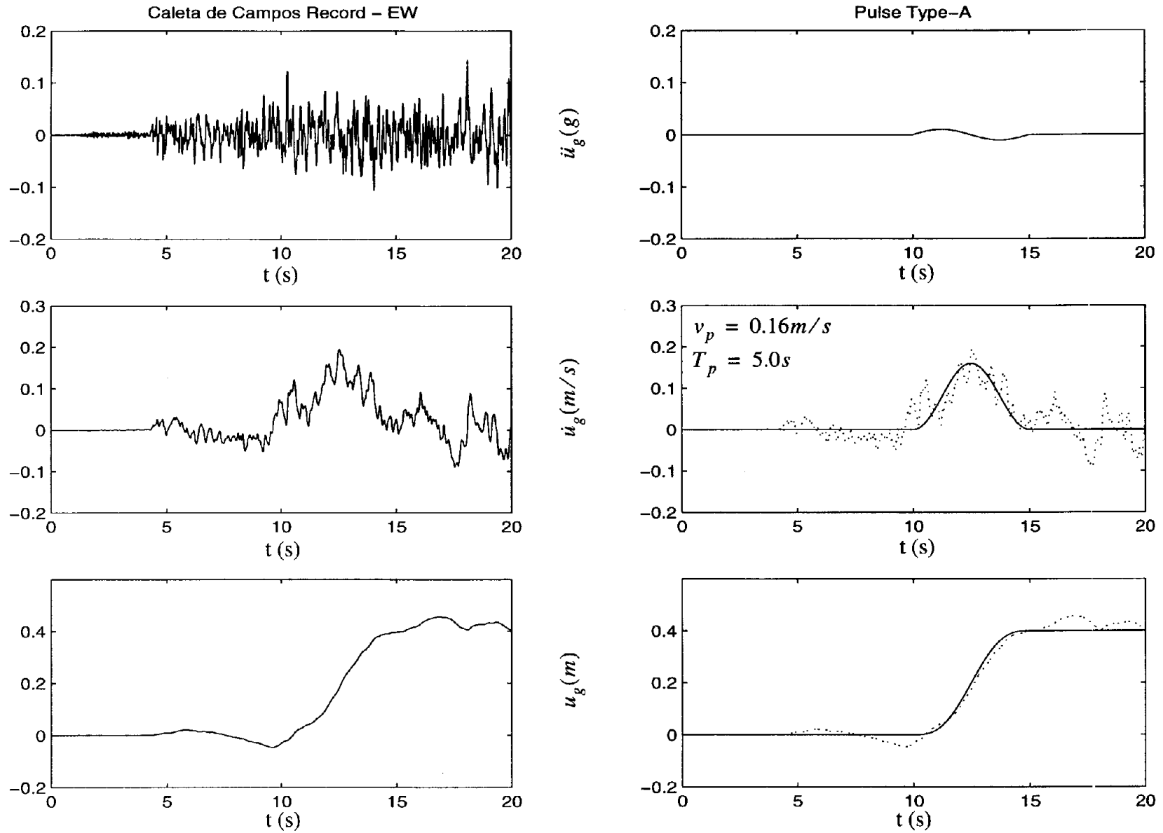
Figure 2: Fault normal components of the acceleration, velocity and displacement time histories recorded at the Caleta de Campos station during the September 19th, 1985 Michoacan, earthquake (left), and a cycloidal type-A pulse (right).
