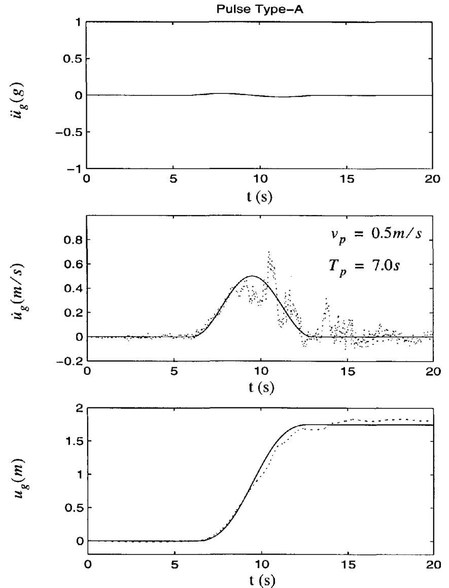
Figure 3: Fault parallel components of the acceleration, velocity and displacement time histories recorded at the Lucerne Valley station during the June 28th, 1992 Landers, California earthquake (left), and a cycloidal type-A pulse (right).
