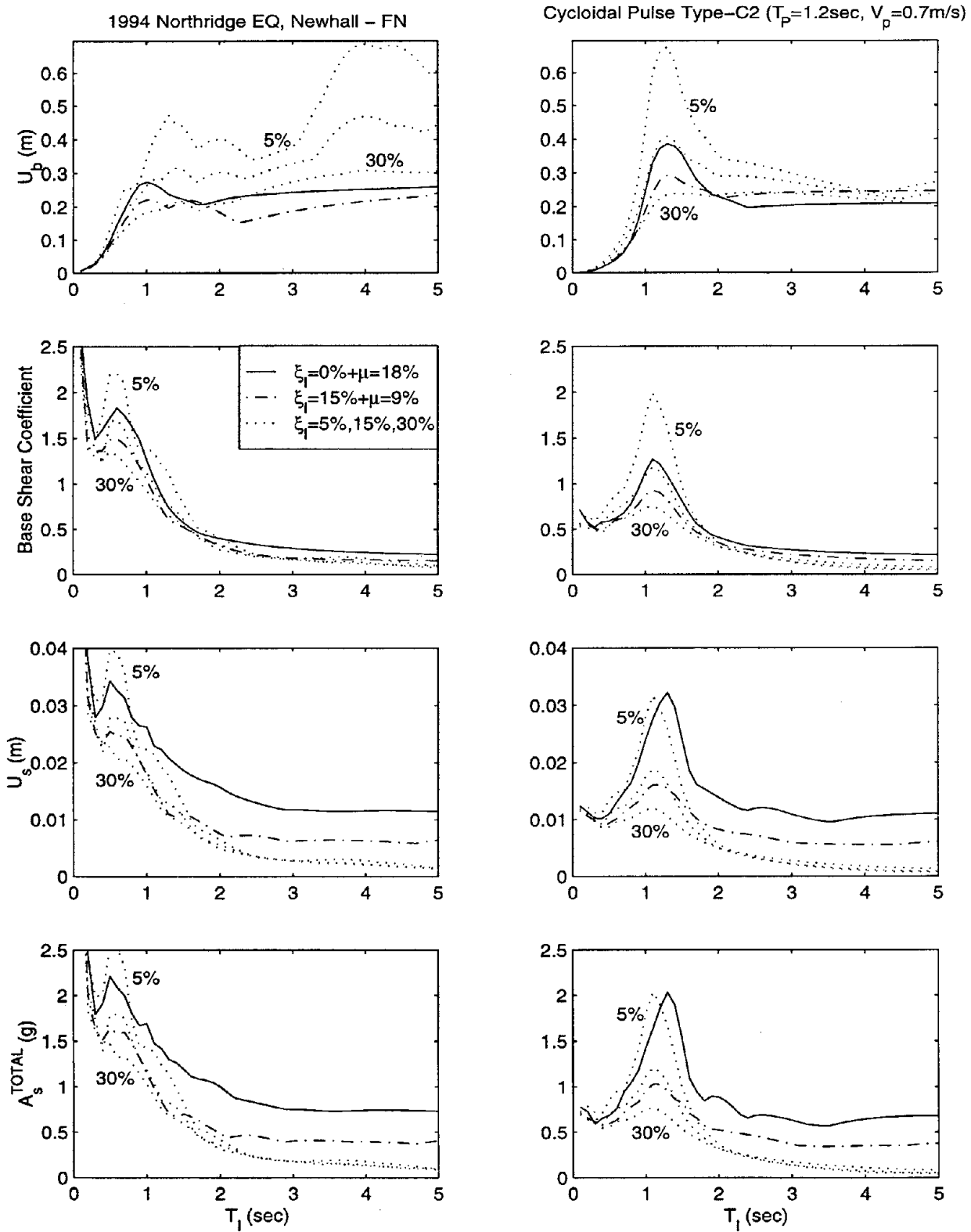
Figure 33: Base displacement, base shear, superstructure drift and total superstructure acceleration spectra of a 2-DOF isolated structure subjected to the fault normal component of the Newhall station record (left) and a type-C 2 pulse (right).
