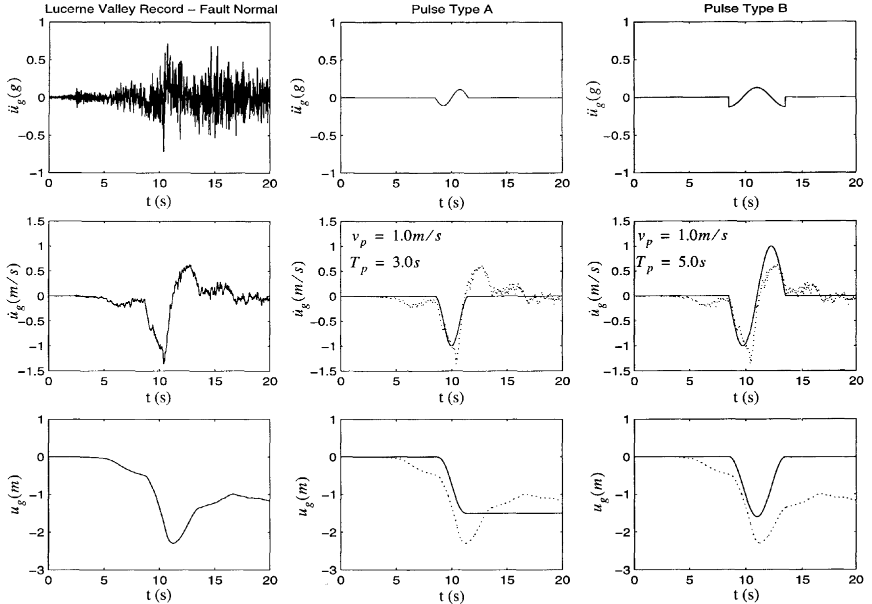
Figure 6: Fault normal components of the acceleration, velocity and displacement time histories recorded at the Lucerne Valley station during the June 28th, 1992 Landers, California earthquake (left), a cycloidal type-A pulse (center) and a cycloidal type-B pulse (right).
