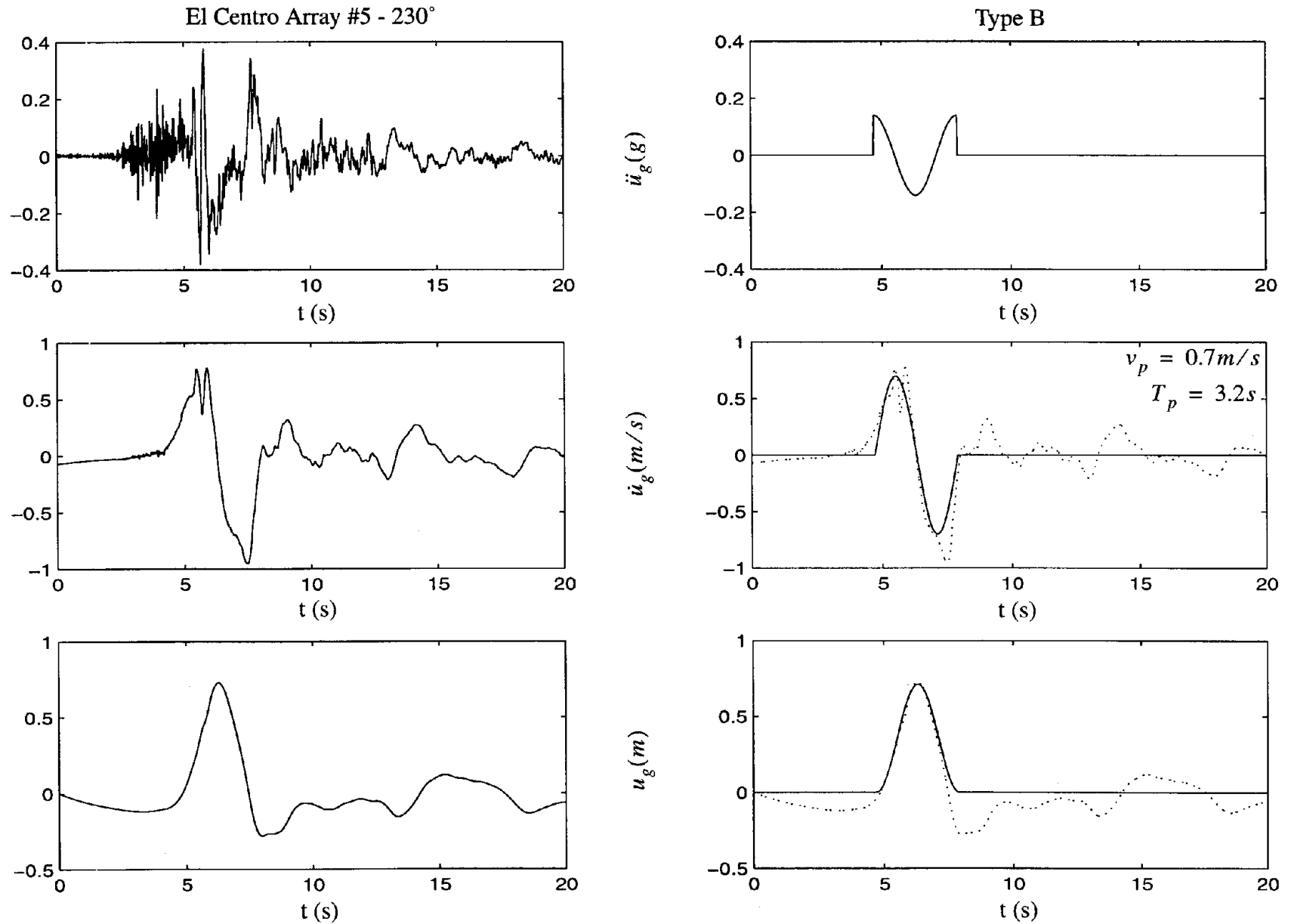
Figure 4: Fault normal components of the acceleration, velocity and displacement time histories recorded at the El Centro Array #5 station during the October 15th, 1979 Imperial Valley, California earthquake (left), and a cycloidal type-B pulse (right).
