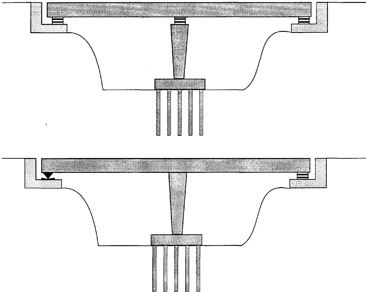
Figure 12: Schematic of a seismically isolated overpass (top) and of an overpass that is supported on bearings at the end abutments (bottom).
