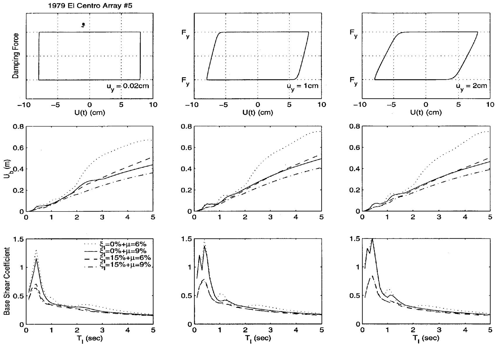
Figure 23: Displacement and base shear spectra of an isolated block subjected to the fault normal component of the El Centro Array #5 station record. Left: u_y = 0.2\text{ mm} ; center: u_y = 10\text{ mm} ; right: u_y = 20\text{ mm} .
