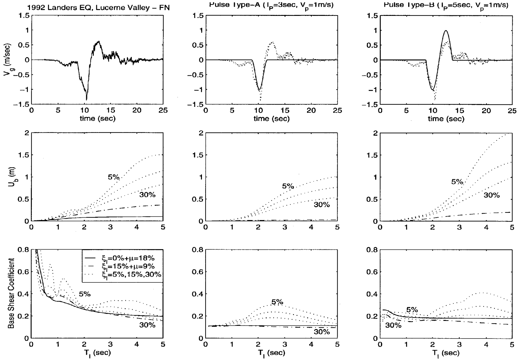
Figure 18: Displacement and base shear spectra of an isolated block subjected to the fault normal component of Lucerne Valley record (left), a type-A pulse (center) and a type-B pulse (right).
