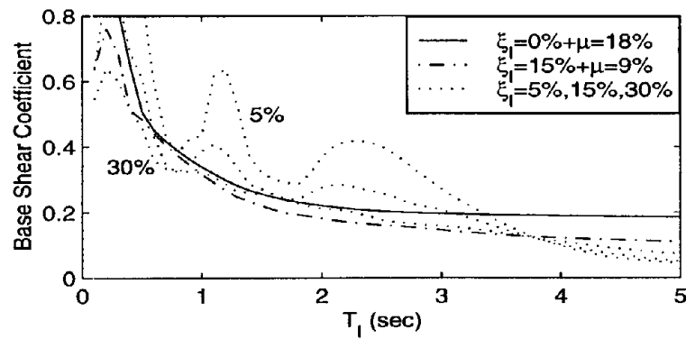
Figure 27: Displacement and base shear spectra of an isolated block subjected to the fault parallel component of the Rinaldi station record (left) and a type-C 2 pulse (right).
