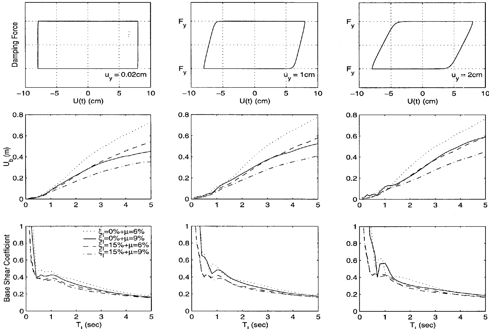
Figure 19: Displacement and base shear spectra of an isolated block subjected to the fault normal component of the Lucerne Valley record. Left: u_y = 0.2\text{ mm} ; center: u_y = 10\text{ mm} ; right: u_y = 20\text{ mm} .
