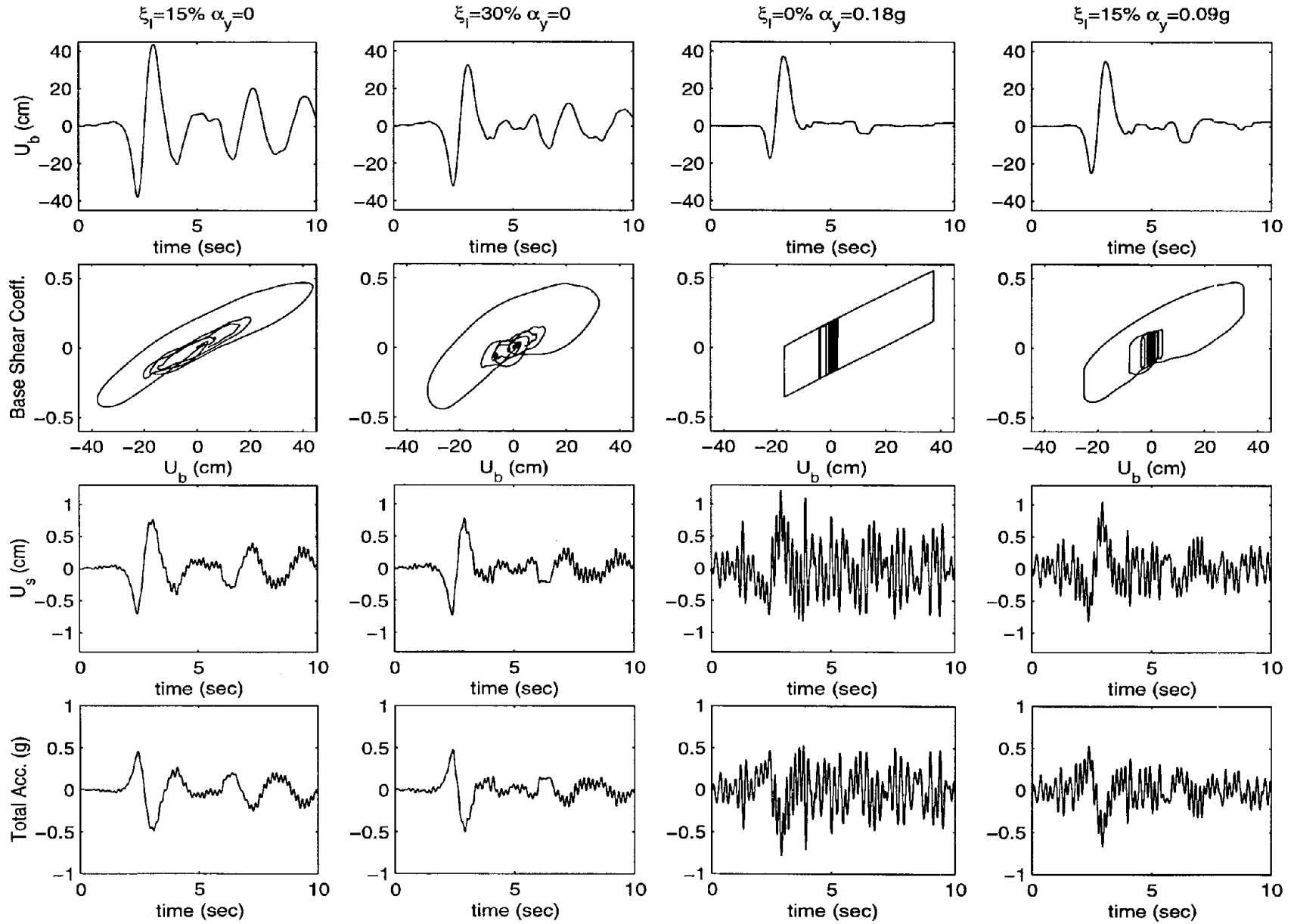
Figure 30: Response quantities of a 2-DOF isolated structure subjected to the fault normal component of the Rinaldi station record.
