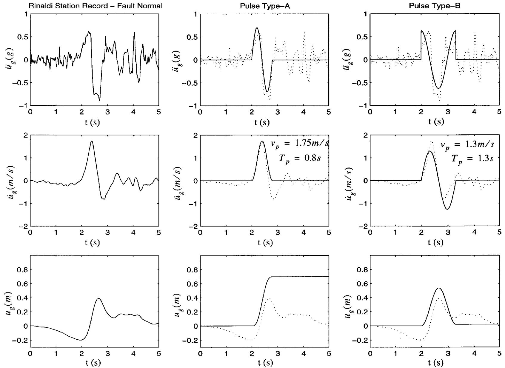
Figure 5: Fault normal components of the acceleration, velocity and displacement time histories recorded at the Rinaldi station during the January 17th, 1994 Northridge, California earthquake (left), a cycloidal type-A pulse (center) and a cycloidal type-B pulse (right).
