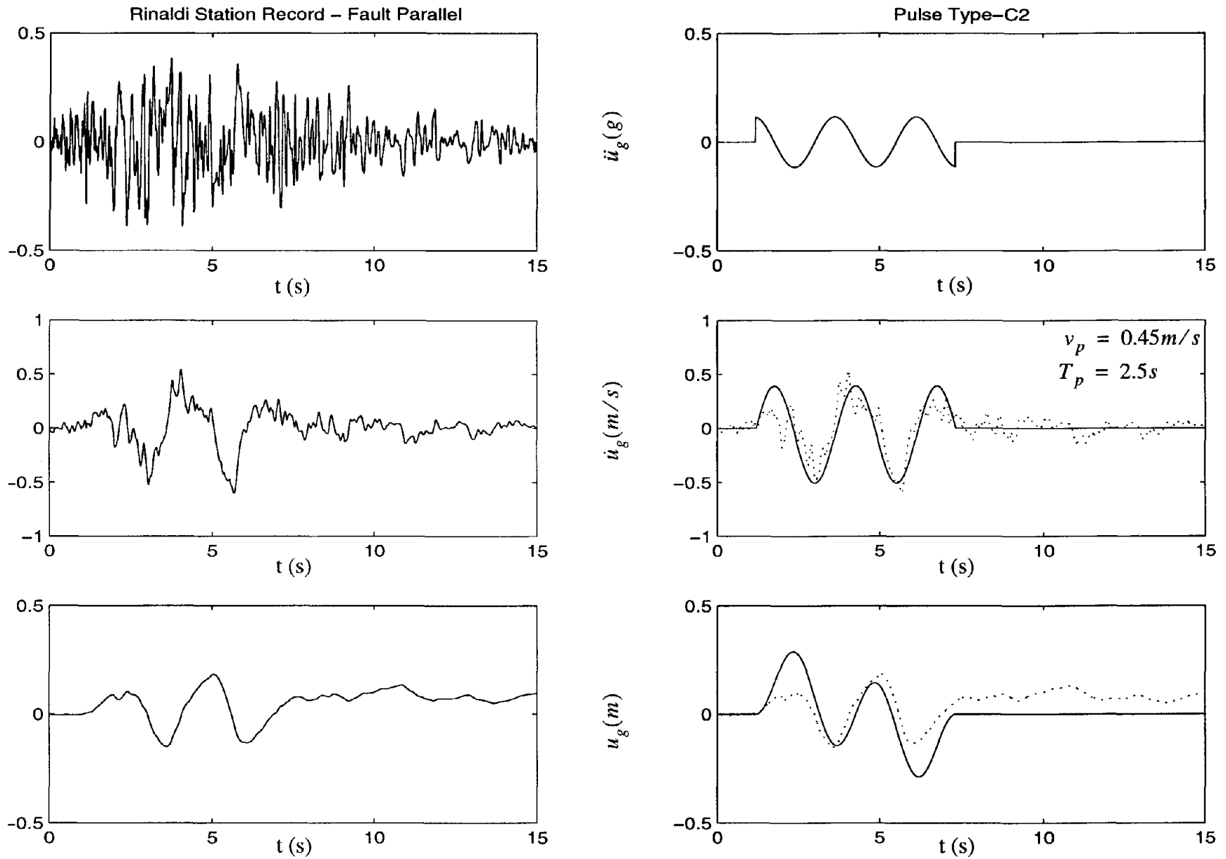
Figure 8: Fault parallel components of the acceleration, velocity and displacement time histories recorded at the Rinaldi station during the January 17th, 1994 Northridge, California earthquake (left) and a cycloidal type-C 2 pulse (right).
