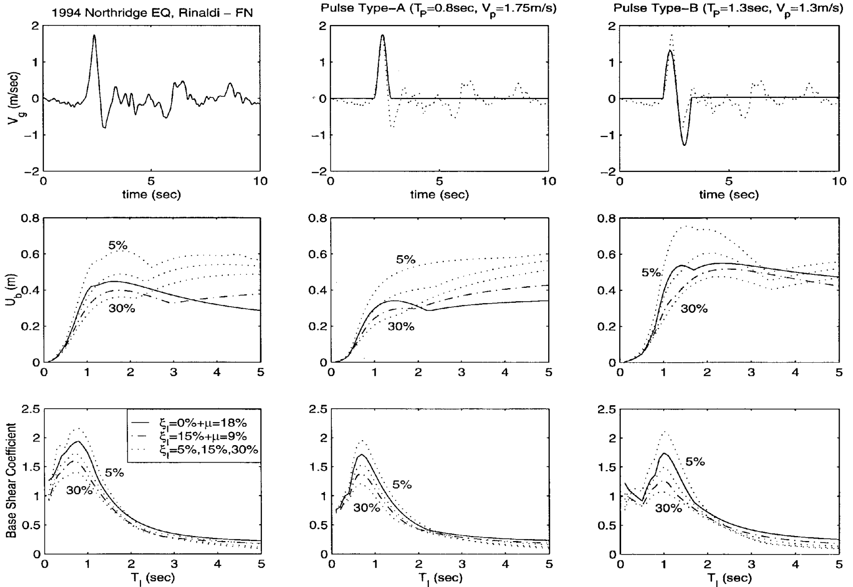
Figure 15: Displacement and base shear spectra of an isolated block subjected to the fault normal component of the Rinaldi station record (left), a type-A pulse (center) and a type-B pulse (right).
