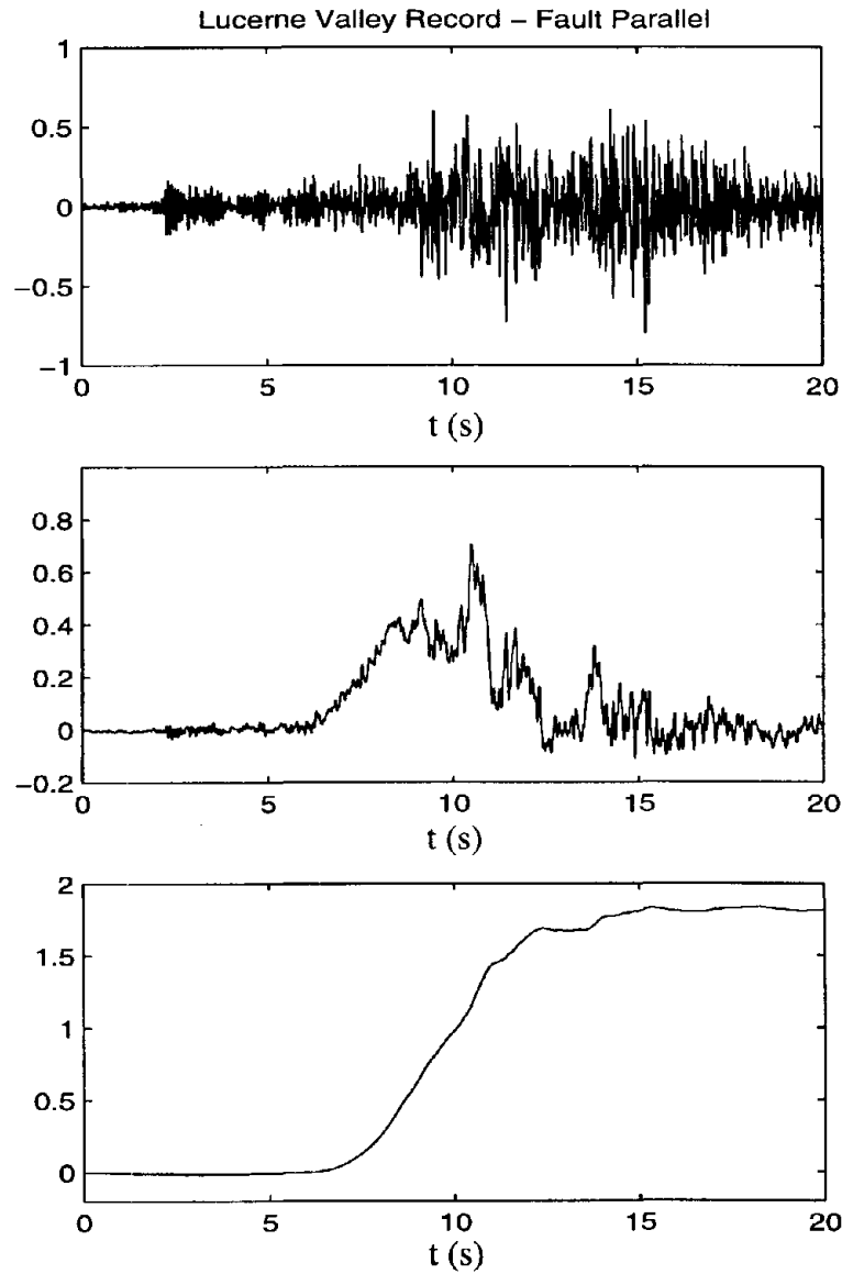
Figure 3: Fault parallel components of the acceleration, velocity and displacement time histories recorded at the Lucerne Valley station during the June 28th, 1992 Landers, California earthquake (left), and a cycloidal type-A pulse (right).
