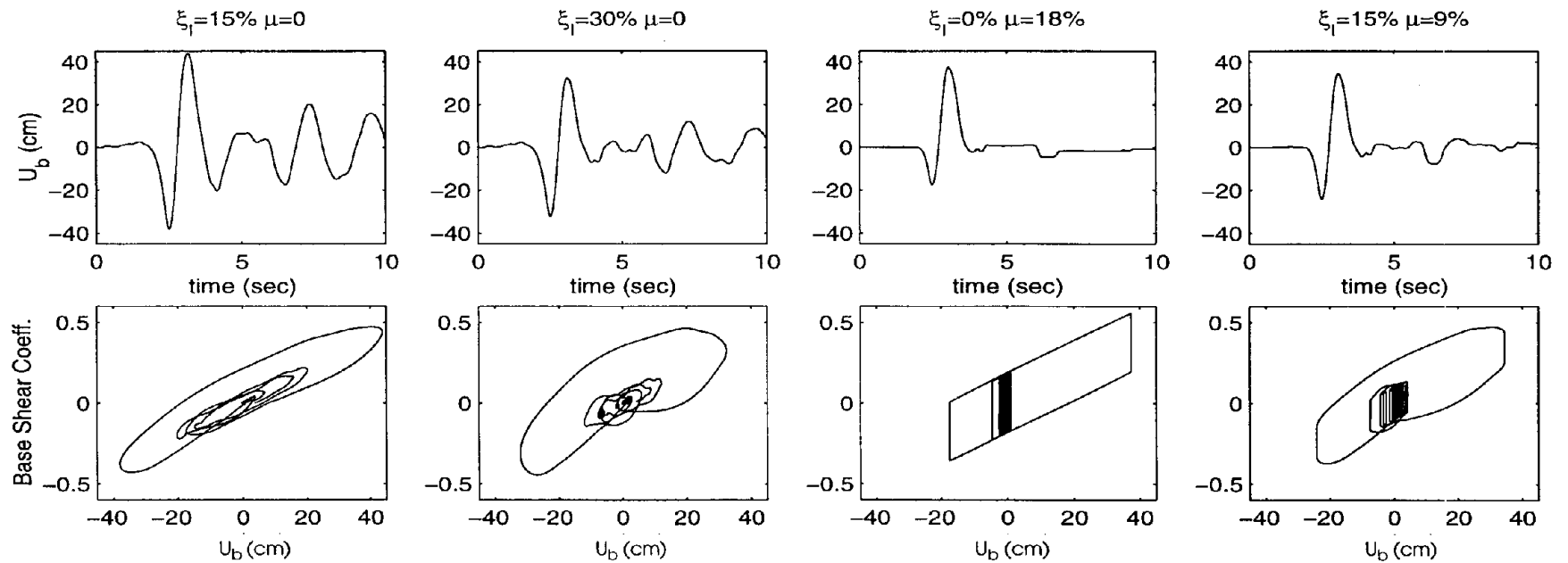
Figure 13: Response quantities of an isolated block with T_I = 2 sec subjected to a type A pulse with T_I = 1 sec (top) and to the Rinaldi station record (bottom)
