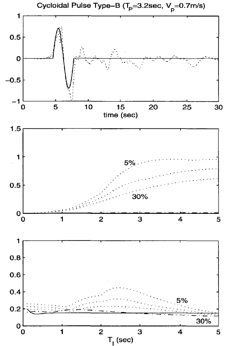
Figure 22: Displacement and base shear spectra of an isolated block subjected to the El Centro Array #5 station record (left) and a type-B pulse (right).
