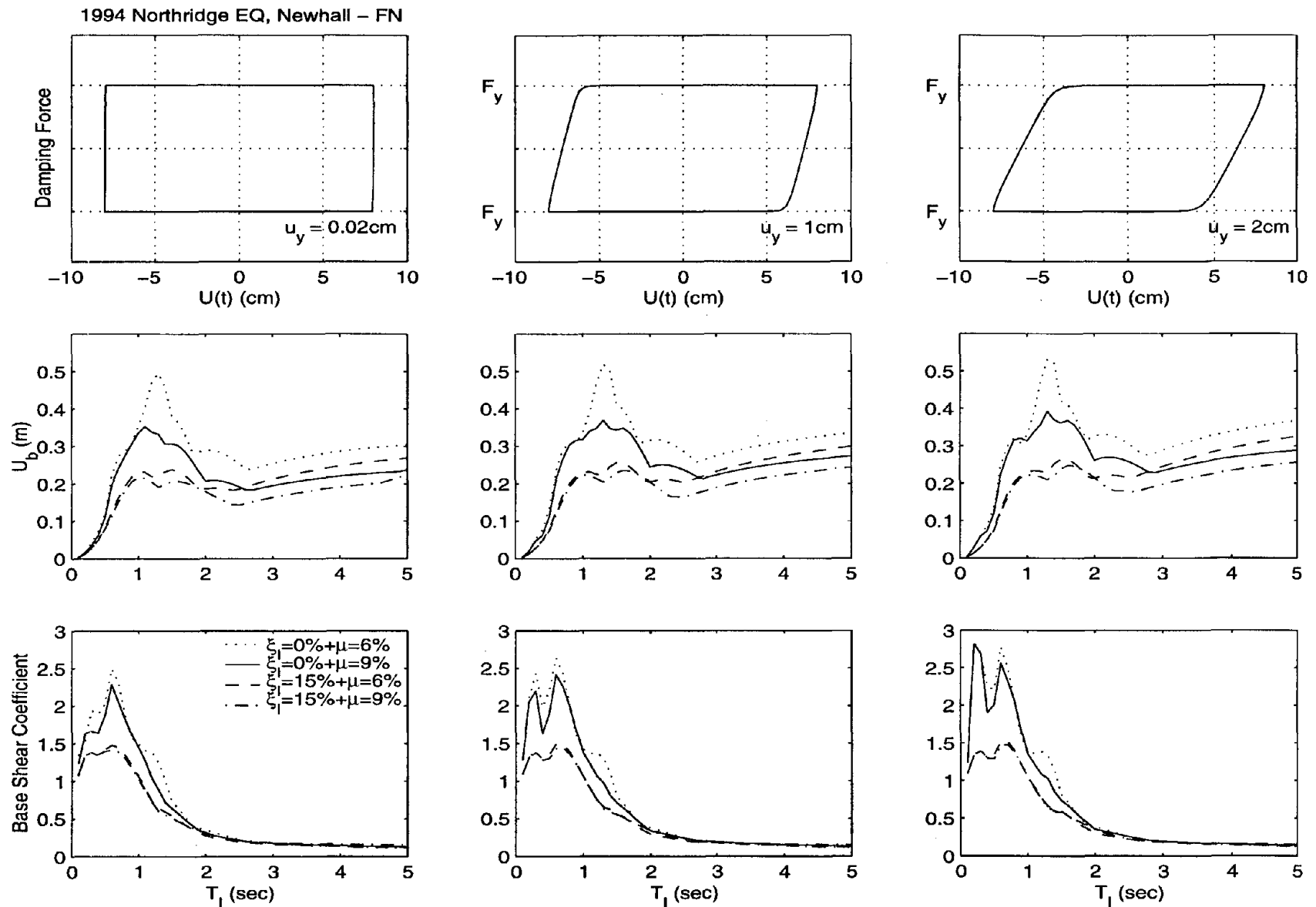
Figure 29: Displacement and base shear spectra of an isolated block subjected to the fault normal component of the Newhall station record. Left: u_y = 0.2 mm; center: u_y = 10 mm; right: u_y = 20 mm.
