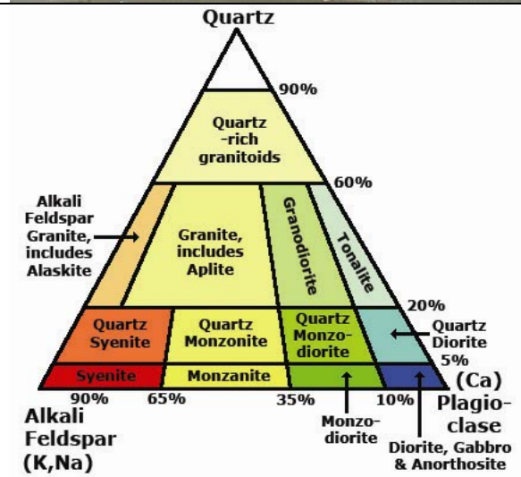
Figure 9-33. Classification of granitic rocks based on composition of feldspars (K-Na-Ca) and quartz. Mafic components are not included (modified classification after igneous petrology chart prepared by the International Union of Geological Sciences and presented by Best, 1982).
