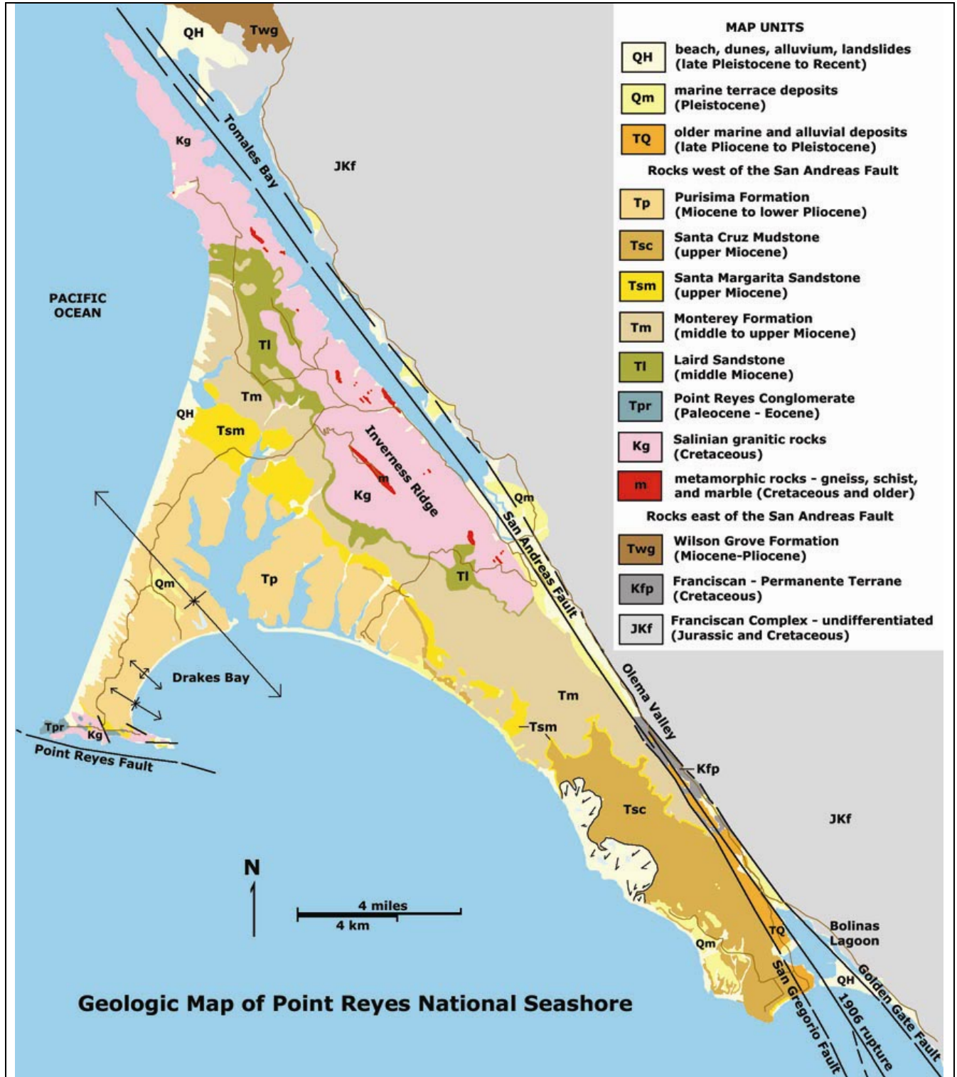
Figure 9-2. Generalized geologic map of Point Reyes National Seashore after Clark and Brabb (1997), Blake and others (2000), and Bruns and others (2002).
