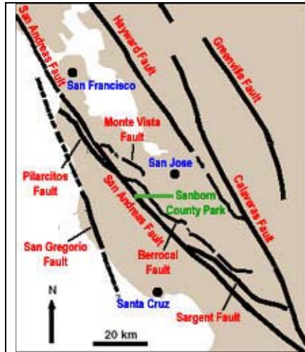
Figure 6-4. The San Andreas Fault System in the San Francisco Bay region.
