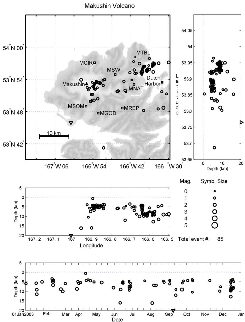
Figure A20. Summary plots of 85 earthquakes located near Makushin Volcano in 2003. Open circles scaled with magnitude show hypocenter locations shallower than 20 km. Hypocenters with depths of 20 km and deeper are shown by open triangles. Hypocenters symbols are scaled with magnitude. Seismograph stations are shown by open squares and labeled by station code. (See Appendix B for station information). Solid triangles are used to show volcanic centers and closed squares are used to show other points of interest.
