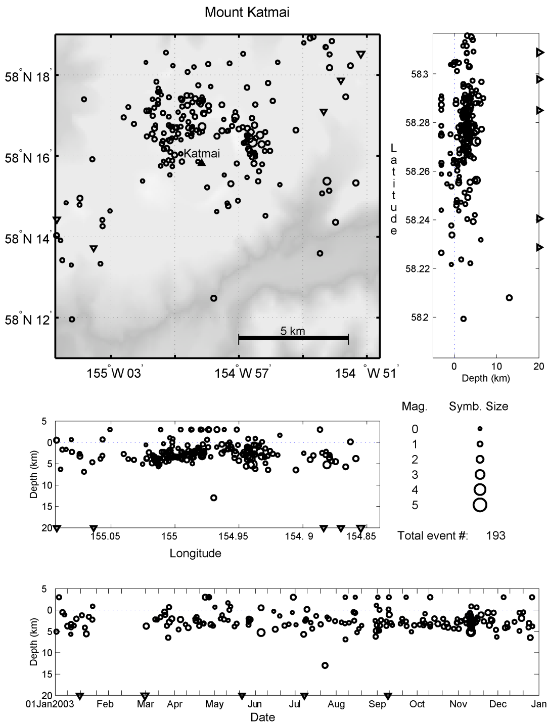
Figure A9. Summary plots of 193 earthquakes located near Mount Katmai in the Katmai volcanic cluster in 2003. Open circles scaled with magnitude show hypocenter locations shallower than 20 km. Hypocenters with depths of 20 km and deeper are shown by open triangles. Hypocenters symbols are scaled with magnitude. Seismograph stations are shown by open squares and labeled by station code. (See Appendix B for station information). Solid triangles are used to show volcanic centers and closed squares are used to show other points of interest.
