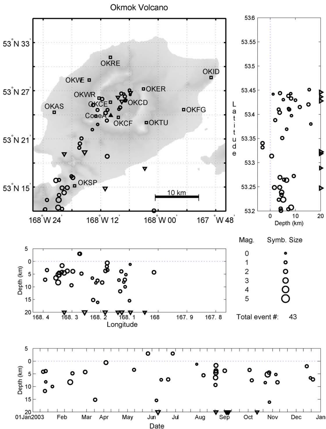
Figure A21. Summary plots of 43 earthquakes located near Okmok Caldera in 2003. Open circles scaled with magnitude show hypocenter locations shallower than 20 km. Hypocenters with depths of 20 km and deeper are shown by open triangles. Hypocenters symbols are scaled with magnitude. Seismograph stations are shown by open squares and labeled by station code. (See Appendix B for station information). Solid triangles are used to show volcanic centers and closed squares are used to show other points of interest.
