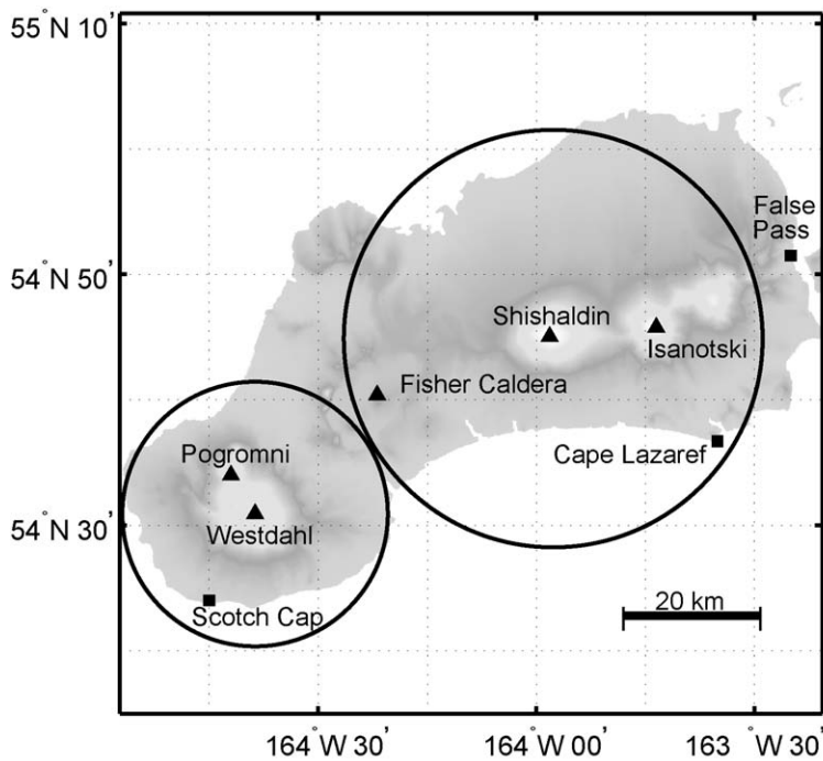
Figure F4. Volcanic zones on Unimak Island. The volcanic zones are modeled using a cylinder centered on Westdahl Peak and a cylinder centered on Shishaldin Volcano.
