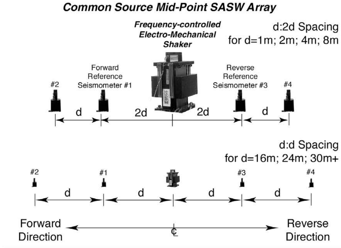
Figure 4. Configuration of the USGS surface wave testing system, composed of 1-Hz sensors and a 100 kg electro-mechanical shakers. Array separation changes from d:2d to d:d for large array separations when signal strength to the outermost receivers is weak.
