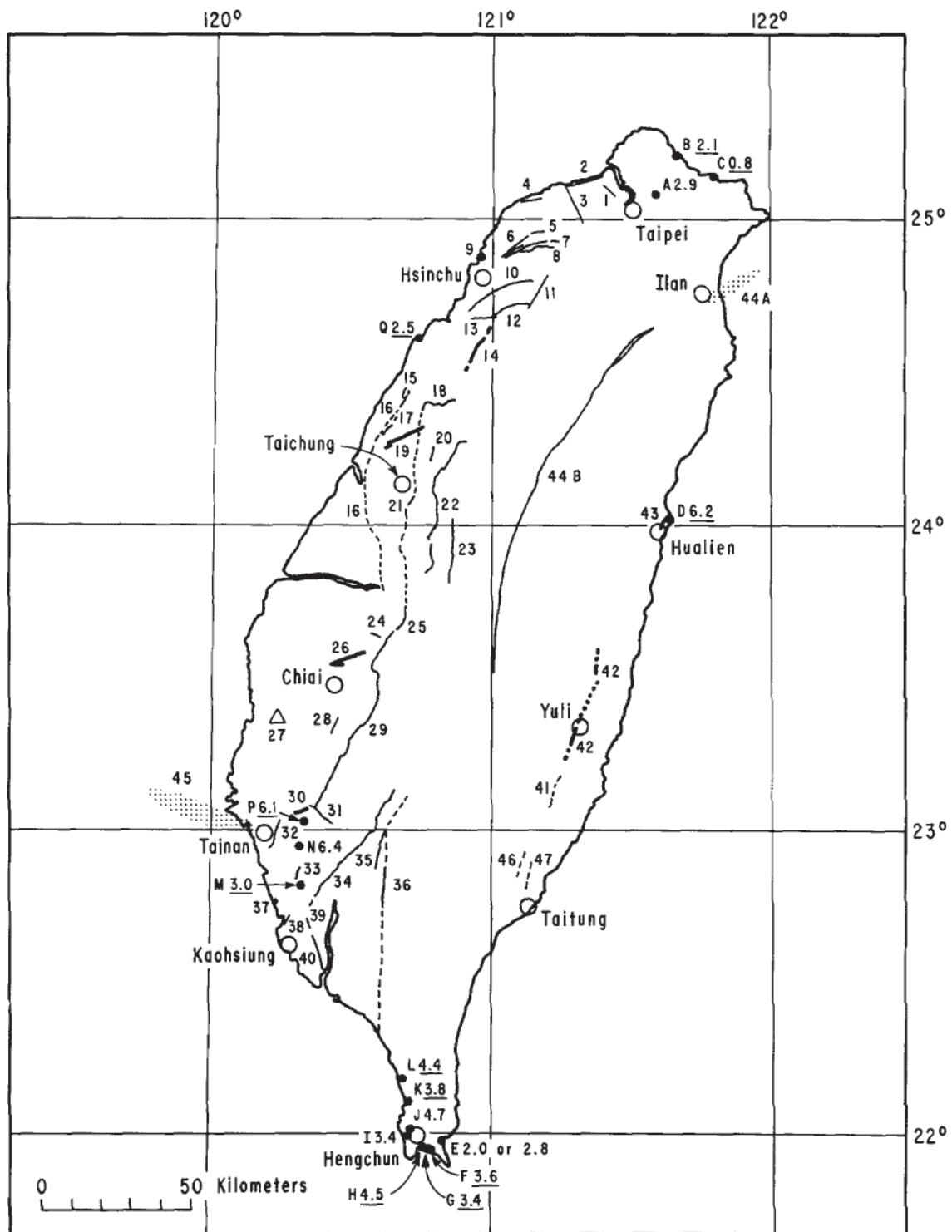
Figure 1. Map of Taiwan showing faults that cut Quaternary deposits. From Bonilla (1977, fig. 1). Surface ruptures (heavy lines) occurred in 1935 on faults numbered 14 and 19; in 1906 on fault number 26; in 1946 on fault 30; and in 1951 in eastern Taiwan on faults numbered 43 (October) and 42 (November). Alignments of epicenters (pattern of dots) at 44A (Tsai and others 1975) and 45 (Tsai and Chiu 1976) indicate concealed historically active faults. Letters A-Q and their associated numbers should be ignored as they relate to a preliminary estimate of rates of Holocene uplift.
