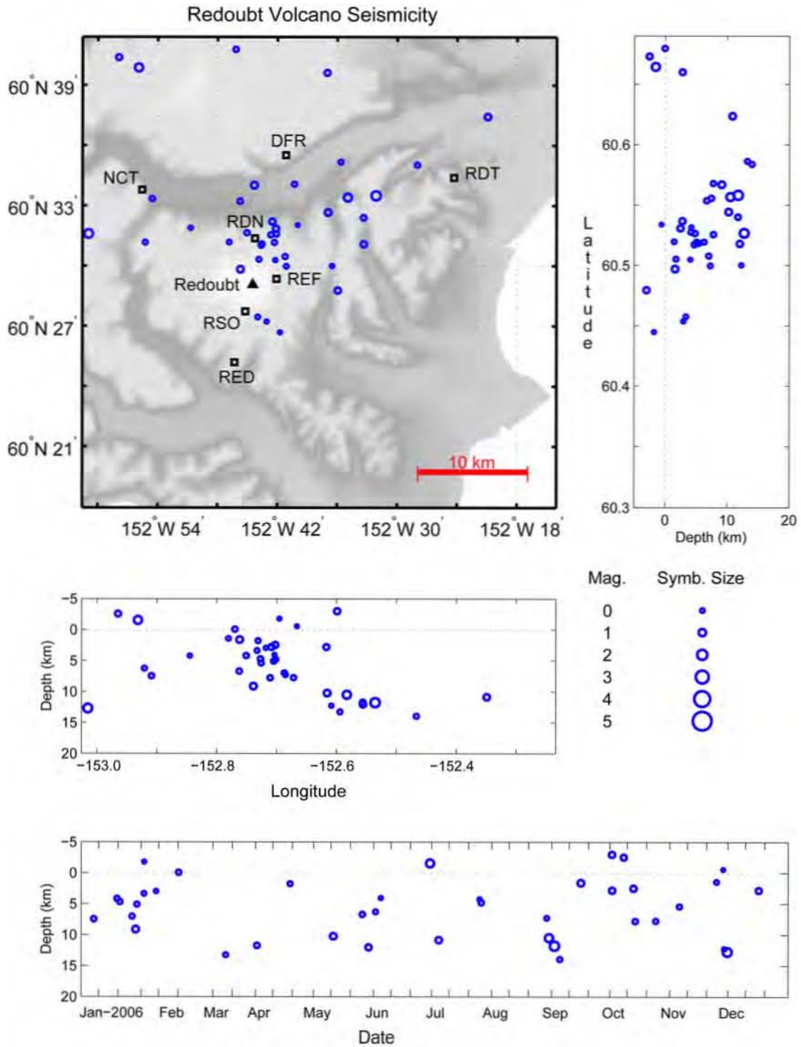
Figure A3. Summary plots of earthquakes located near Redoubt Volcano in 2006. Open circles scaled with magnitude show hypocenter locations. Permanent seismograph stations are shown by open squares and labeled by station code. Solid triangles are used to show volcanic centers. See appendix B for station information.
