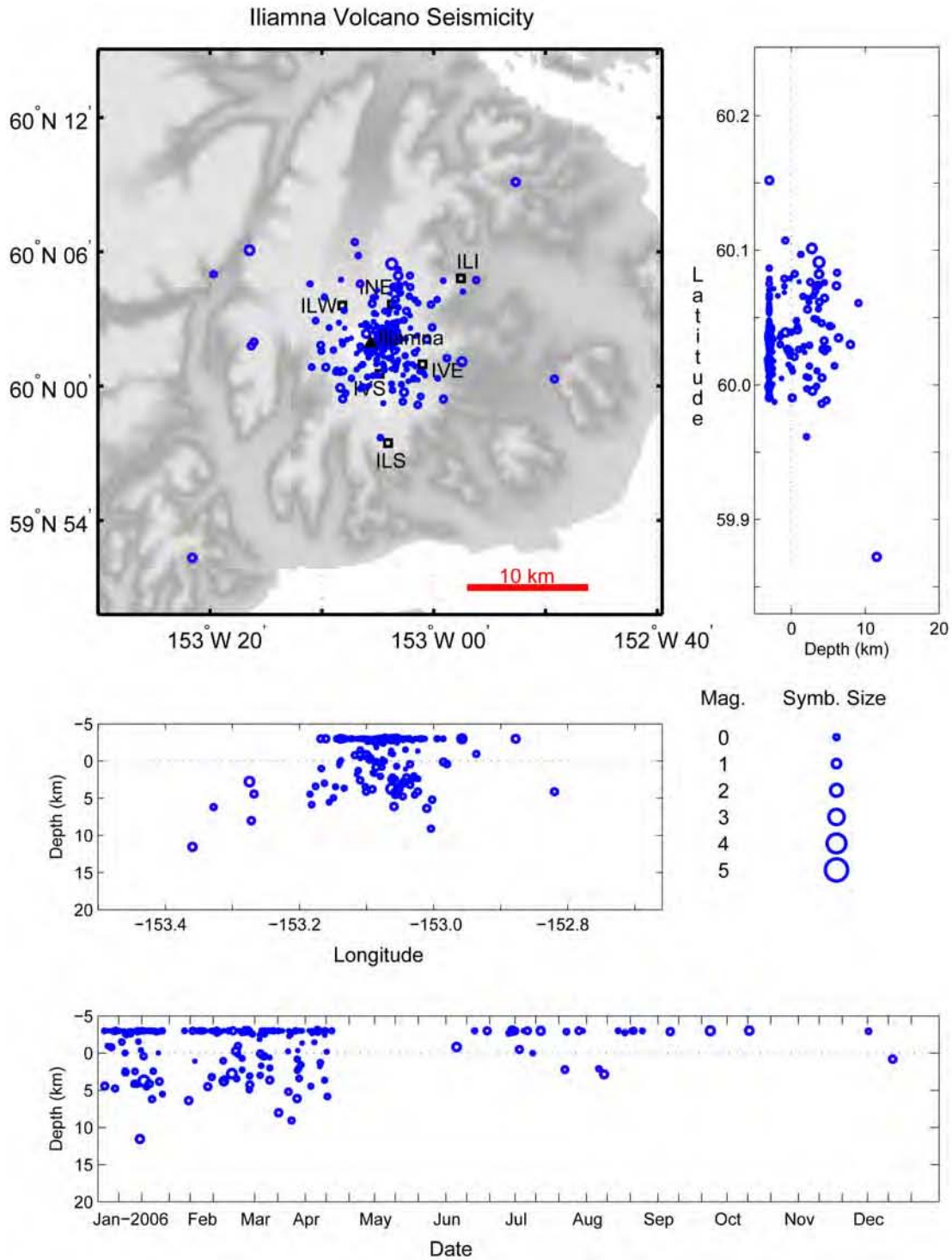
Figure A4. Summary plots of earthquakes located near Iliamna Volcano in 2006. Open circles scaled with magnitude show hypocenter locations. Permanent seismicograph stations are shown by open squares and labeled by station code. Solid triangles are used to show volcanic centers. See appendix B for station information.
