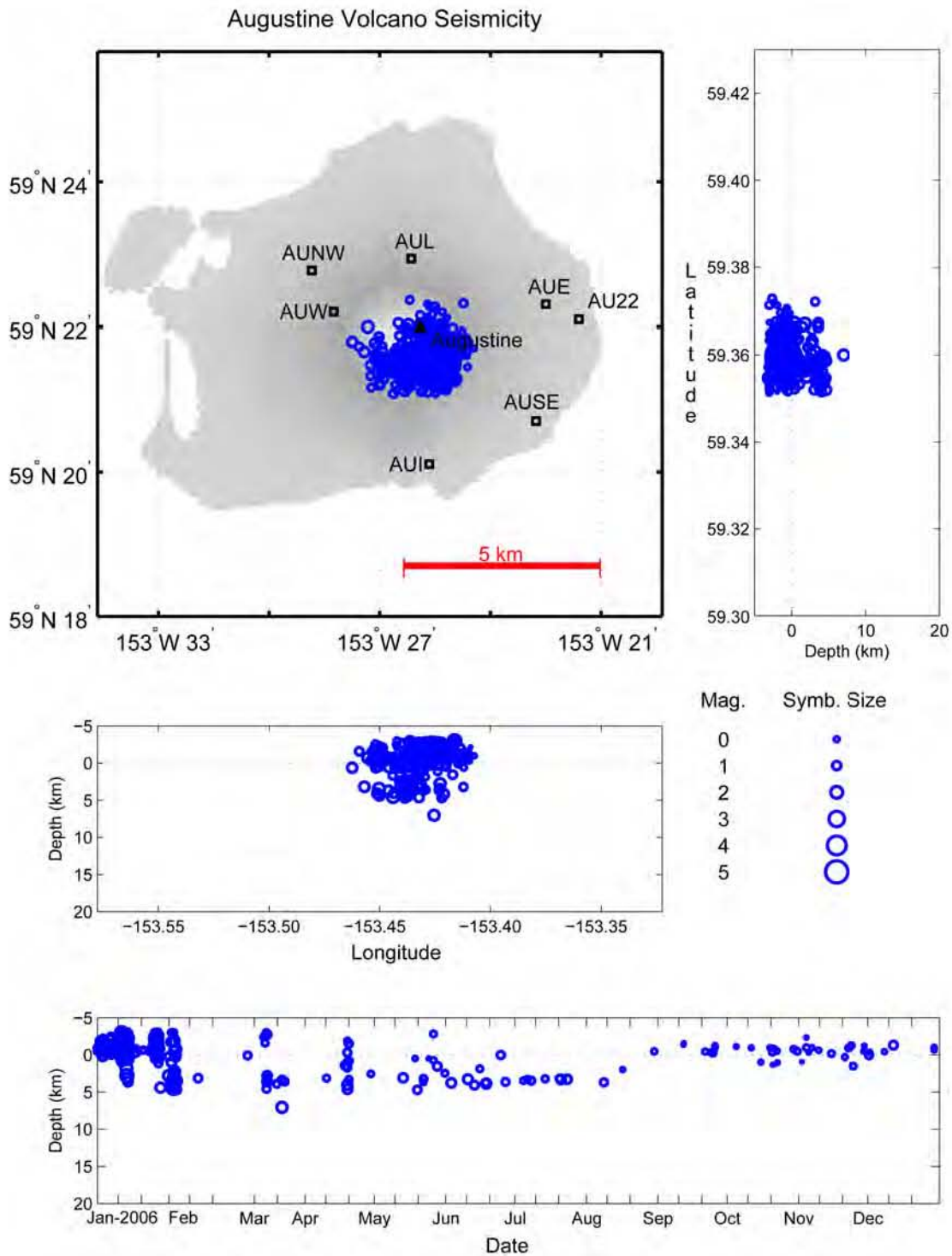
Figure A5. Summary plots of earthquakes located near Augustine Volcano in 2006. Open circles scaled with magnitude show hypocenter locations. Permanent seismicograph stations are shown by open squares and labeled by station code. Solid triangles are used to show volcanic centers. See appendix B for station information. See text for a discussion on hypocenter depths.
