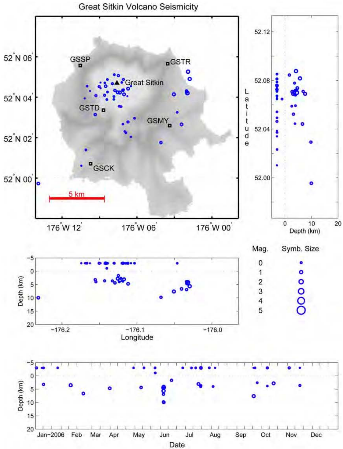
Figure A25. Summary plots of earthquakes located near Great Sitkin Volcano in 2006. Open circles scaled with magnitude show hypocenter locations. Permanent seismicograph stations are shown by open squares and labeled by station code. Solid triangles are used to show volcanic centers. See appendix B for station information.
