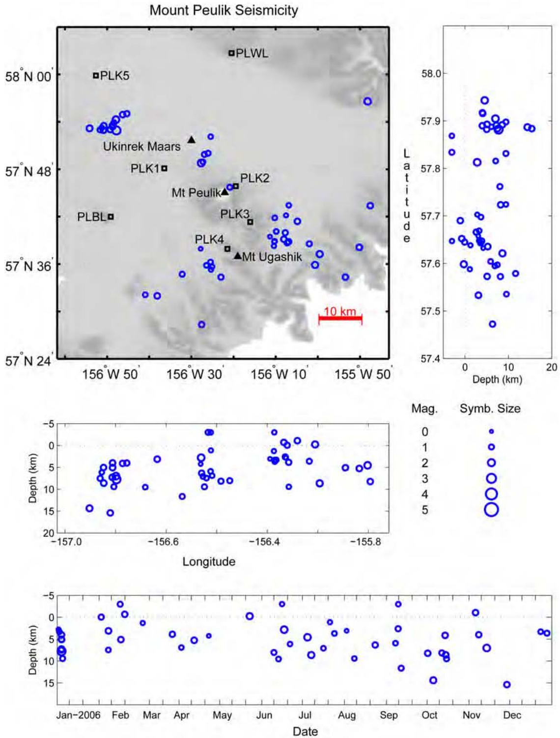
Figure A13. Summary plots of earthquakes located near Mount Peulik in 2006. Open circles scaled with magnitude show hypocenter locations. Permanent seismograph stations are shown by open squares and labeled by station code. Solid triangles are used to show volcanic centers. See appendix B for station information.
