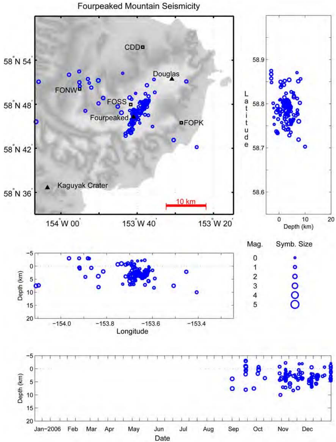
Figure A6. Summary plots of earthquakes located near Fourpeaked Mountain in 2006. Open circles scaled with magnitude show hypocenter locations. Permanent seismograph stations are shown by open squares and labeled by station code. Solid triangles are used to show volcanic centers. See appendix B for station information.
