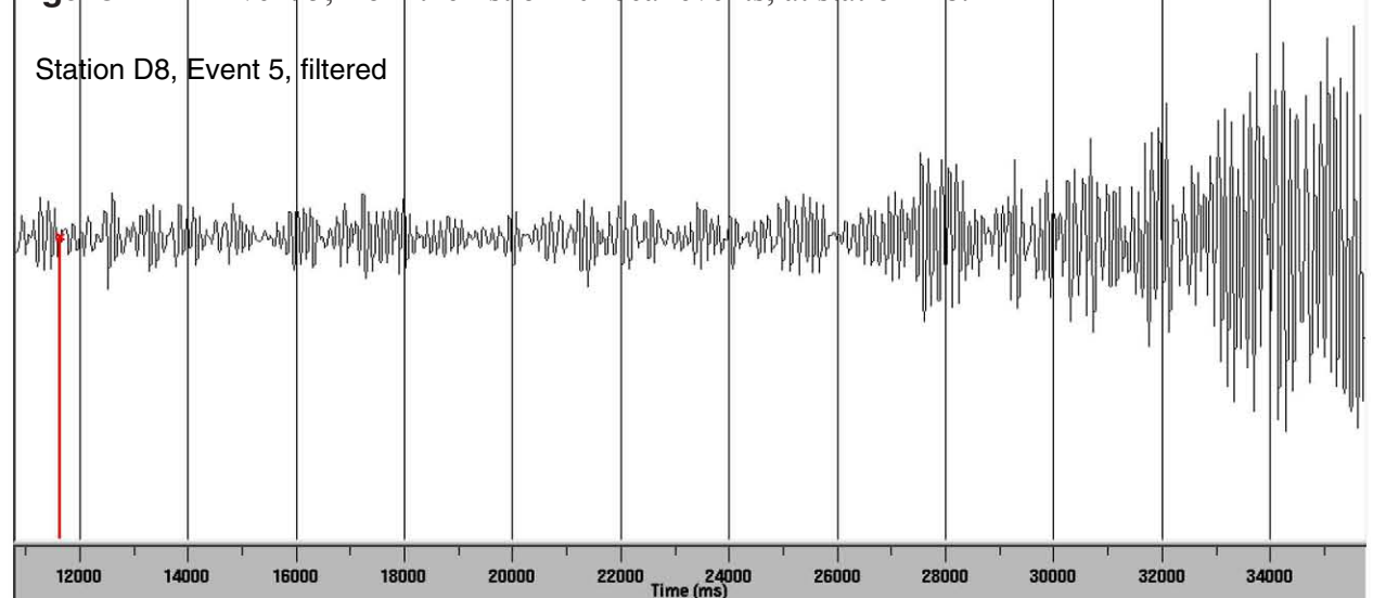
Figure B42. Event 5, from the list of 20 local events, at station D8.
