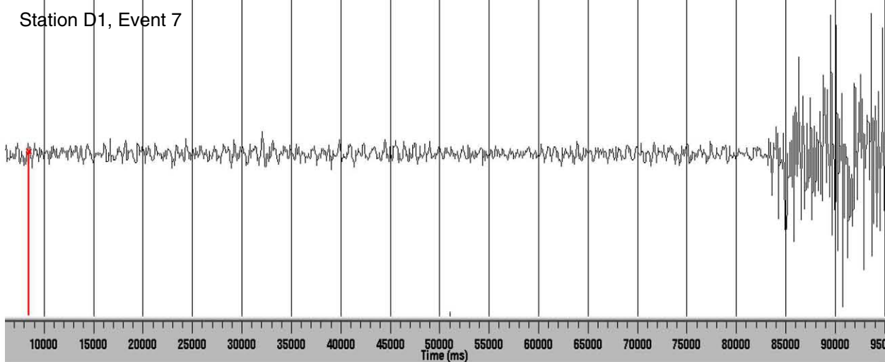
Figure B28. Event 7, from the list of 20 local events, at station D1.
