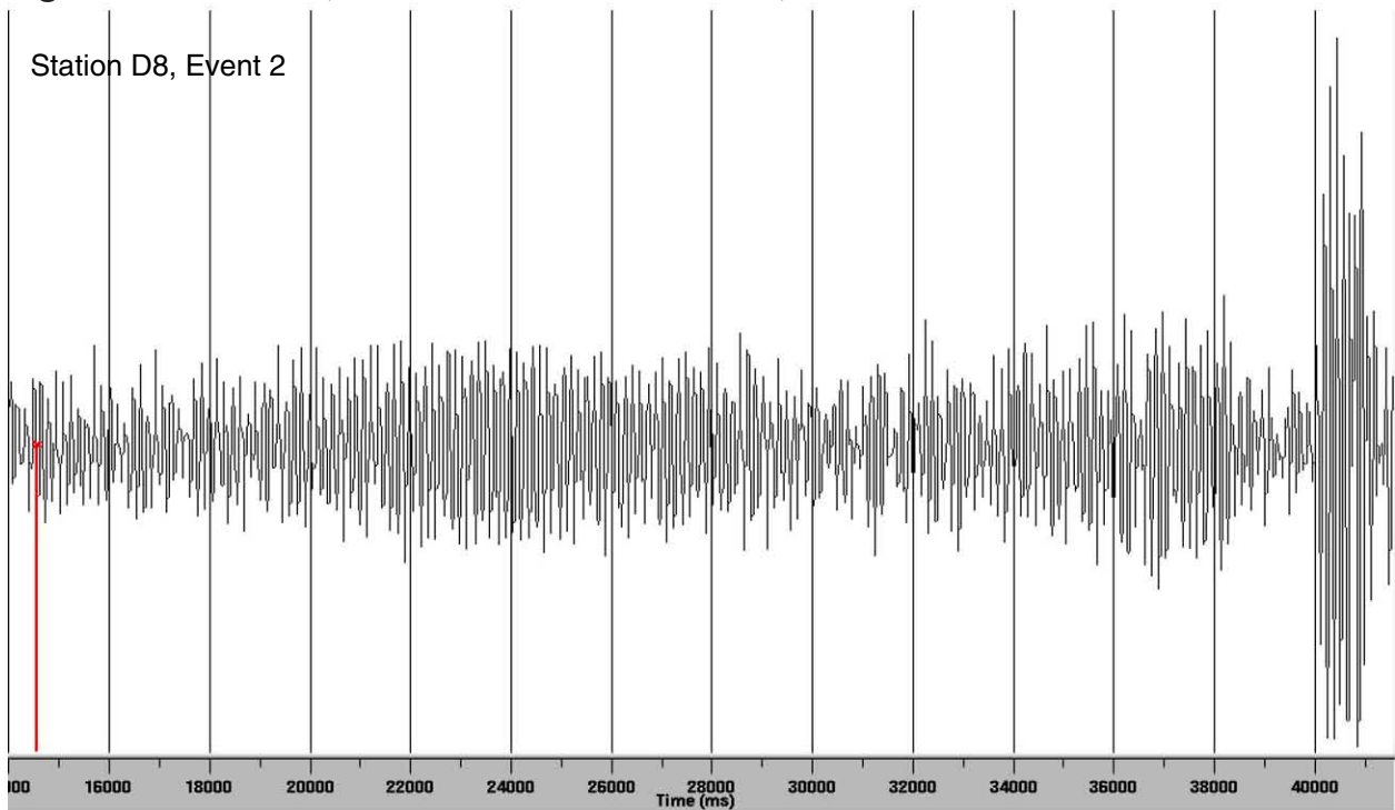
Figure B40. Event 2, from the list of 20 local events, at station D8.
