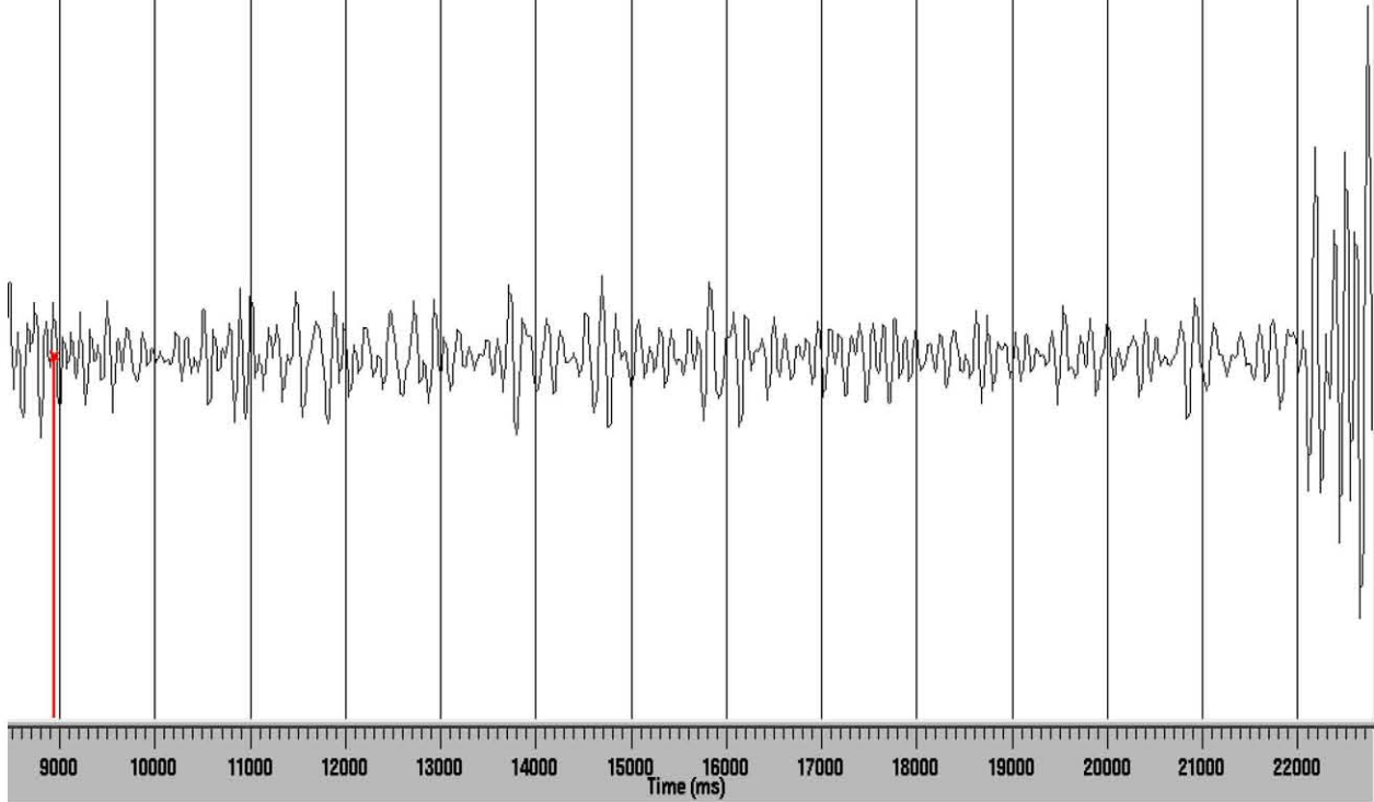
Figure B53. Event 3, from the list of 20 local events, at station A2.
