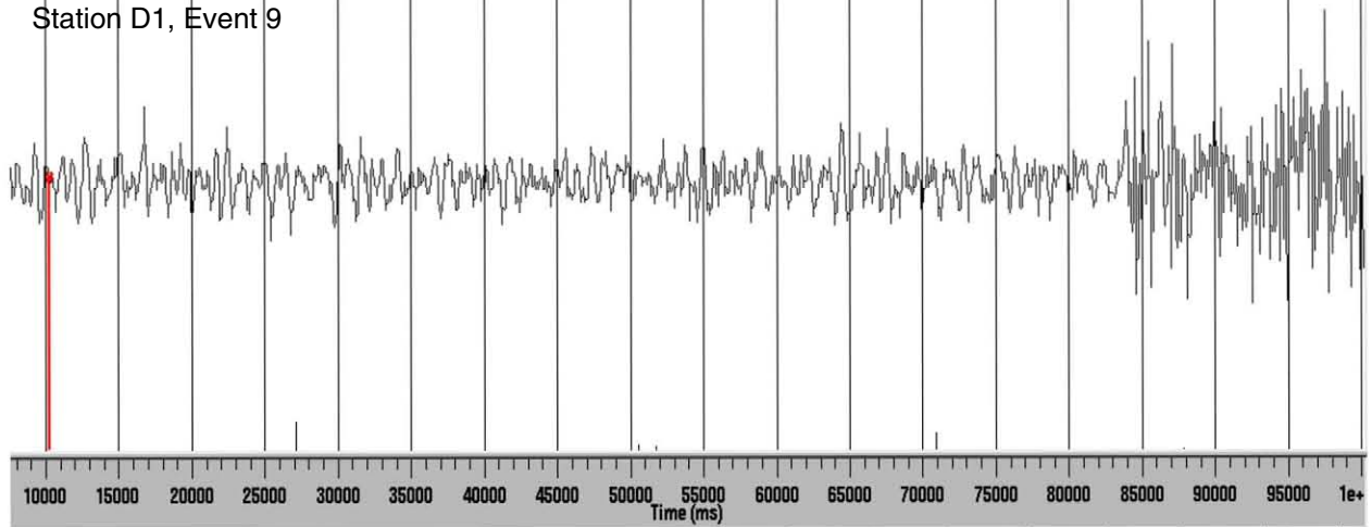
Figure B30. Event 10, from the list of 20 local events, at station D1.
