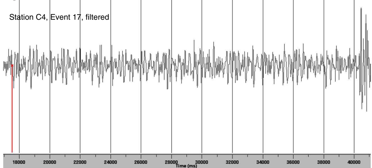
Figure B22. Event 17, from the list of 20 local events, at station C4.
