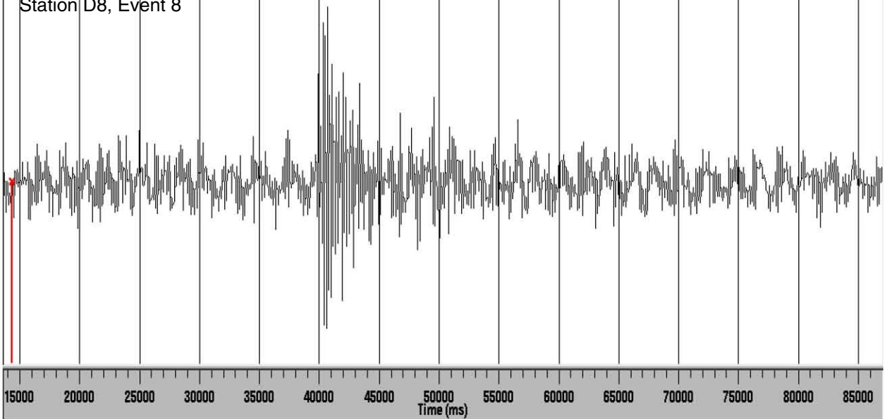
Figure B44. Event 8, from the list of 20 local events, at station D8.
