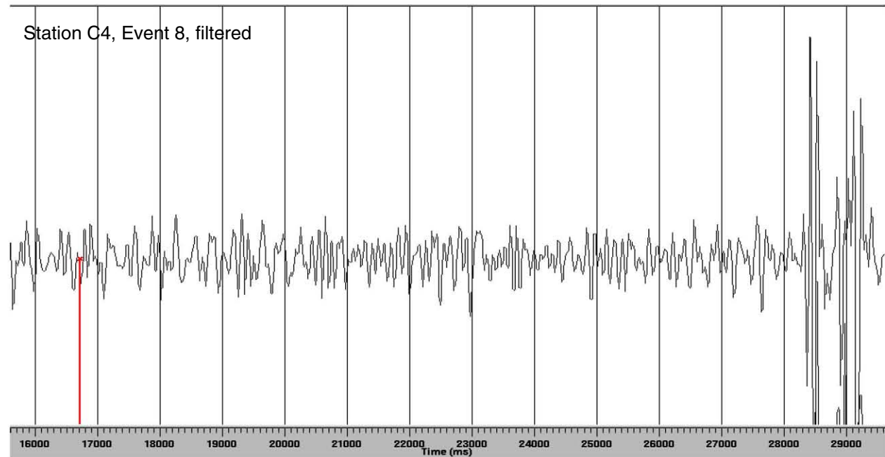
Figure B17. Event 8, from the list of 20 local events, at station C4.
