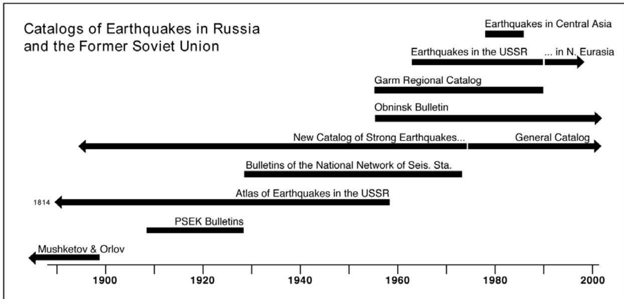
Figure 3. Publication date ranges for the principal Russian and Soviet catalogs of seismicity.
