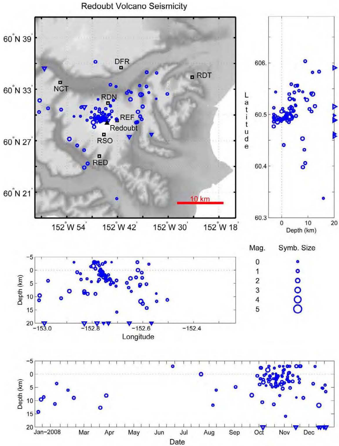
Figure A3. Summary plots of earthquakes located near Redoubt Volcano in 2008. Open circles show hypocenter locations shallower than 20 km and open triangles indicate times of hypocenters with depths of 20 km and deeper. Hypocenter symbols are scaled with magnitude. Permanent seismograph stations are shown by open squares and labeled by station code. Solid triangles are used to show volcanic centers. See appendix B for station information.
