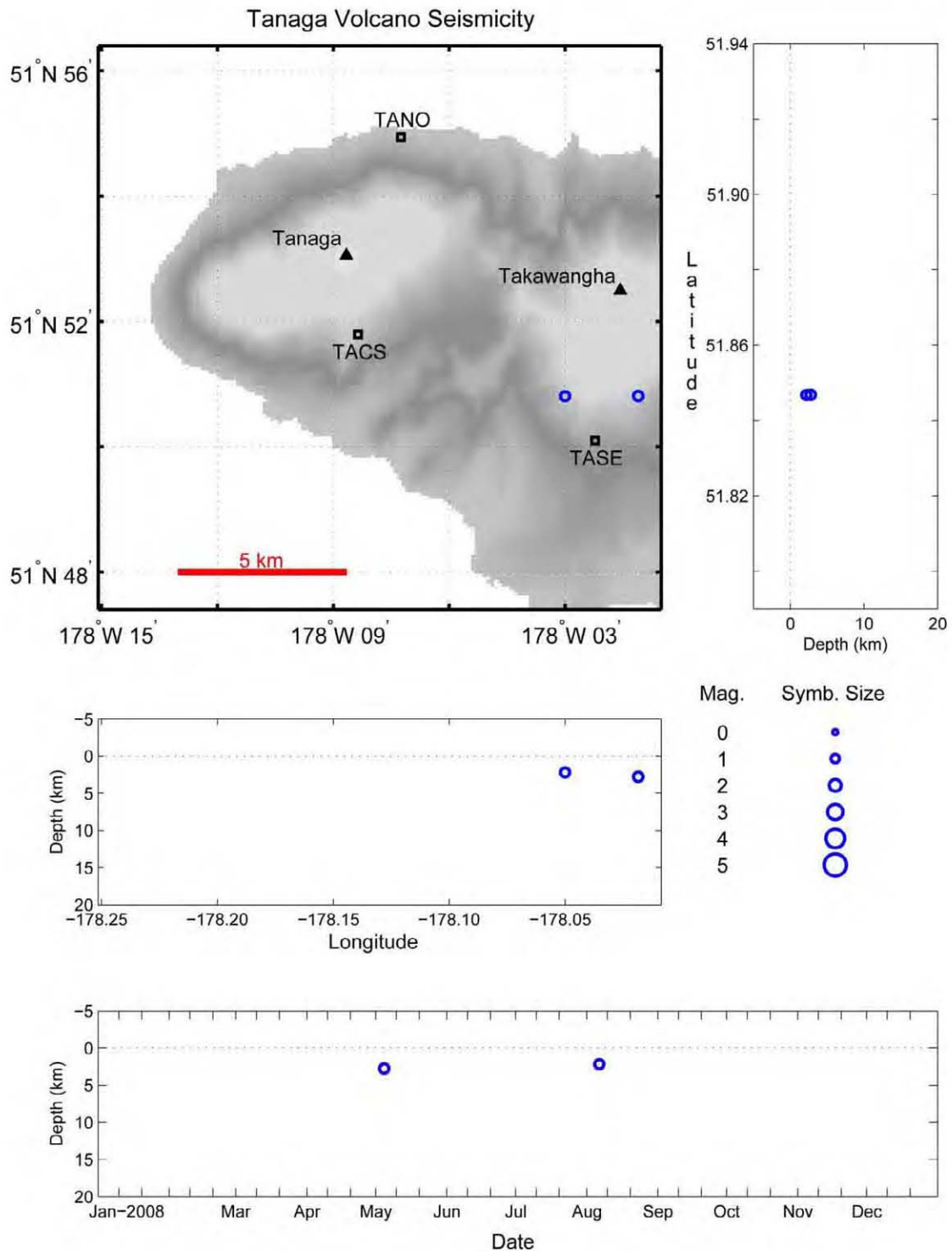
Figure A29. Summary plots of earthquake located near Tanaga Volcano in 2008. Most earthquakes associated with the Tanaga volcanic center do not plot on this figure but to the east as seen on figure A28. Open circles show hypocenter locations shallower than 20 km. Hypocenter symbols are scaled with magnitude. Permanent seismograph stations are shown by open squares and labeled by station code. Solid triangles are used to show volcanic centers. See appendix B for station information.
