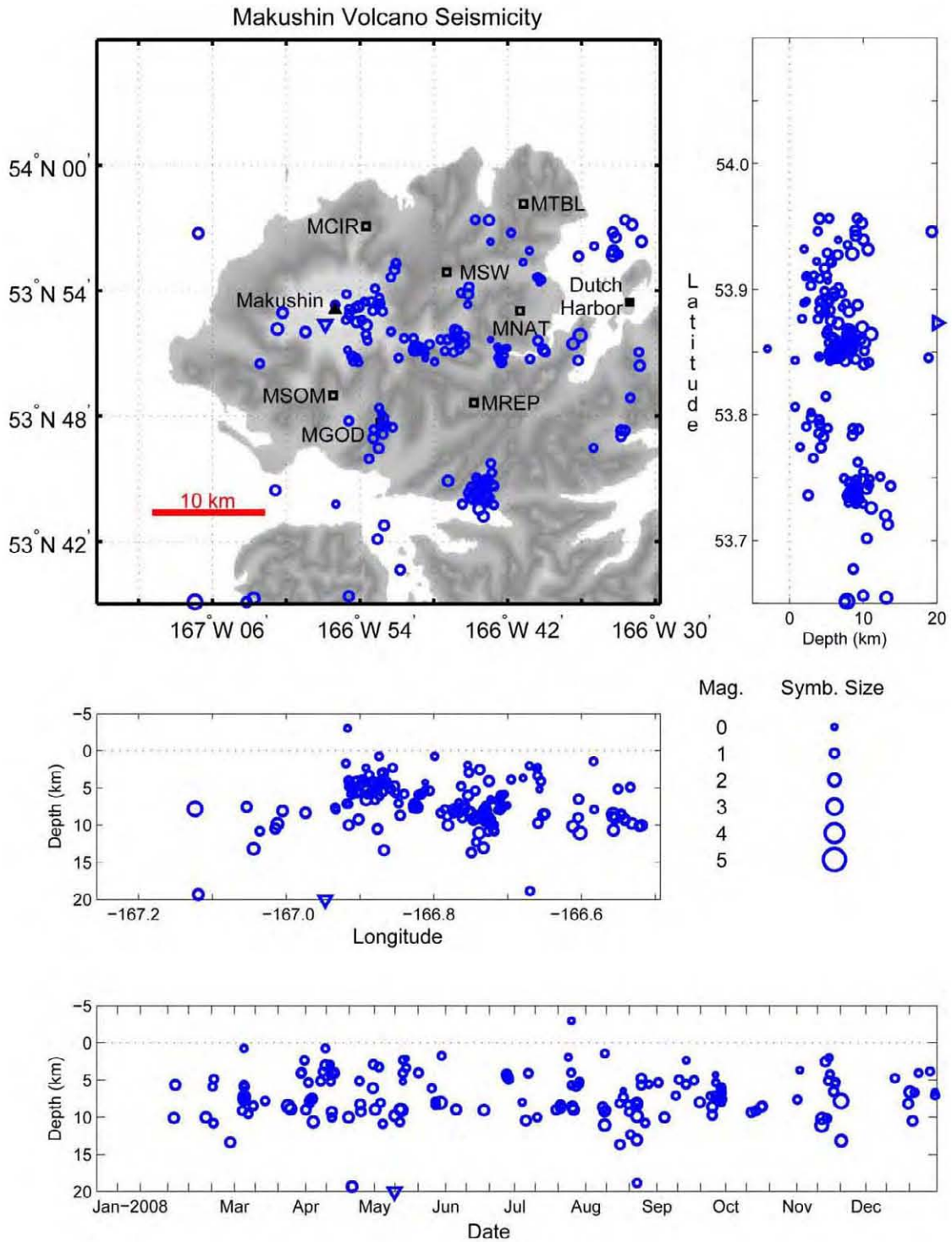
Figure A22. Summary plots of earthquakes located near Makushin Volcano in 2008. Open circles show hypocenter locations shallower than 20 km and open triangles indicate times of hypocenters with depths of 20 km and deeper. Hypocenter symbols are scaled with magnitude. Permanent seismograph stations are shown by open squares and labeled by station code. Solid triangles are used to show volcanic centers and solid squares are used to show other points of interest. See appendix B for station information.
