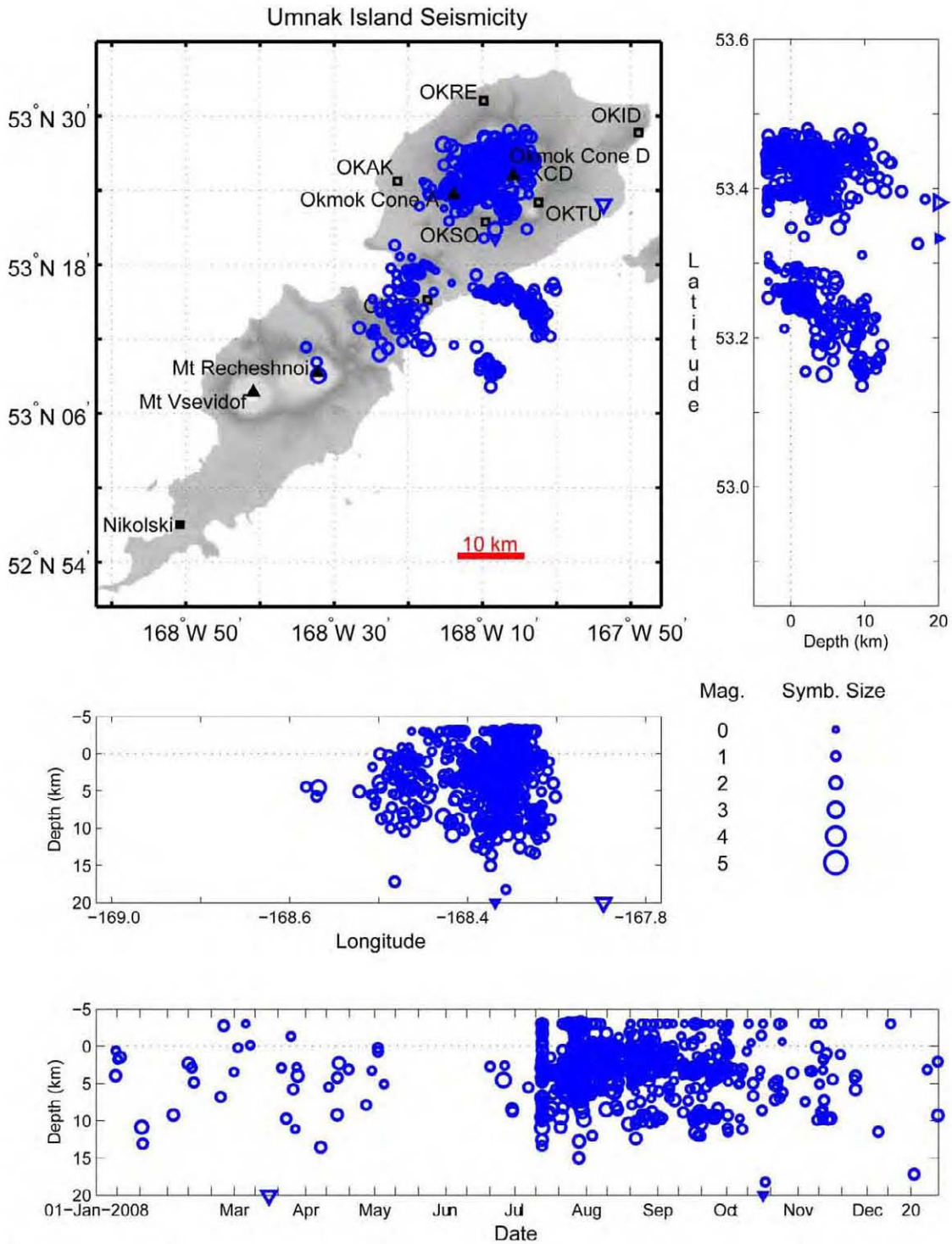
Figure A23. Summary plots of earthquakes located on Umnak Island in 2008. Open circles show hypocenter locations shallower than 20 km and open triangles indicate times of hypocenters with depths of 20 km and deeper. Hypocenter symbols are scaled with magnitude. Permanent seismograph stations are shown by open squares and labeled by station code. Solid triangles are used to show volcanic centers and solid squares are used to show other points of interest. See appendix B for station information.
