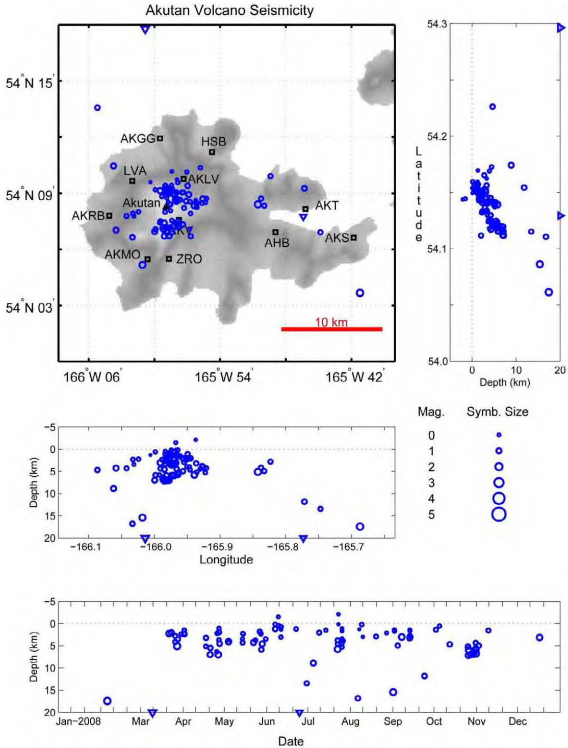
Figure A21. Summary plots of earthquakes located near Akutan Peak in 2008. Open circles show hypocenter locations shallower than 20 km and open triangles indicate times of hypocenters with depths of 20 km and deeper. Hypocenter symbols are scaled with magnitude. Permanent seismograph stations are shown by open squares and labeled by station code. Solid triangles are used to show volcanic centers. See appendix B for station information.
