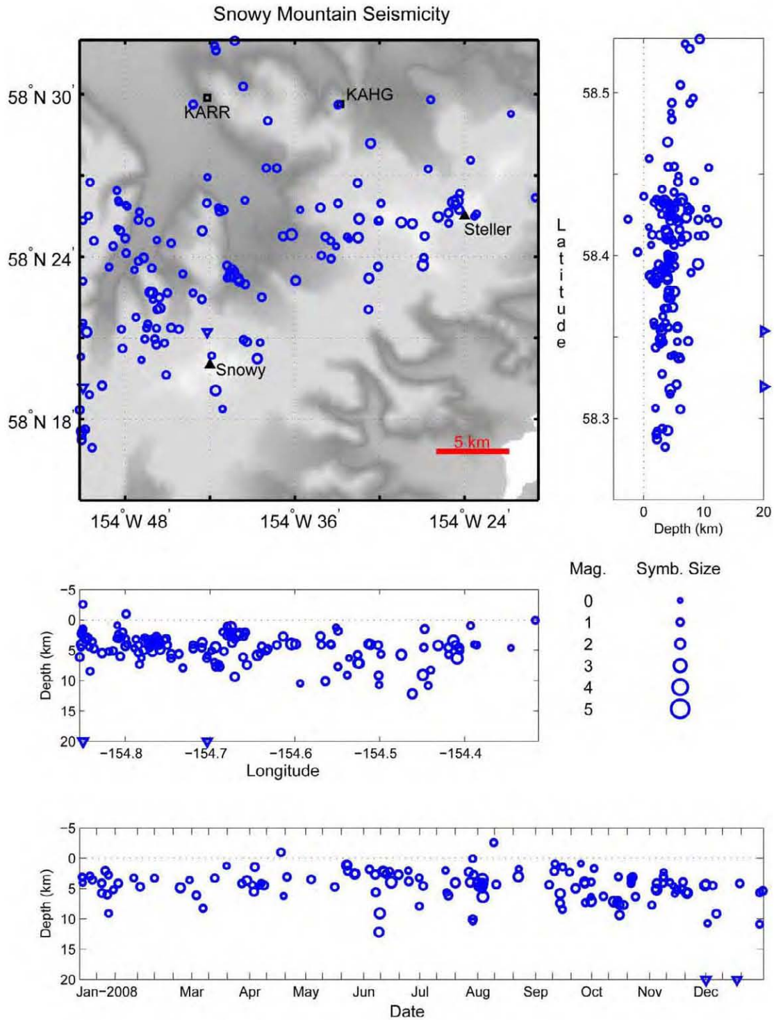
Figure A8. Summary plots of earthquakes located near Snowy Mountain in the Katmai volcanic cluster in 2008. Open circles show hypocenter locations shallower than 20 km and open triangles indicate times of hypocenters with depths of 20 km and deeper. Hypocenter symbols are scaled with magnitude. Permanent seismograph stations are shown by open squares and labeled by station code. Solid triangles are used to show volcanic centers. See appendix B for station information.
