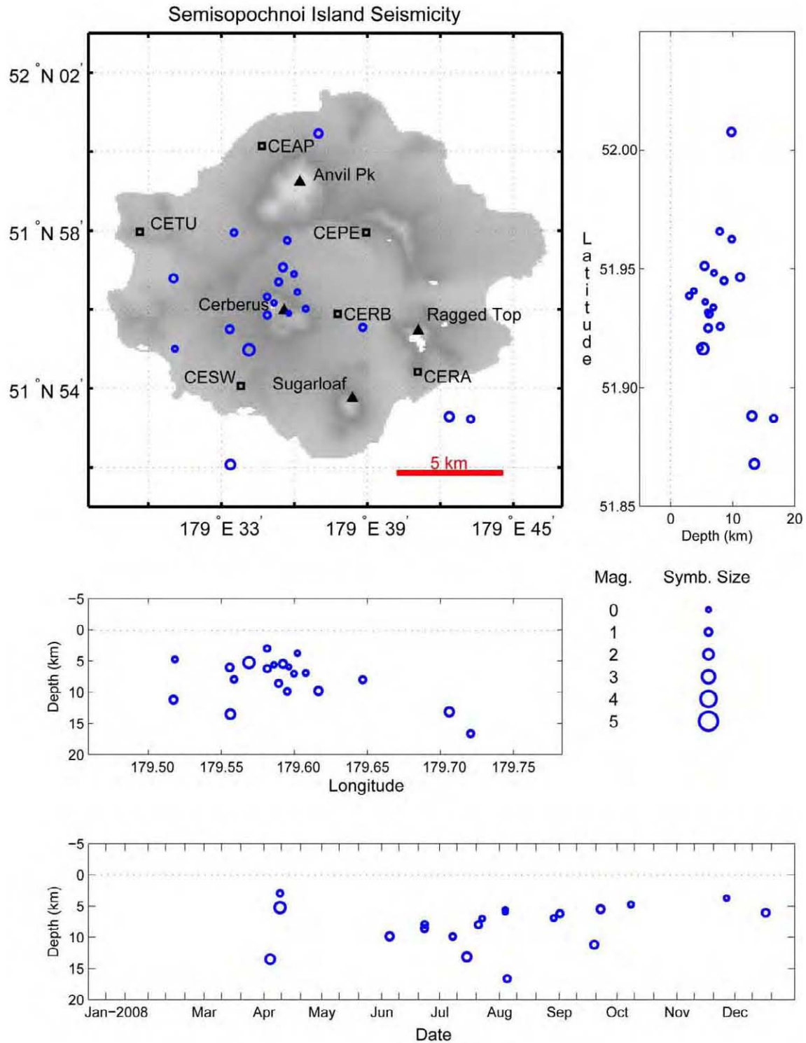
Figure A31. Summary plots of earthquakes located on Semisopochnoi Island in 2008. Open circles show hypocenter locations shallower than 20 km. Hypocenter symbols are scaled with magnitude. Permanent seismograph stations are shown by open squares and labeled by station code. Solid triangles are used to show volcanic centers. See appendix B for station information.
