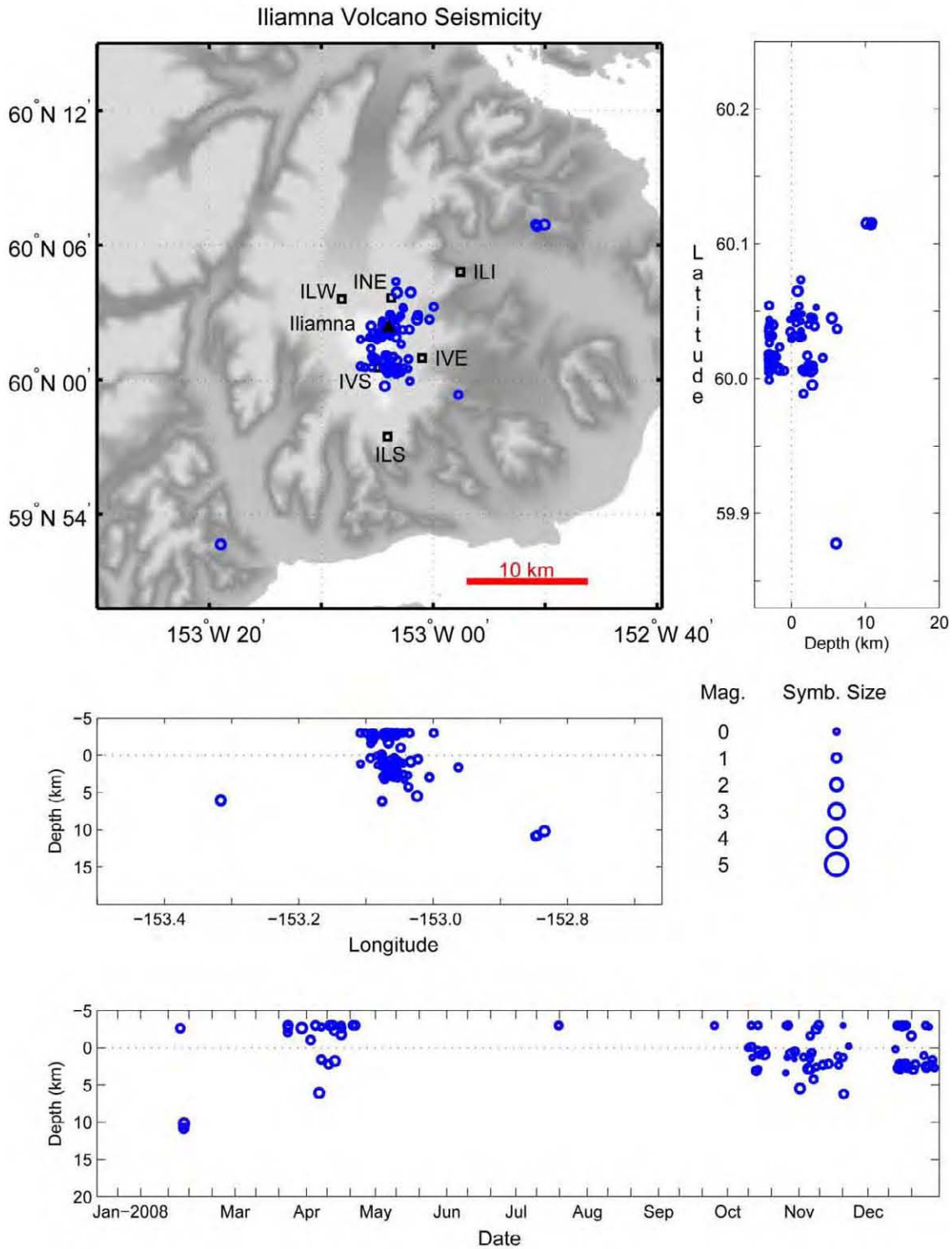
Figure A4. Summary plots of earthquakes located near Iliamna Volcano in 2008. Open circles scaled with magnitude show hypocenter locations. Hypocenter symbols are scaled with magnitude. Permanent seismograph stations are shown by open squares and labeled by station code. Solid triangles are used to show volcanic centers. See appendix B for station information.
