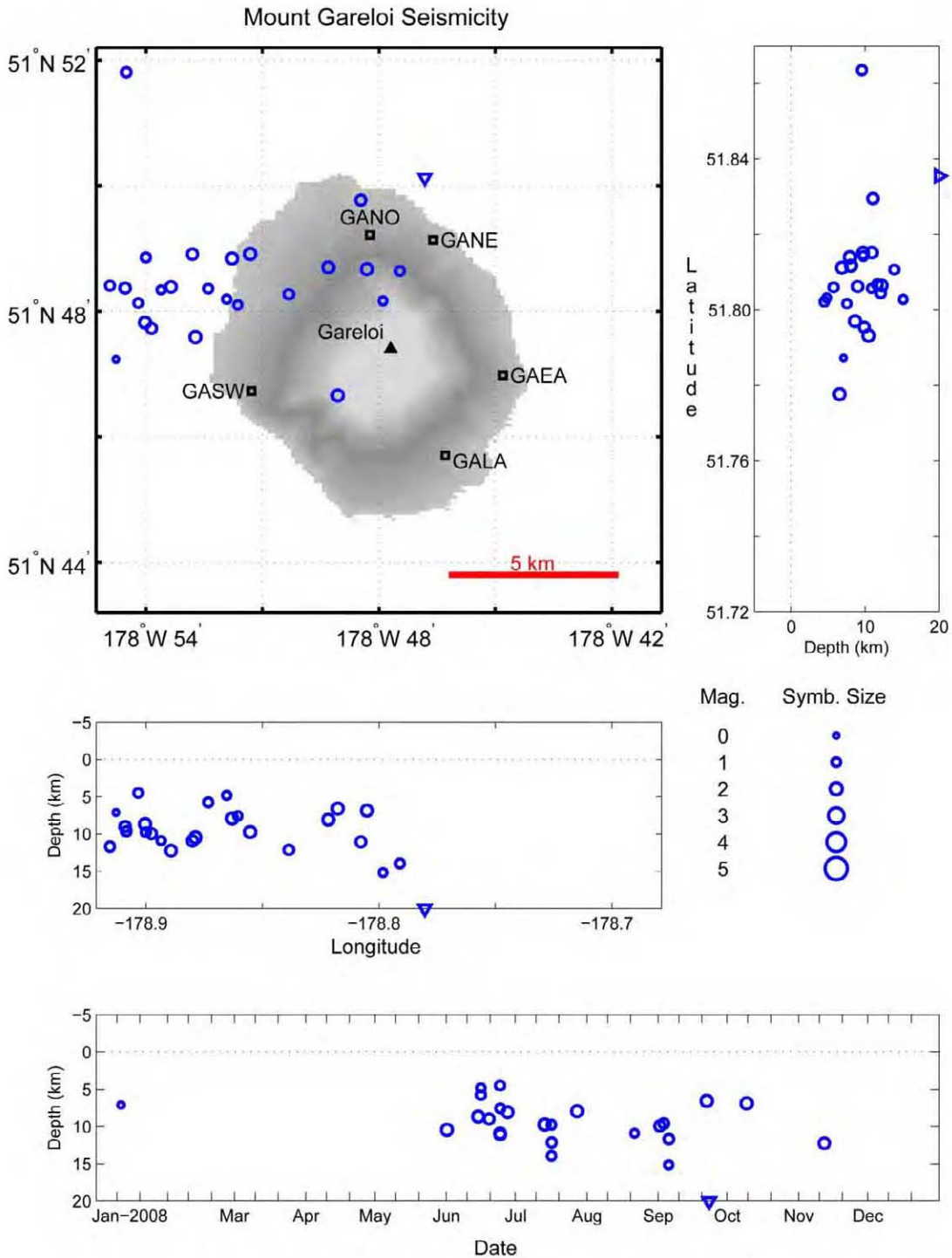
Figure A30. Summary plots of earthquakes located near Mount Gareloi in 2008. Open circles show hypocenter locations shallower than 20 km and open triangles indicate times of hypocenters with depths of 20 km and deeper. Hypocenter symbols are scaled with magnitude. Permanent seismograph stations are shown by open squares and labeled by station code. Solid triangles are used to show volcanic centers. See appendix B for station information.
