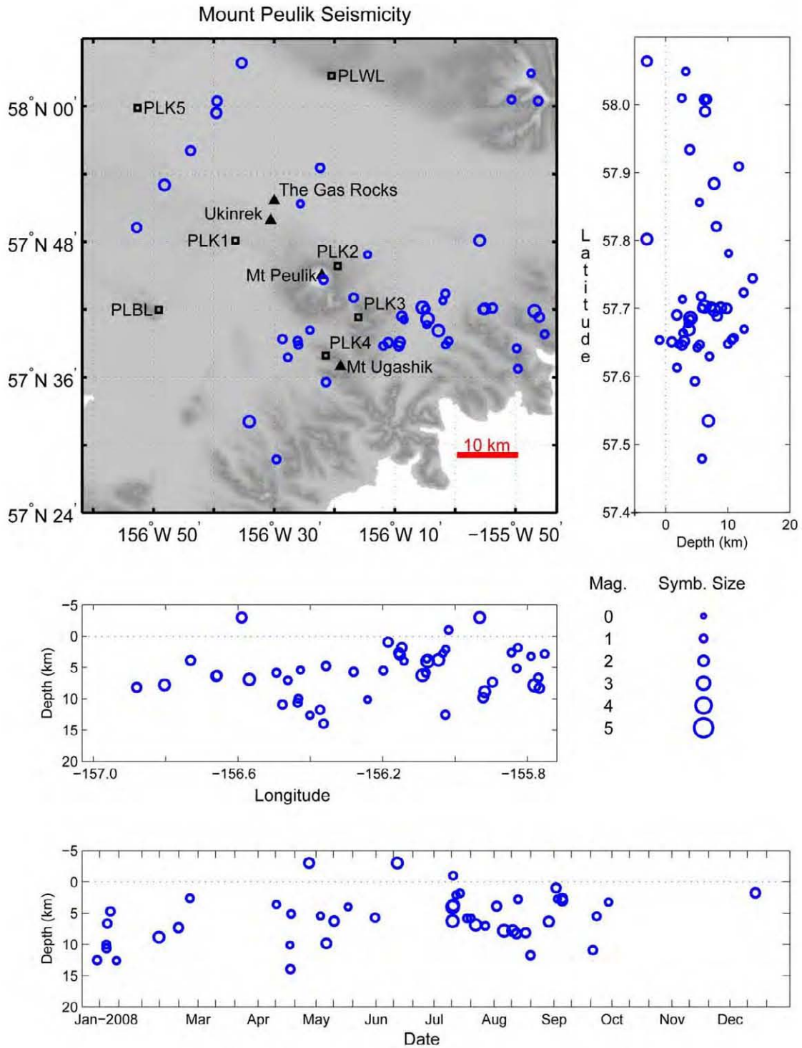
Figure A13. Summary plots of earthquakes located near Mount Peulik in 2008. Open circles show hypocenter locations shallower than 20 km. Hypocenter symbols are scaled with magnitude. Permanent seismograph stations are shown by open squares and labeled by station code. Solid triangles are used to show volcanic centers. See appendix B for station information.
