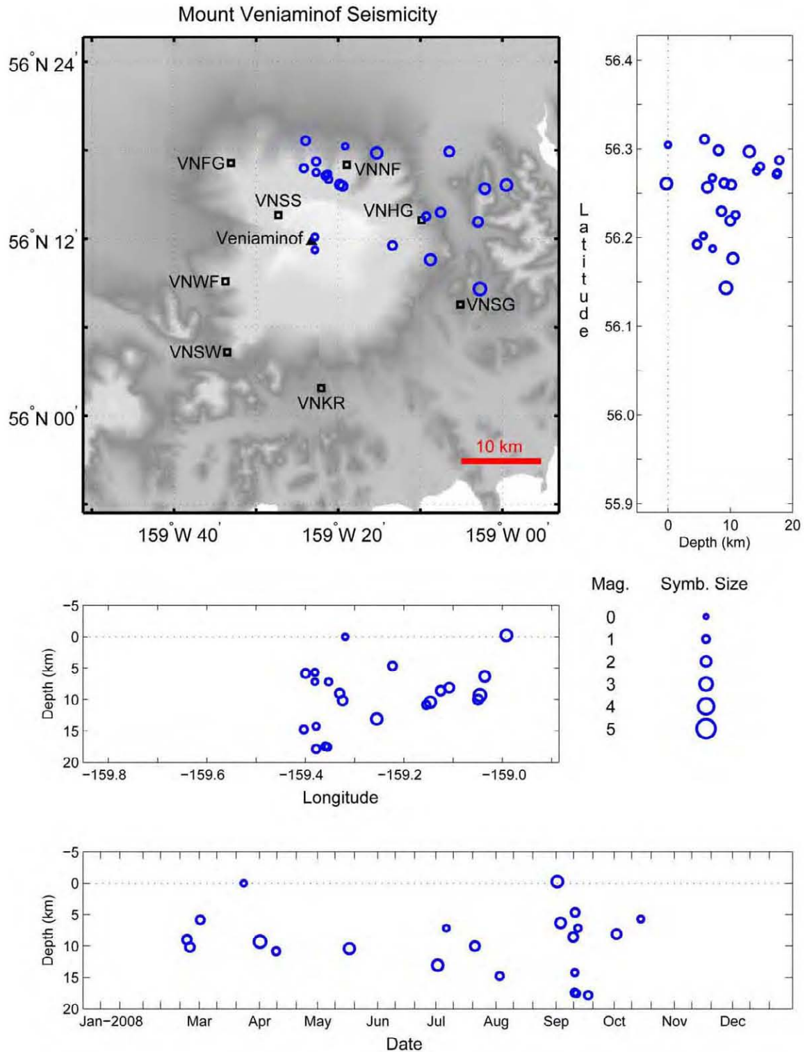
Figure A15. Summary plots of earthquakes located near Mount Veniaminof in 2008. Open circles show hypocenter locations shallower than 20 km. Hypocenter symbols are scaled with magnitude. Permanent seismograph stations are shown by open squares and labeled by station code. Solid triangles are used to show volcanic centers. See appendix B for station information.
