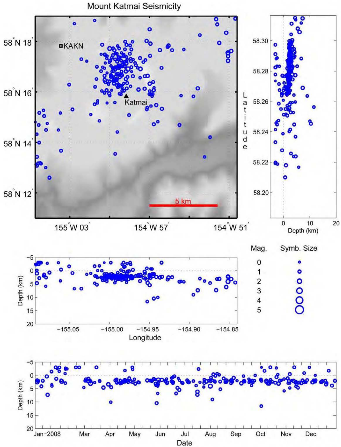
Figure A10. Summary plots of earthquakes located near Mount Katmai in the Katmai volcanic cluster in 2008. Open circles scaled with magnitude show hypocenter locations. Hypocenter symbols are scaled with magnitude. Permanent seismograph stations are shown by open squares and labeled by station code. Solid triangles are used to show volcanic centers. See appendix B for station information. Several earthquakes that appear on this figure appear on other figures.
