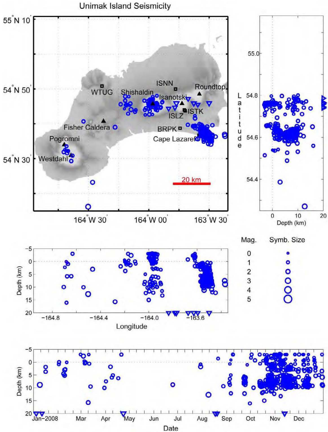
Figure A18. Summary plots of earthquakes located near Unimak Island in 2008. Open circles show hypocenter locations shallower than 20 km and open triangles indicate times of hypocenters with depths of 20 km and deeper. Hypocenter symbols are scaled with magnitude. Permanent seismograph stations are shown by open squares and labeled by station code. Solid triangles are used to show volcanic centers. See appendix B for station information.
