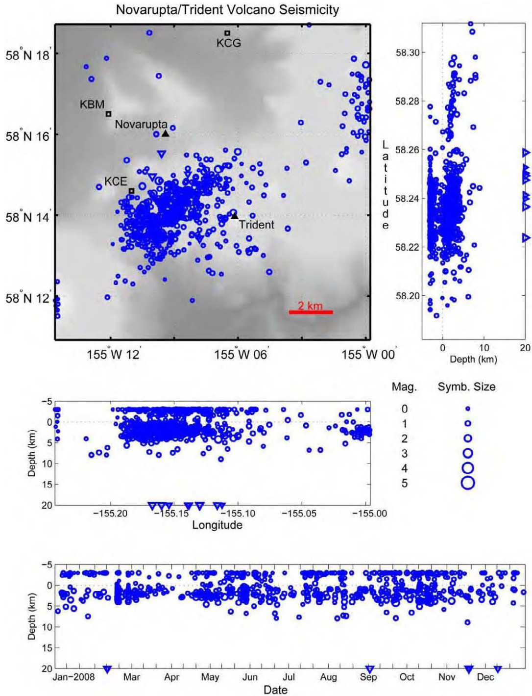
Figure A11. Summary plots of earthquakes located near Novarupta and Trident Volcano in the Katmai volcanic cluster in 2008. Open circles show hypocenter locations shallower than 20 km and open triangles indicate times of hypocenters with depths of 20 km and deeper. Hypocenter symbols are scaled with magnitude. Permanent seismicograph stations are shown by open squares and labeled by station code. Solid triangles are used to show volcanic centers. See appendix B for station information. Several earthquakes that appear on this figure appear on other figures.
