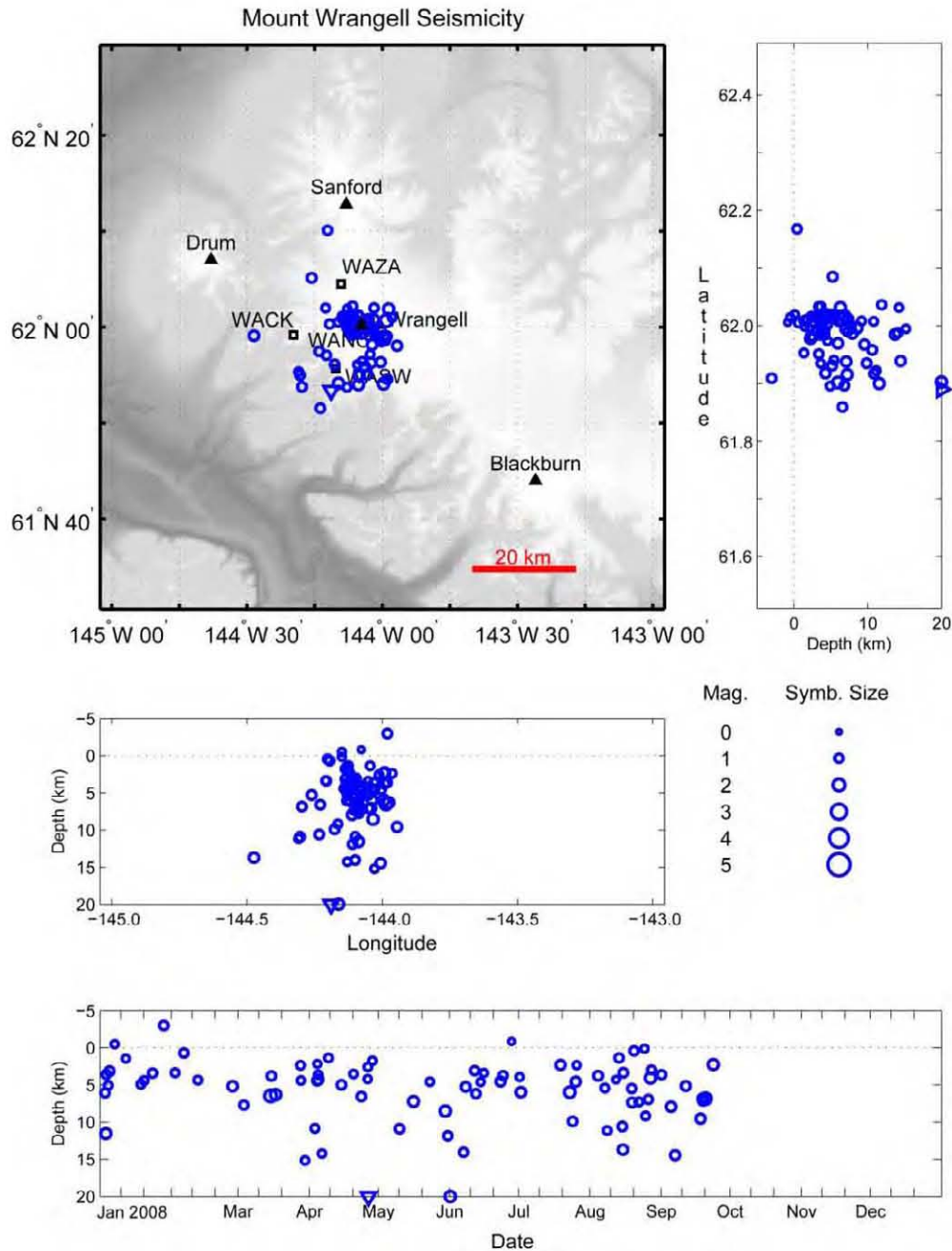
Figure A1. Summary plots of earthquakes located near Mount Wrangell in 2008. Open circles show hypocenter locations shallower than 20 km and open triangles indicate times of hypocenters with depths of 20 km and deeper. Hypocenter symbols are scaled with magnitude. Permanent seismograph stations are shown by open squares and labeled by station code. Solid triangles are used to show volcanic centers. See appendix B for station information.
