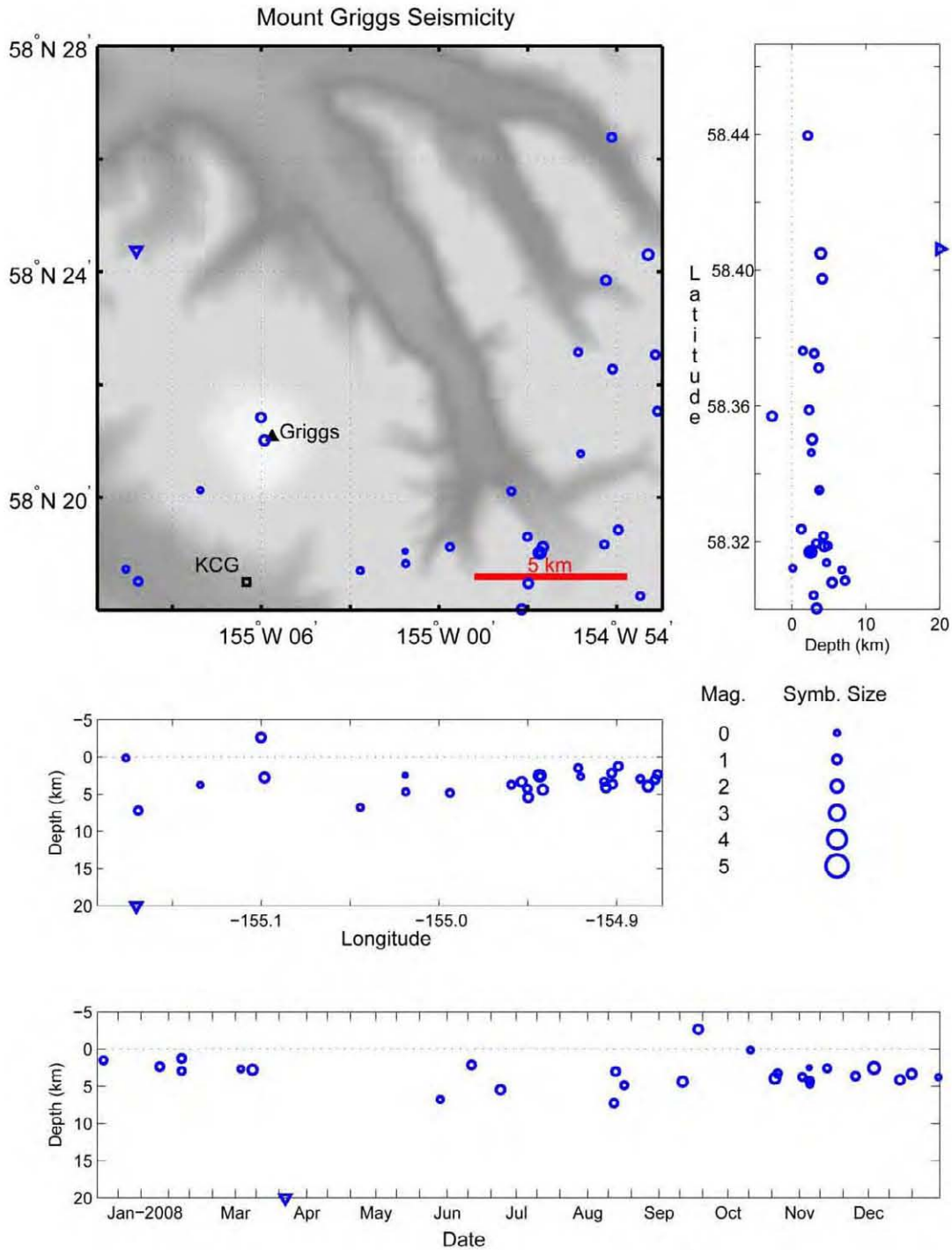
Figure A9. Summary plots of earthquakes located near Mount Griggs in the Katmai volcanic cluster in 2008. Open circles show hypocenter locations shallower than 20 km and open triangles show hypocenters with depths of 20 km and deeper. Hypocenter symbols are scaled with magnitude. Permanent seismograph stations are shown by open squares and labeled by station code. Solid triangles are used to show volcanic centers. See appendix B for station information. Several earthquakes that appear on this figure appear on other figures.
