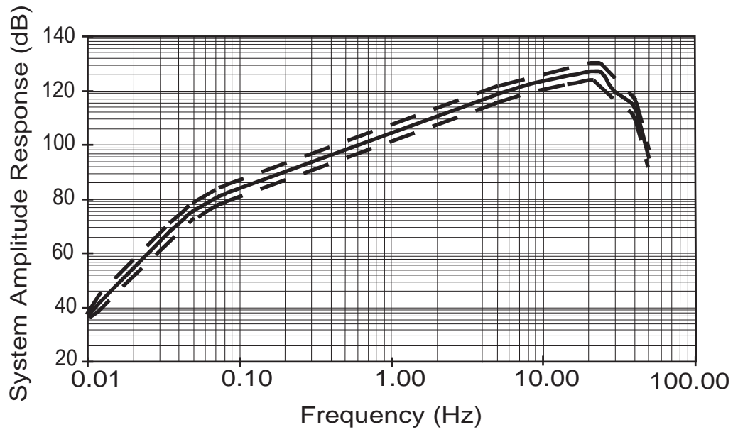
Figure 5. Log-log plot of representative displacement response curves for the broadband stations using a Guralp CMG-40T seismometer. The solid line illustrates the typical calibration curve and the dashed lines show the range of calibration curves for all AVO stations using Guralp CMG-40T seismometers.
