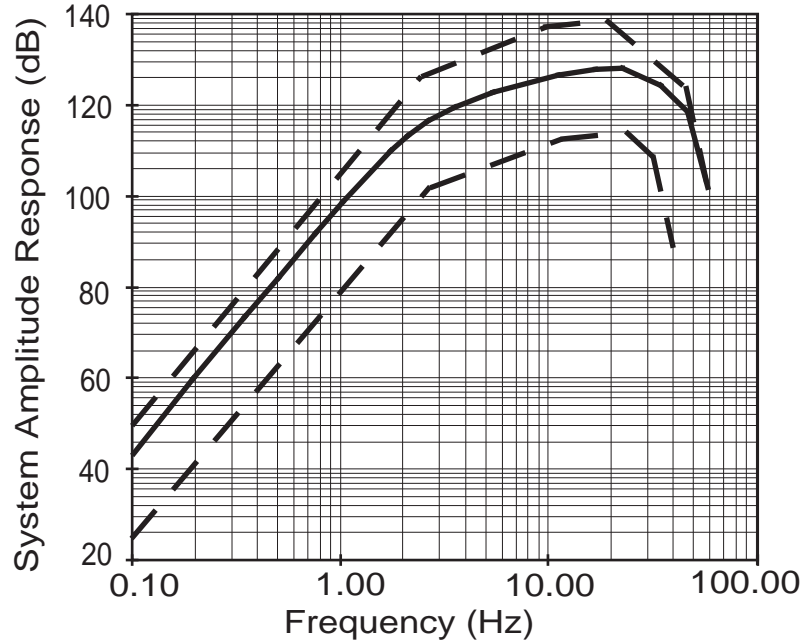
Figure 3. Log-log plot of representative displacement response curves for the short-period stations using a Mark Products L22 seismometer. The solid line illustrates the typical calibration curve and the dashed lines show the range of calibration curves for all AVO stations using L22 seismometers.
