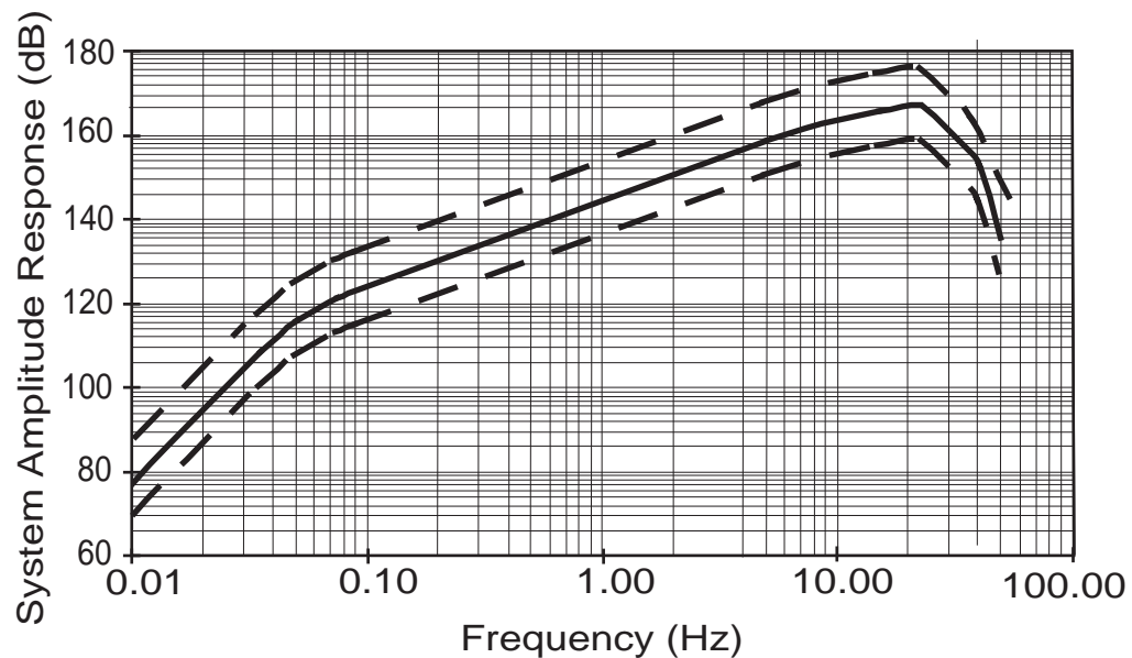
Figure 6. Log-log plot of representative displacement response curves for the broadband stations using a Guralp CMG-6TD seismometer. The solid line illustrates the typical calibration curve and the dashed lines show the range of calibration curves for all AVO stations using Guralp CMG-6TD seismometers.
