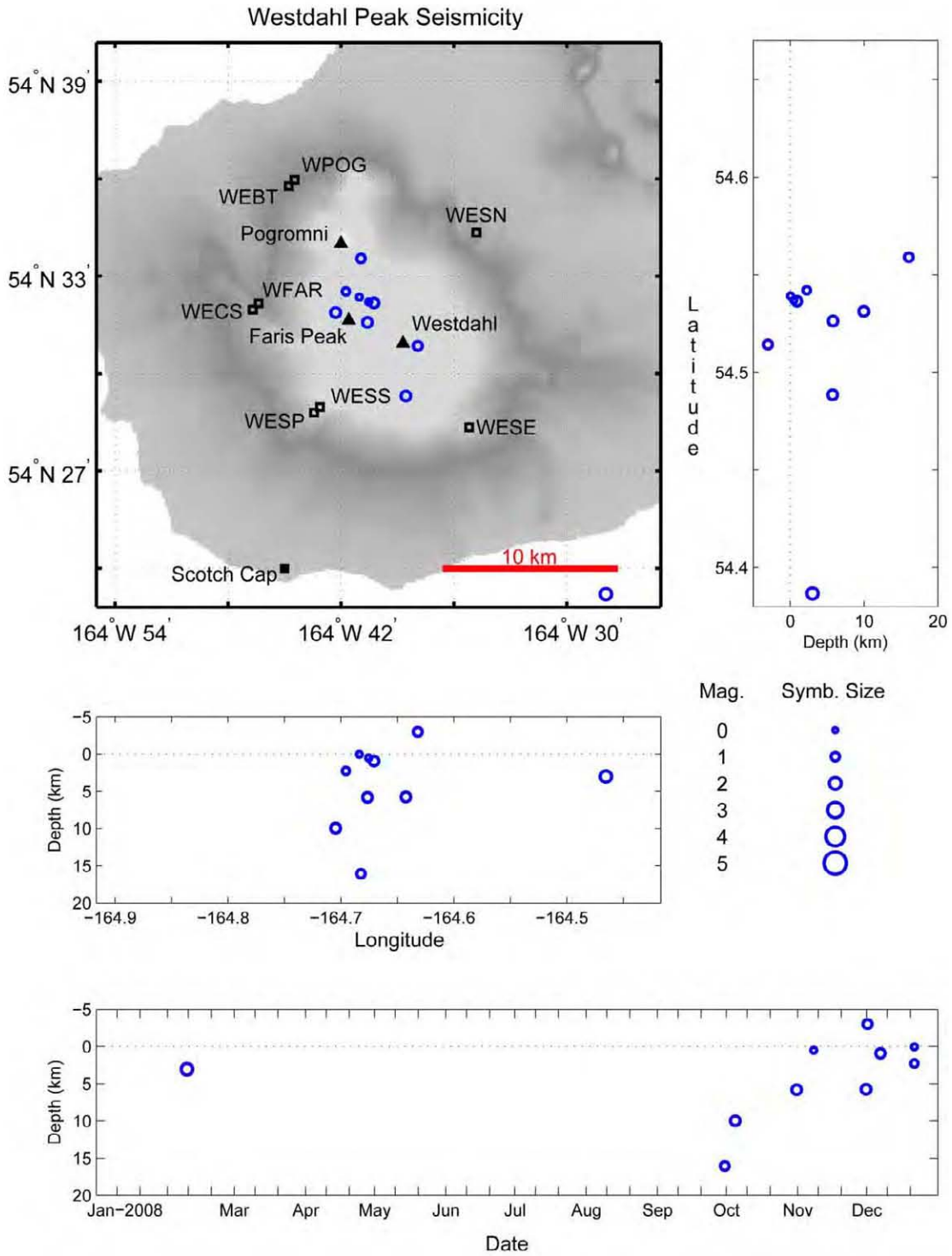
Figure A20. Summary plots of earthquakes located near Westdahl Peak in 2008. Open circles show hypocenter locations shallower than 20 km. Hypocenter symbols are scaled with magnitude. Permanent seismograph stations are shown by open squares and labeled by station code. Solid triangles are used to show volcanic centers and solid squares are used to show other points of interest. See appendix B for station information.
