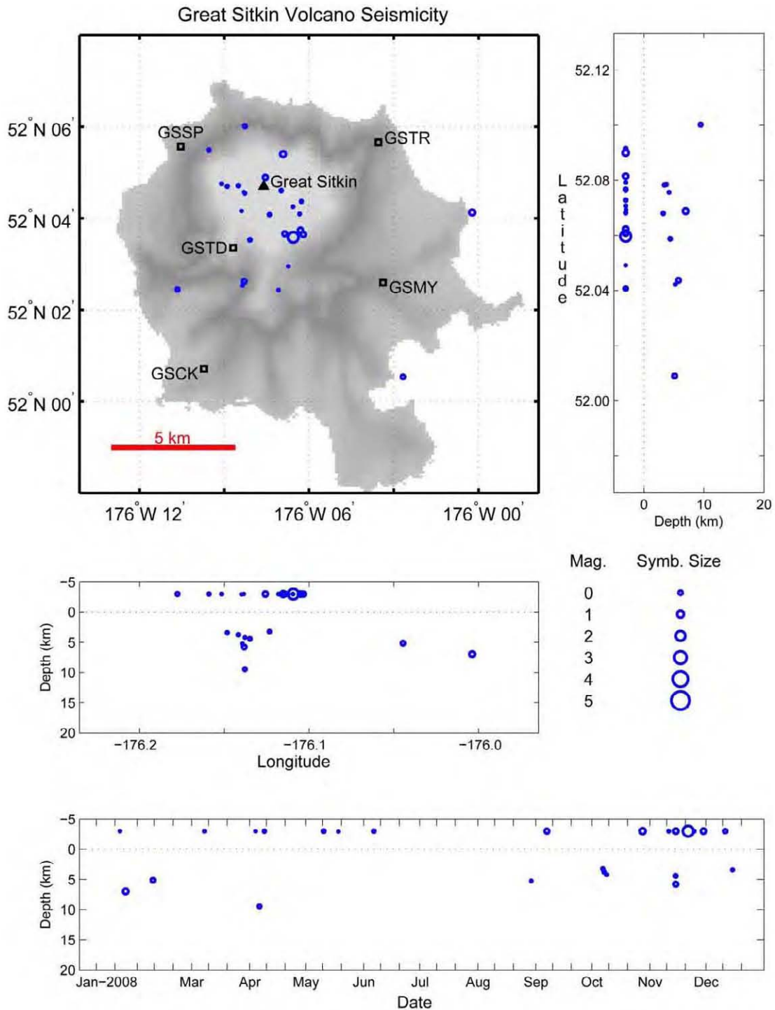
Figure A26. Summary plots of earthquakes located near Great Sitkin Volcano in 2008. Open circles show hypocenter locations shallower than 20 km. Hypocenter symbols are scaled with magnitude. Permanent seismograph stations are shown by open squares and labeled by station code. Solid triangles are used to show volcanic centers. See appendix B for station information.
