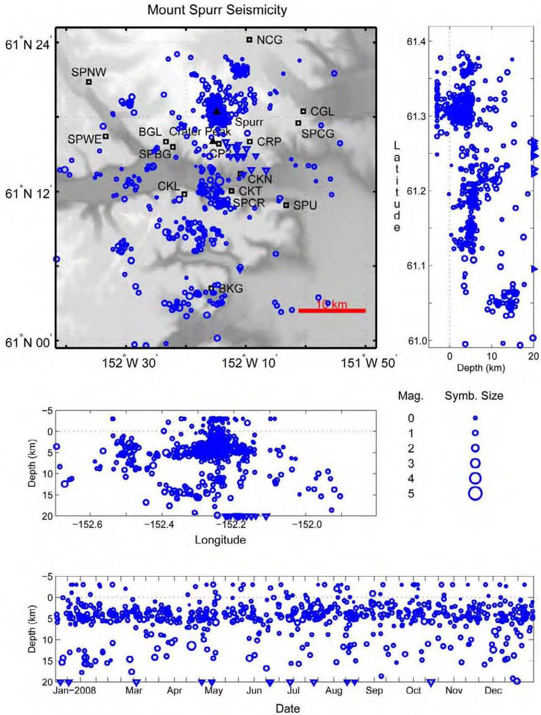
Figure A2. Summary plots of earthquakes located near Mount Spurr in 2008. Open circles show hypocenter locations shallower than 20 km and open triangles indicate times of hypocenters with depths of 20 km and deeper. Hypocenter symbols are scaled with magnitude. Permanent seismograph stations are shown by open squares and labeled by station code. Solid triangles are used to show volcanic centers. See appendix B for station information.
