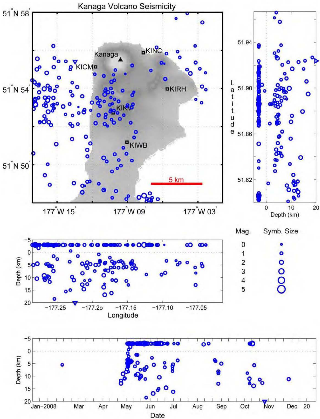
Figure A27. Summary plots of earthquakes located near Kanaga Volcano in 2008. Open circles show hypocenter locations shallower than 20 km and open triangles indicate times of hypocenters with depths of 20 km and deeper. Hypocenter symbols are scaled with magnitude. Permanent seismograph stations are shown by open squares and labeled by station code. Solid triangles are used to show volcanic centers. See appendix B for station information.
