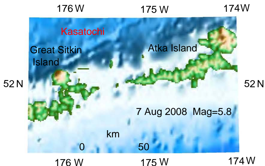
Figure 7. Earthquakes located by AEIC associated with the Kasatochi eruption (Ruppert, 2008b). The focal mechanism shown is for the largest earthquake ( M_w=5.8 ) shown by the star. Kasatochi Volcano is shown by the inverted triangle.
