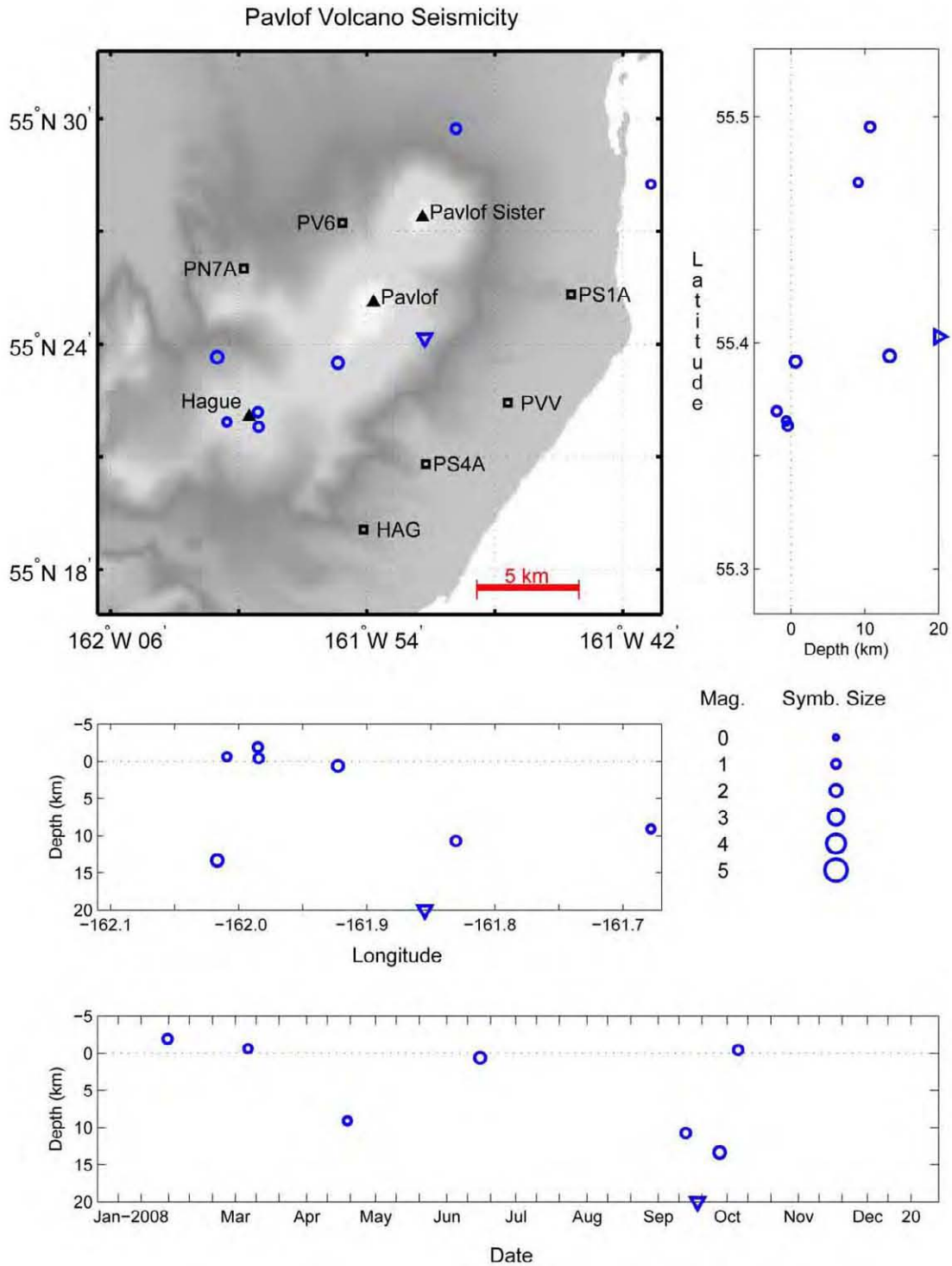
Figure A16. Summary plots of earthquakes located near Pavlof Volcano in 2008. Open circles show hypocenter locations shallower than 20 km and open triangles indicate times of hypocenters with depths of 20 km and deeper. Hypocenter symbols are scaled with magnitude. Permanent seismograph stations are shown by open squares and labeled by station code. Solid triangles are used to show volcanic centers. See appendix B for station information.
