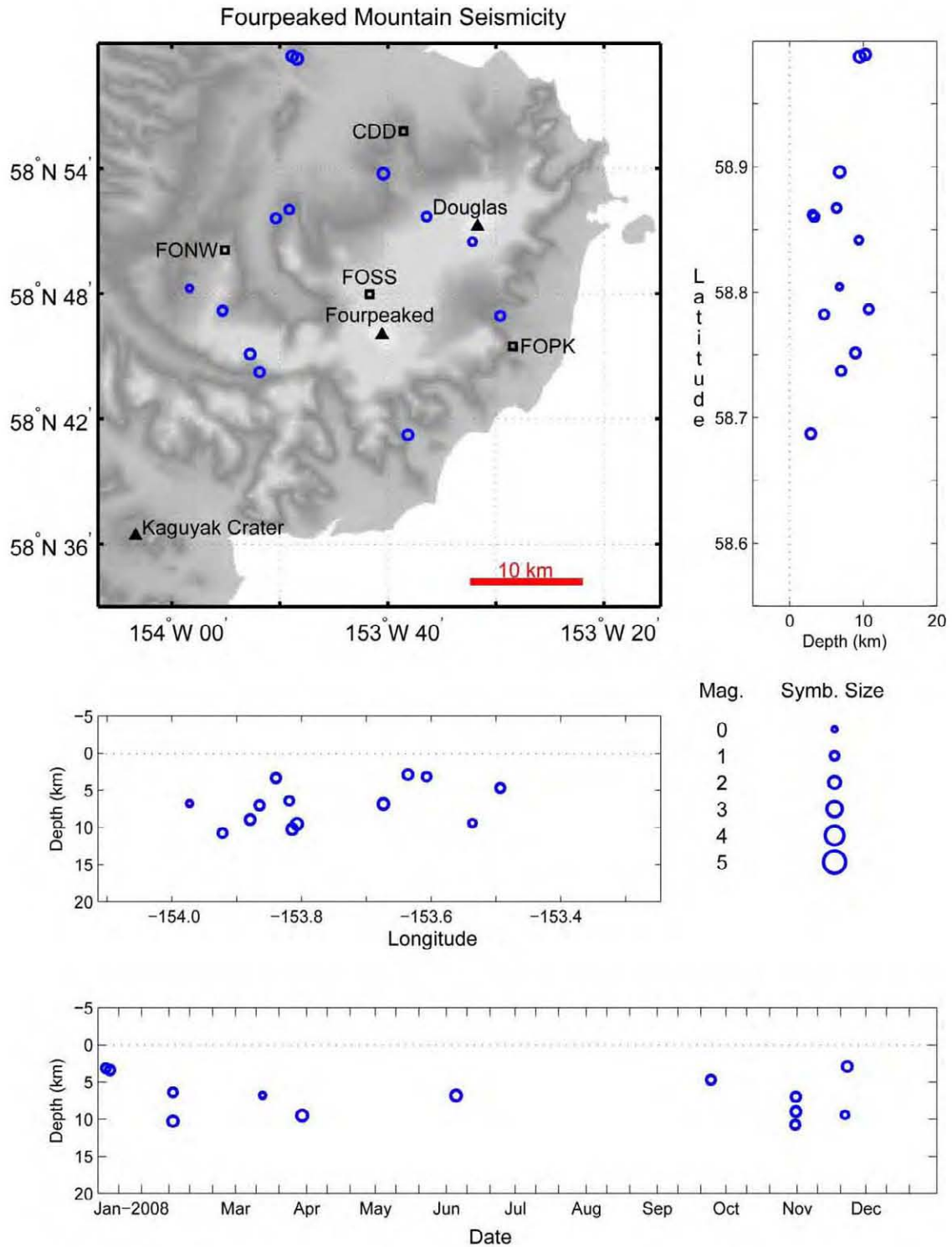
Figure A6. Summary plots of earthquakes located near Fourpeaked Mountain in 2008. Open circles show hypocenter locations shallower than 20 km. Hypocenter symbols are scaled with magnitude. Permanent seismograph stations are shown by open squares and labeled by station code. Solid triangles are used to show volcanic centers. See appendix B for station information.
