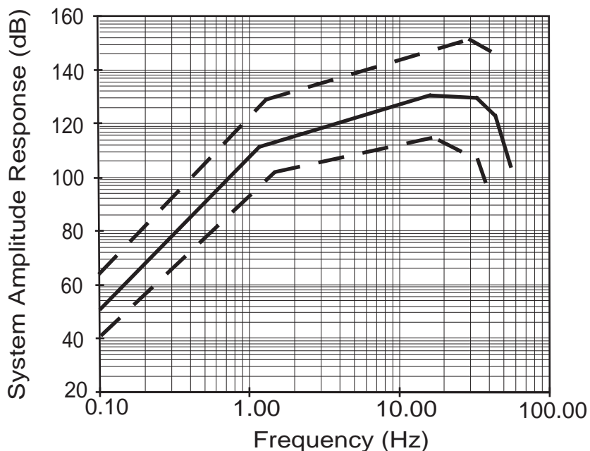
Figure 2. Log-log plot of representative displacement response curves for the short-period stations using a Mark Products L4 or L4-3D seismometer. The solid line illustrates the typical calibration curve and the dashed lines show the range of calibration curves for all AVO stations using L4 or L4-3D seismometers.
