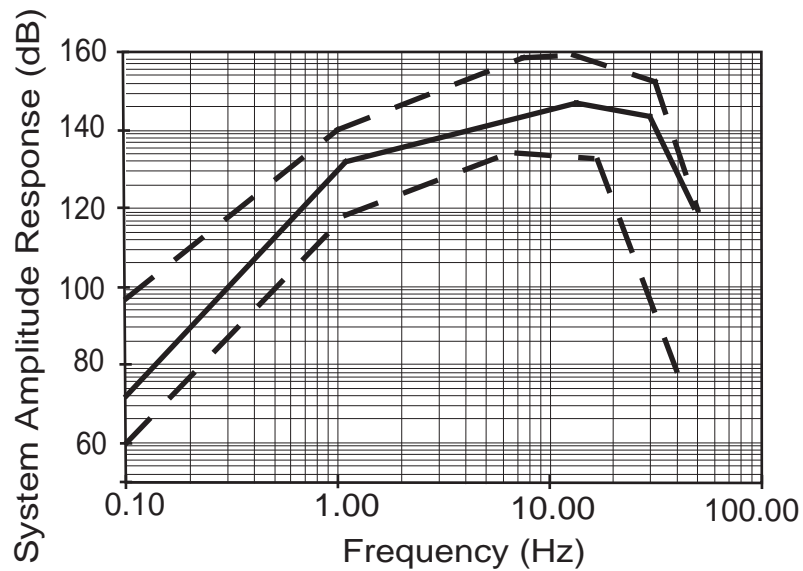
Figure 4. Log-log plot of representative displacement response curves for the short-period stations using a Teledyne-Geotech S13 seismometer. The solid line illustrates the typical calibration curve and the dashed lines show the range of calibration curves for all AVO stations using S13 seismometers.
