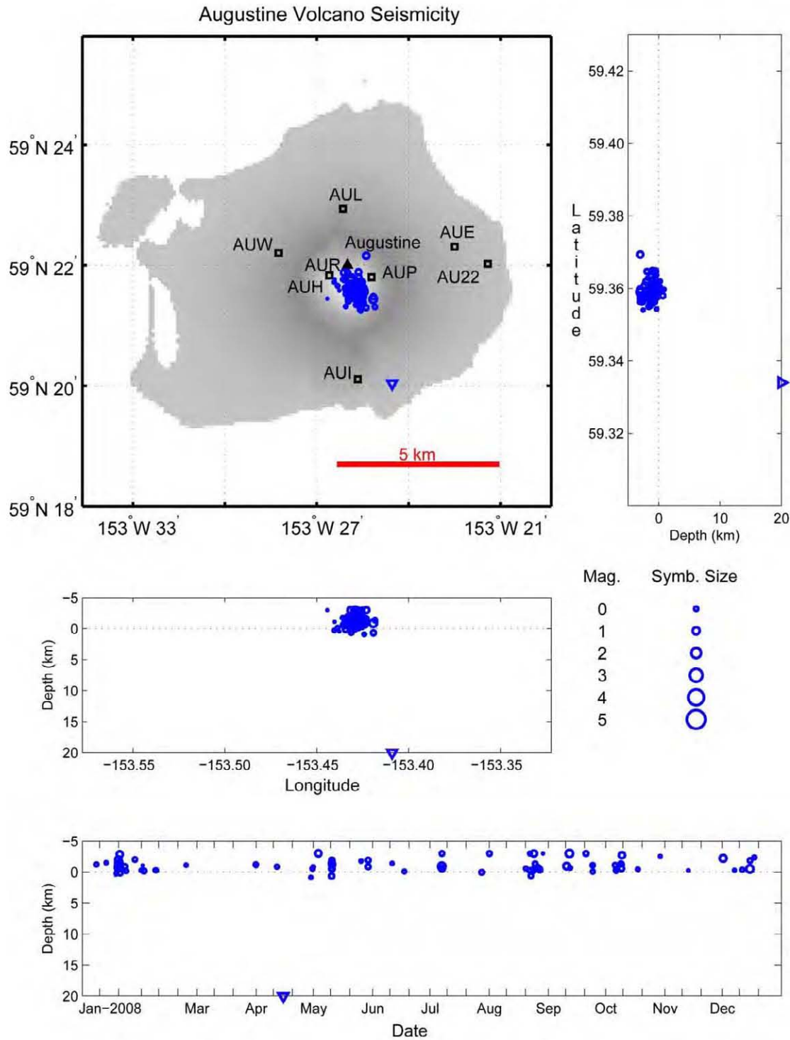
Figure A5. Summary plots of earthquakes located near Augustine Volcano in 2008. Open circles show hypocenter locations shallower than 20 km and open triangles indicate times of hypocenters with depths of 20 km and deeper. Hypocenter symbols are scaled with magnitude. Permanent seismograph stations are shown by open squares and labeled by station code. Solid triangles are used to show volcanic centers. See appendix B for station information.
