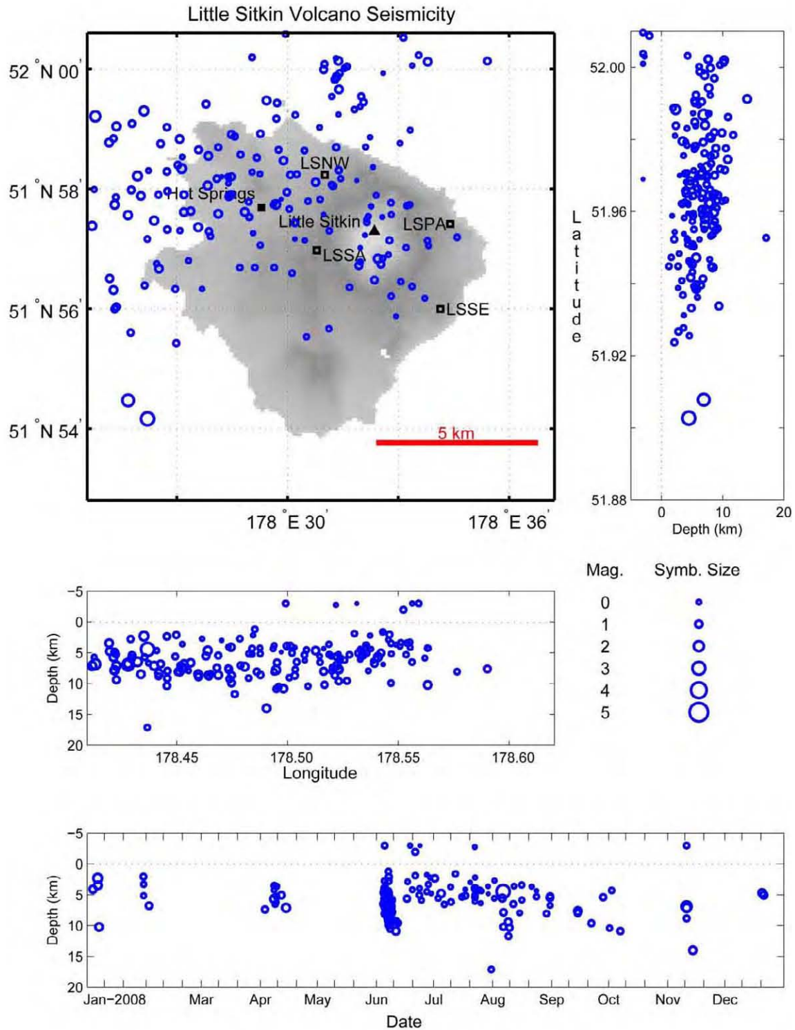
Figure A32. Summary plots of earthquakes located near Little Sitkin Volcano in 2008. Open circles show hypocenter locations shallower than 20 km. Hypocenter symbols are scaled with magnitude. Permanent seismograph stations are shown by open squares and labeled by station code. Solid triangles are used to show volcanic centers. See appendix B for station information.
