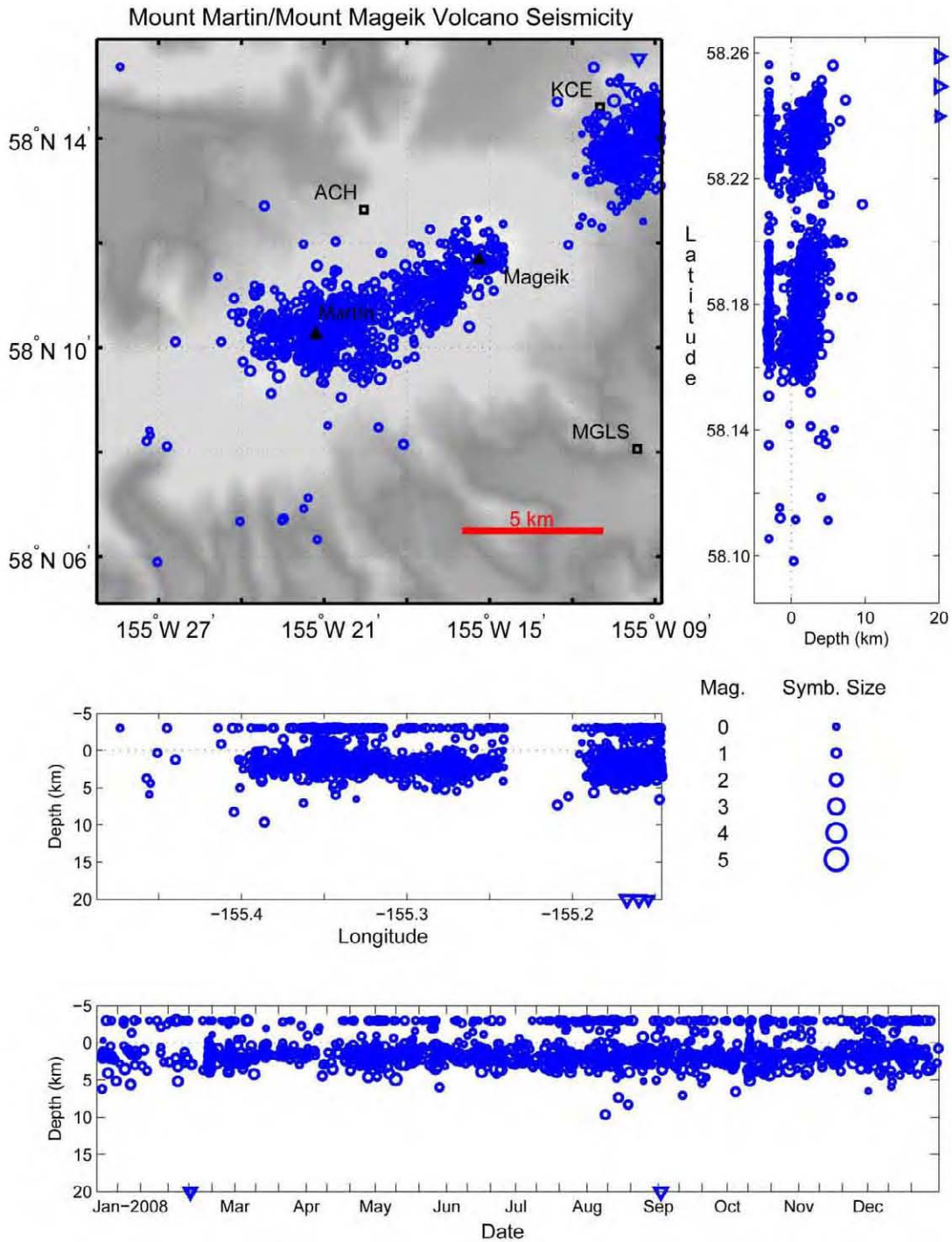
Figure A12. Summary plots of earthquakes located near Mount Mageik and Mount Martin in the Katmai volcanic cluster in 2008. Open circles show hypocenter locations shallower than 20 km and open triangles indicate times of hypocenters with depths of 20 km and deeper. Hypocenter symbols are scaled with magnitude. Permanent seismograph stations are shown by open squares and labeled by station code. Solid triangles are used to show volcanic centers. See appendix B for station information. Several earthquakes that appear on this figure appear on other figures.
