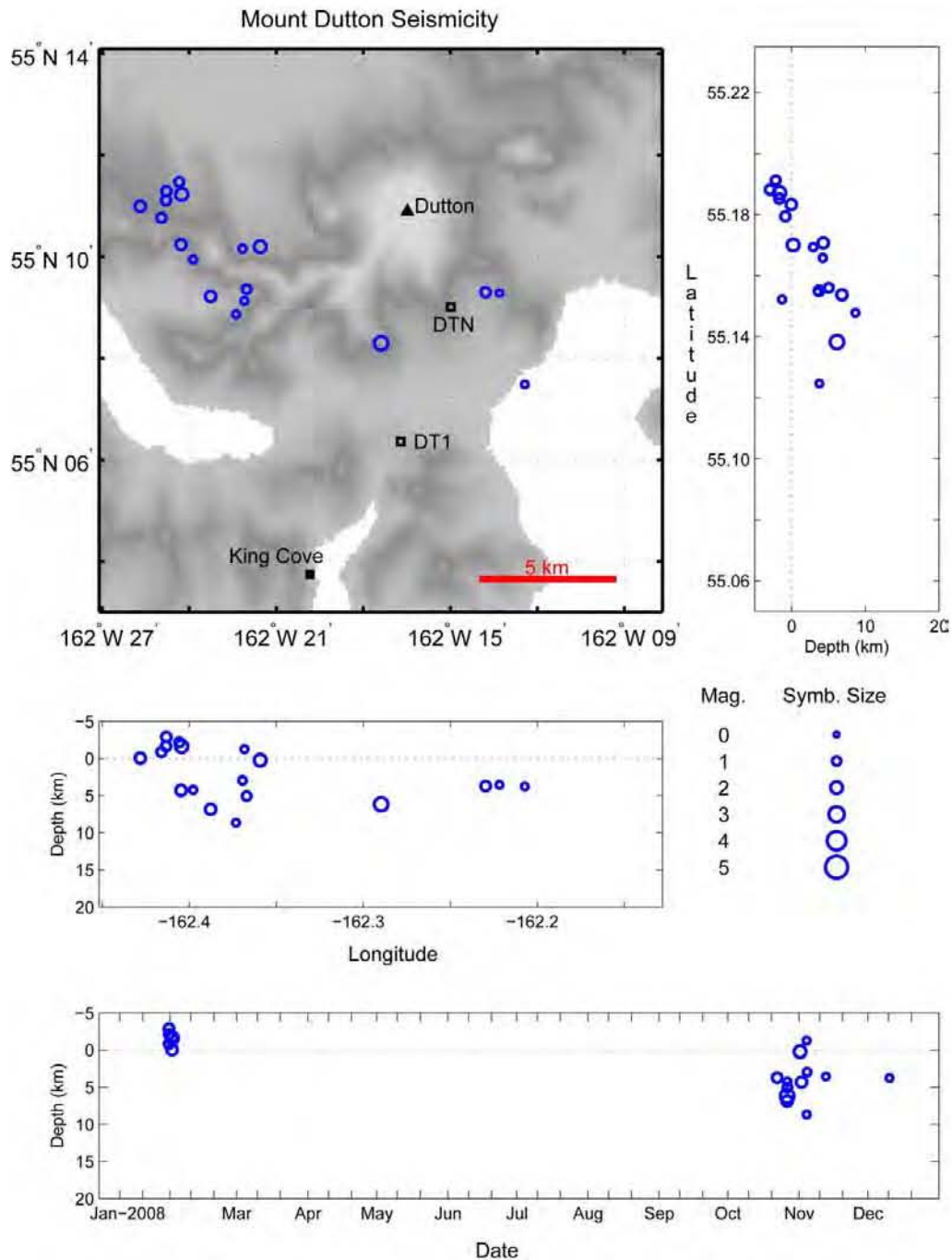
Figure A17. This summary plot shows earthquakes located near Mount Dutton in 2008. Open circles show hypocenter locations shallower than 20 km. Hypocenter symbols are scaled with magnitude. Permanent seismograph stations are shown by open squares and labeled by station code. Solid triangles are used to show volcanic centers and solid squares are used to show other points of interest. See appendix B for station information.
