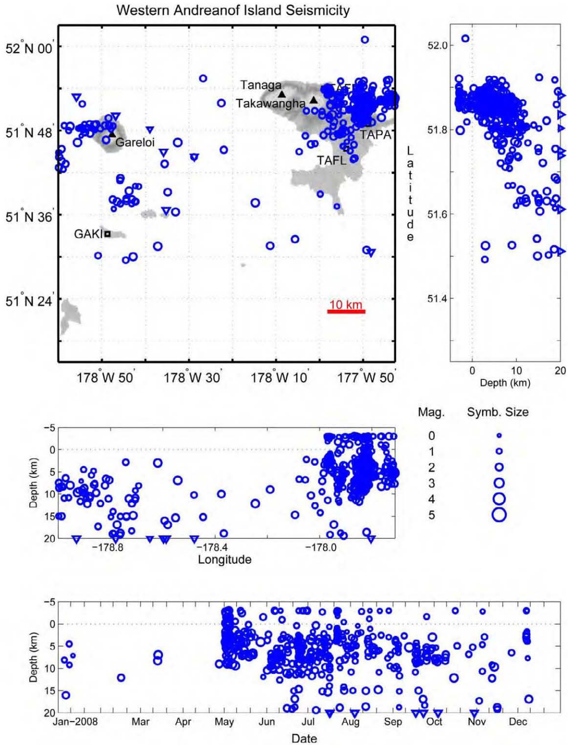
Figure A28. Summary plots of earthquakes located in the Western Andreanof Islands in 2008. Open circles show hypocenter locations shallower than 20 km and open triangles indicate times of hypocenters with depths of 20 km and deeper. Hypocenter symbols are scaled with magnitude. Permanent seismograph stations are shown by open squares and labeled by station code. Solid triangles are used to show volcanic centers. See appendix B for station information.
