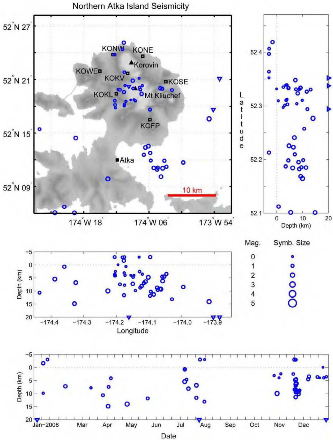
Figure A24. Summary plots of earthquakes located near Korovin Volcano and Mount Kliuchef in 2008. Open circles show hypocenter locations shallower than 20 km and open triangles indicate times of hypocenters with depths of 20 km and deeper. Hypocenter symbols are scaled with magnitude. Permanent seismograph stations are shown by open squares and labeled by station code. Solid triangles are used to show volcanic centers and solid squares are used to show other points of interest. See appendix B for station information.
