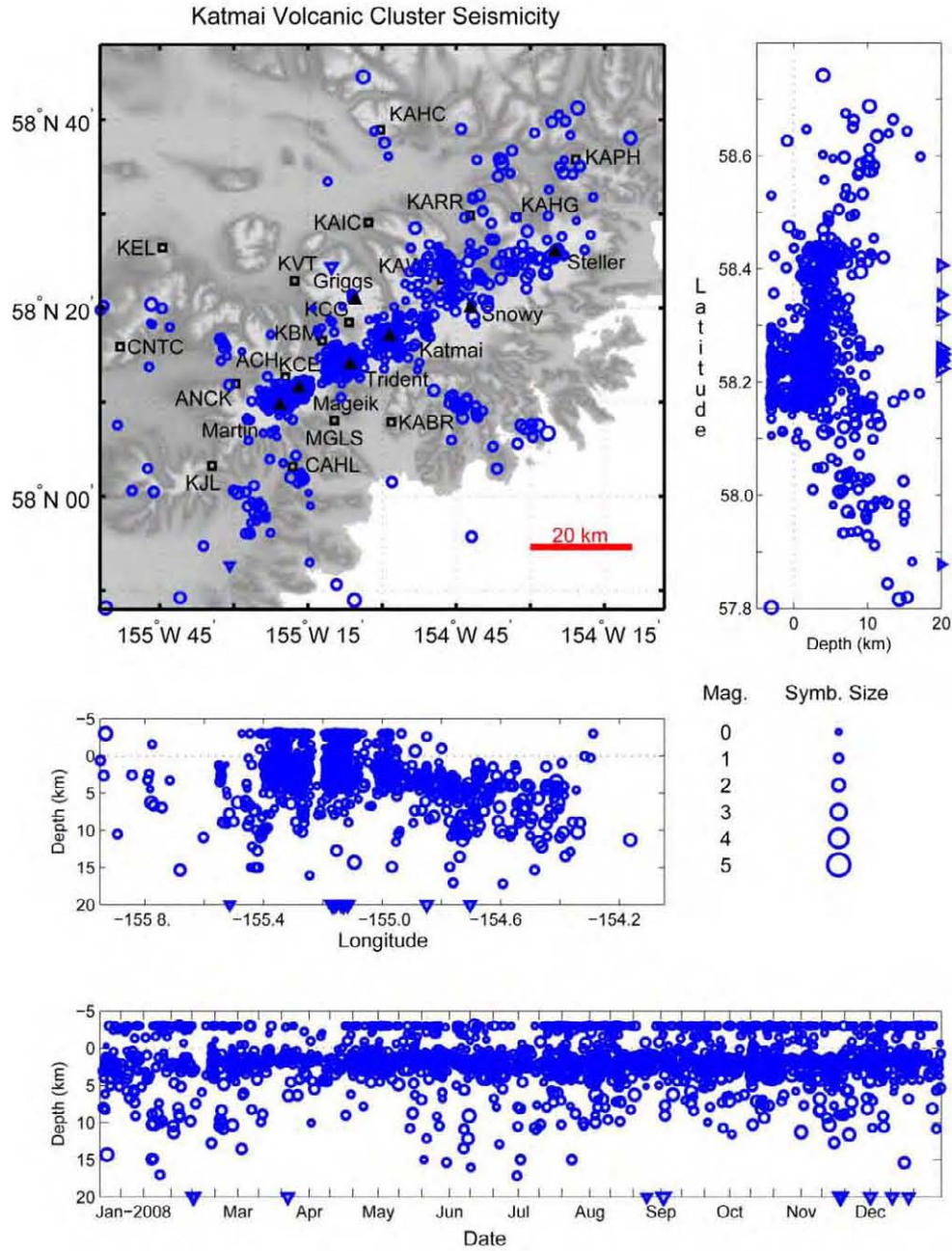
Figure A7. Summary plots of earthquakes located near the Katmai volcanic cluster in 2008. Open circles show hypocenter locations shallower than 20 km and open triangles indicate times of hypocenters with depths of 20 km and deeper. Hypocenter symbols are scaled with magnitude. Permanent seismograph stations are shown by open squares and labeled by station code. Solid triangles are used to show volcanic centers. See appendix B for station information.
