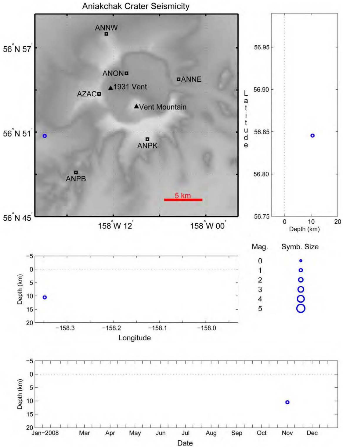
Figure A14. Summary plots of earthquakes located near Aniakchak Crater in 2008. Open circles show hypocenter locations shallower than 20 km. Hypocenter symbols are scaled with magnitude. Permanent seismograph stations are shown by open squares and labeled by station code. Solid triangles are used to show volcanic centers. See appendix B for station information.
