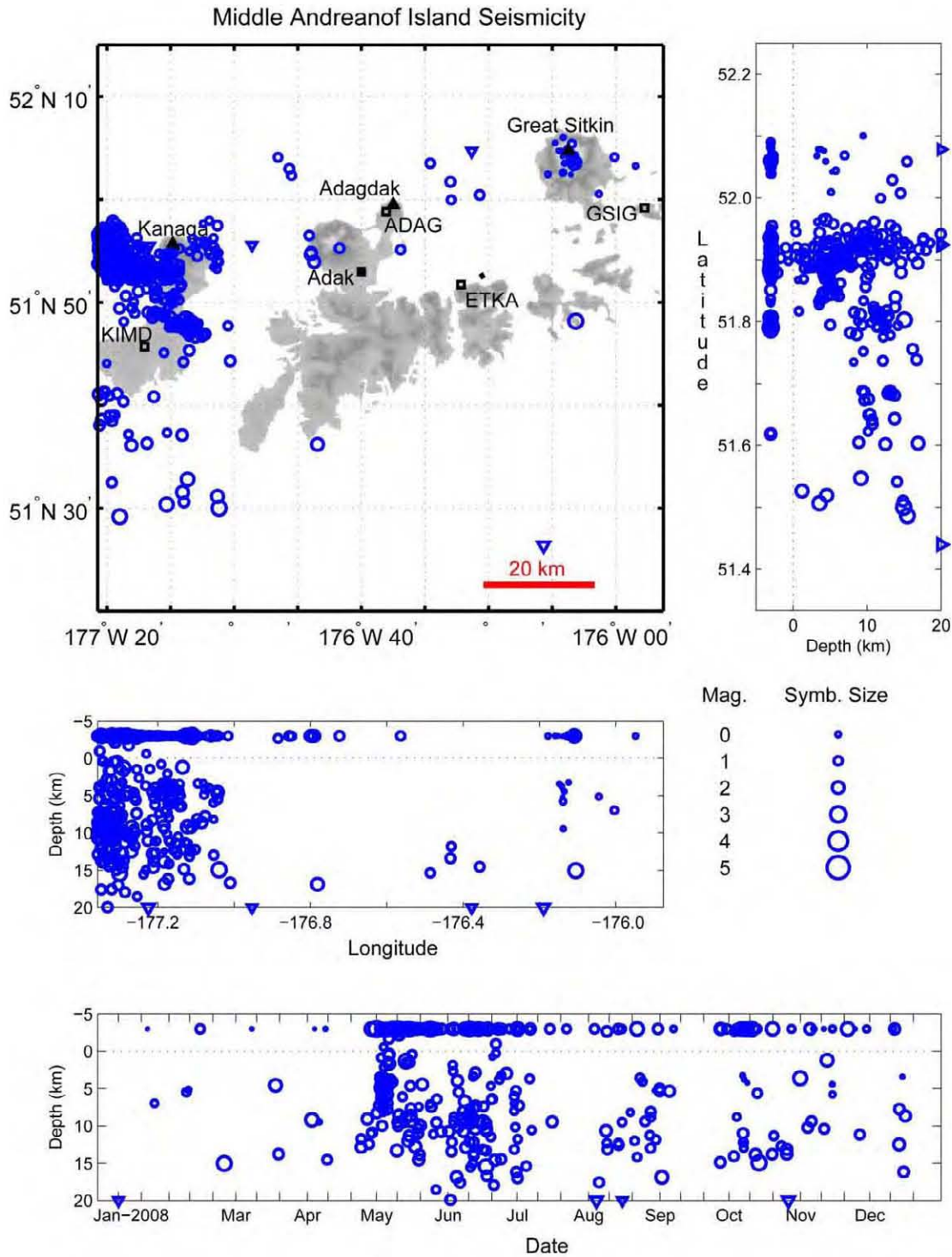
Figure A25. Summary plots of earthquakes located in the Middle Andeanof Islands in 2008. Open circles show hypocenter locations shallower than 20 km and open triangles indicate times of hypocenters with depths of 20 km and deeper. Hypocenter symbols are scaled with magnitude. Permanent seismograph stations are shown by open squares and labeled by station code. Solid triangles are used to show volcanic centers and solid squares are used to show other points of interest. See appendix B for station information.
