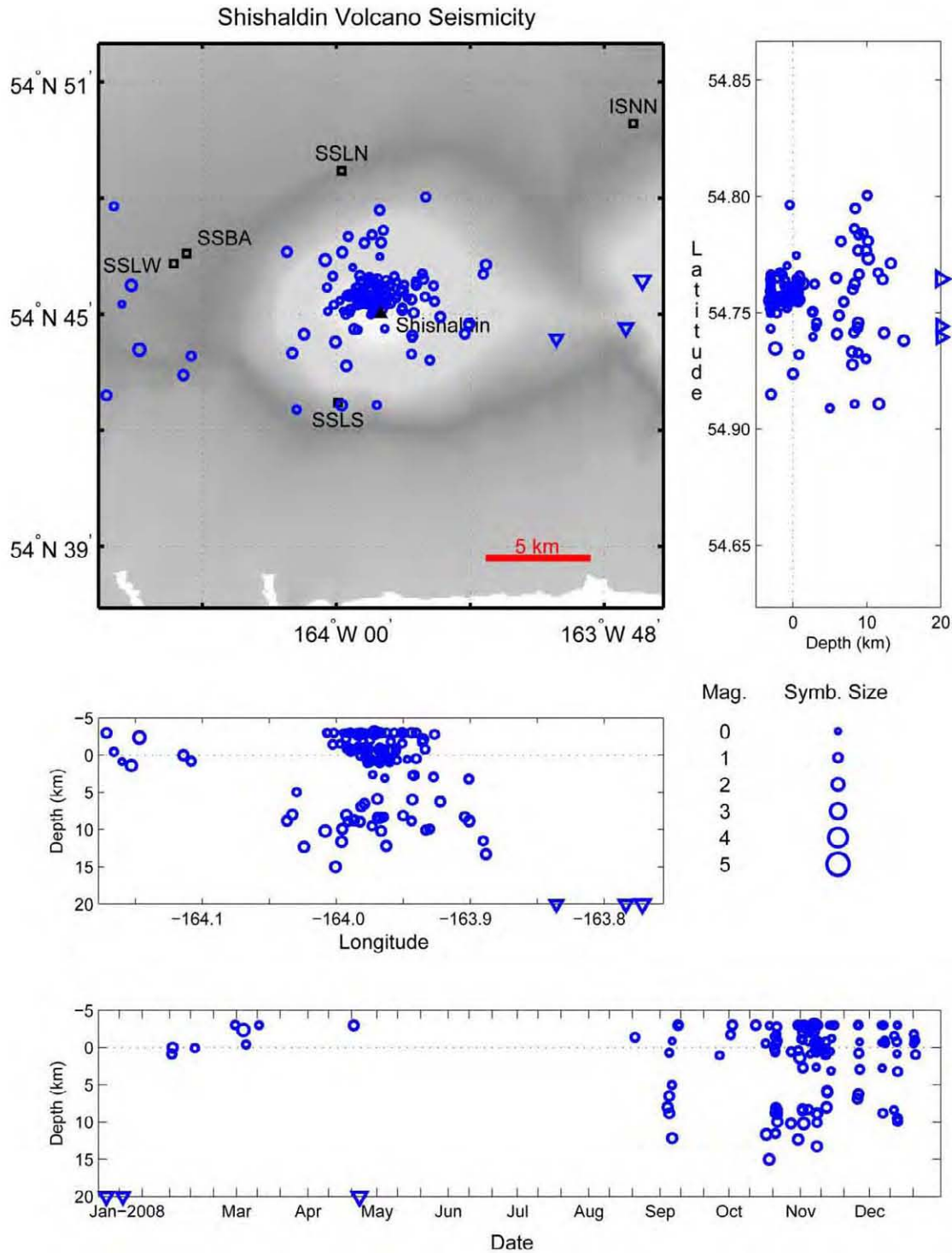
Figure A19. Summary plots of earthquakes located near Shishaldin Volcano in 2008. Open circles show hypocenter locations shallower than 20 km and open triangles indicate times of hypocenters with depths of 20 km and deeper. Hypocenter symbols are scaled with magnitude. Permanent seismograph stations are shown by open squares and labeled by station code. Solid triangles are used to show volcanic centers. See appendix B for station information.
